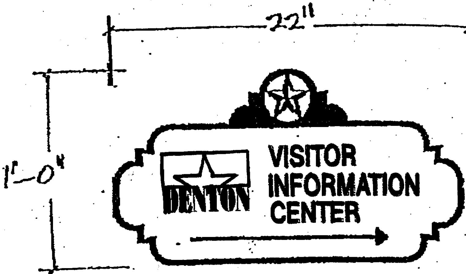
SIGN - TYPE "B"
