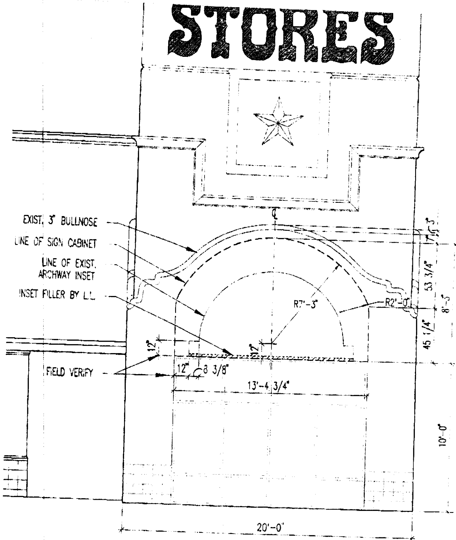
TOWER #1 VISITOR INFORMATION SIGNAGE DIMENSIONAL LAYOUT CONTROL - SHEET 2A
