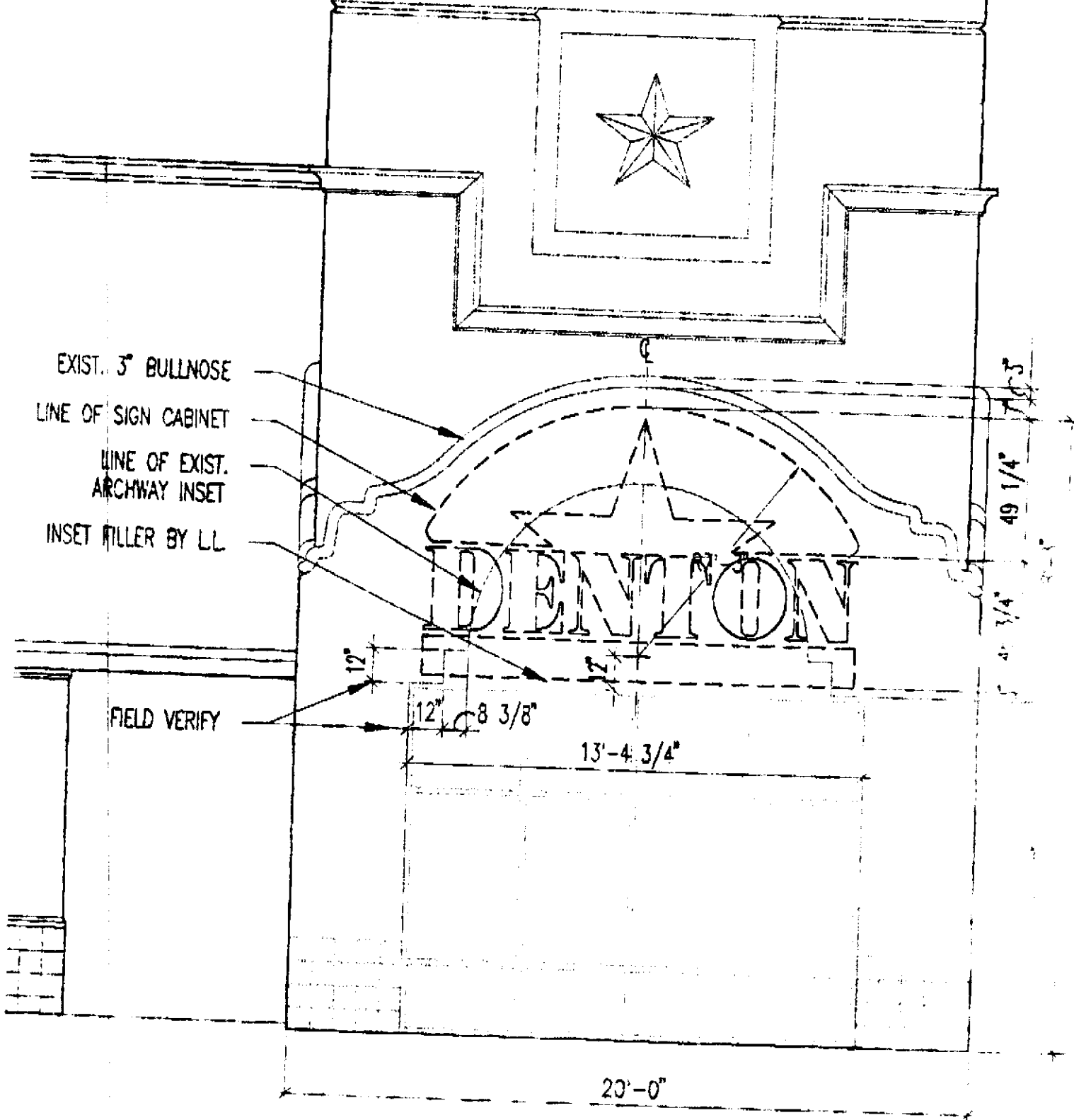
TOWER #1 VISITOR INFORMATION SIGNAGE DIMENSIONAL LAYOUT CONTROL - SHEET 3A
