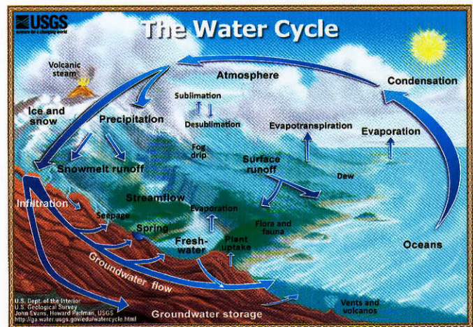
Figure 2.2 - The Hydrologic Cycle. Diagram courtesy of the USGS.
