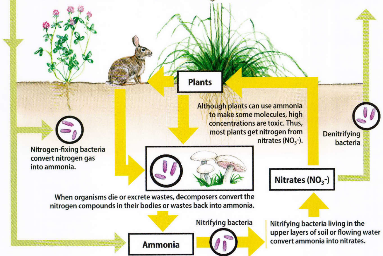
Figure 3.3 - Physical and biological components of the nitrogen cycle. Image used with permission from the Missouri Department of Conservation.
