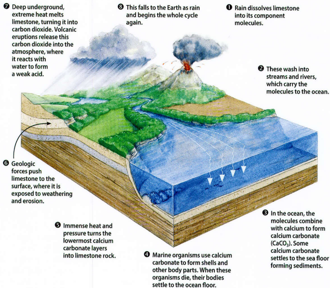
Figure 4.4 - Geological Carbon Cycle. Image used with permission from the Missouri Department of Conservation.
