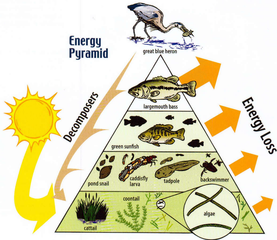
Figure 3.2 - Energy Transfer and Losses. Image used with permission from the Missouri Department of Conservation.
