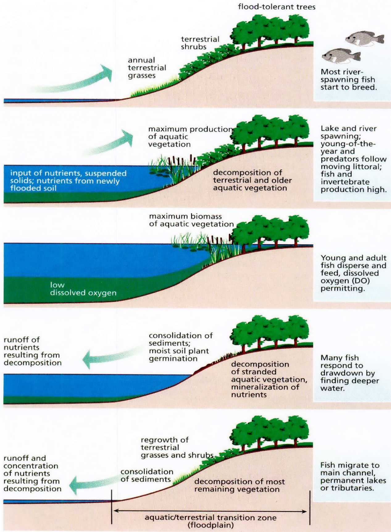
Figure 5.4 - The flood-pulse concept diagrammed in five stages of an annual hydrologic cycle. The left column describes nutrient movement, the right describes typical life history traits of fish. From Bayley, P. BioScience vol 45 no 3, p. 154, March 1995. ©1995 American by permission of Oxford University Press.
