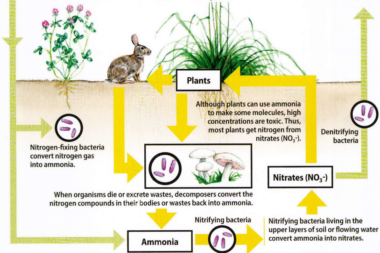
Figure 4.3 - This graphic, introduced in chapter 3, is shown here again to show the important role that decomposers like bacteria, fungi, microbes, and more play in the nitrogen cycle. Image used with permission from the Missouri Department of Conservation.
