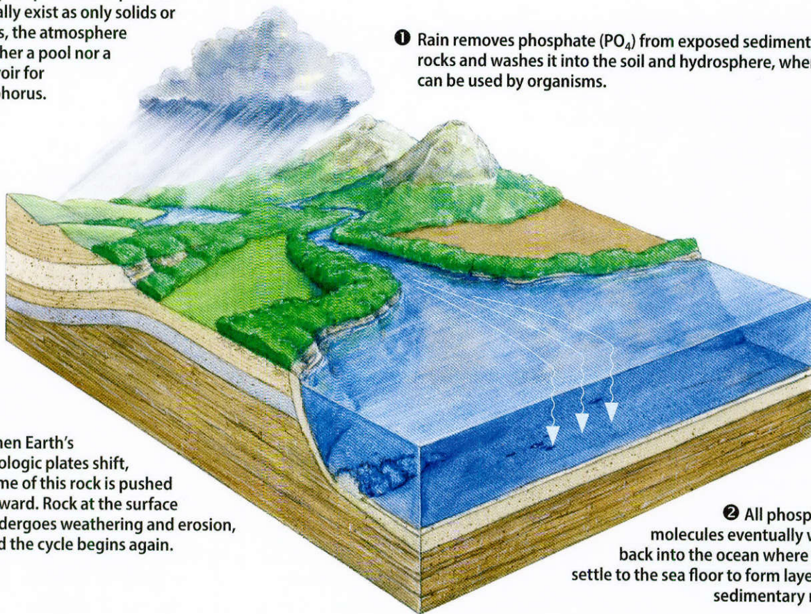
Figure 3.4 - Phosphorus cycle. Image used with permission from the Missouri Department of Conservation.
