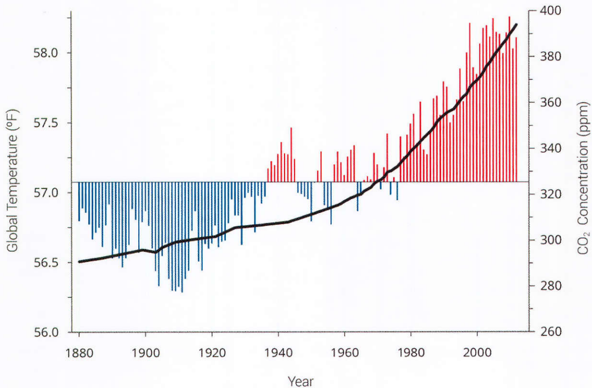
Figure 8.21 - Global temperature and carbon dioxide concentration. Image courtesy of the National Climate Assessment report 2014.
