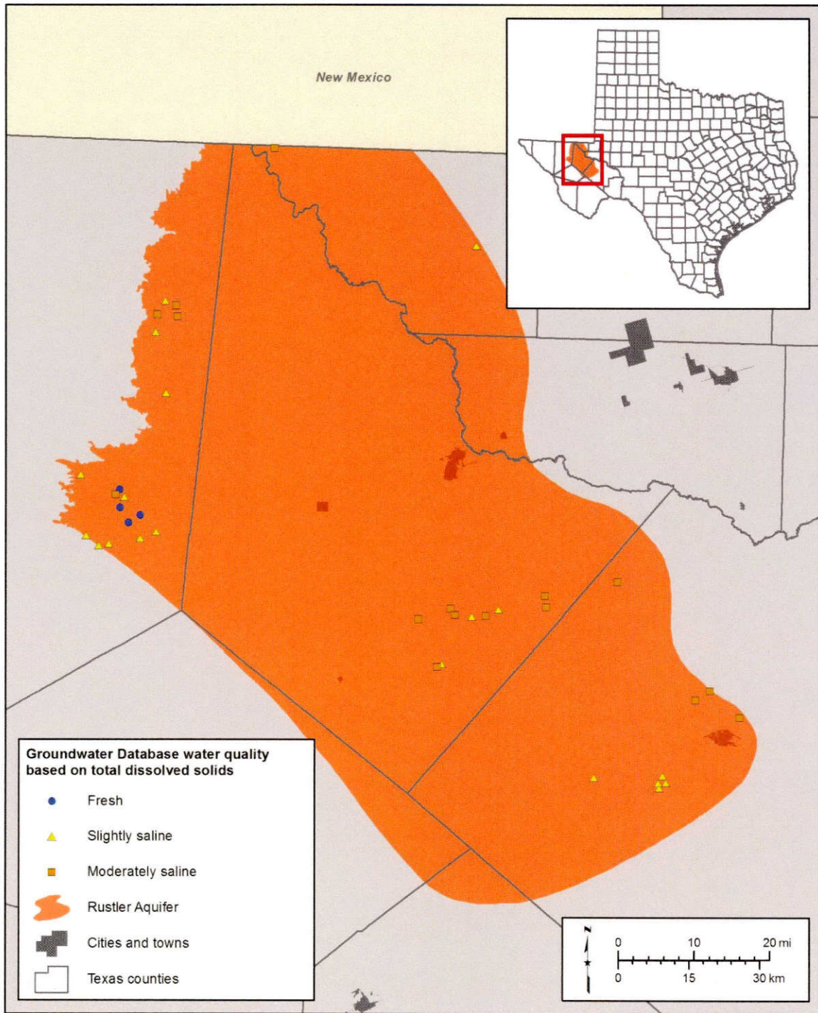
Figure D-6. Salinity (total dissolved solids) of water samples from the Rustler Aquifer based on the most recent samples in the TWDB Groundwater Database. Fresh (0 to 999 milligrams per liter total dissolved solids), slightly saline (1,000 to 2,999 milligrams per liter total dissolved solids), and moderately saline (3,000 to 9,999 milligrams per liter total dissolved solids).
