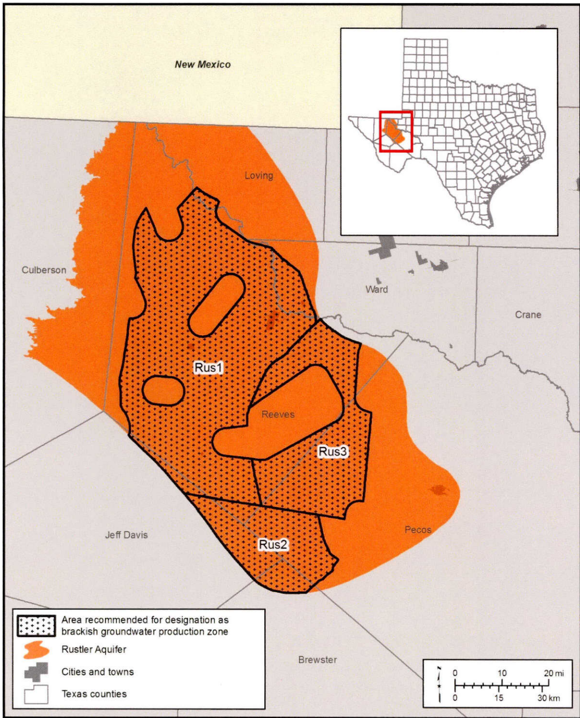
Figure D-1. The TWDB designated three brackish groundwater production zones within the Rustler Aquifer (Rus1, Rus2, and Rus3). The zones contain slightly to moderately saline groundwater (1,000 to 9,999 milligrams per liter of total dissolved solids).
