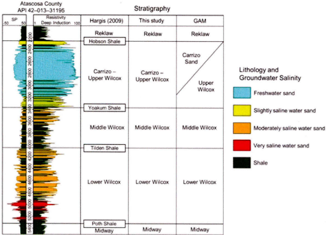
Figure 10. Stratigraphic subdivision of the Carrizo-Wilcox Aquifer in the project area.
