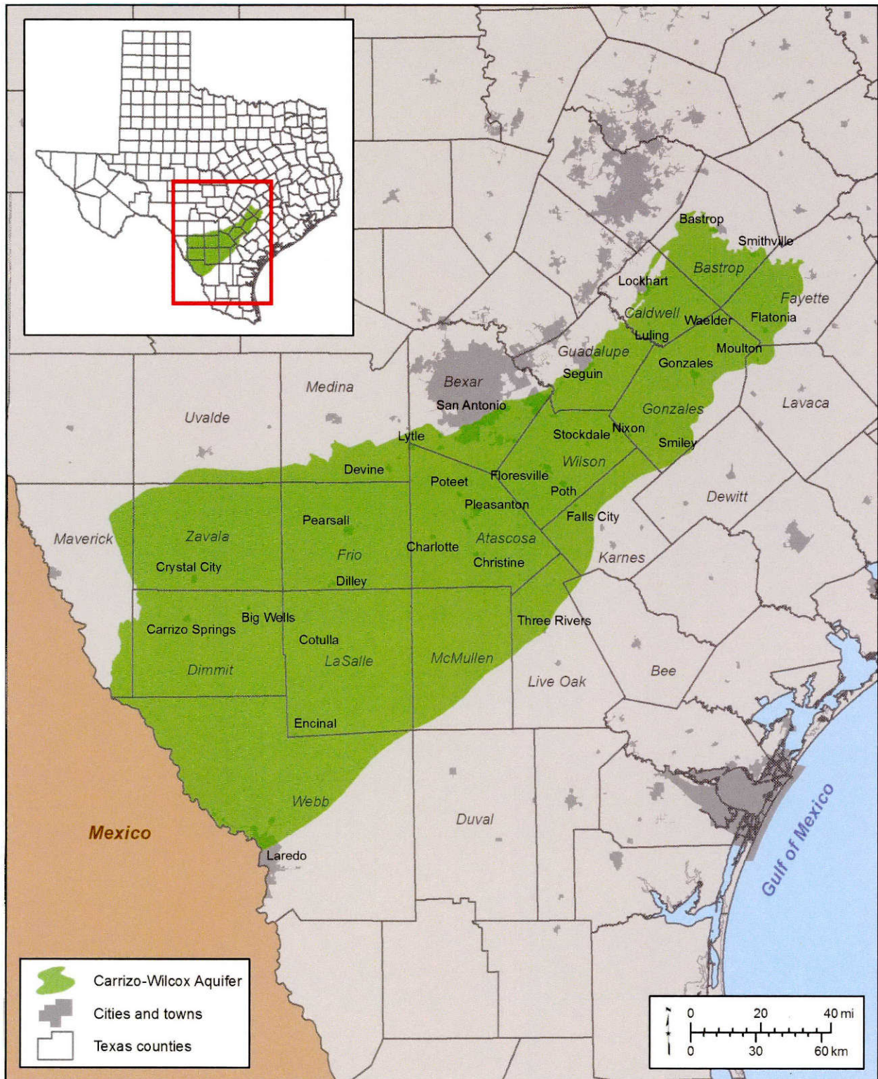
Figure A-1. The extent of the Carrizo-Wilcox Aquifer project area. The northeastern extent of the Carrizo-Wilcox Aquifer is not shown.
