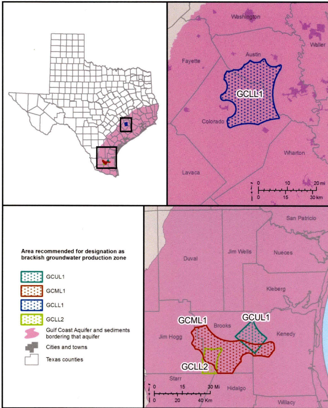
Figure B-5. Gulf Coast Aquifer, sediments bordering that aquifer, and four brackish groundwater production zones (GCUL1, GCML1, GCLL1, and GCLL2). The areas contain groundwater that is slightly to moderately saline (1,000 to 9,999 milligrams per liter of total dissolved solids).
