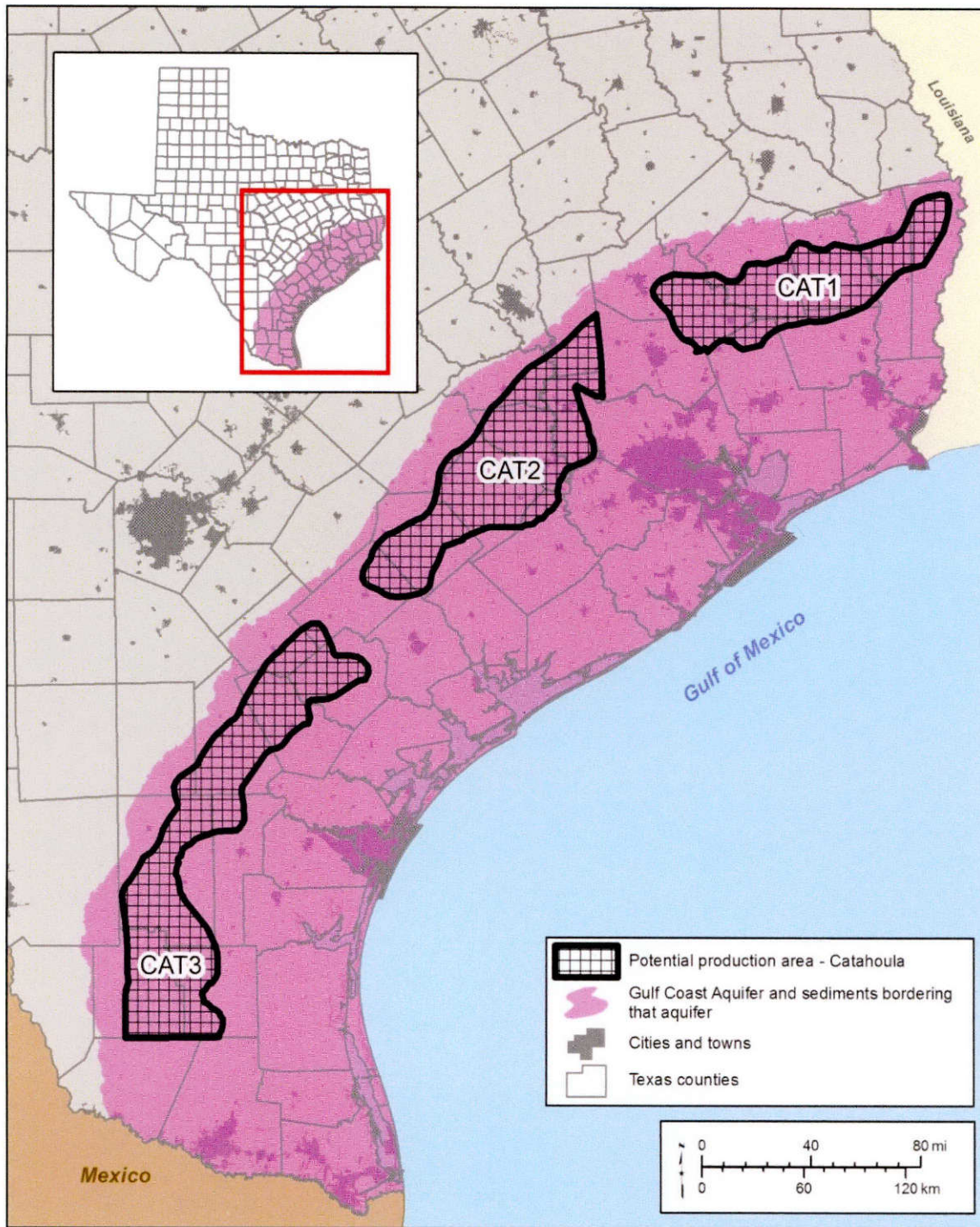
Figure B-12. Potential production areas in the Catahoula Formation in the Gulf Coast Aquifer System.
