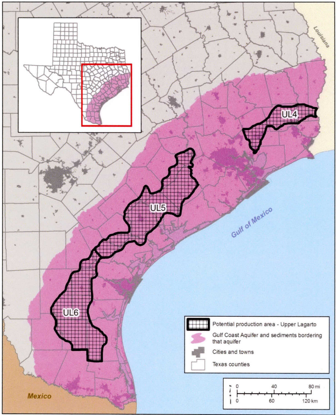
Figure B-8. Potential production areas in the Upper Lagarto Formation in the Gulf Coast Aquifer System.
