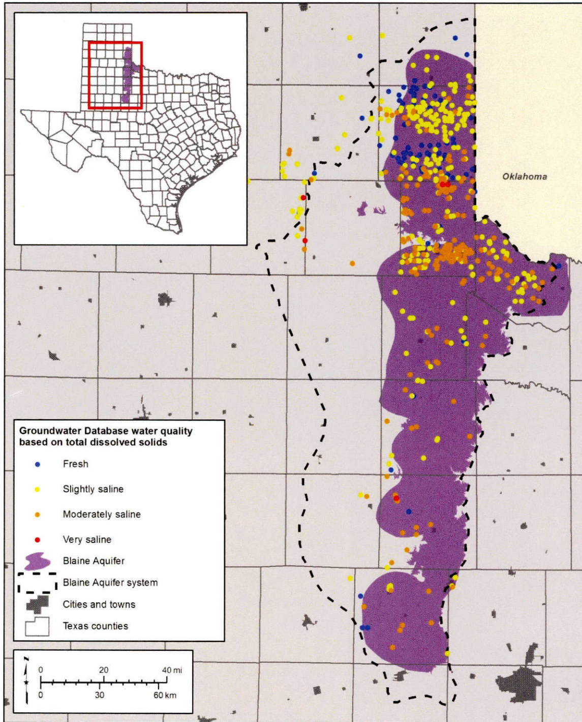
Figure C-5. Salinity (total dissolved solids) of water samples from the Blaine Aquifer and Whitehorse Group based on the most recent samples in the TWDB Groundwater Database. Fresh (0 to 999 milligrams per liter total dissolved solids), slightly saline (1,000 to 2,999 milligrams per liter total dissolved solids), moderately saline (3,000 to 9,999 milligrams per liter total dissolved solids), and very saline (10,000 to 35,000 milligrams per liter total dissolved solids).
