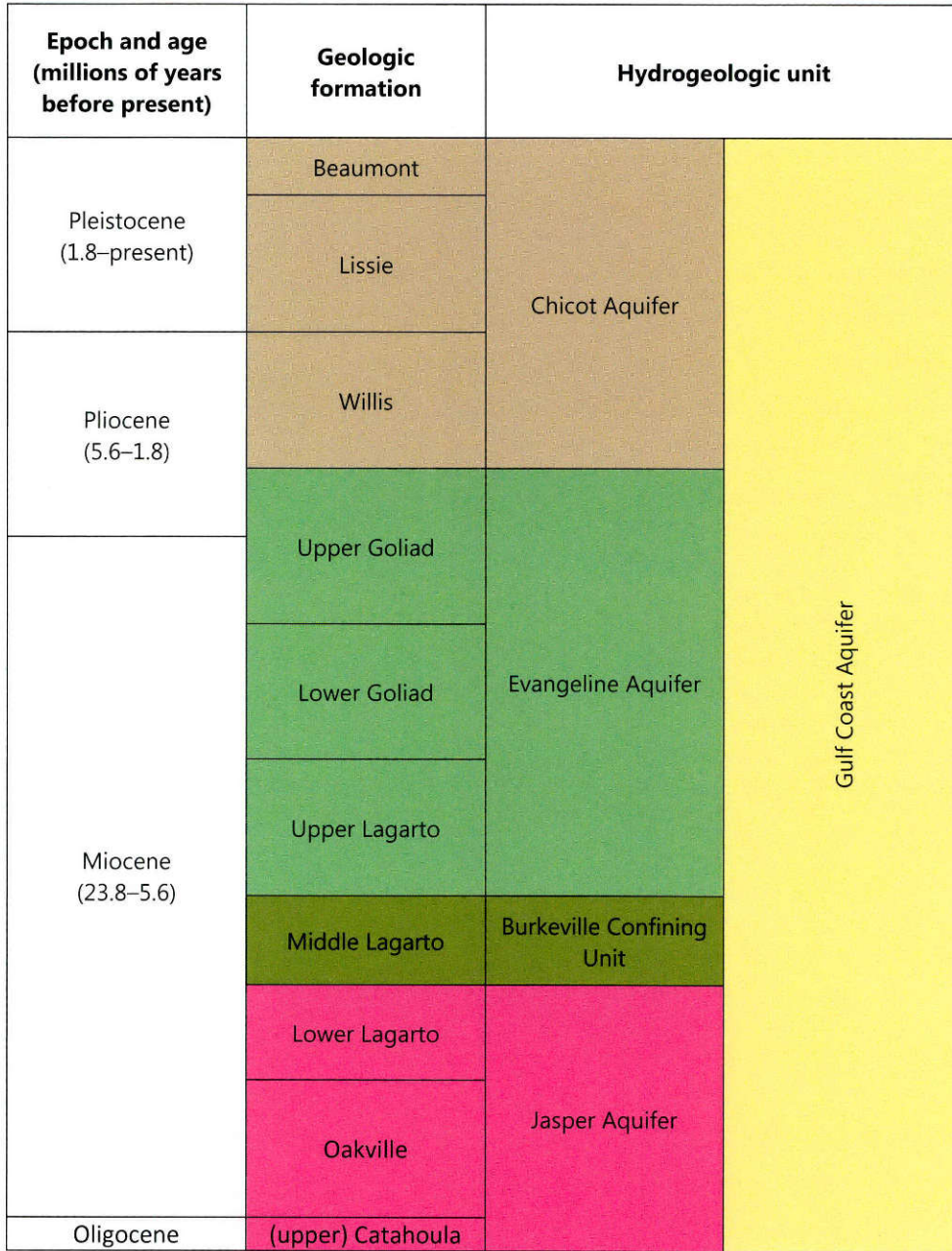
Figure 11. Stratigraphy and hydrostratigraphy of the Gulf Coast Aquifer system in the project area.
