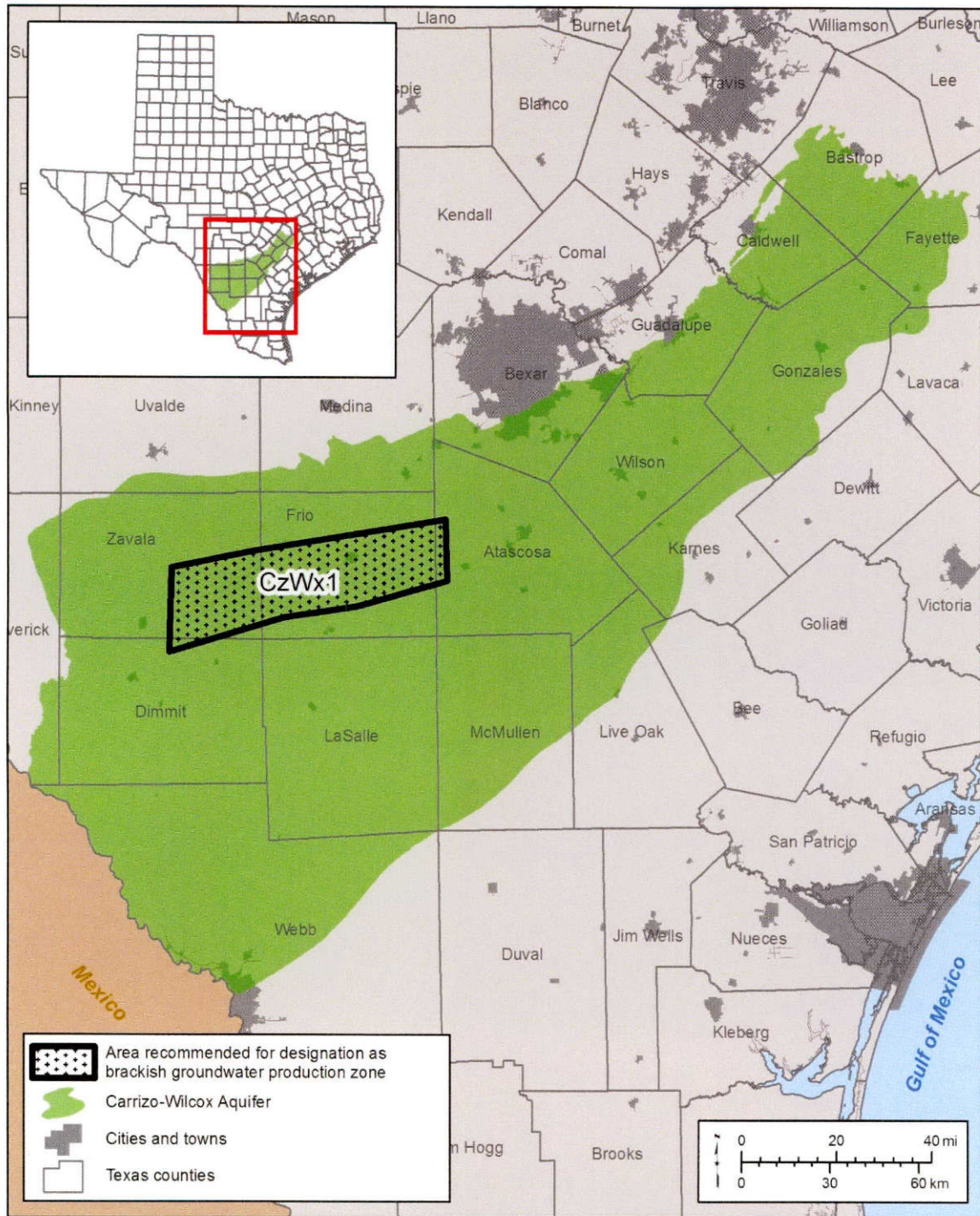
Figure A-4. Carrizo-Wilcox Aquifer located between the Colorado River and the Rio Grande. The TWDB designated one brackish groundwater production zone (CzWx1) within the lower Wilcox Formation. The zone contains slightly saline (1,000 to 2,999 milligrams per liter of total dissolved solids) to moderately saline (3,000 to 9,999 milligrams per liter of total dissolved solids) groundwater.
