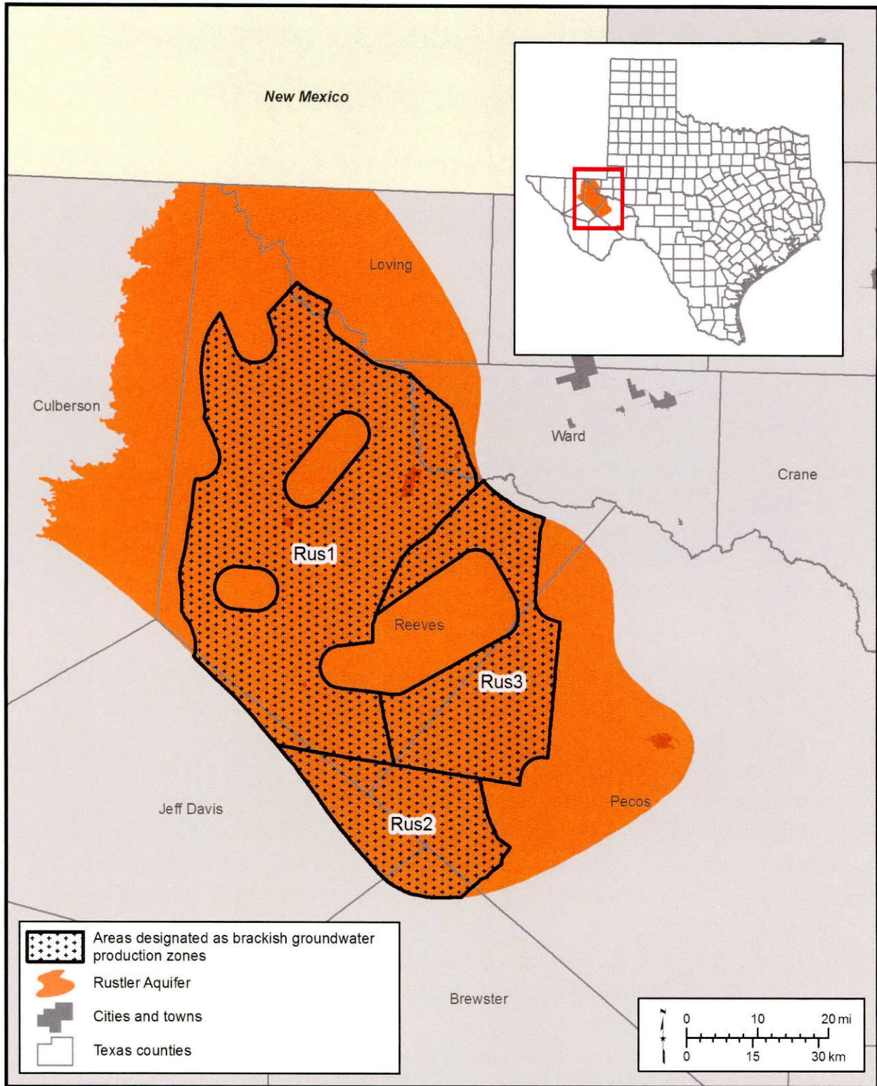
Figure 15. Rustler Aquifer showing three brackish groundwater production zones.
