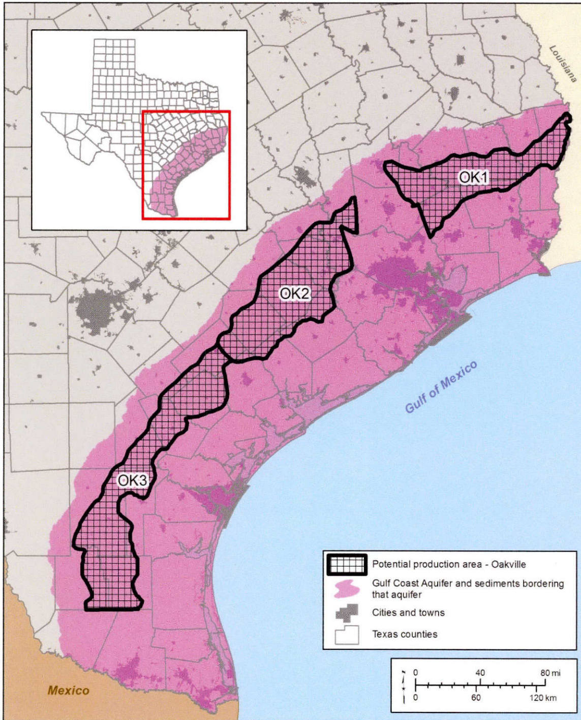
Figure B-11. Potential production areas in the Oakville Formation in the Gulf Coast Aquifer System.
