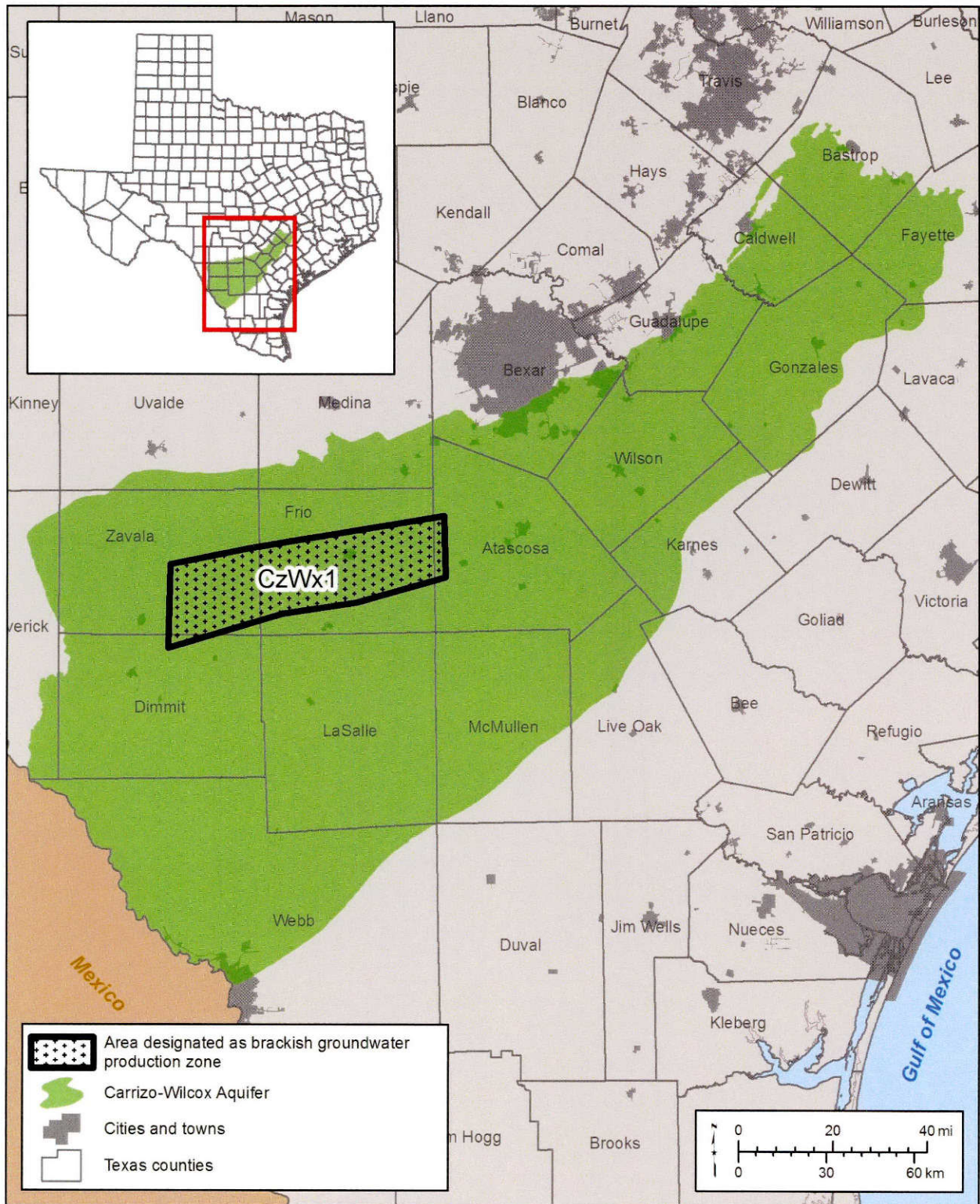
Figure 9. Carrizo-Wilcox Aquifer located between the Colorado River and the Rio Grande showing one brackish groundwater production zone within the lower Wilcox Formation.
