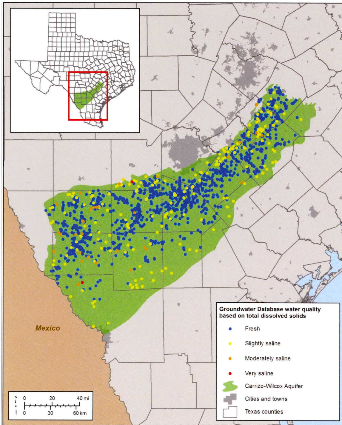
Figure A-7. Carrizo-Wilcox Aquifer total dissolved solids concentration based on the most recent samples in the TWDB Groundwater Database. Salinity classes are defined as fresh (0 to 999 milligrams per liter total dissolved solids), slightly saline (1,000 to 2,999 milligrams per liter total dissolved solids), moderately saline (3,000 to 9,999 milligrams per liter total dissolved solids), and very saline (10,000 to 35,000 milligrams per liter total dissolved solids).
