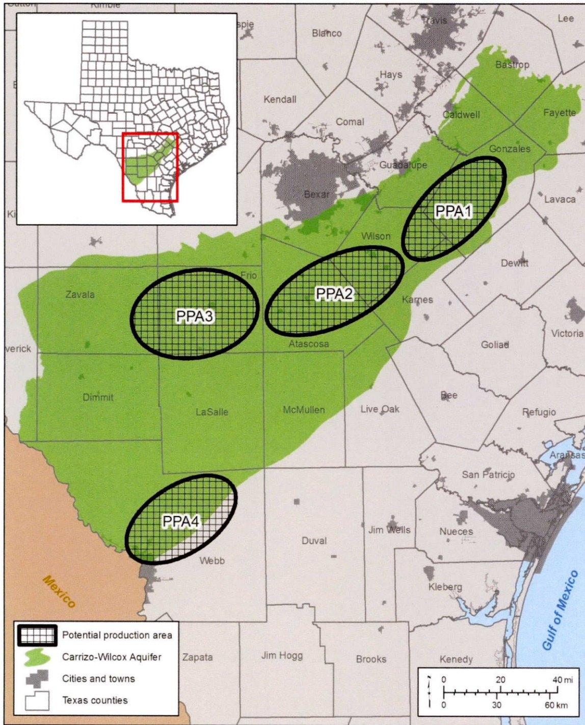
Figure A-5. Potential production areas in the Carrizo-Wilcox Aquifer project area.
