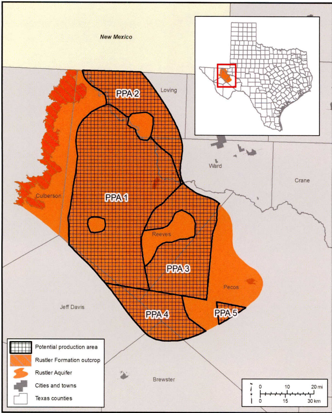
Figure D-5. Rustler Aquifer potential production areas modeled by the contractor (Lupton and others, 2016).
