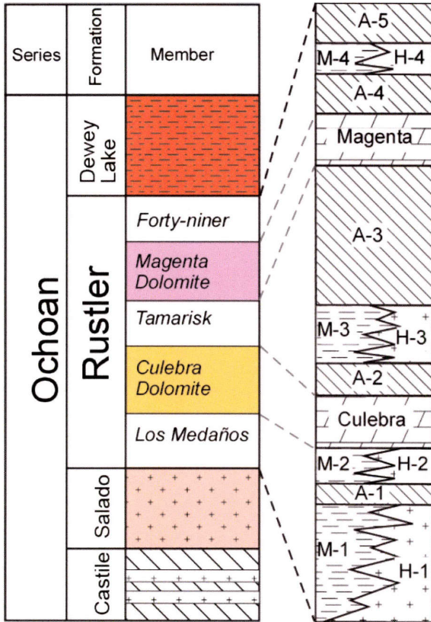
Figure D-2. Stratigraphy of the Rustler Aquifer (Lupton and others, 2016). The Rustler Aquifer occurs in the Rustler Formation, which forms part of the Upper Permian Ochoan series in the Delaware Basin of West Texas and New Mexico. The Rustler Formation is subdivided into its members and informal submembers. For the informal submembers, "A" = anhydrite, "M" = mud, and "H" = halite. The Delaware Mountain Group occurs below the Castile Formation in the majority of the project area. Lateral equivalent units, mainly the Capitan/Goat Seep Reefs and members of the Artesia Group, occur beneath the Castile Formation in the southeastern portions of the project area.
