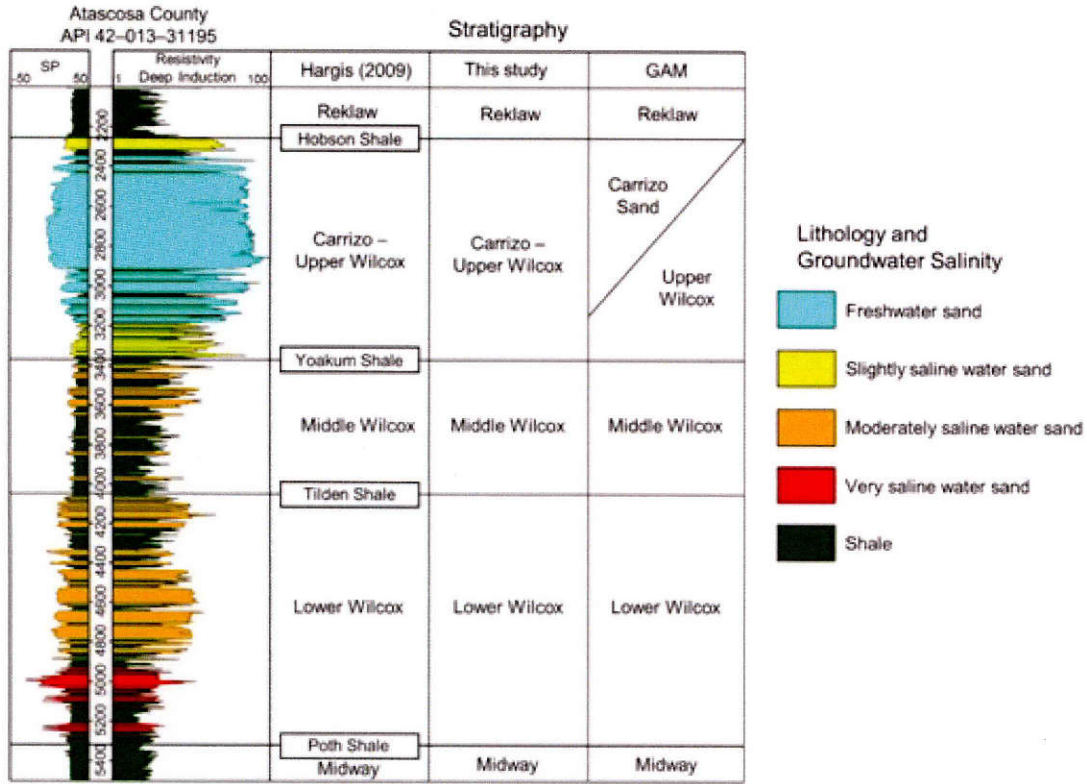
Figure A-6. Stratigraphic subdivision of the Carrizo-Wilcox Aquifer in the project area. The aquifer includes the Carrizo-upper Wilcox, middle Wilcox, and lower Wilcox geological formations. The resistivity and spontaneous potential tools on the geophysical well log have been divided into sand and shale layers. The sand layers were interpreted and are colored based on salinity (total dissolved solids) using the U.S. Geological Survey salinity classification (Winslow and Kister, 1956). Figure from Hamlin and others (2016, Figure 4-2).
