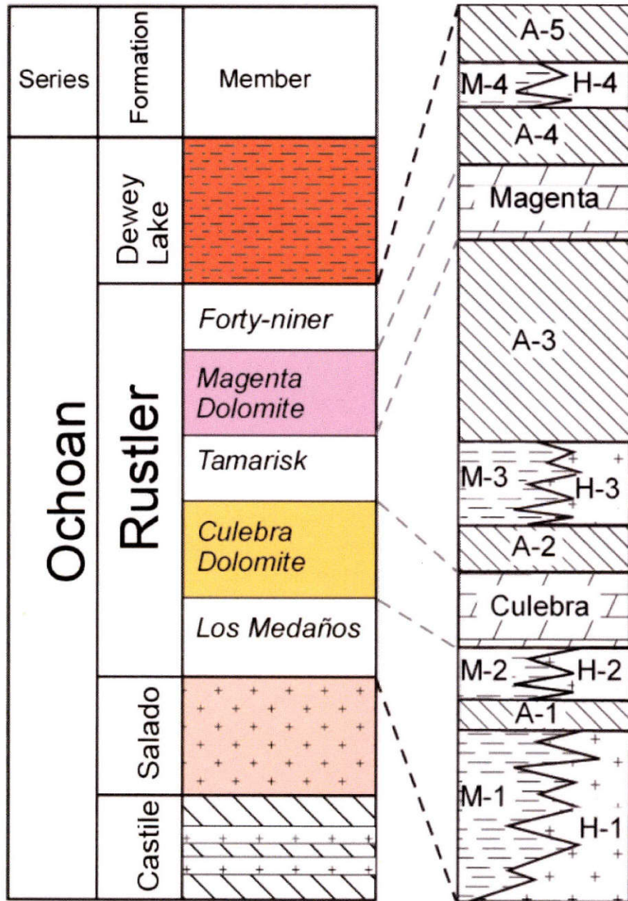
Figure 14. Stratigraphy of the Rustler Aquifer (Lupton and others, 2016). For the informal submembers, "A"= anhydrite, "M"= mud and "H"= halite.
