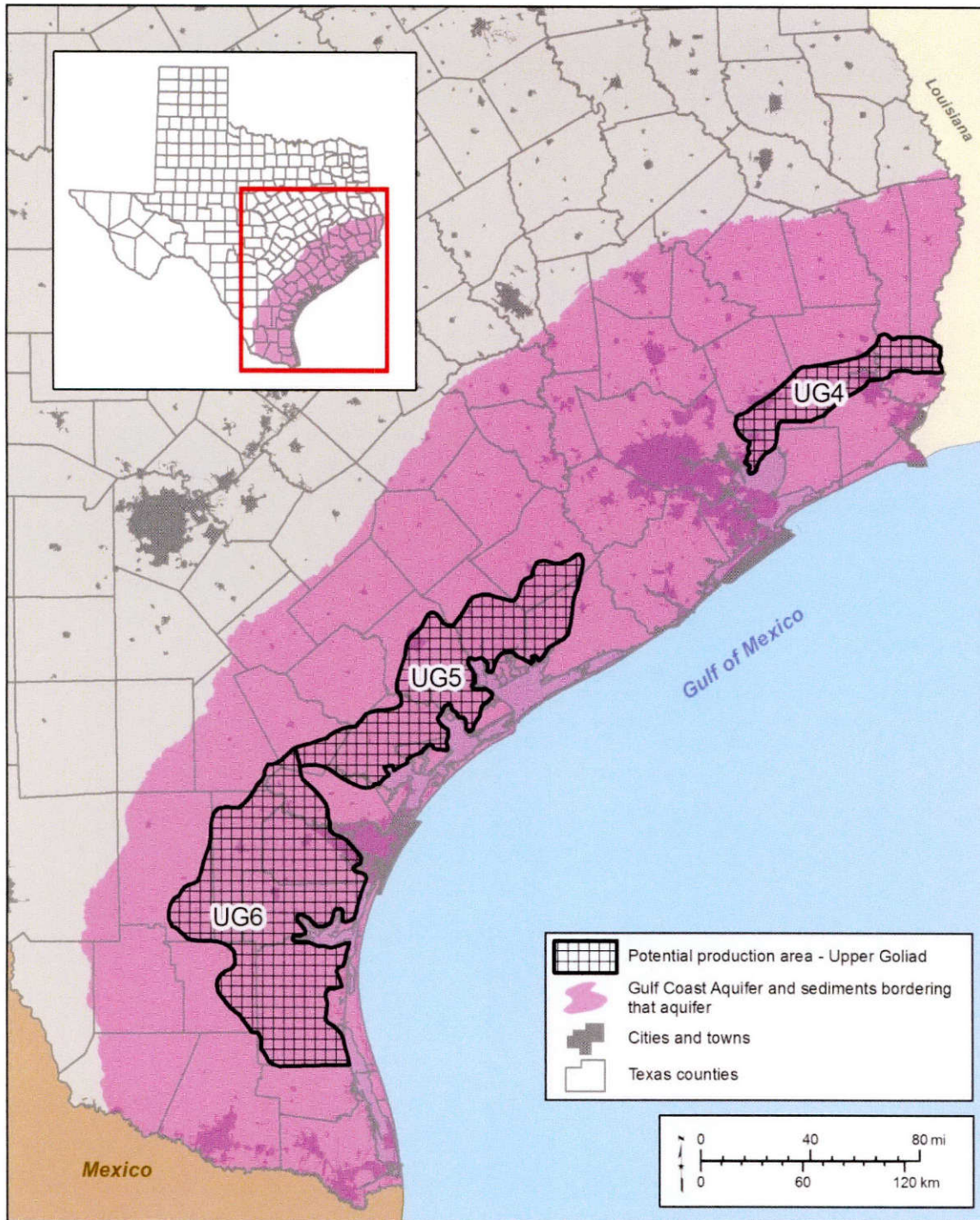
Figure B-6. Potential production areas in the Upper Goliad Formation in the Gulf Coast Aquifer System.
