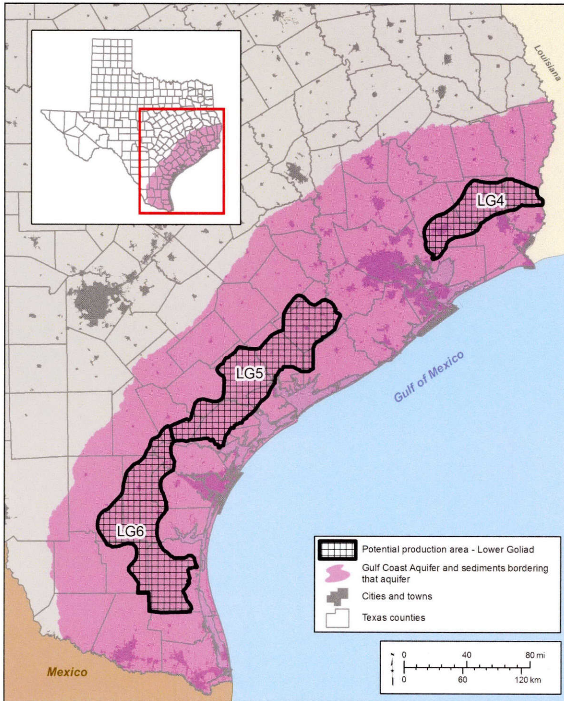
Figure B-7. Potential production areas in the Lower Goliad Formation in the Gulf Coast Aquifer System.
