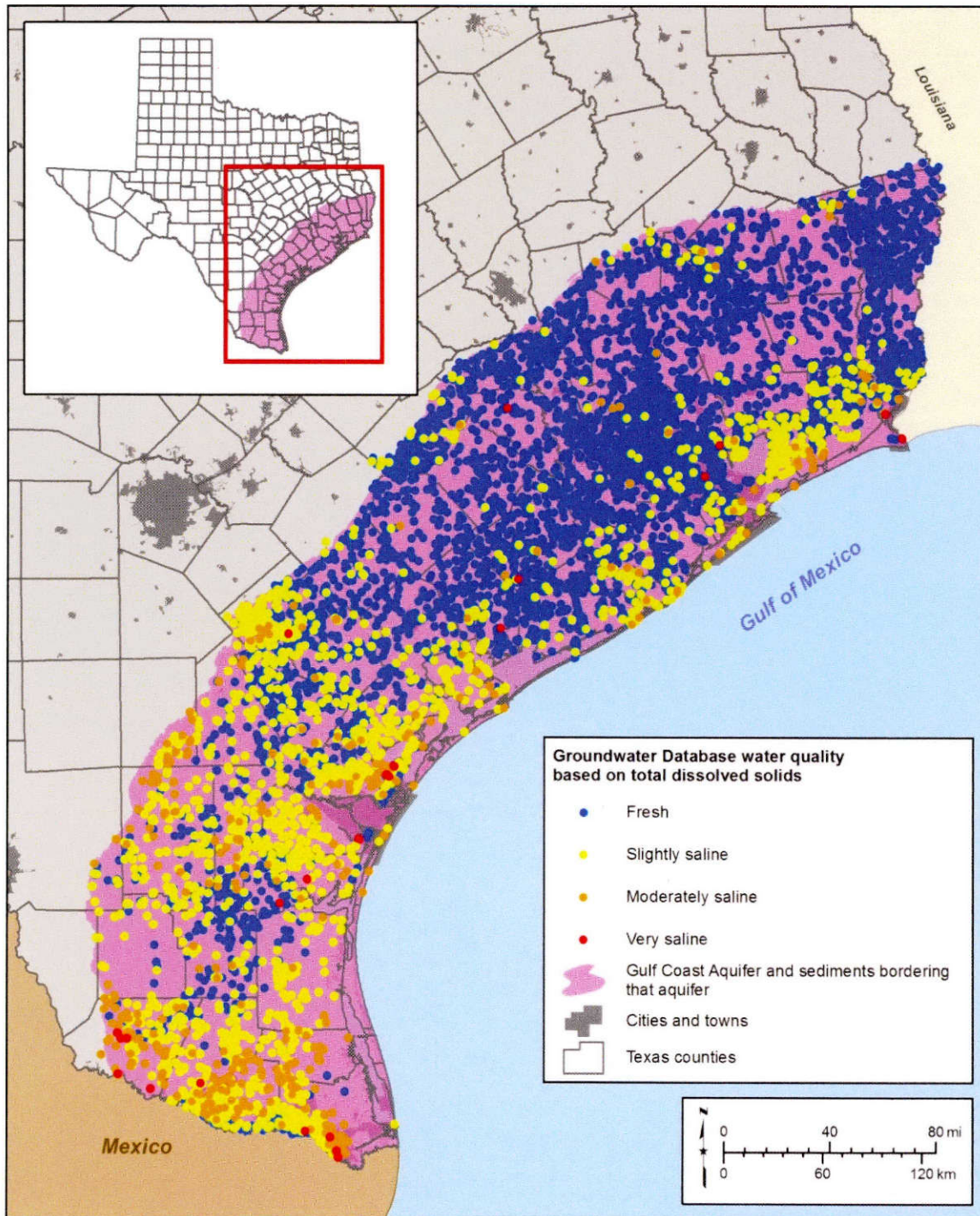
Figure B-13. Groundwater quality in the Gulf Coast Aquifer System showing total dissolved solids concentration based on the most recent samples in the TWDB Groundwater Database. Salinity classes are defined as: fresh (0 to 999 milligrams per liter total dissolved solids), slightly saline (1,000 to 2,999 milligrams per liter total dissolved solids), moderately saline (3,000 to 9,999 milligrams per liter total dissolved solids), and very saline (10,000 to 35,000 milligrams per liter total dissolved solids).
