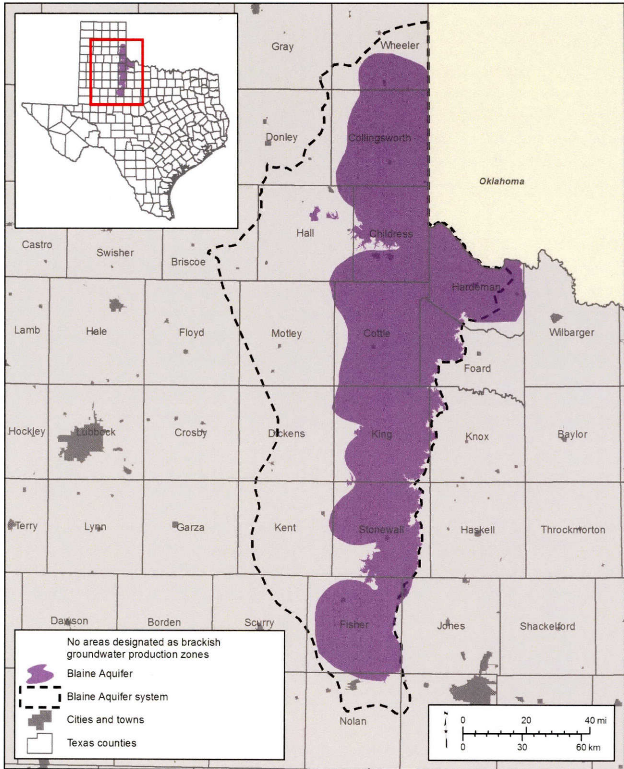
Figure 13. Blaine Aquifer showing no areas designated as brackish groundwater production zones.
