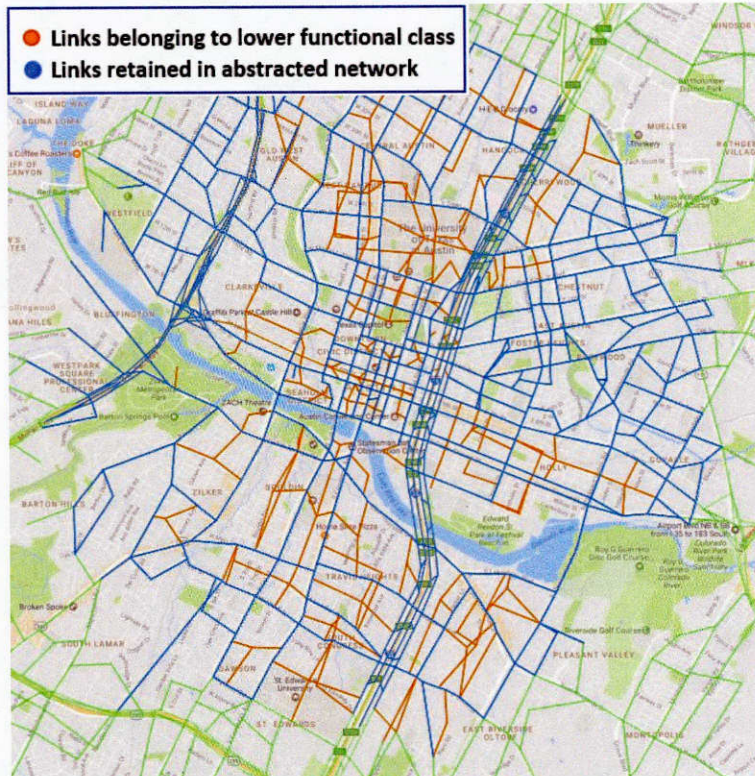
Figure 29 Link extraction for a section of the Austin network
