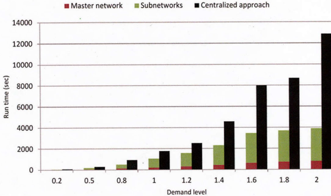
Figure 39 Computational time of the master (red) and subnetworks (green) in DSTAP compared to centralized run time (black) for different demand levels
