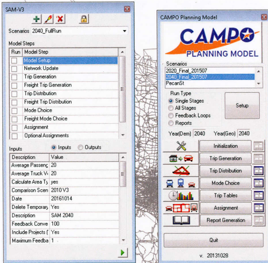
Figure 23 Comparison of SAM (left) and CAMPO (right) model interfaces
