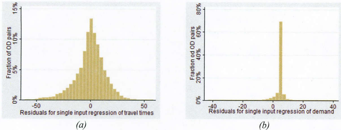
Figure 20 Single-input regression model: histogram counts of residual errors on validation data for (a) travel time and (b) demand
