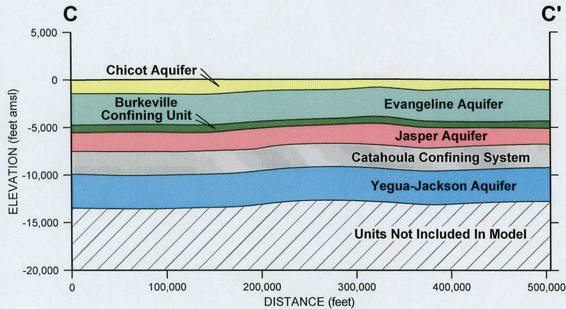
FIGURE 4.1.4. HYDROGEOLOGIC SECTIONS A, B, AND C
