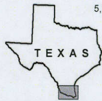
FIGURE 4.2.8. LOCATIONS OF SELECTED GROUNDWATER LEVEL HYDROGRAPHS
