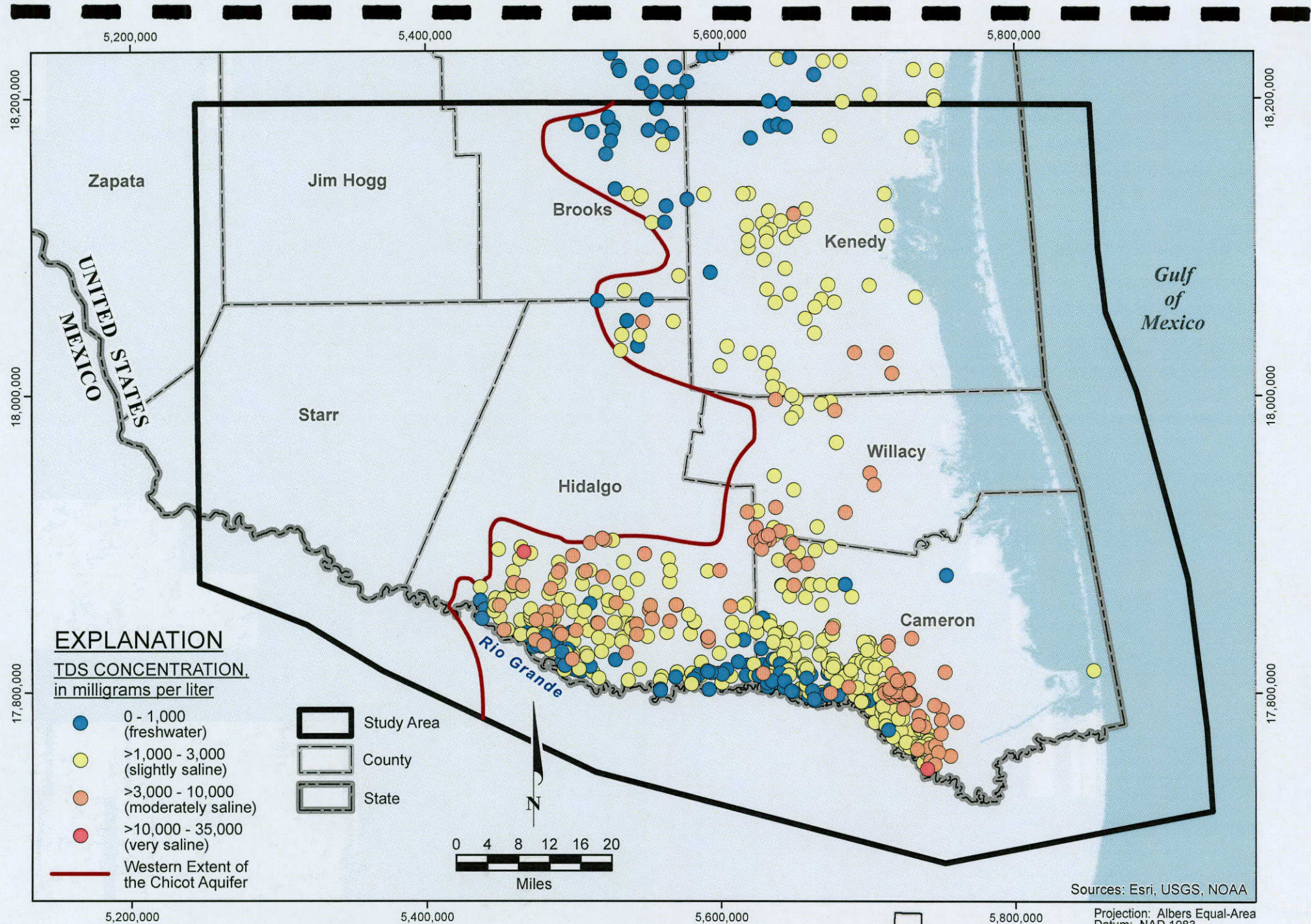
FIGURE 4.8.7. MEASURED TOTAL DISSOLVED SOLIDS CONCENTRATIONS CHICOT AQUIFER, 1940 THROUGH 2014
