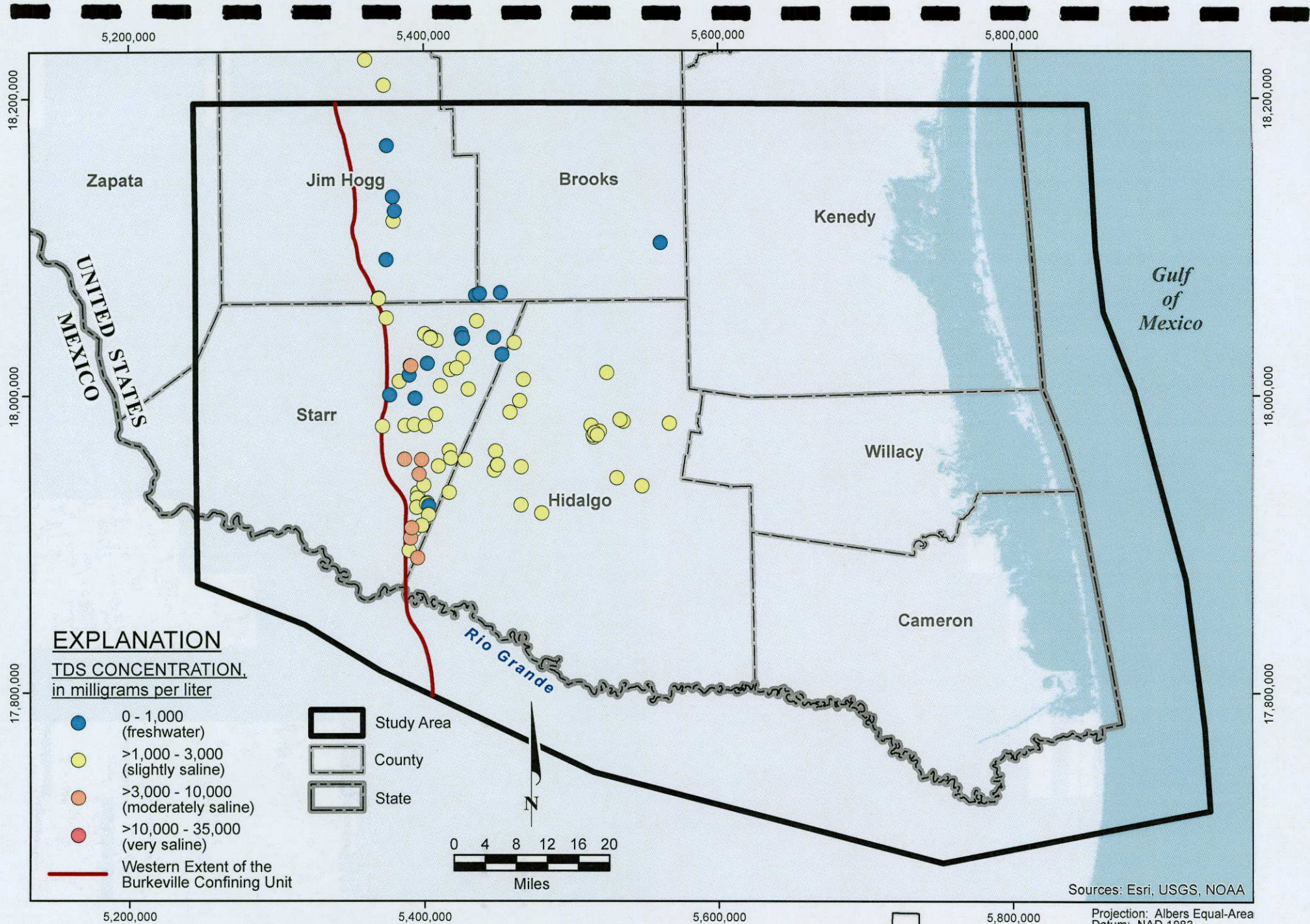
FIGURE 4.8.9. MEASURED TOTAL DISSOLVED SOLIDS CONCENTRATIONS BURKEVILLE CONFINING UNIT, 1940 THROUGH 2014
