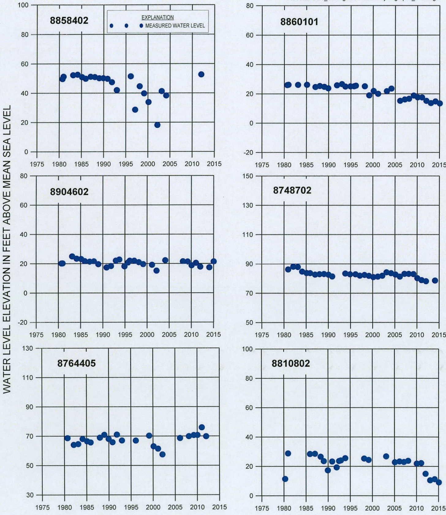
FIGURE 4.2.9. WATER LEVEL HYDROGRAPHS FOR SELECTED WELLS IN THE CHICOT AQUIFER, LOWER RIO GRANDE VALLEY, TEXAS
