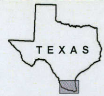
FIGURE 2.3.2a. SURFICIAL GEOLOGY IN LOWER RIO GRANDE VALLEY
