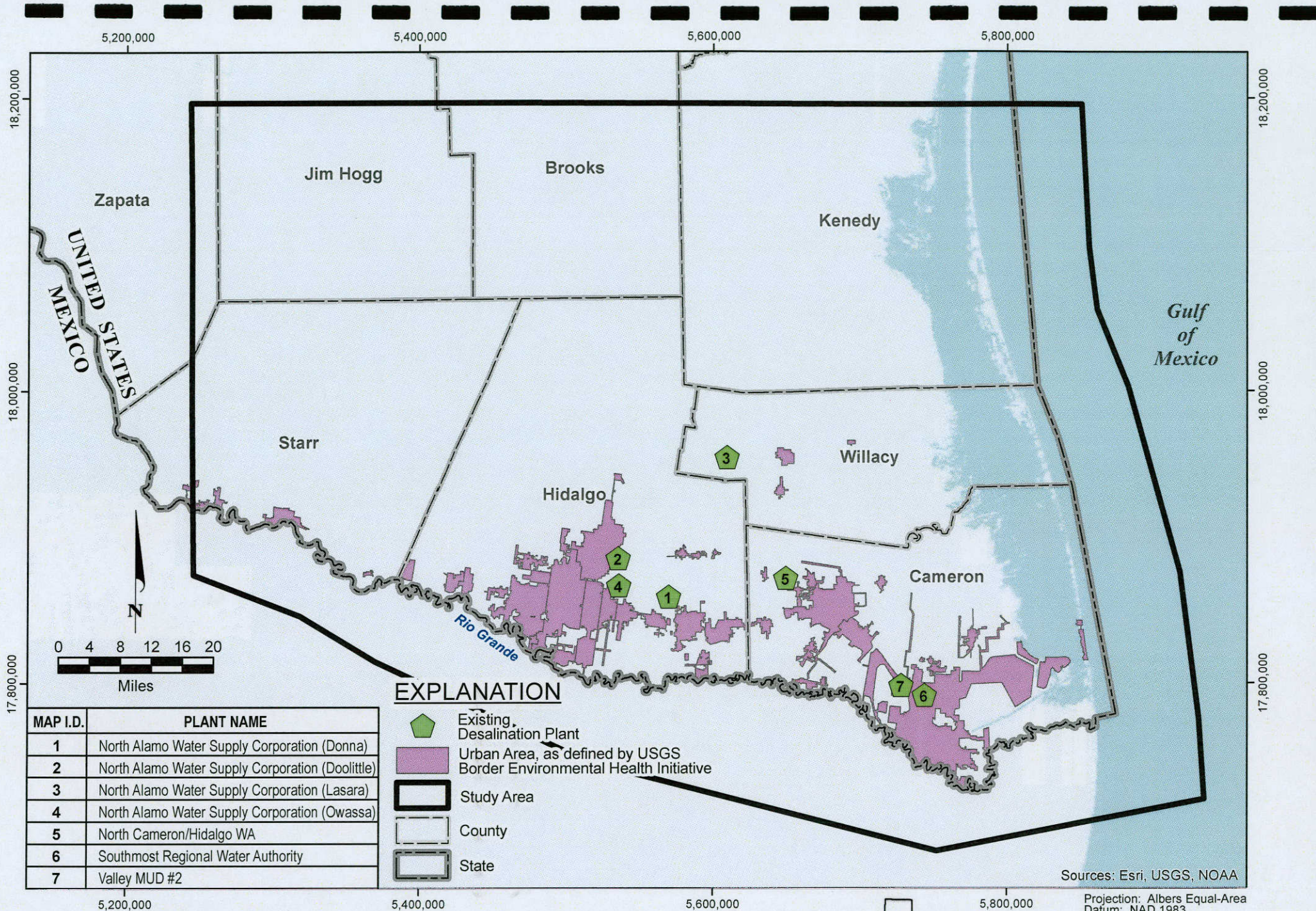
FIGURE 1.0.4. EXISTING BRACKISH GROUNDWATER DESALINATION PLANTS IN LOWER RIO GRANDE VALLEY
