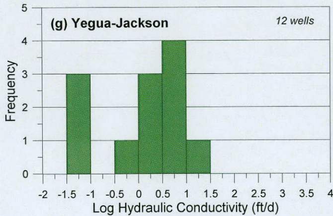
FIGURE 4.5.3. HISTOGRAMS OF ESTIMATED HYDRAULIC CONDUCTIVITY FOR THE LOWER RIO GRANDE VALLEY HYDROSTRATIGRAPHIC UNITS
