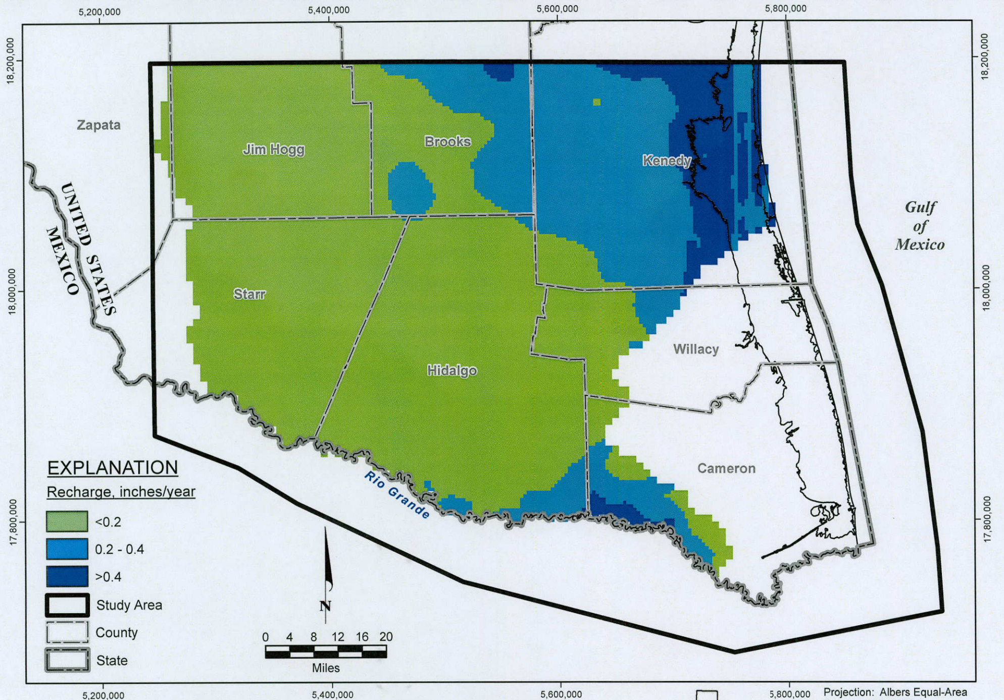
FIGURE 4.3.1. DISTRIBUTION OF AVERAGE ESTIMATED ANNUAL RECHARGE RATES IN LOWER RIO GRANDE VALLEY
