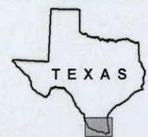
FIGURE 4.1.23. THICKNESS CONTOURS FOR THE YEGUA-JACKSON AQUIFER LOWER RIO GRANDE VALLEY STUDY AREA
