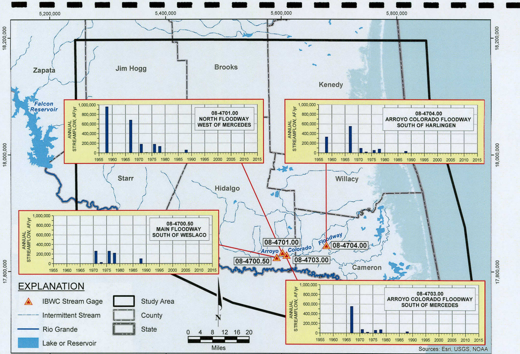
FIGURE 4.4.3. ANNUAL STREAMFLOWS ALONG ARROYO COLORADO FLOODWAY IN LOWER RIO GRANDE VALLEY
