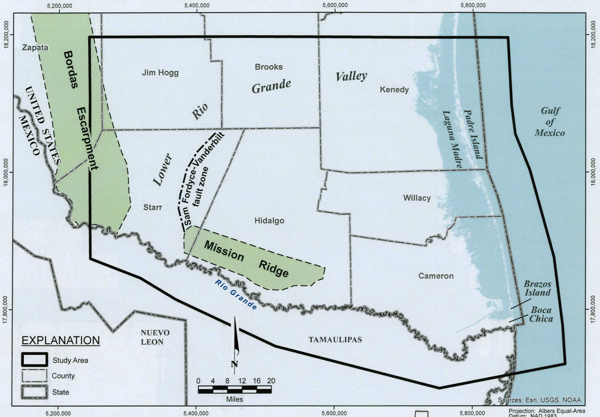
FIGURE 2.1.1. MAJOR PHYSIOGRAPHIC FEATURES IN THE STUDY AREA
