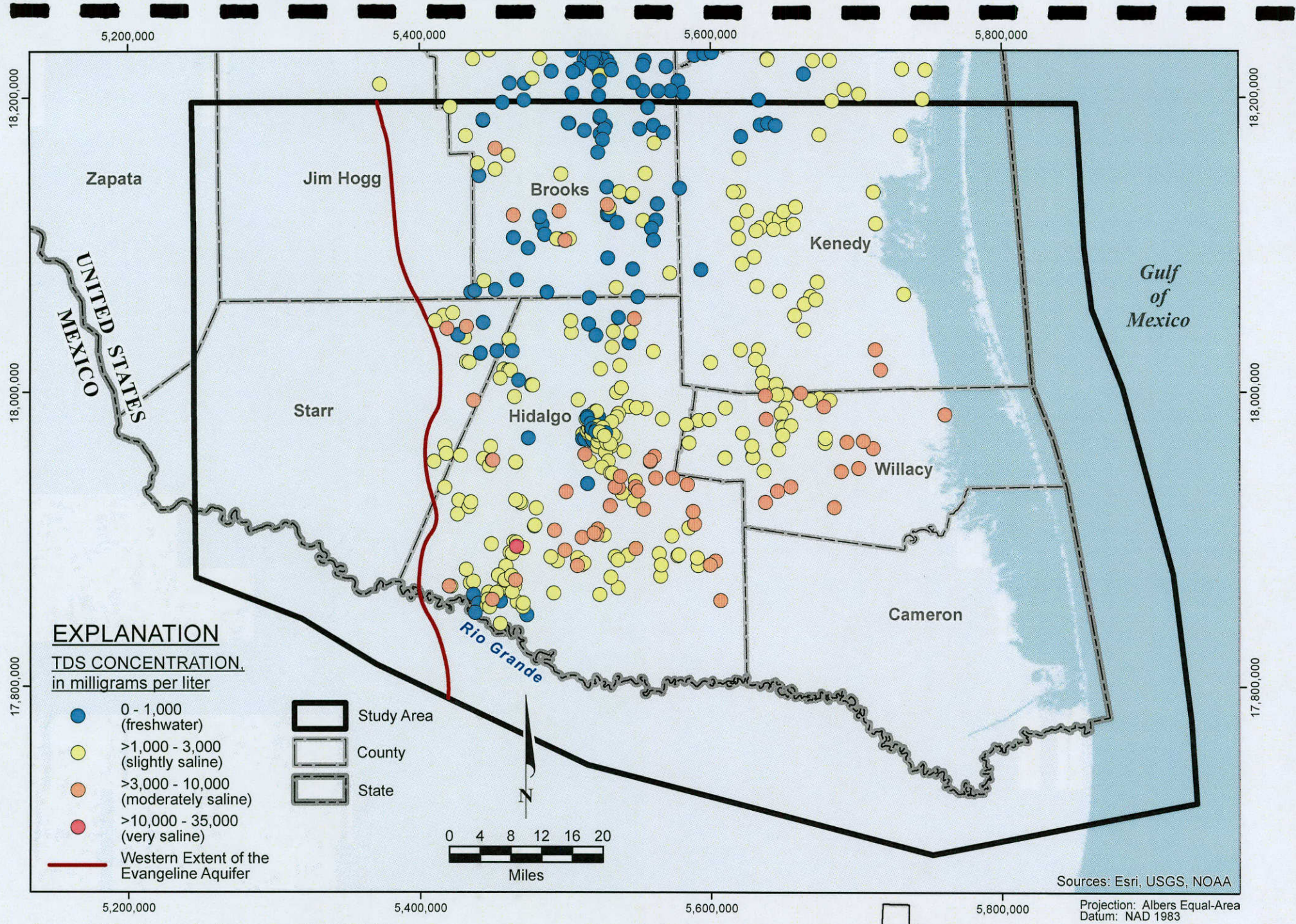
FIGURE 4.8.8. MEASURED TOTAL DISSOLVED SOLIDS CONCENTRATIONS EVANGELINE AQUIFER, 1940 THROUGH 2014
