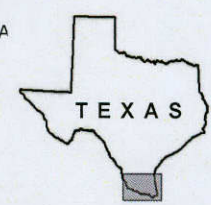
FIGURE 4.8.11. SELECTED TOTAL DISSOLVED SOLIDS HYDROGRAPHS FOR GULF COAST AQUIFER IN LOWER RIO GRANDE VALLEY
