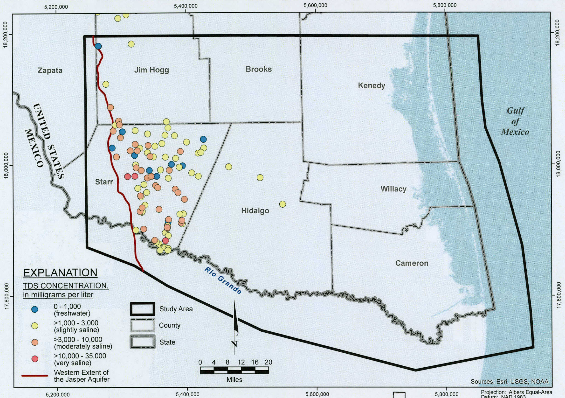
FIGURE 4.8.10. MEASURED TOTAL DISSOLVED SOLIDS CONCENTRATIONS JASPER AQUIFER, 1940 THROUGH 2014
