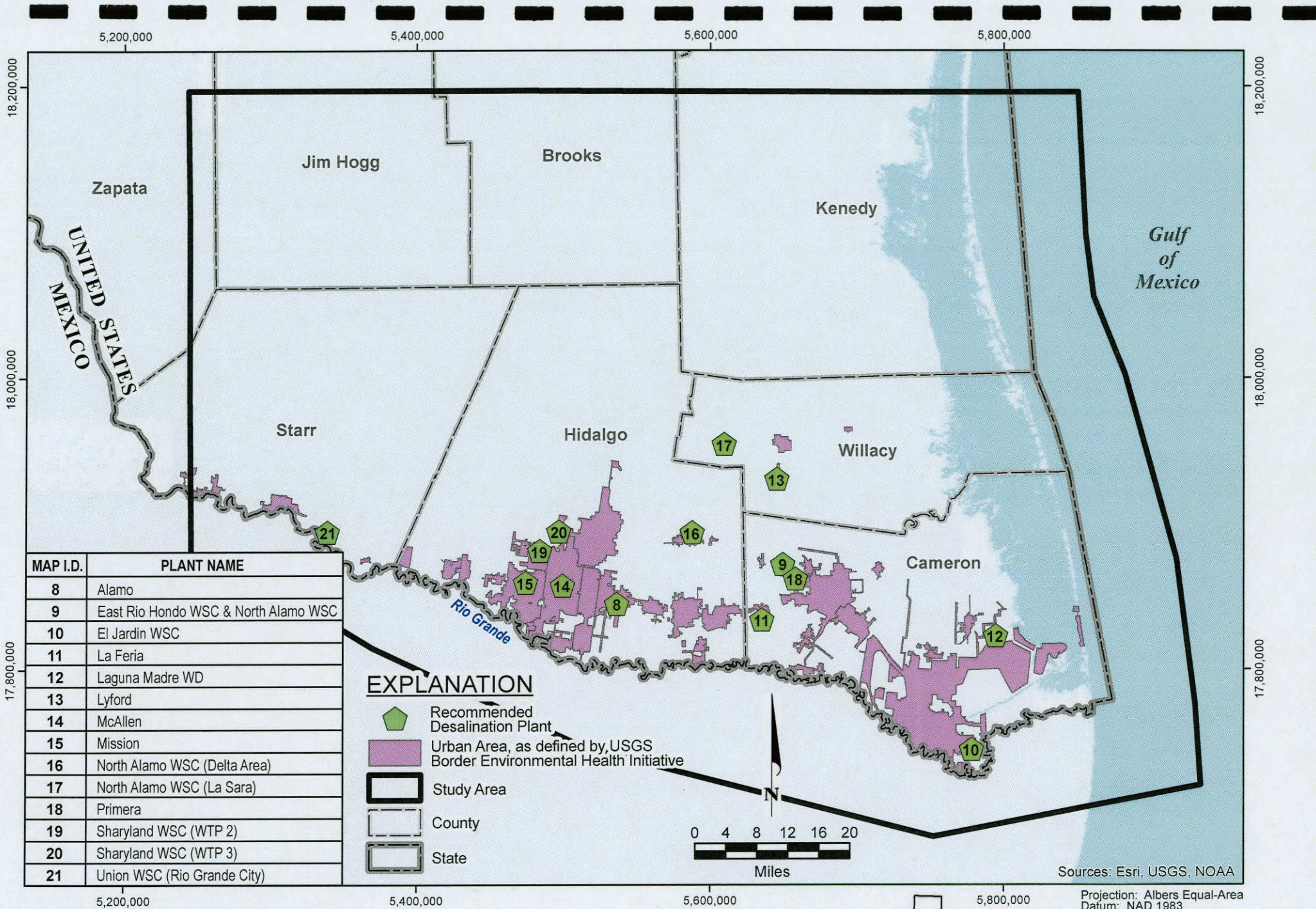
FIGURE 1.0.5. RECOMMENDED BRACKISH GROUNDWATER DESALINATION PLANTS IN LOWER RIO GRANDE VALLEY
