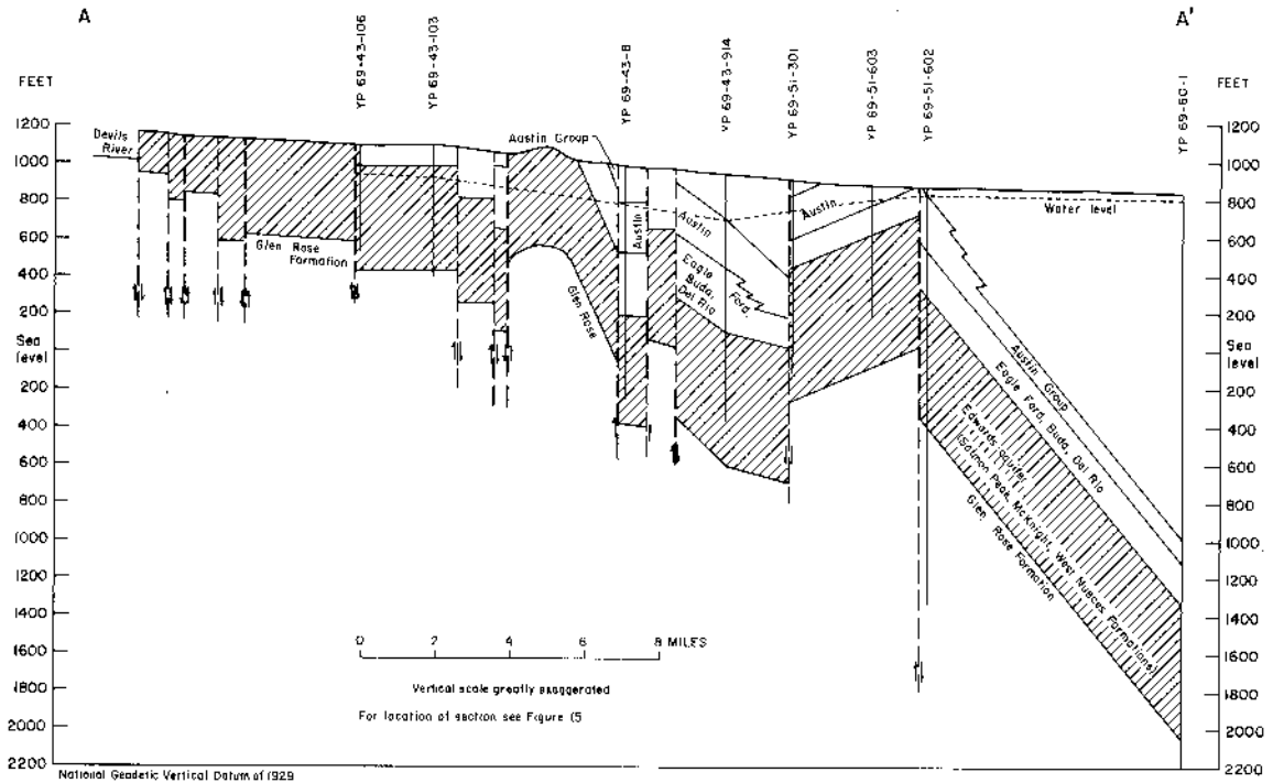
Figure 16a.—Hydrogeologic Section A-A' Through the Edwards Aquifer
