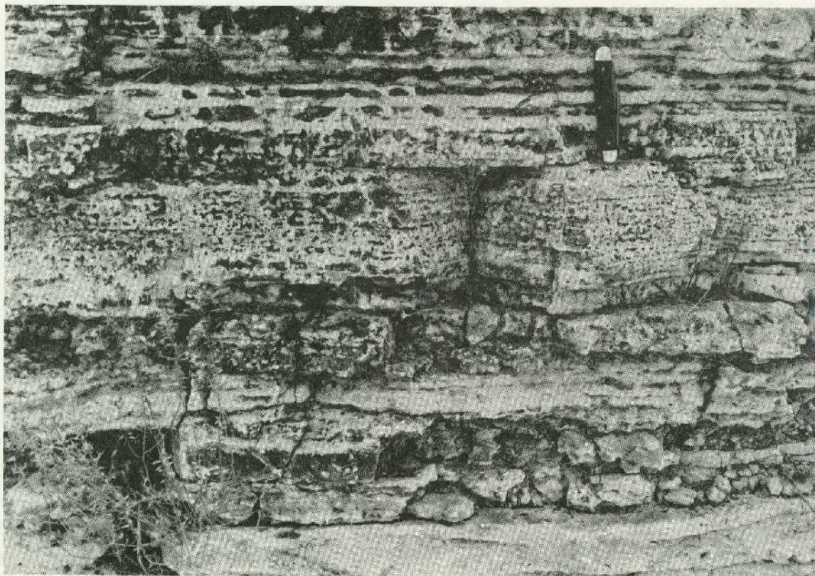
Figure 10.—Diagenetic Features of Representative Rocks From the Edwards Aquifer
