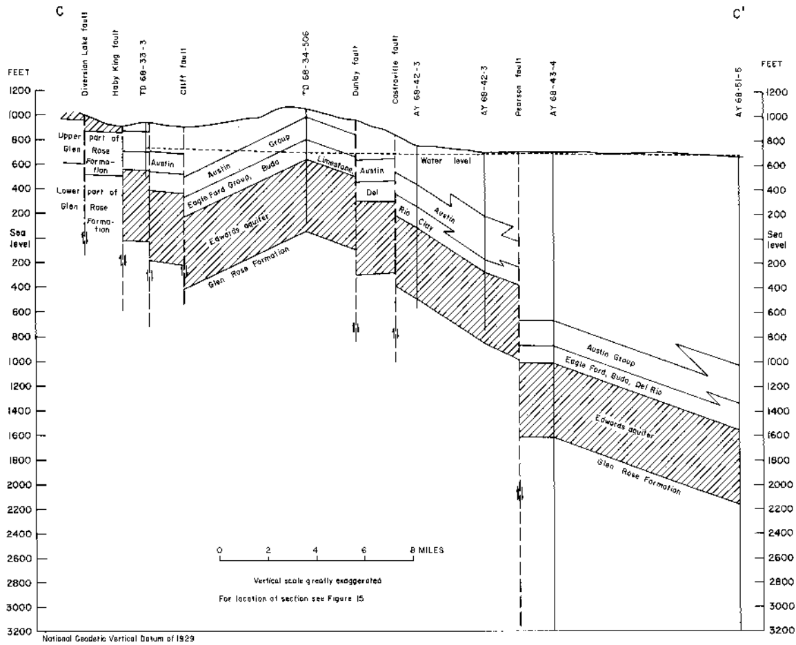
Figure 16c.—Hydrogeologic Section C-C' Through the Edwards Aquifer
