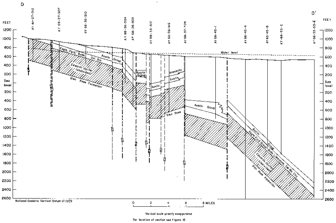
Figure 16d.—Hydrogeologic Section D-D' Through the Edwards Aquifer
