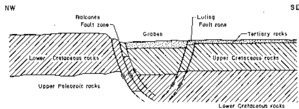
Figure 4.—Conceptual Section Showing the Regional Graben Formed by the Balcones and Luling Fault Zones in Bexar County
