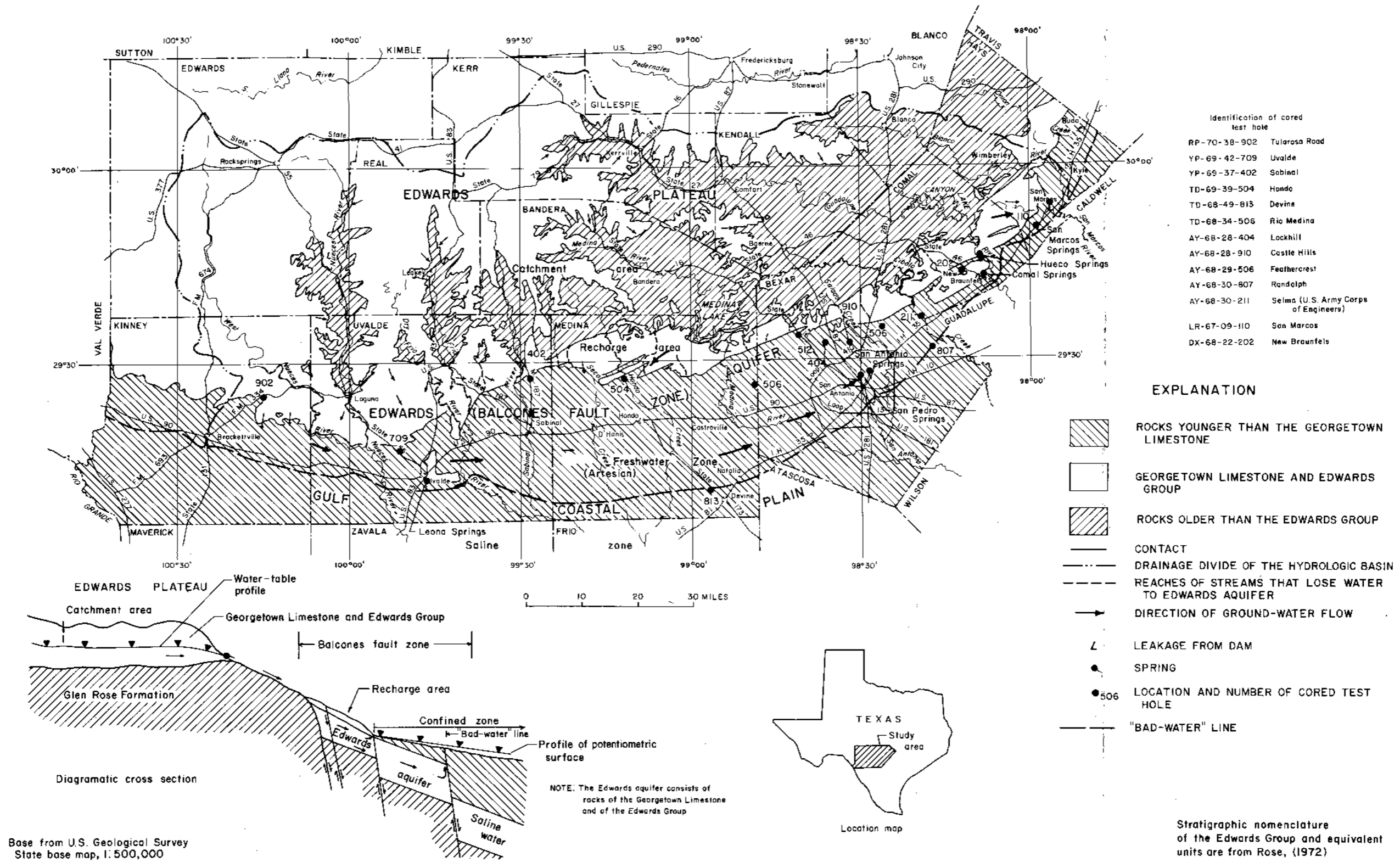
Figure 1 Location and Extent of the Edwards Aquifer, Recharge Basins, and Data-Collection Sites
