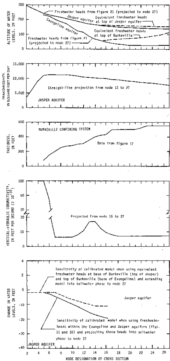
Figure 25.—Hydrologic Parameters for the Cross Section of the Model Extended Into the Part of the Aquifer Containing Saltwater and Sensitivity of the Calibrated Model to the Downdip Extension
