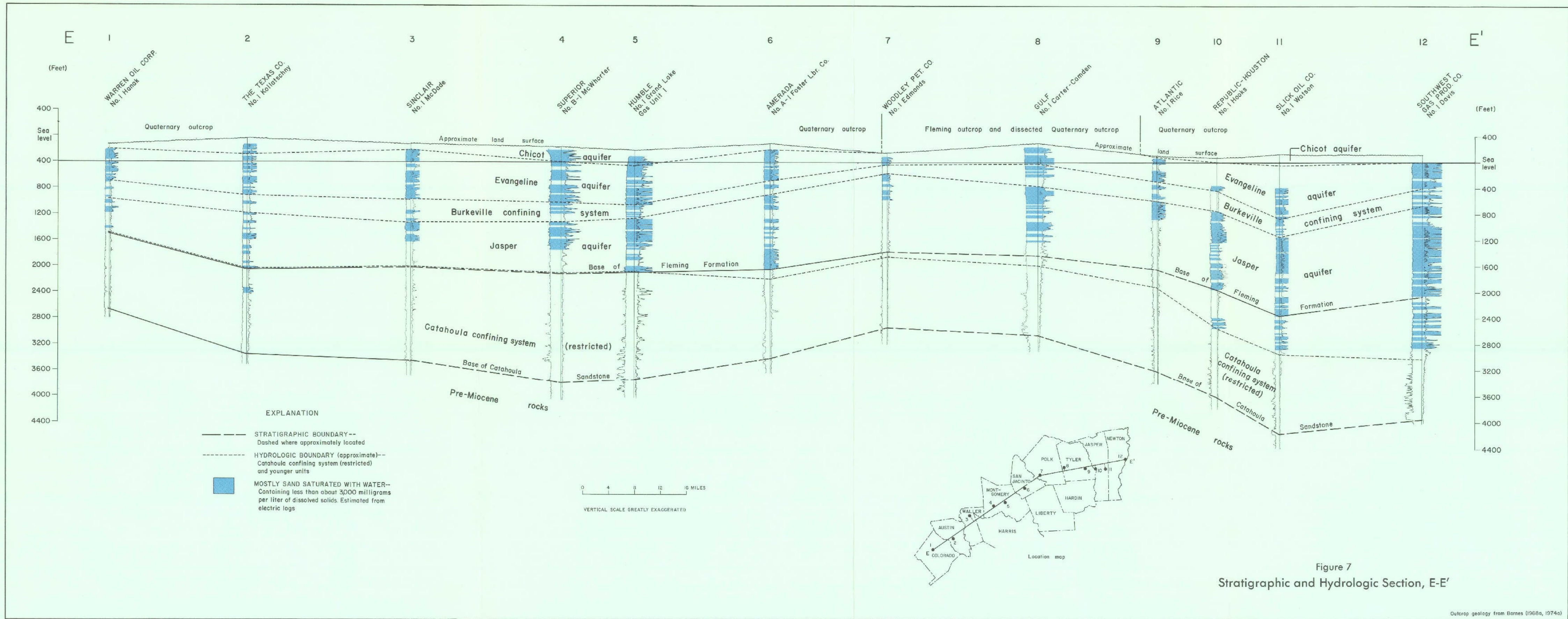
Figure 7.—Stratigraphic and hydrologic section, E-E'.
