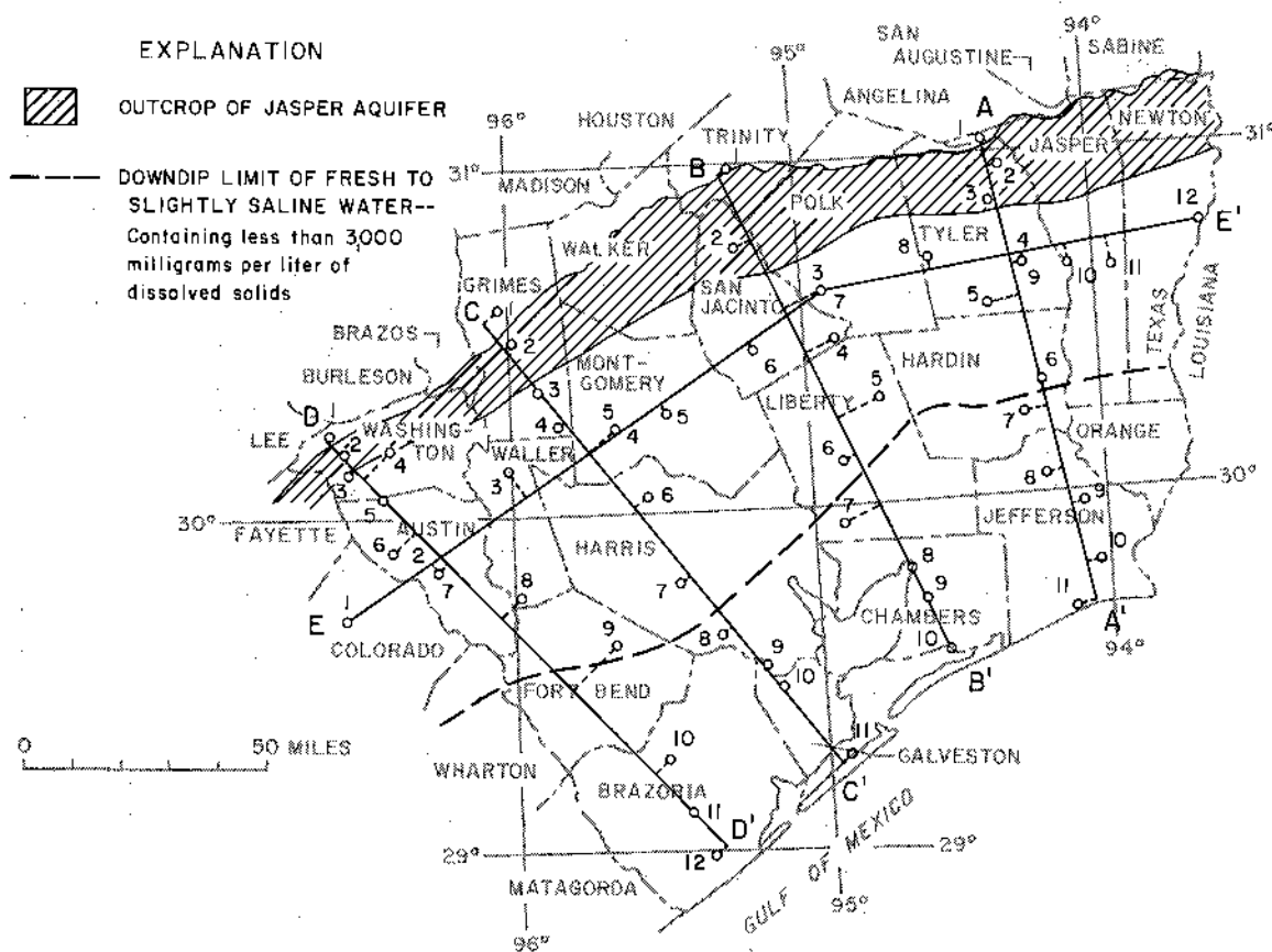
Figure 2.—Location of Stratigraphic and Hydrologic Sections
