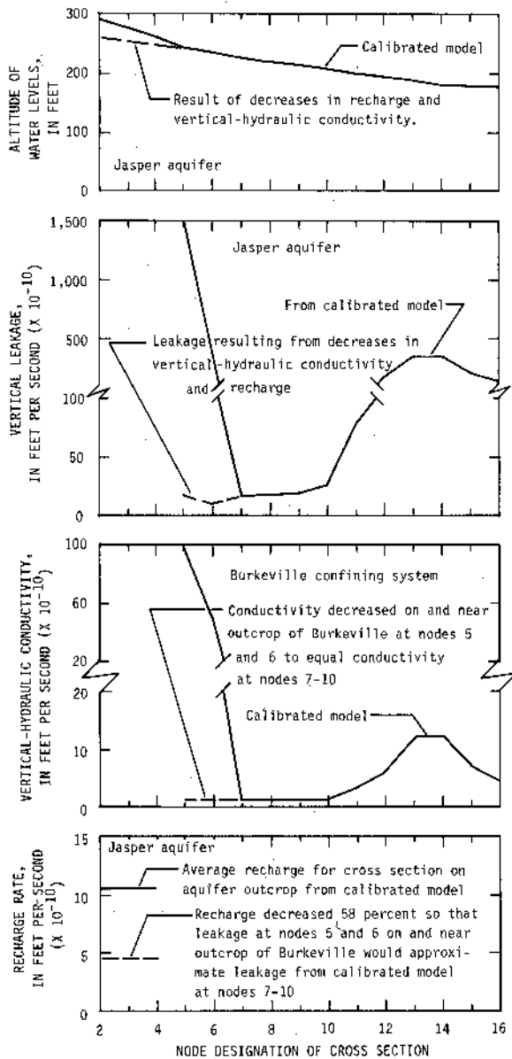
Figure 24.—Distribution of Leakage and Sensitivity of Water Levels to Reductions in Recharge and Vertical-Hydraulic Conductivity on and Near the Outcrop of the Jasper Aquifer and Burkeville Confining System
