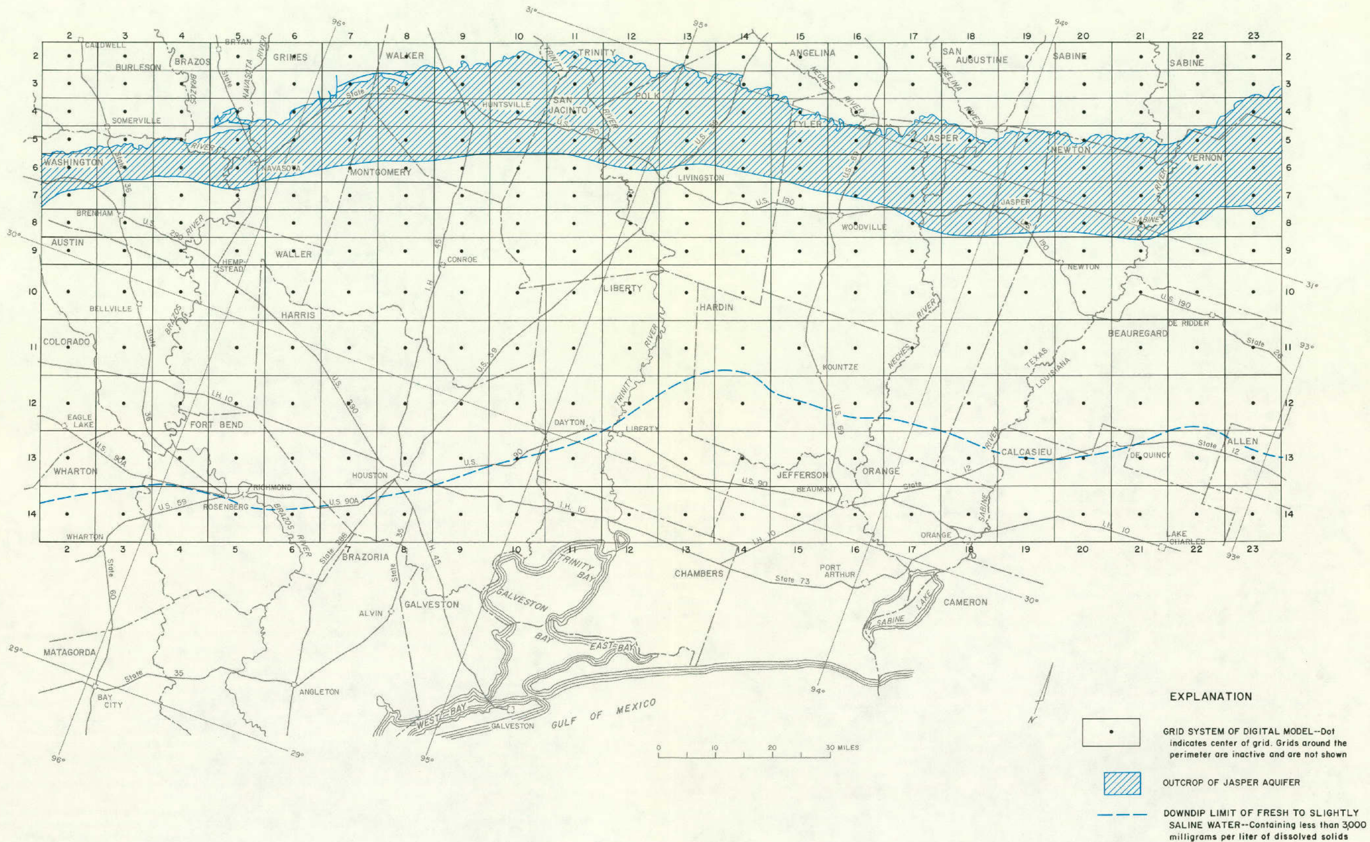
Figure 13 Boundaries and Grid Patterns of the Model
