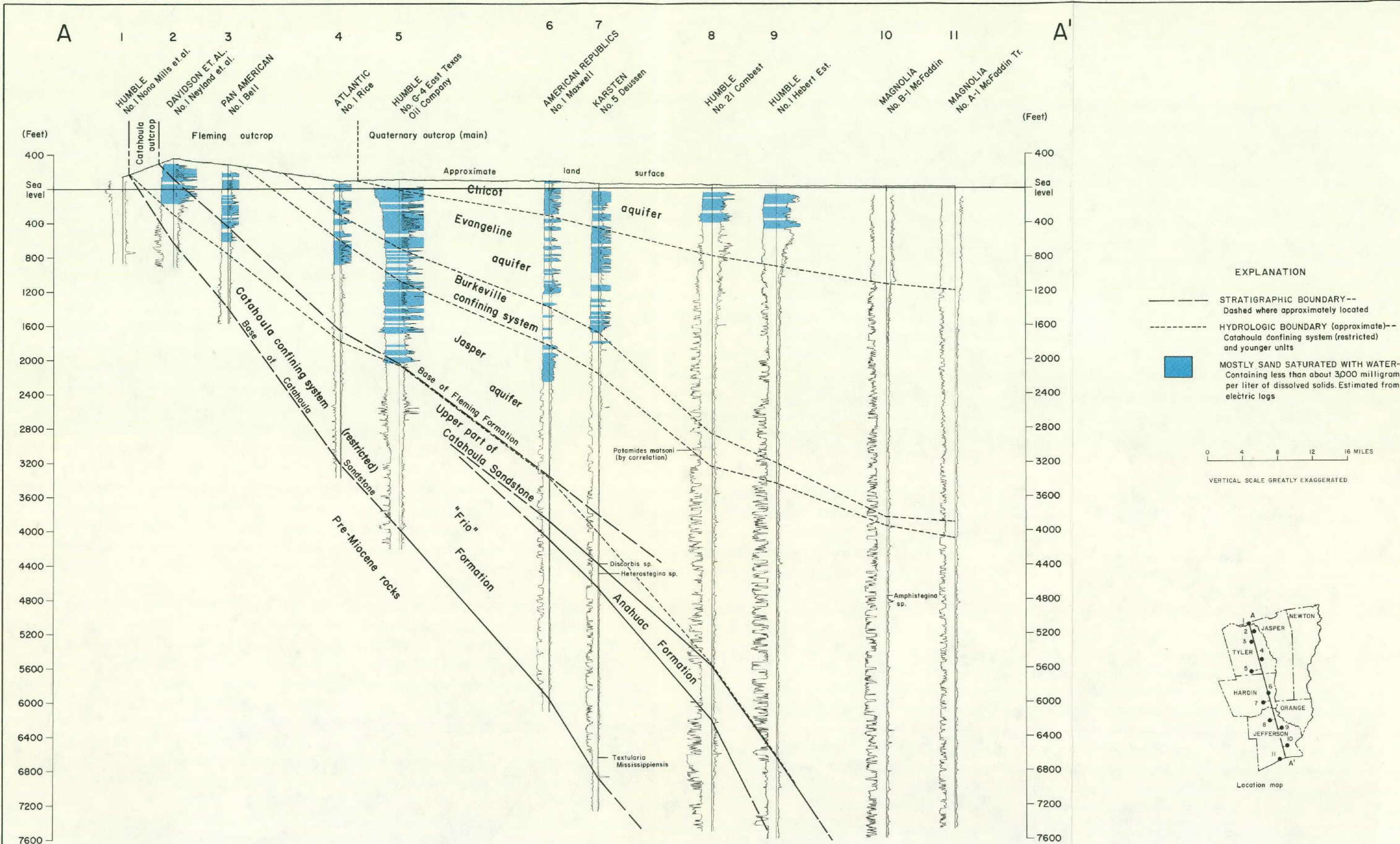
Figure 3 Stratigraphic and Hydrologic Section, A-A'
