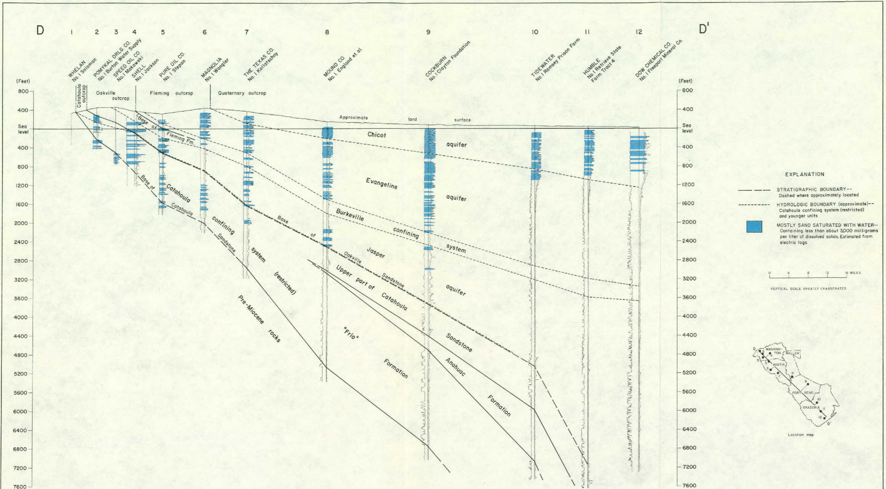
Figure 6 Stratigraphic and Hydrologic Section, D-D'
