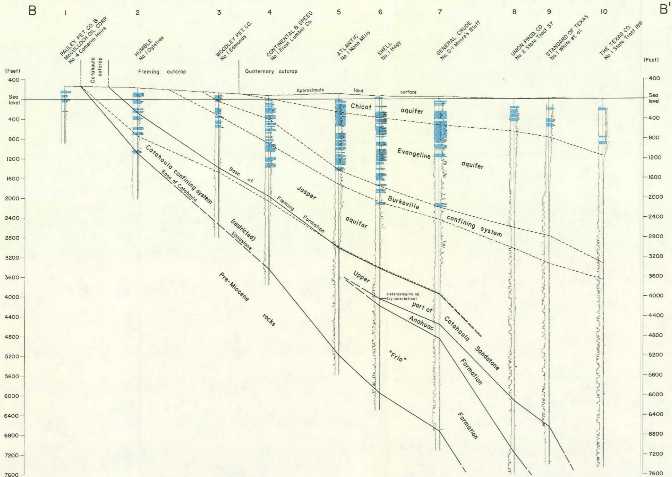
Figure 4 Stratigraphic and Hydrologic Section, B-B'
