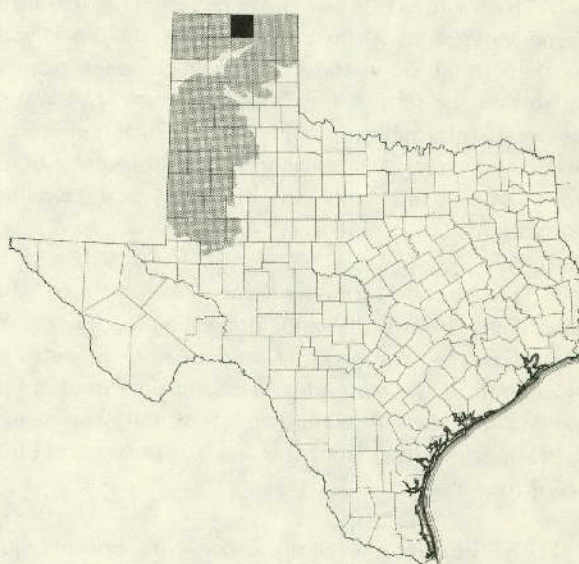
Location of Hansford County, and Extent of the Ogallala Aquifer in Texas
