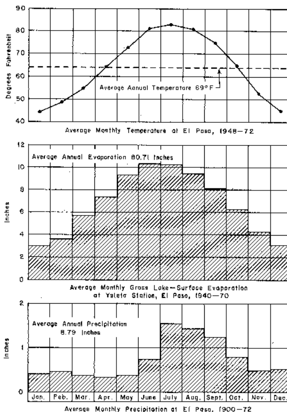
Figure 2.—Average Monthly Temperature, Evaporation, and Precipitation at El Paso (Temperature and precipitation data from National Weather Service; lake-surface evaporation obtained as described in Kane, 1967)
