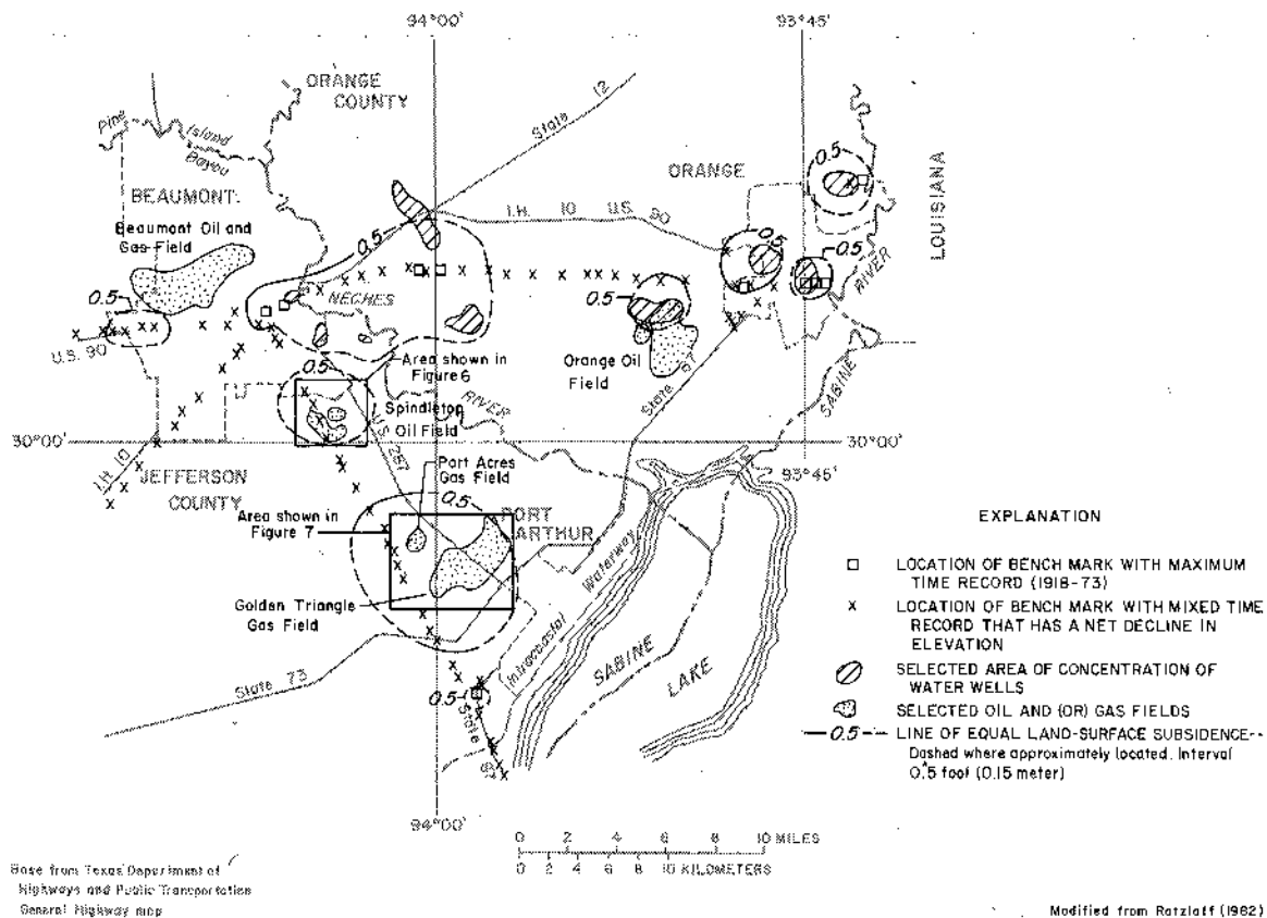
Figure 5.—Locations of Bench Mark and Land-Surface Subsidence in the Beaumont, Orange, Port Arthur, Texas, Area, 1953-55 to 1973
