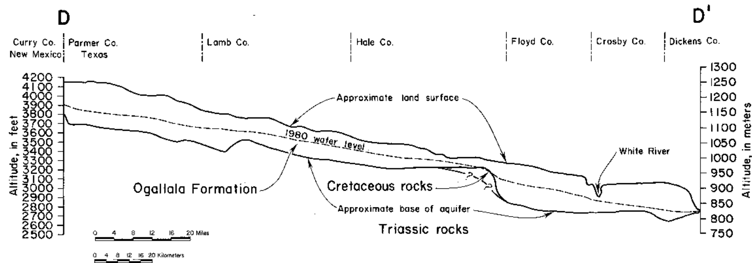
Figure 25 Generalized Geologic Section D-D'
