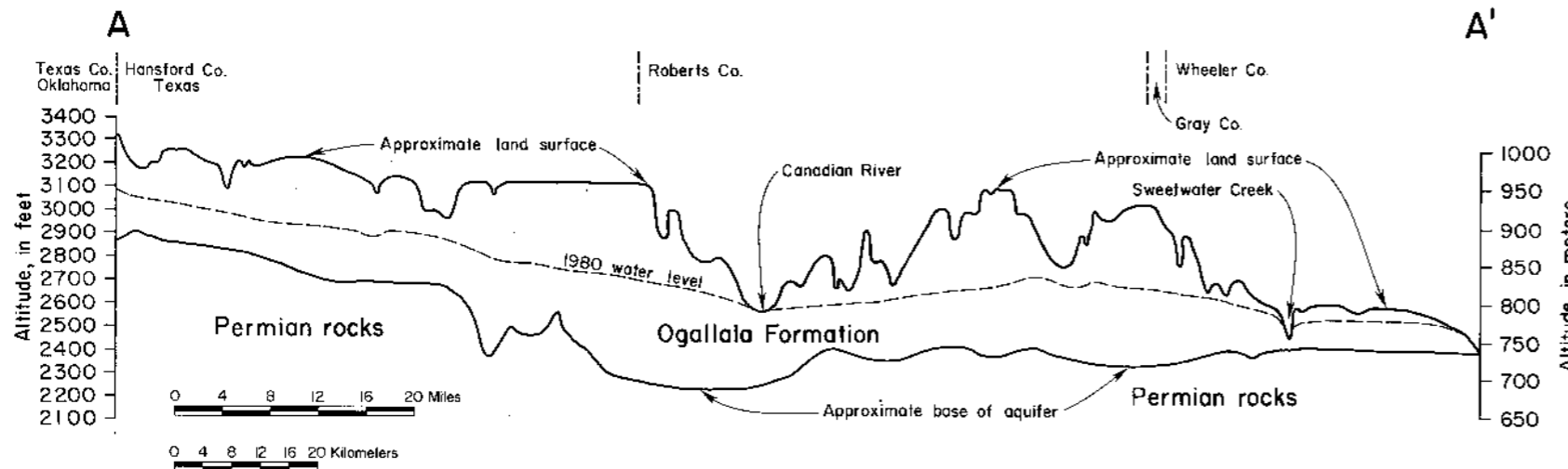
Figure 22 Generalized Geologic Section A-A'
