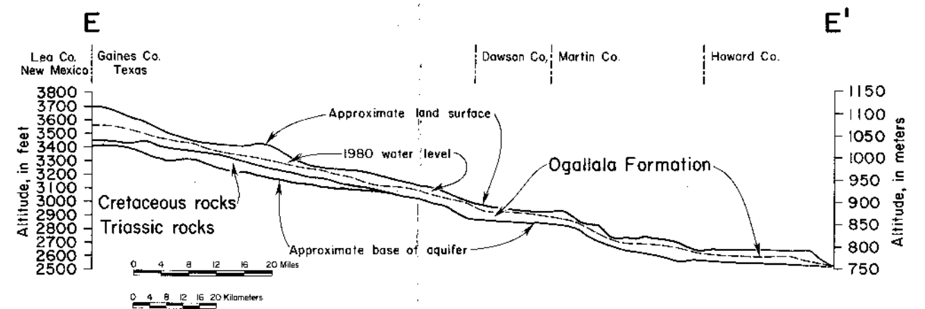
Figure 26 Generalized Geologic Section E-E'
