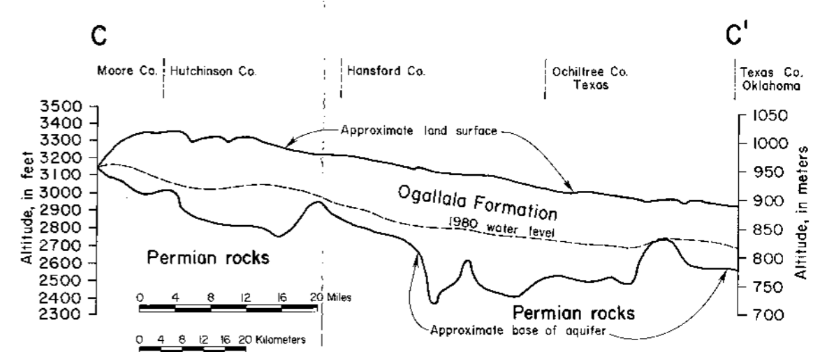
Figure 24 Generalized Geologic Section C-C'
