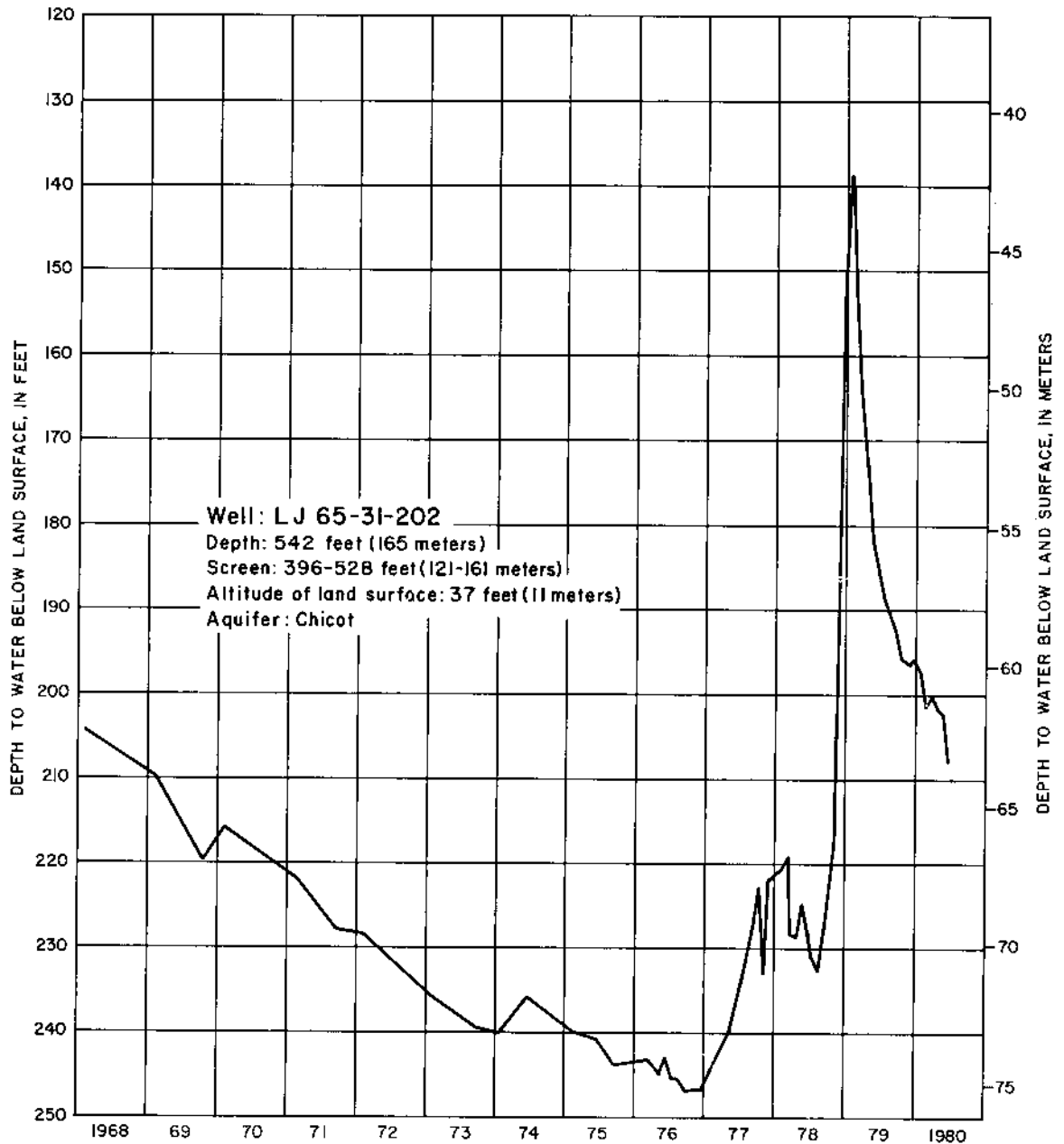
Figure 19.—Hydrograph Showing Changes in Water Levels in a Well Completed in the Chicot Aquifer Near a Ruptured Gas Well in Southeastern Harris County
