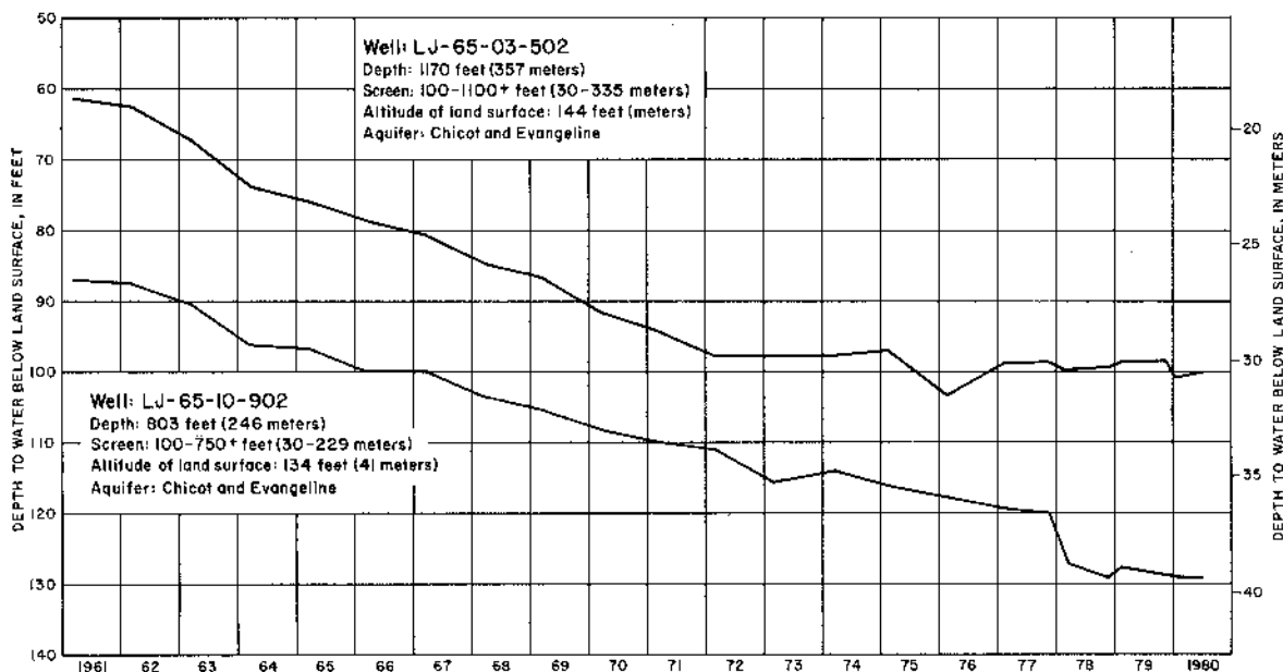
Figure 13.—Hydrographs Showing Changes in Water Levels in Two Wells in the Katy Area
