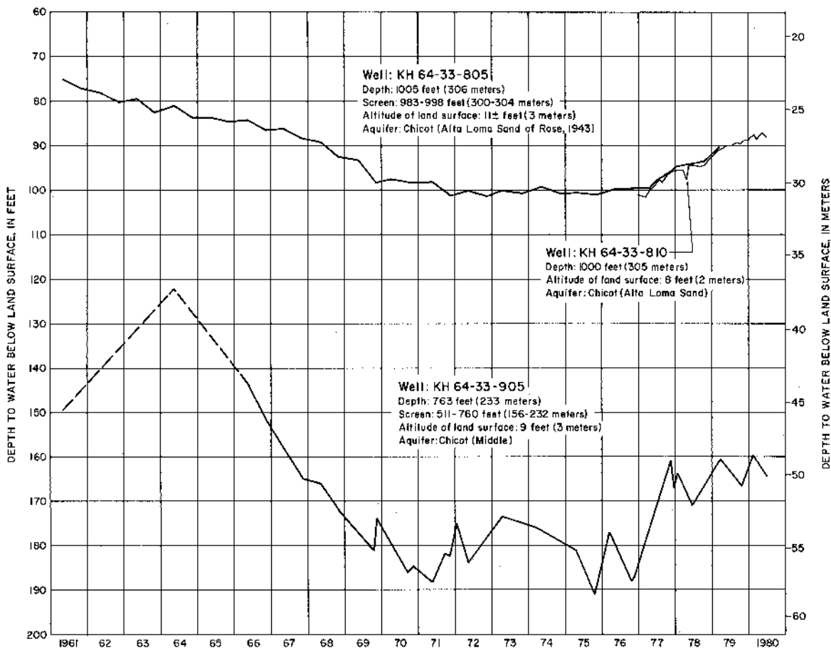
Figure 16.—Hydrographs Showing Changes in Water Levels in Three Wells in the Texas City Area
