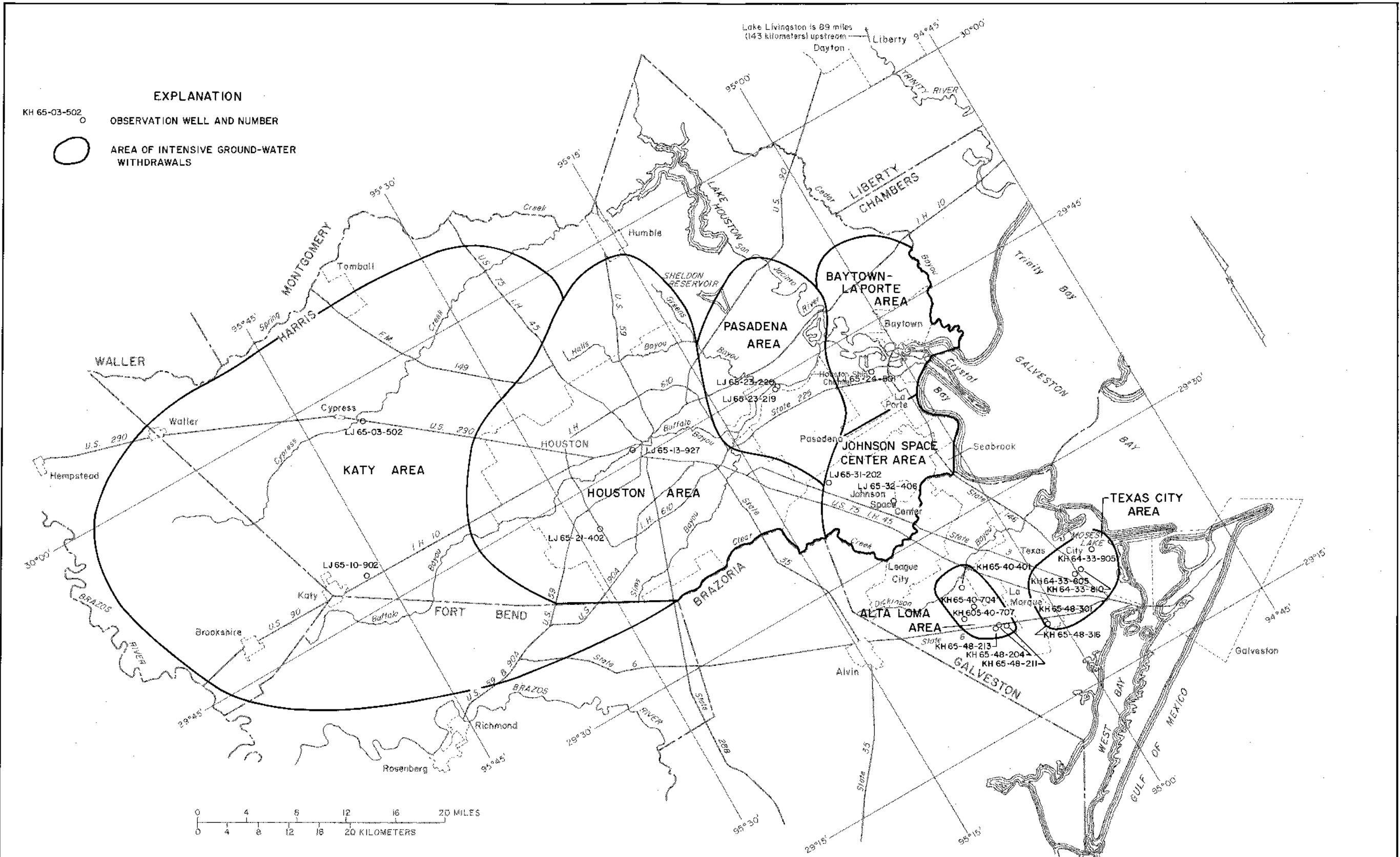
Figure 2 Location of Observation Wells and Areas of Intensive Ground-Water Withdrawals
