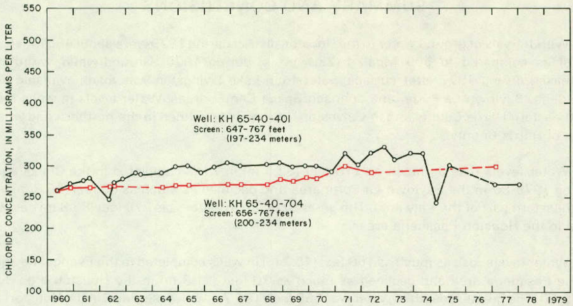
Figure 21.—Changes in Chloride Concentrations in Water From Two Wells in the City of Galveston's "New" Well Field North of Alta Loma
