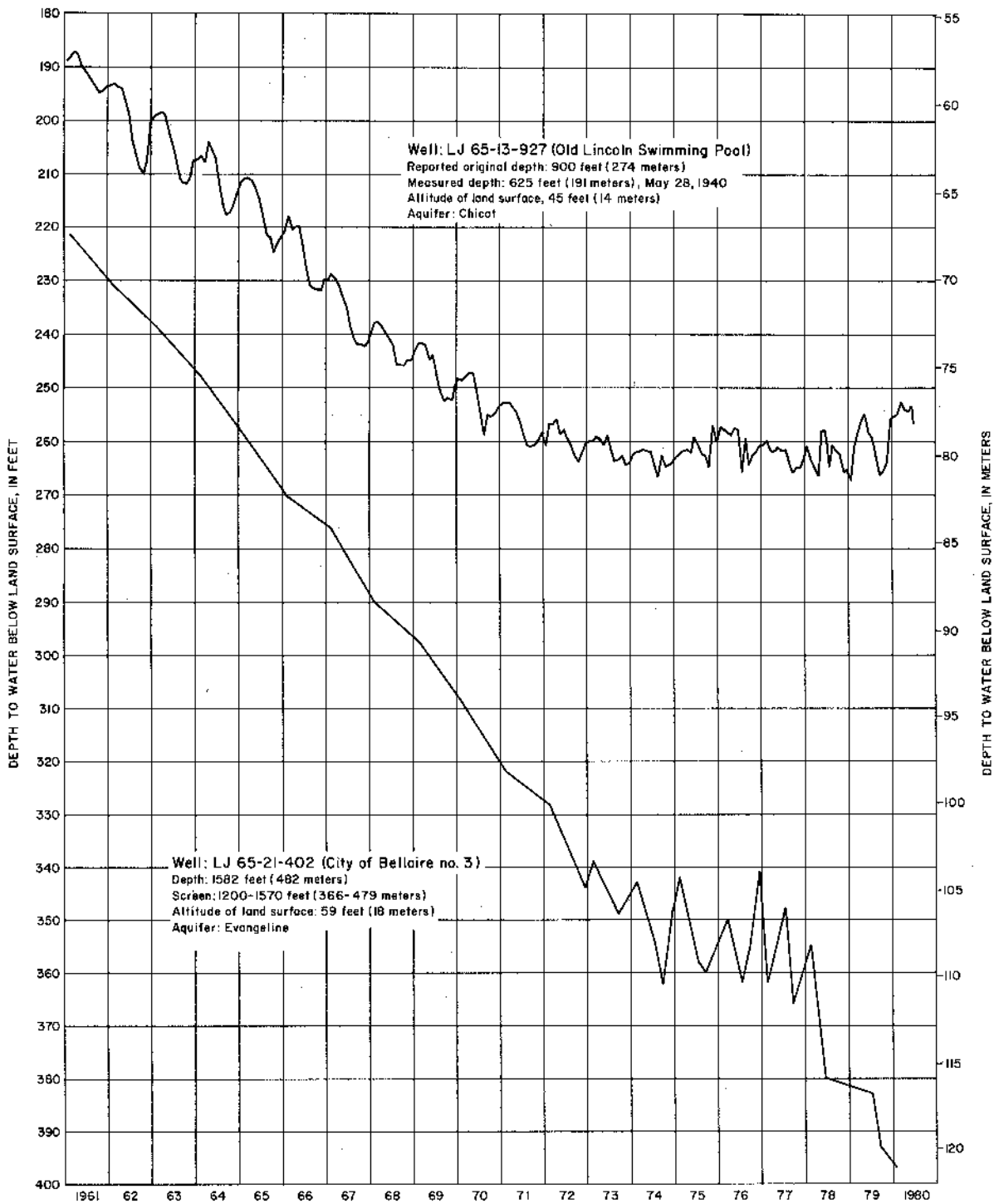
Figure 11 Hydrographs Showing Changes in Water Levels in Two Wells in the Houston Area
