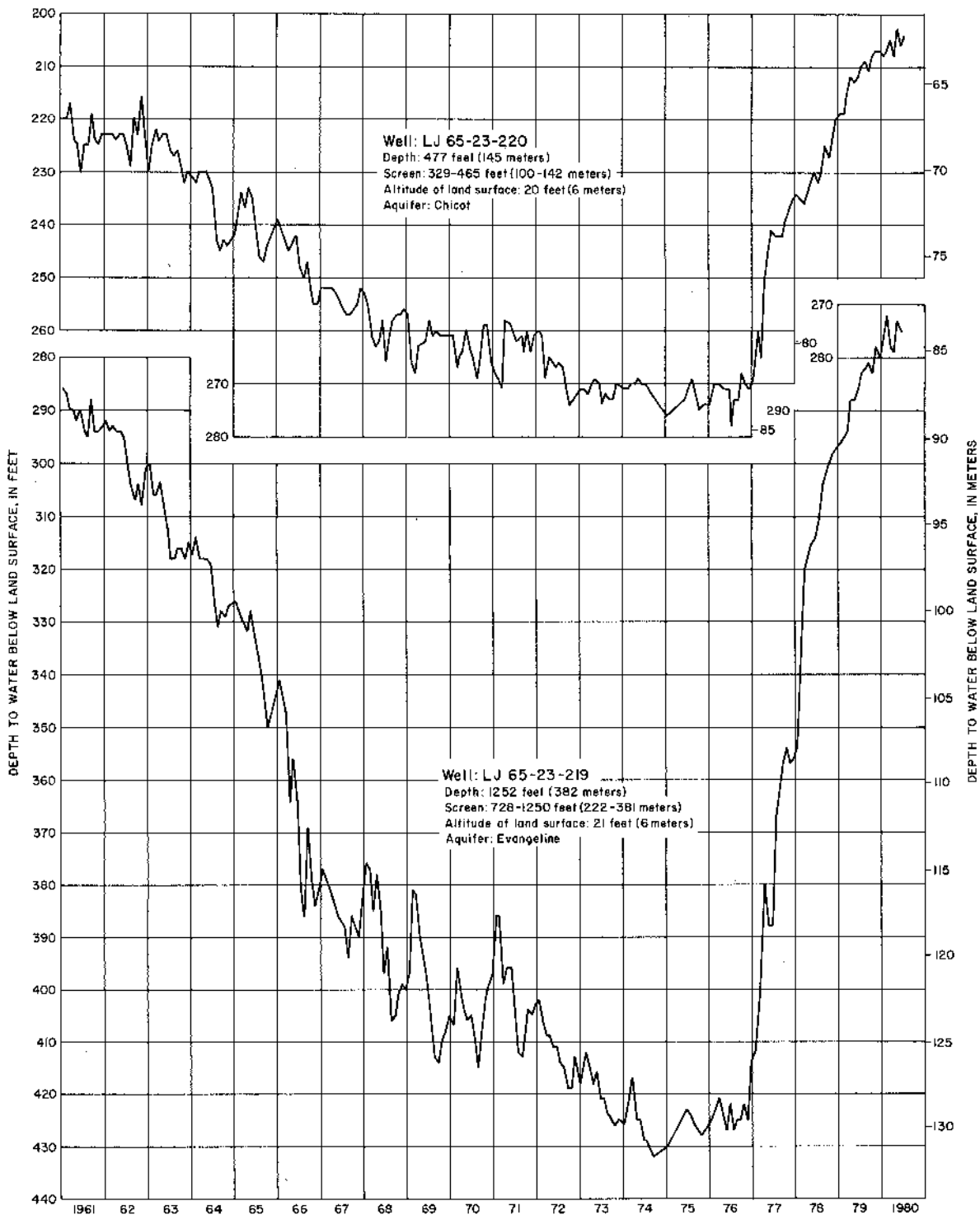
Figure 12 Hydrographs Showing Changes in Water Levels in Two Wells in the Pasadena Area
