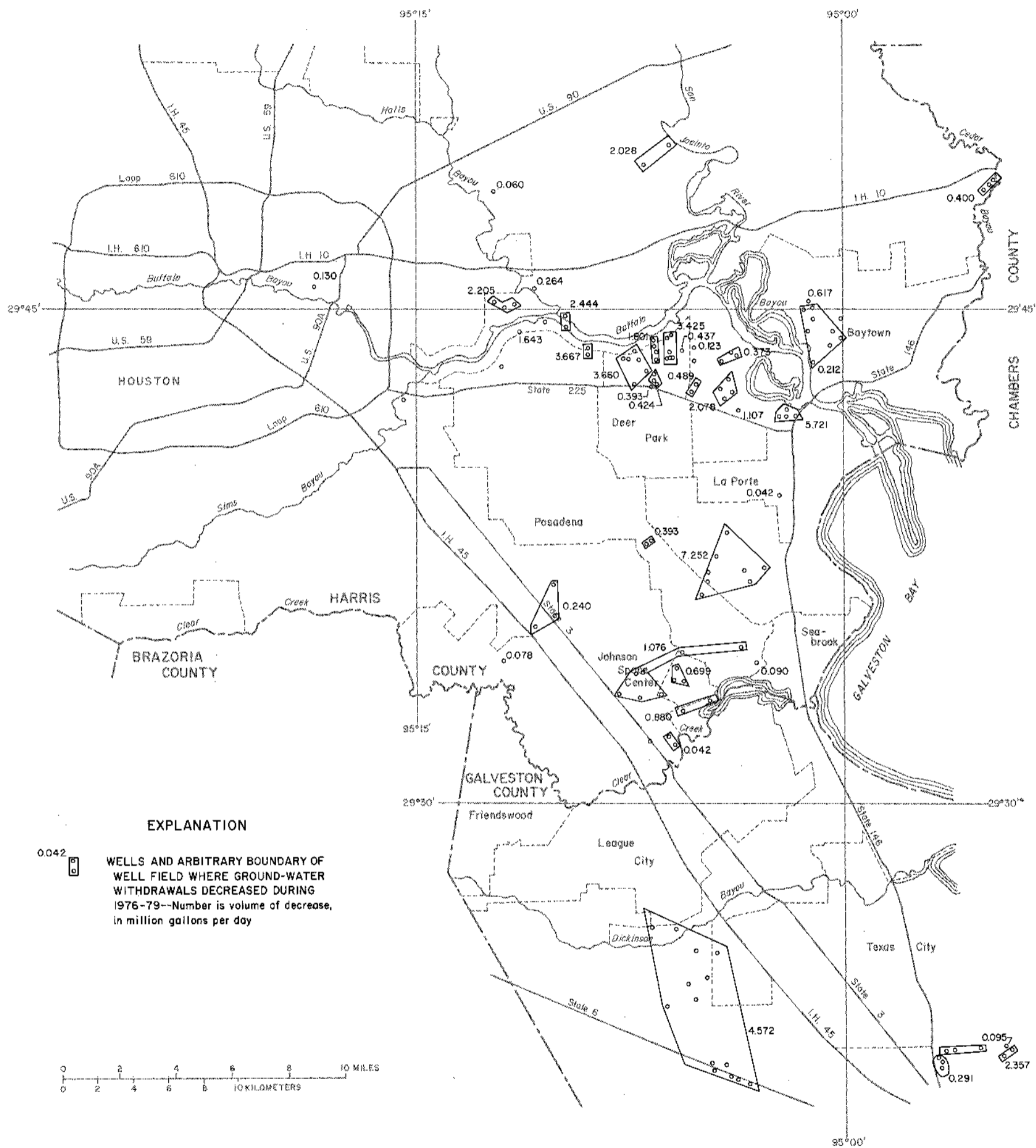
Figure 3 Location and Rate of Decrease in Ground-Water Production From the Chicot Aquifer, 1976-79
