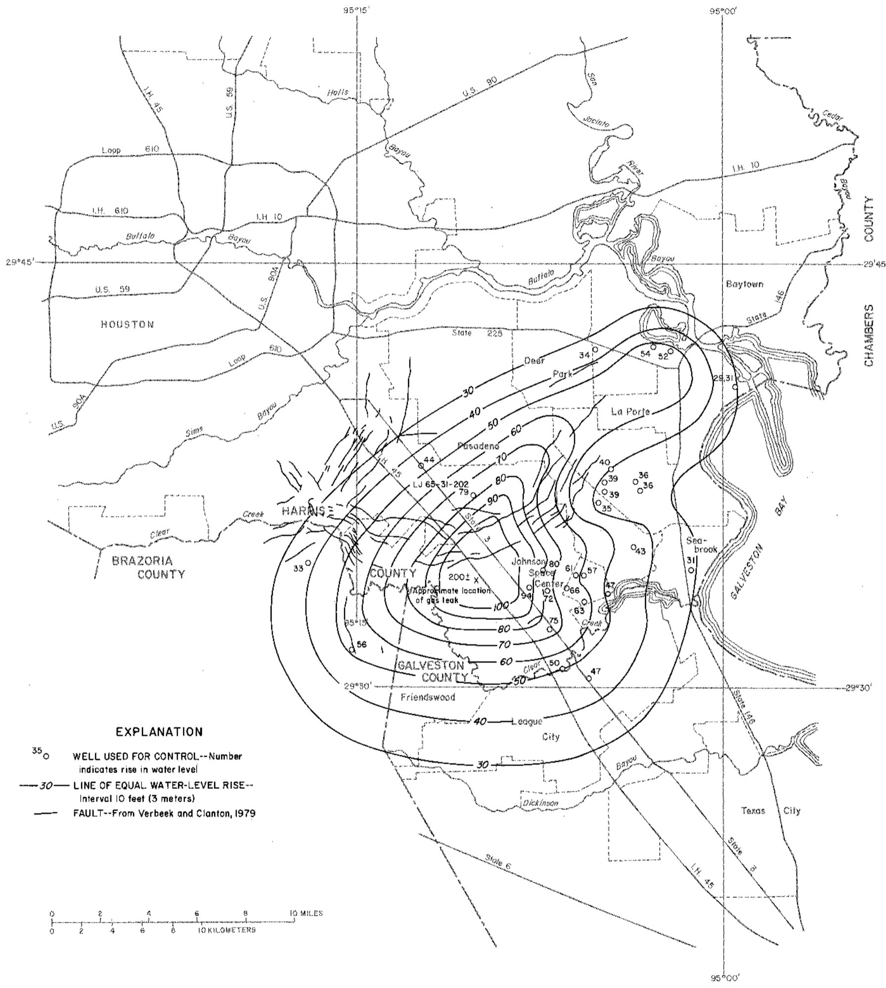
Figure 18 Changes in Water Levels in Wells Completed in the Chicot Aquifer Caused by a Leaking Gas Well
