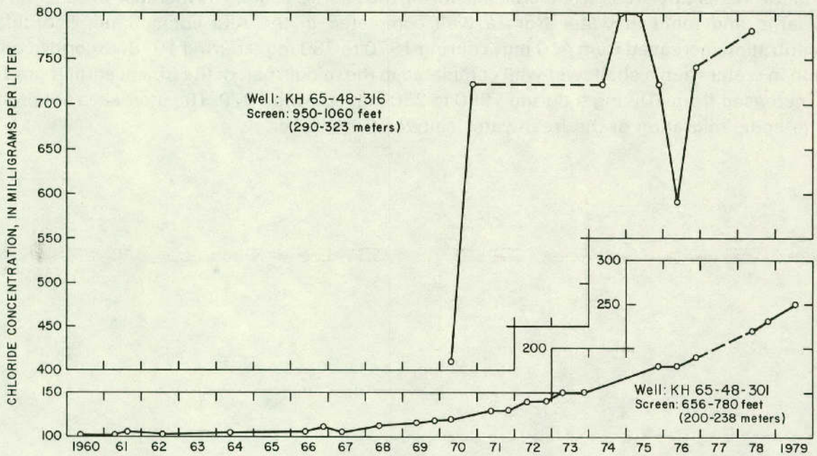
Figure 22.—Changes in Chloride Concentrations in Water From Two Wells in the Texas City Area
