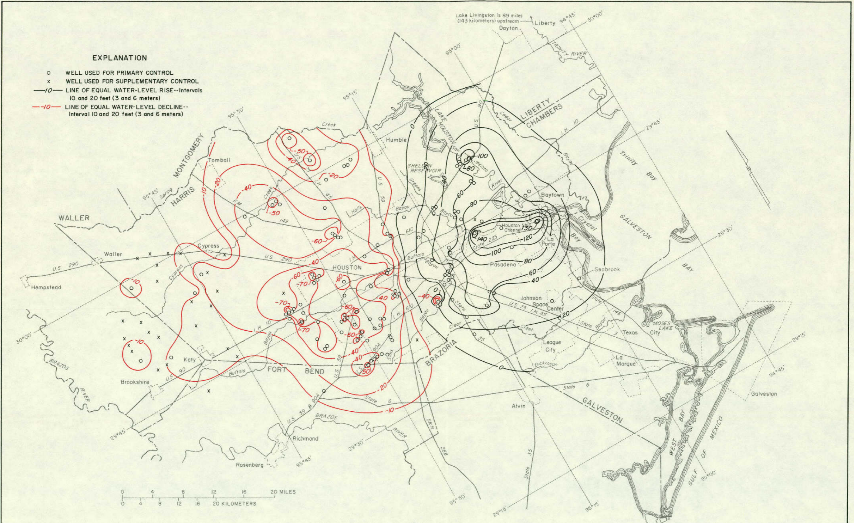
Figure 6 Approximate Water-Level Changes in Wells Completed in the Evangeline Aquifer, Spring 1975 to 1980
