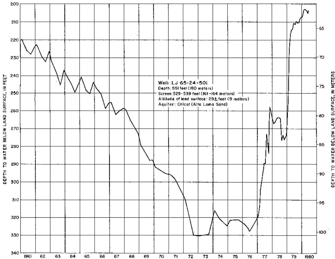
Figure 14.—Hydrograph Showing Changes in Water Levels in a Well Completed in the Alta Loma Sand of Rose (1943) in the Baytown-La Porte Area
