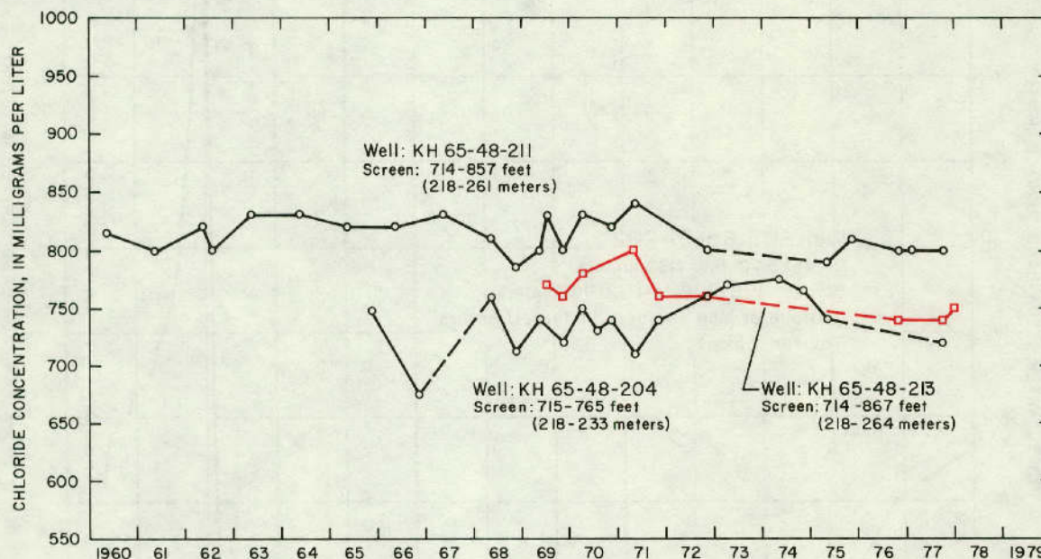
Figure 20.—Changes in Chloride Concentrations in Water From Three Wells in the City of Galveston's "Old" Well Field at Alta Loma
