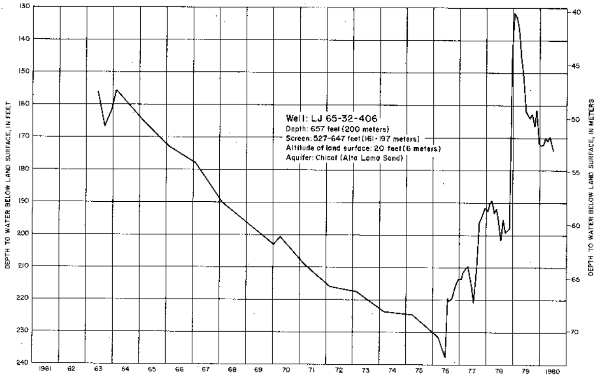
Figure 15.—Hydrograph Showing Changes in Water Levels in a Well Completed in the Alta Loma Sand of Rose (1943) in the Johnson Space Center Area
