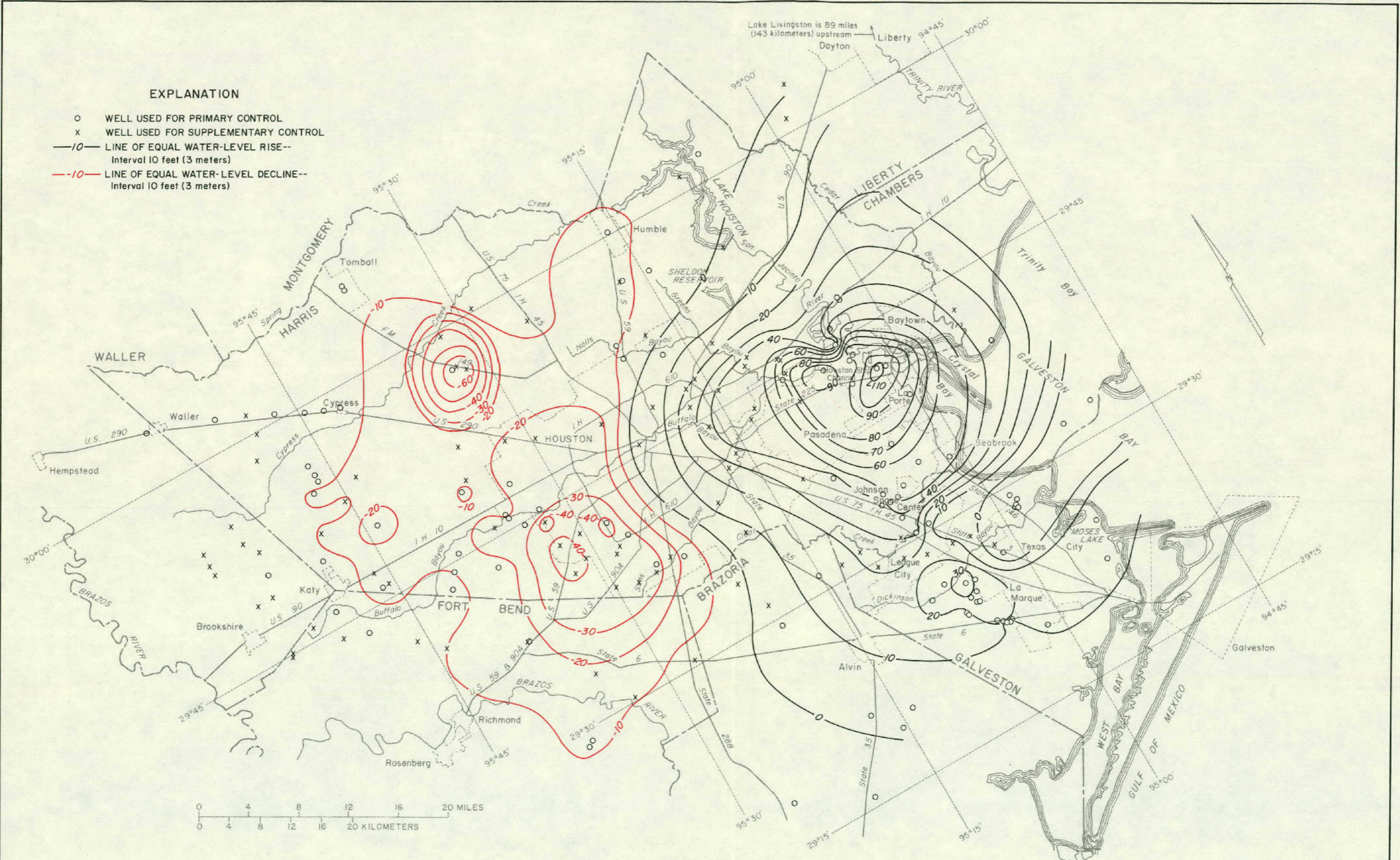
Figure 5 Approximate Water-Level Changes in Wells Completed in the Chicot Aquifer, Spring 1975 to Spring 1980
