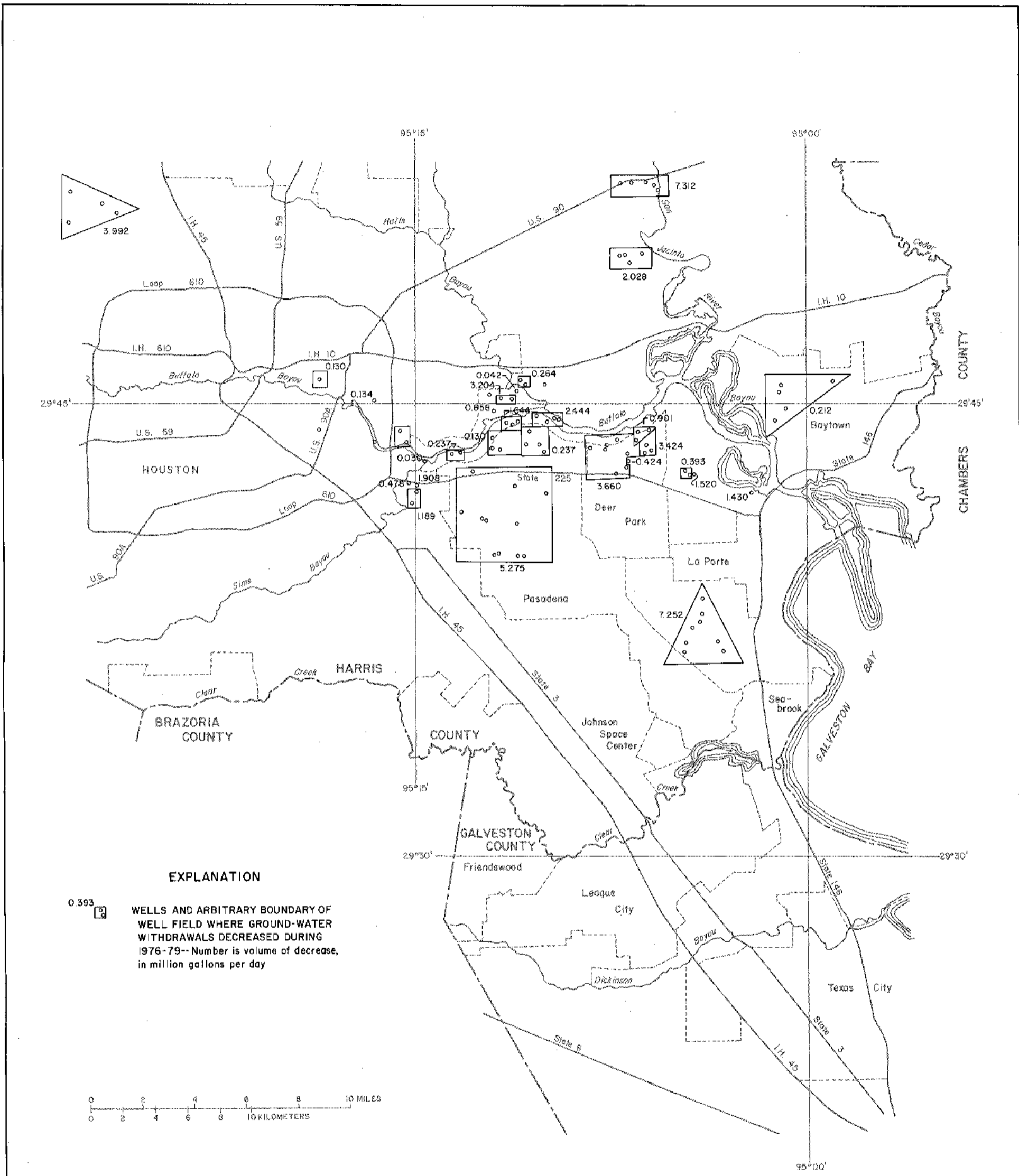
Figure 4 Location and Rate of Decrease in Ground-Water Production From the Evangeline Aquifer, 1976-79
