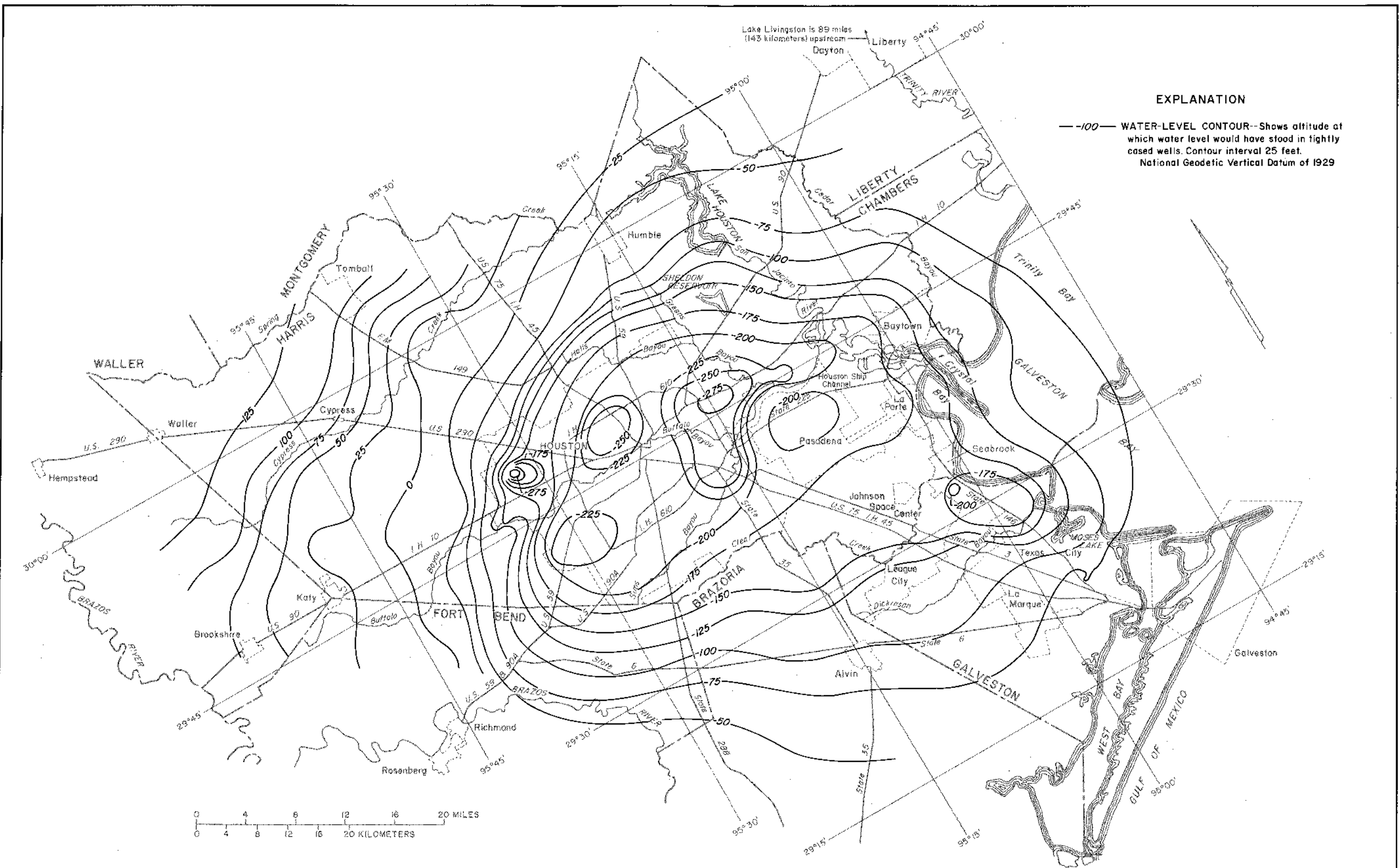
Figure 10 Approximate Altitude of Water Levels in Wells Completed in the Evangeline Aquifer, Spring 1980
