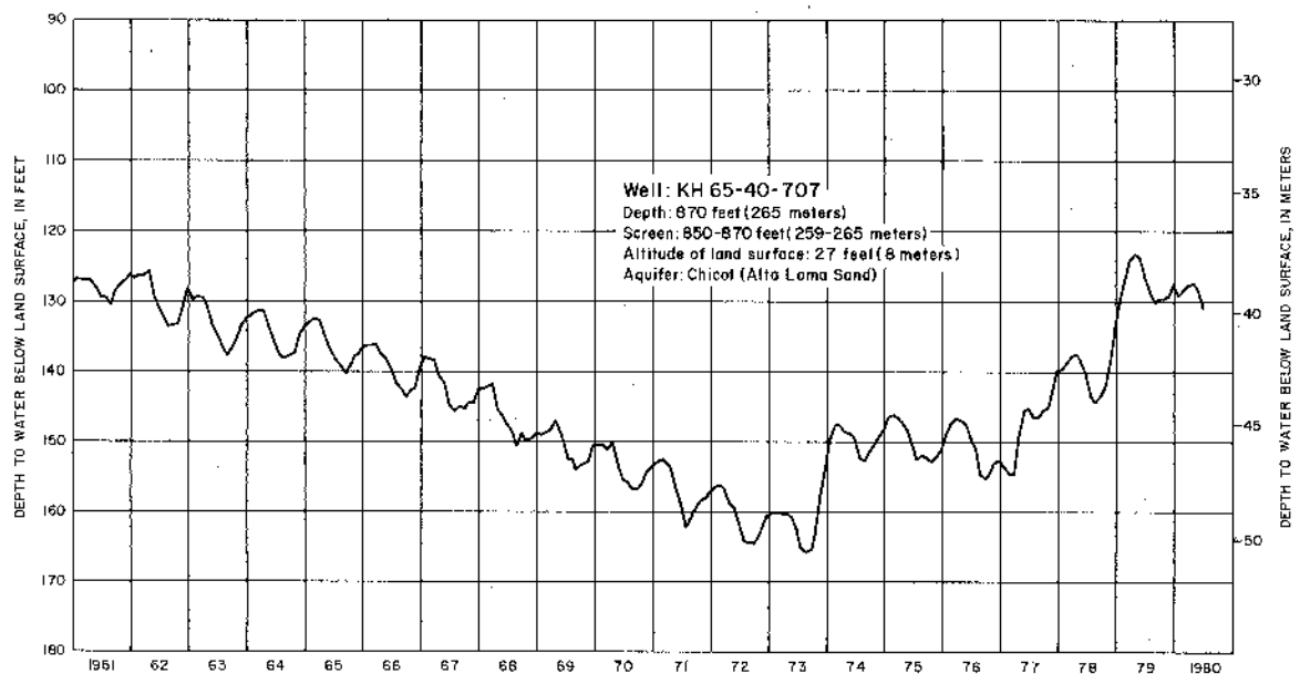
Figure 17.—Hydrographs Showing Changes in Water Levels in a Well Completed in the Alta Loma Sand of Rose (1943)
