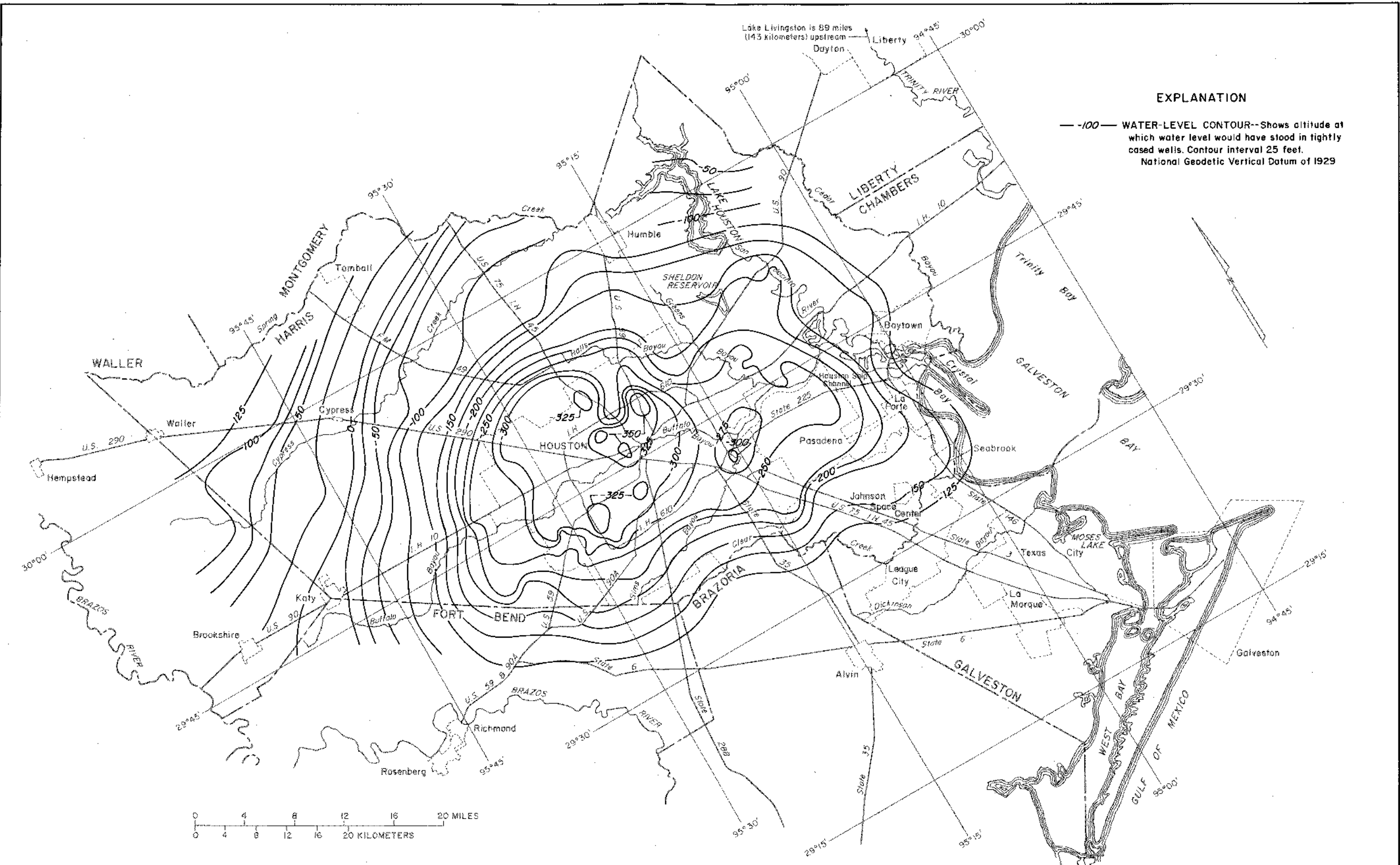
Figure 9 Approximate Altitude of Water Levels in Wells Completed in the Chicot Aquifer, Spring 1980
