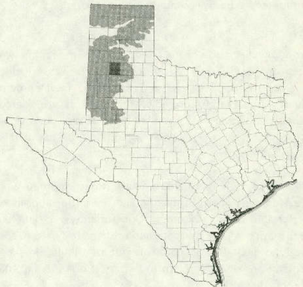
Location of Hale County, and Extent of the Ogallala Aquifer in Texas
