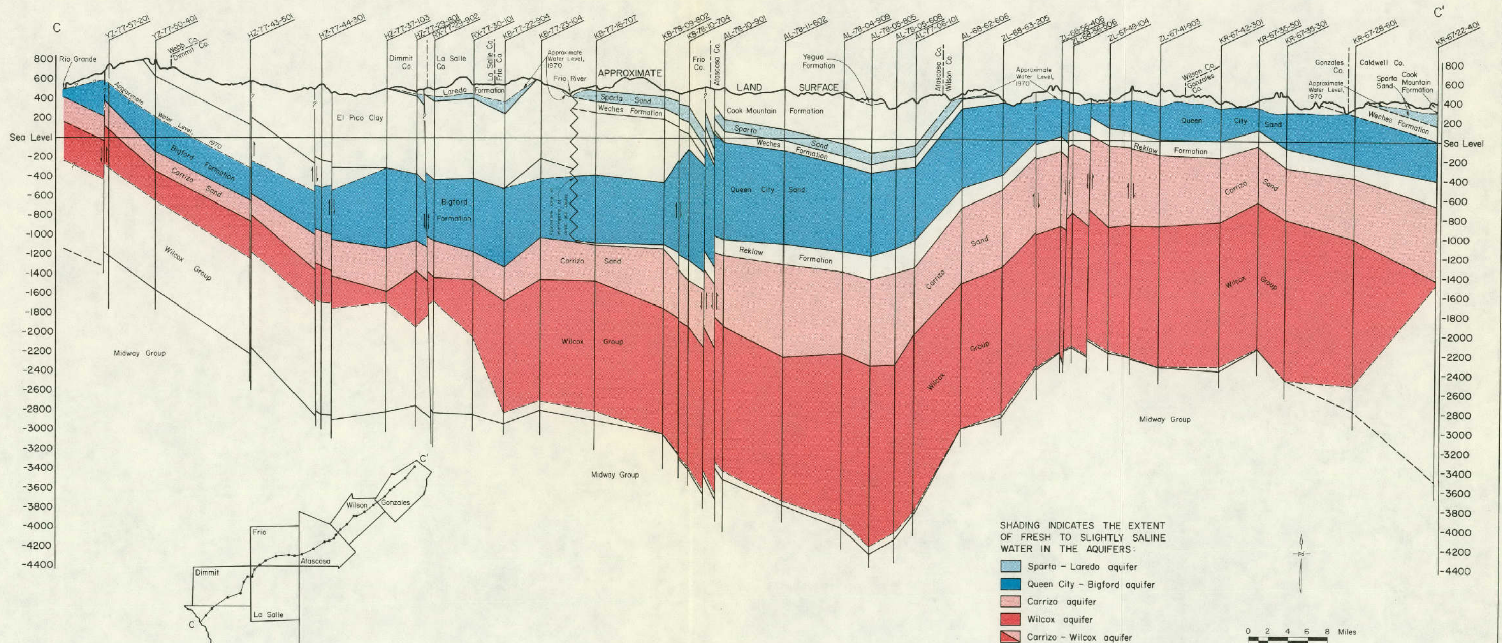
Figure 29 Geohydrologic Section C-C', Webb, Dimmit, La Salle, Frio, Atascosa, Wilson, and Gonzales Counties
