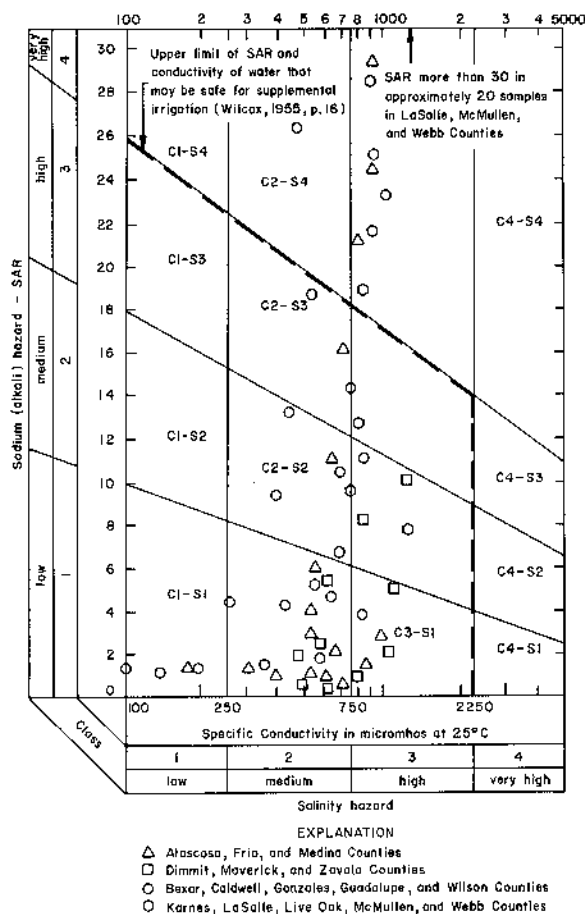
Figure 6.—Classification of Irrigation Waters, and Quality of Water From Representative Wells in the Carrizo Aquifer (After U.S. Salinity Laboratory Staff, 1954, p. 80)
