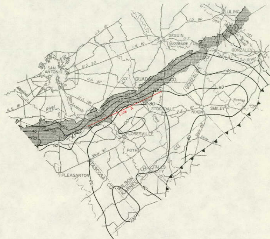
Proposed Line of Wells (Line B) Pumping 20,000 Acre-Feet Per Year Under Artesian Conditions
