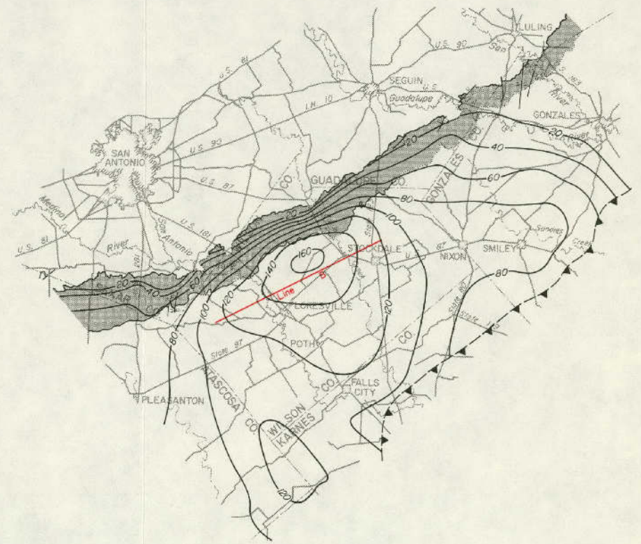
Proposed Line of Wells (Line A) Pumping 40,000 Acre-Feet Per Year Under Water - Table Conditions
