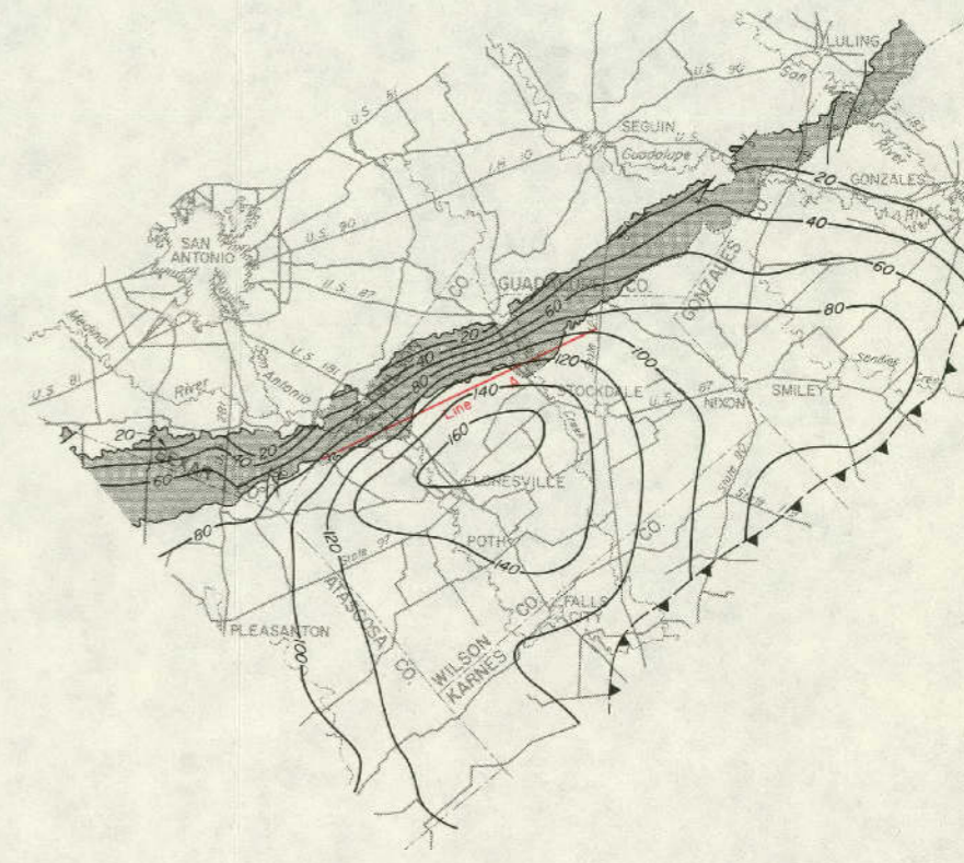
Proposed Line of Wells (Line B) Pumping 40,000 Acre-Feet Per Year Under Artesian Conditions
