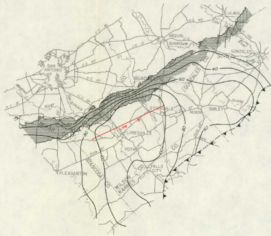
Proposed Line of Wells (Line A) Pumping 30,000 Acre-Feet Per Year Under Water - Table Conditions
