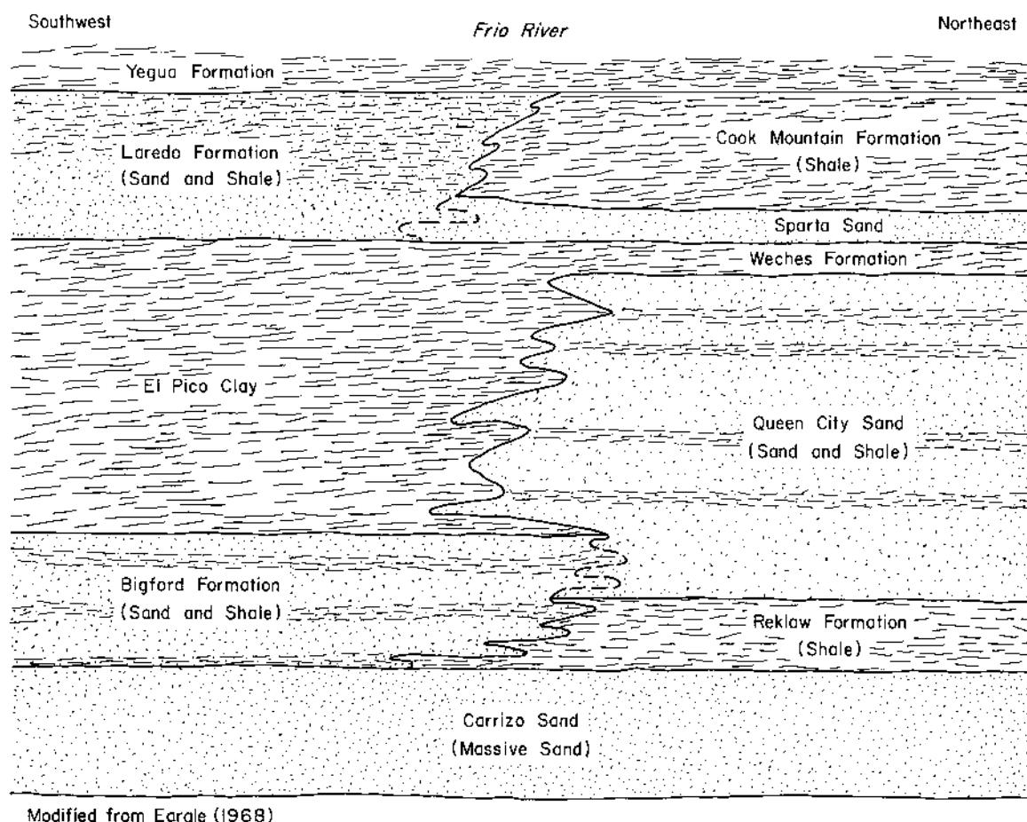
Figure 3.—Idealized Geologic Section Illustrating the Interfingering of Sands and Shales of the Claiborne Group in the Vicinity of the Frio River
