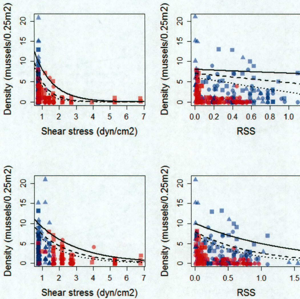
Figure 23. Quantile regression models for mussel density for Shear stress ( \tau , dynes/cm 2 ) and Relative shear stress (RSS) at low (top) and high (bottom) flows. Solid, dashed, and dotted lines represent 95 th , 90 th , and 85 th quantile regression lines, respectively. Points shaded blue denote 0.25 m 2 quadrats from protected habitat types (i.e., BH = bank habitat; BPB = immediately downstream of point bar; and BW = backwater), whereas points shaded red indicate quadrats from exposed habitat types (i.e., MC = mid-channel and FPB = front of point bars).
