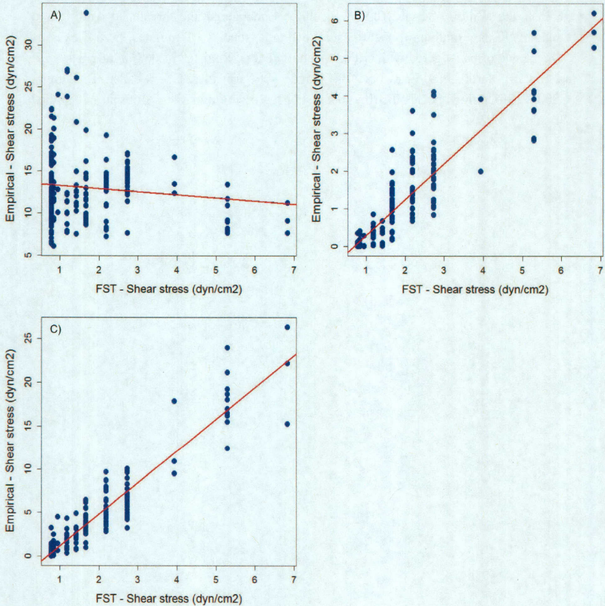
Figure A. Relationship between empirically derived shear stress (Empirical) and point-specific shear stress (FST). Empirically derived values of shear stress in panel (A) were calculated using the following formula: \tau = gSd ; where g is the acceleration due to gravity ( 980 \text{ cm/s}^2 ), S is slope of the water surface, and d is water depth (cm). For panels (B) and (C), empirical shear stress was obtained using the following: U/5.75 \log_{10}(12d/k_s) ; where U is currently velocity (cm/s) measured at the bed surface (for panel B) or at 0.6 \times depth (for panel C), d is water depth (cm), and k_s is bed roughness (see Table 3). The best-fit line, using OLS regression is shown for reference: (A) R^2 = 0.01 , p = 0.08 , (B) R^2 = 0.84 , p < 0.001 , and (C) R^2 = 0.89 , p < 0.001 .
