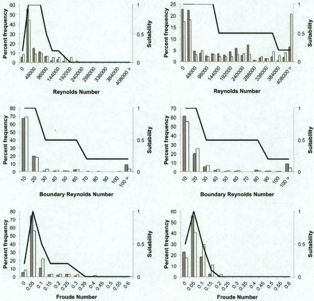
Figure 15. Percent frequency of occurrence (grey bars), habitat availability (white bars), and NPTL values (solid line; 95% confidence level) for Reynolds number, Boundary Reynolds number, and Froude number during low (left) and high (right) flows. Suitability criteria are shown only for all mussels and are based on abundance data from quantitative sampling. The number of observations used were: N = 524.
