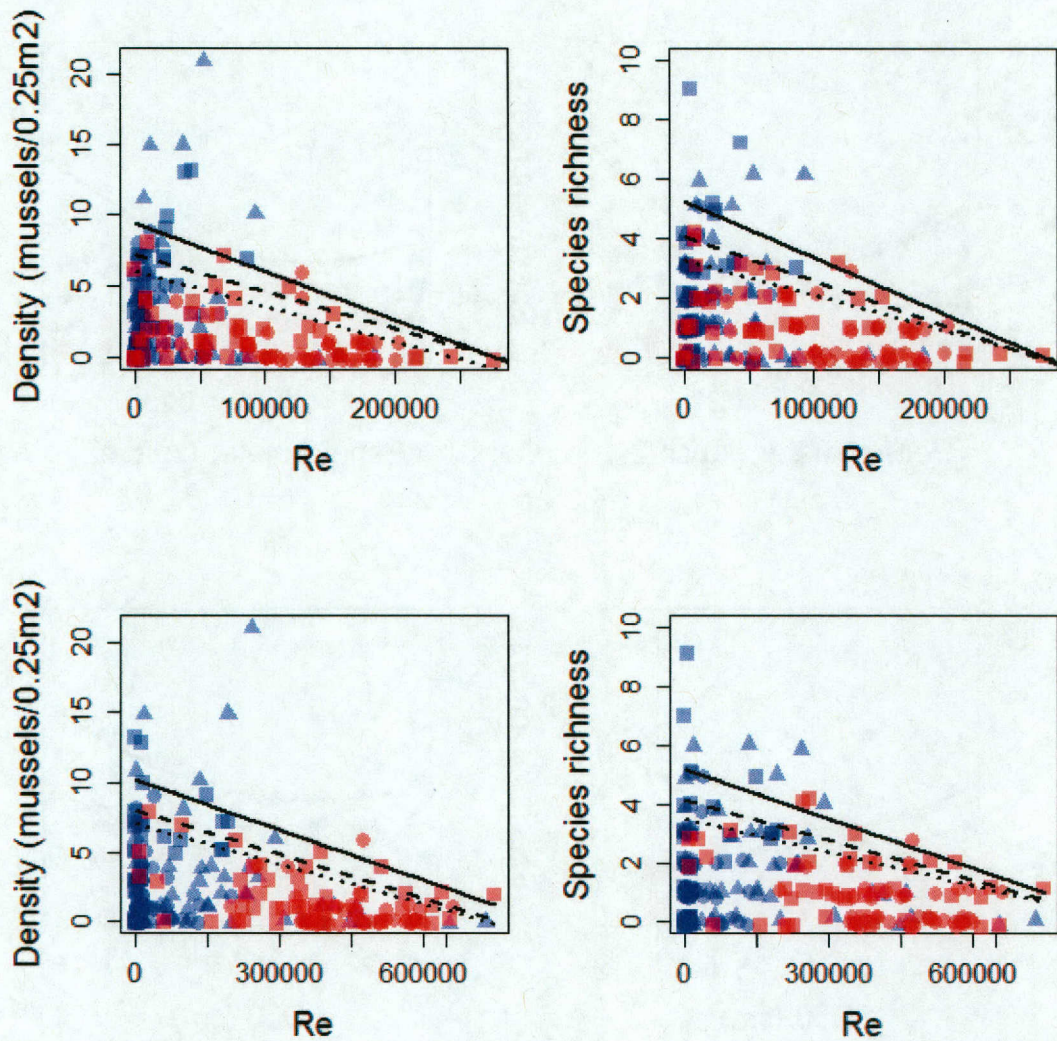
Figure 25. Quantile regression models for Reynolds number ( Re ) for mussel density (left) and species richness (right) at low (top) and high (bottom) flows. Solid, dashed, and dotted lines represent 95 th , 90 th , and 85 th quantile regression lines, respectively. Points shaded blue denote 0.25 m 2 quadrats from protected habitat types (i.e., BH = bank habitat; BPB = immediately downstream of point bar; and BW = backwater), whereas points shaded red indicate quadrats from exposed habitat types (i.e., MC = mid-channel and FPB = front of point bars).
