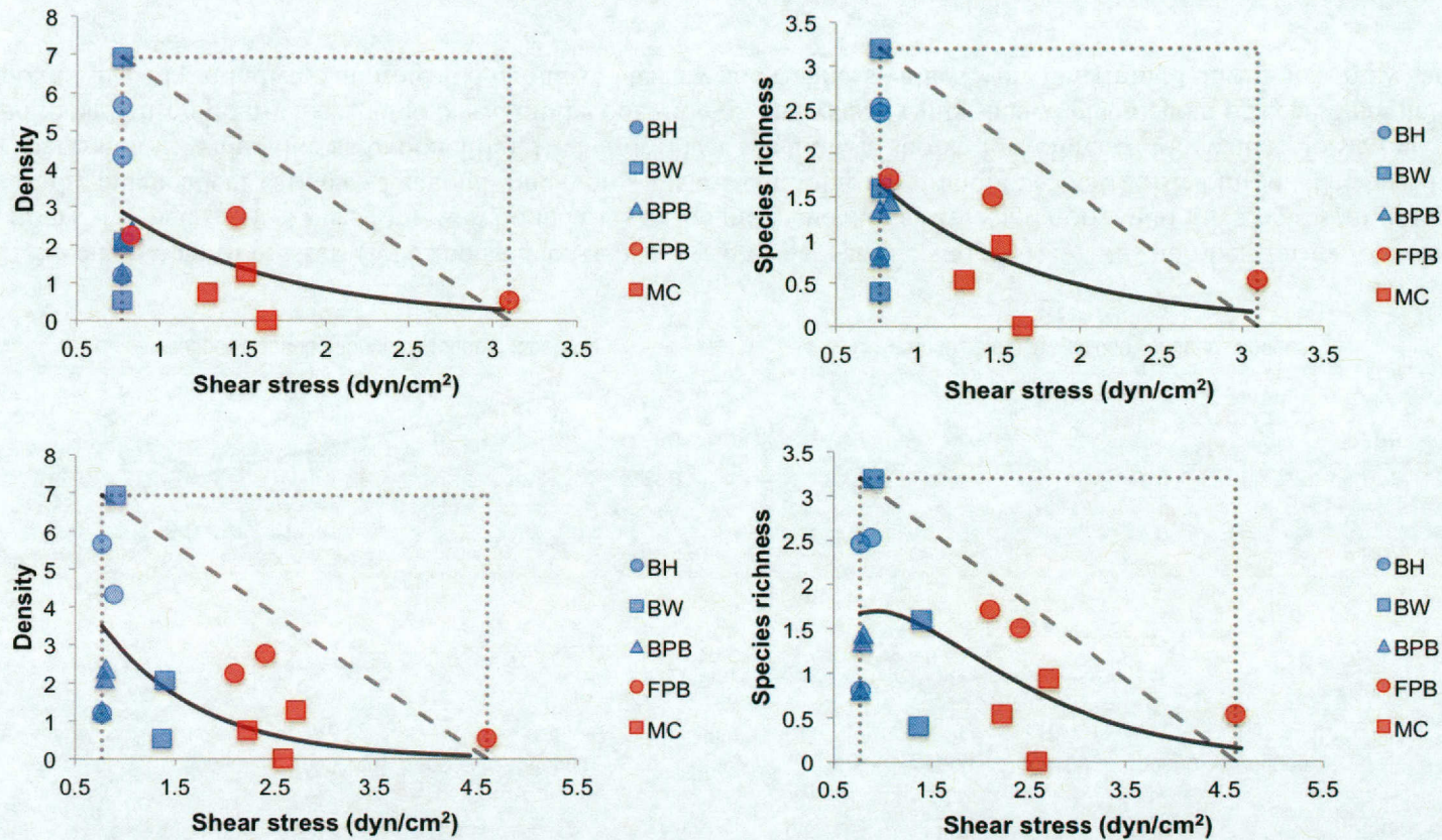
Figure 11. Mean number of mussels (left) and species richness (right) per sample site for Shear stress during low (top) and high flows (bottom). Dashed vertical lines represent boundaries of the independent variable and horizontal lines represent the upper boundary of the independent variable. Diagonal line represents the cut point for a random (50:50) distribution. The best-fit line, using nonlinear regression fit with either an exponential, Richer or linear function, is shown for reference for scatter plots where sites were determined to be non-randomly distributed based on the post-hoc X^2 analysis. Points shaded blue denote protected habitat types, whereas points shaded red indicate unprotected habitats.
