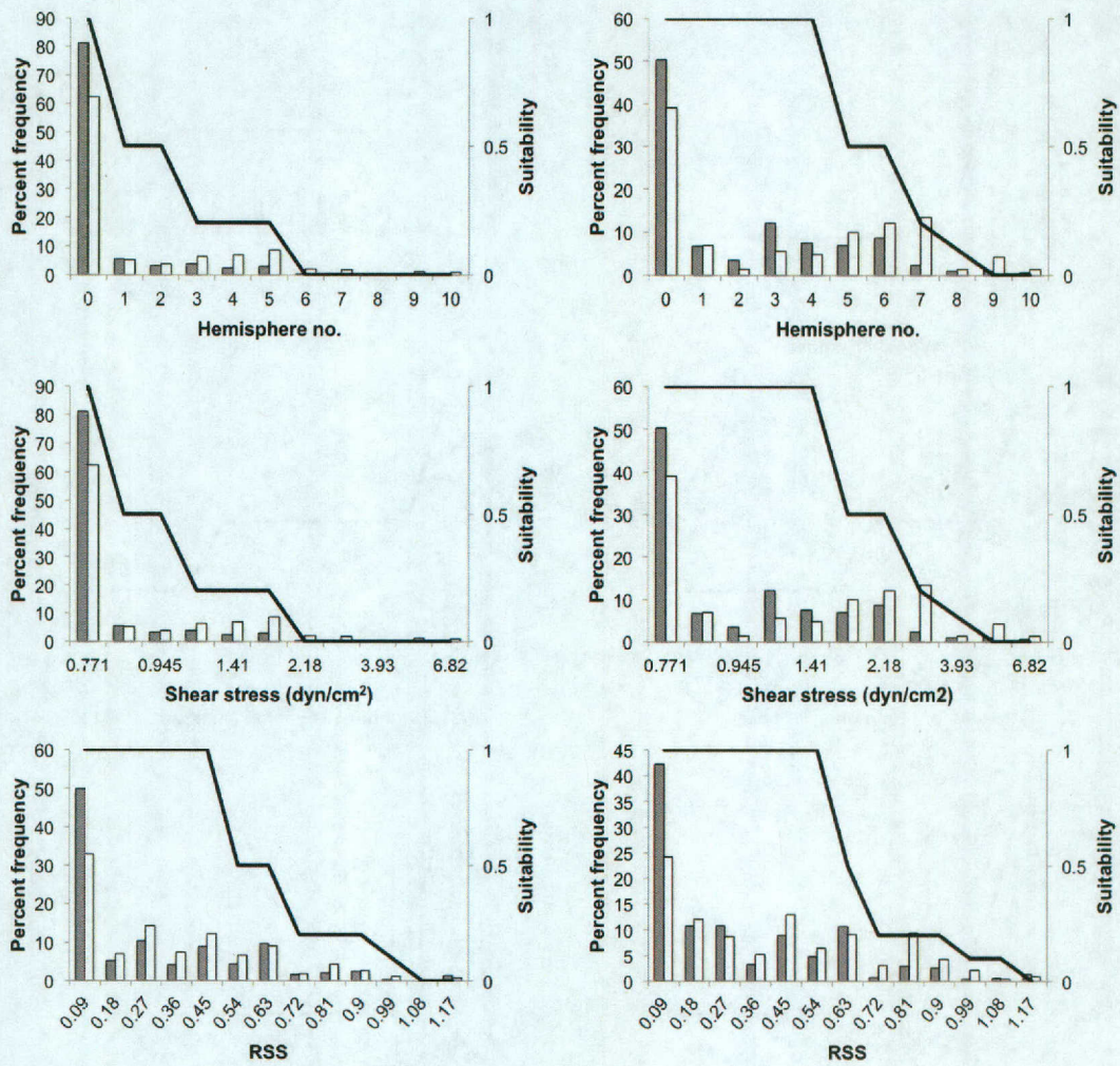
Figure 16. Percent frequency of occurrence (grey bars), habitat availability (white bars), and NPTL values (solid line; 95% confidence level) for Hemisphere no., shear stress, and RSS during low (left) and high (right) flows. Suitability criteria are shown only for all mussels and are based on abundance data from quantitative sampling. The number of observations used were: N = 524.
