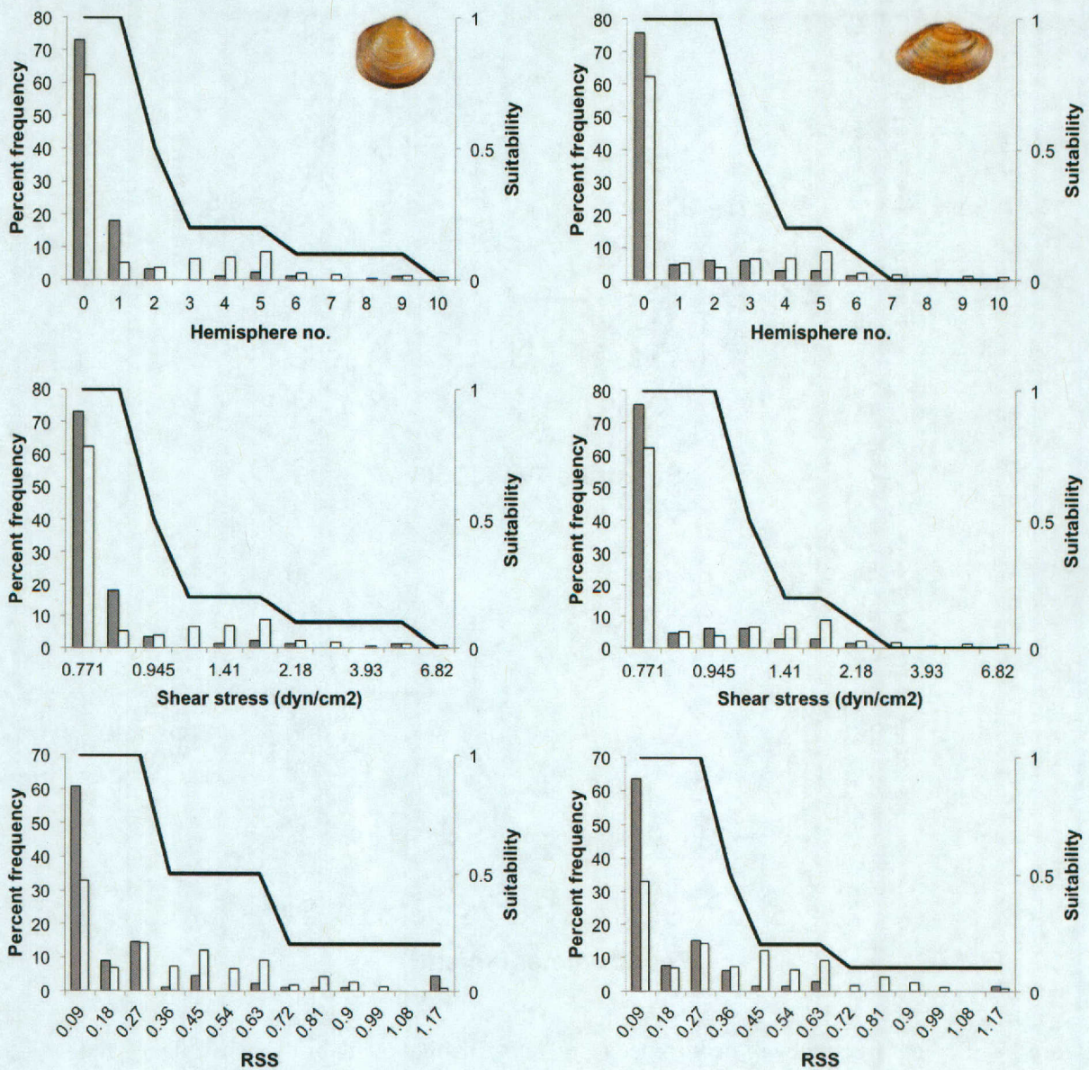
Figure 18. Percent frequency of occurrence (grey bars), habitat availability (white bars), and NPTL values (solid line; 95% confidence level) for Hemisphere no., shear stress, and RSS during low flows. Suitability criteria are shown for Q. houstonensis (left) and T. macrodon (right). Suitability criteria are based on abundance data from quantitative sampling. The number of observations used were: N = 89 ( Q. houstonensis ) and N = 66 ( T. macrodon ).
