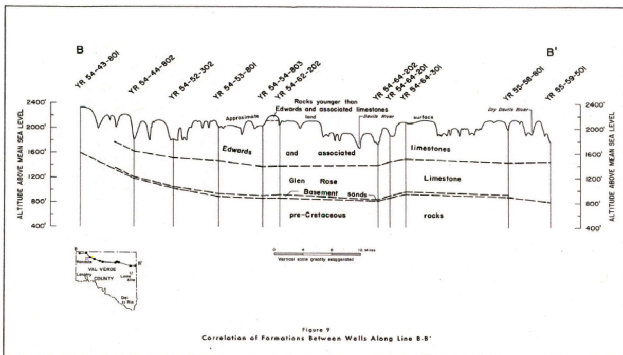
Figure 3-4. Generalized cross-section (B-B') of Cretaceous deposits in Val Verde County (Reeves and Small, 1973).
