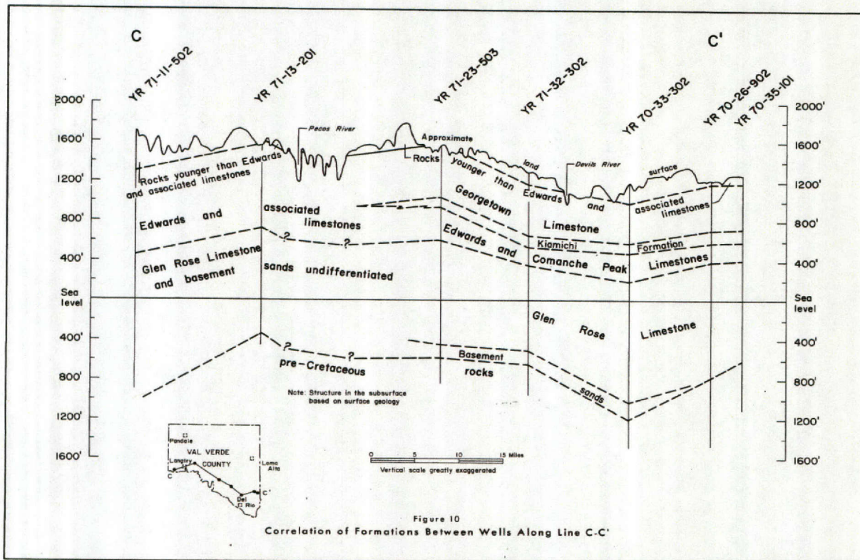
Figure 3-5. Generalized cross-section (C-C') of Cretaceous deposits in Val Verde County (Reeves and Small, 1973).
