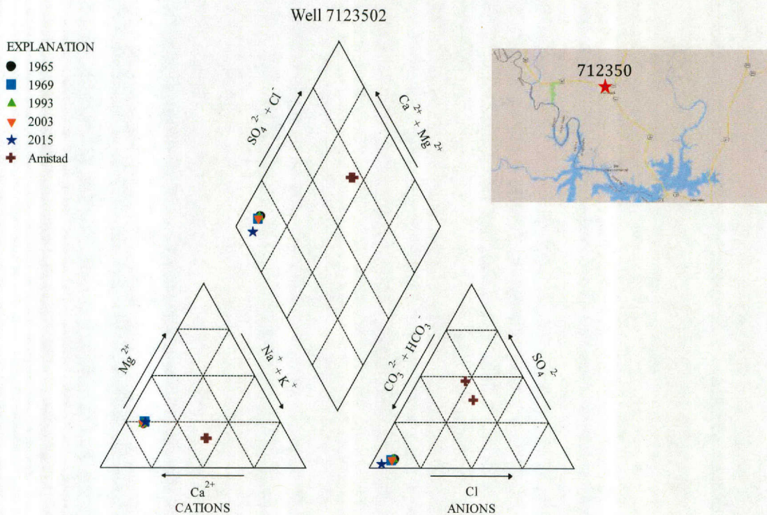
Figure 4-25. Piper diagram for Well 7123502, located 5.75 miles north of Amistad Reservoir near Comstock. The groundwater chemistry in this area has not changed appreciably since the reservoir filled. Data from TWDB and TCEQ, 2018a.
