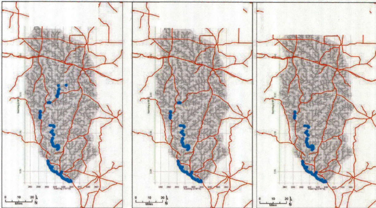
Figure 5-5. Simulation of spring locations (shown in blue) based on various groundwater pumping scenarios (Toll and others, 2017).
