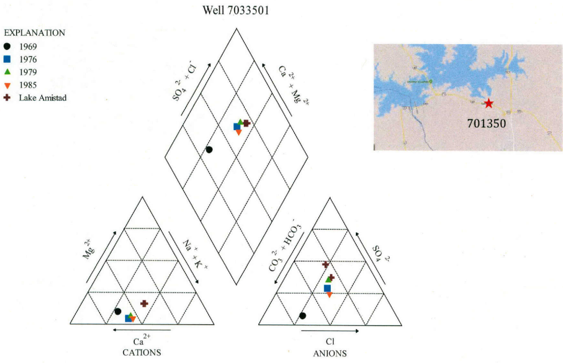
Figure 4-23. Piper diagram for Well 7033501, 0.75 miles southeast of Amistad Reservoir. Groundwater chemistry in this area is dominated by the reservoir influence by 1976. Data from TWDB and TCEQ, 2018a.
