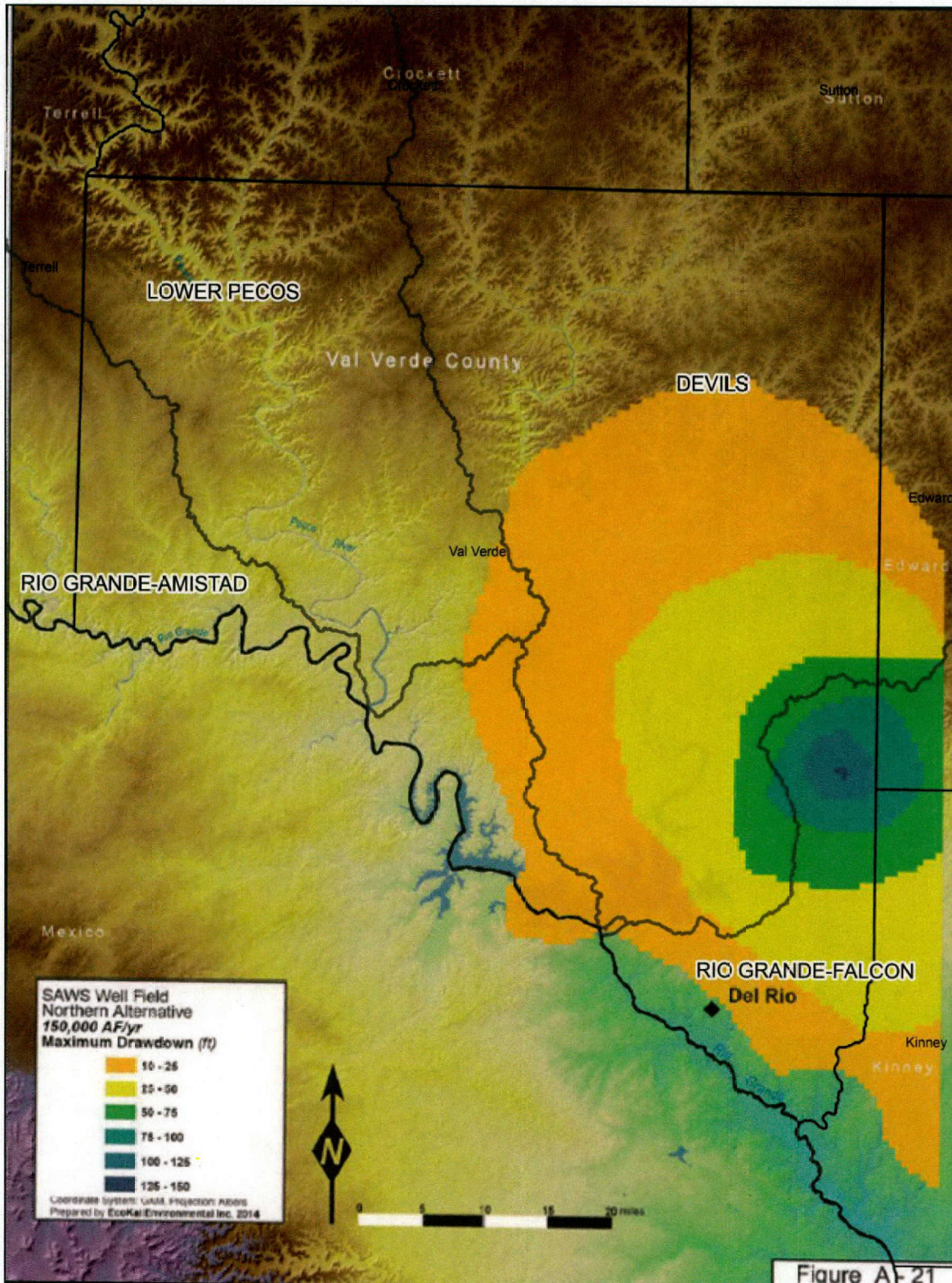
Figure 9. Simulated drawdown of pumping from the SAWS well field-northern alternative. Figure A-21 from EcoKai Environmental, Inc. and Hutchison (2014)
