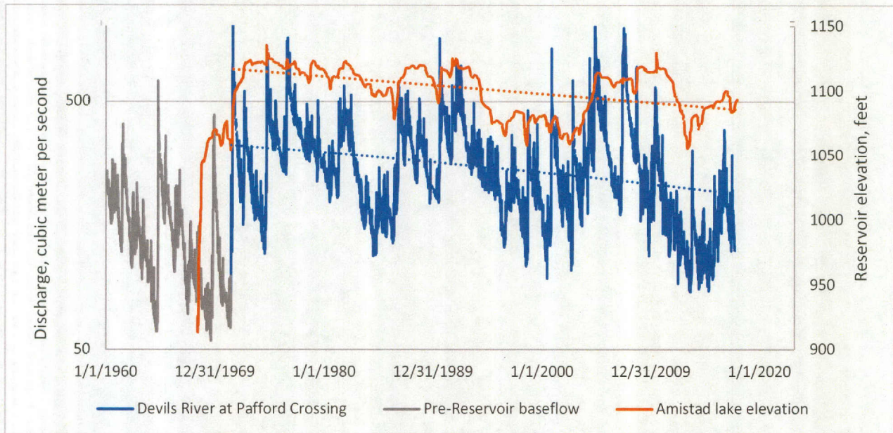
Figure 6-5. Comparison of Amistad Reservoir surface elevation and Devils River baseflow measured at Pafford Crossing. Decadal trends in stream baseflow mimic variability in reservoir elevation. Linear trend lines for baseflow and reservoir elevation are shown as dotted lines. Data from International Boundary and Water Commission, 2018.
