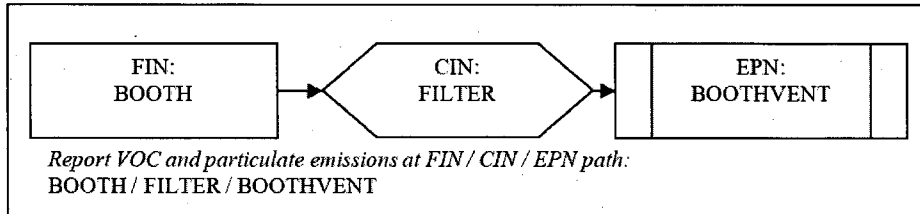
Figure 3-16. Paint Booth: Particulate Emissions Abated by a Filter
