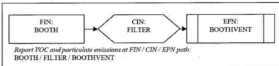
Figure 3-16. Paint Booth-Particulate Emissions Abated by a Filter
