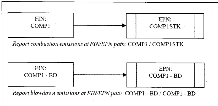
Figure 3-11. Blowdown-Separate Compressor Engine and Blowdown Vents
