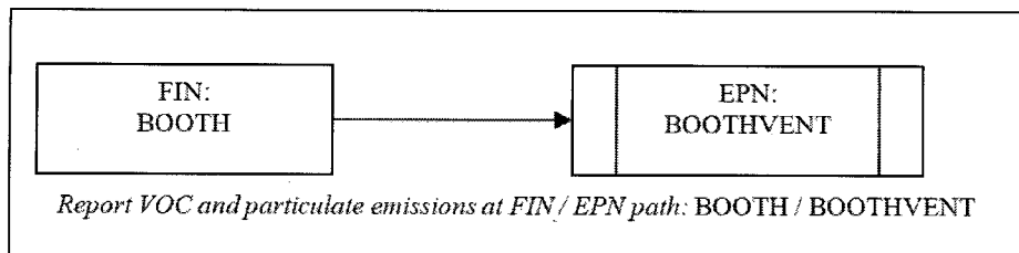
Figure 3-15. Paint Booth-Unabated
