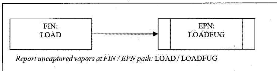
Figure 3-9. Loading Area-Unabated
