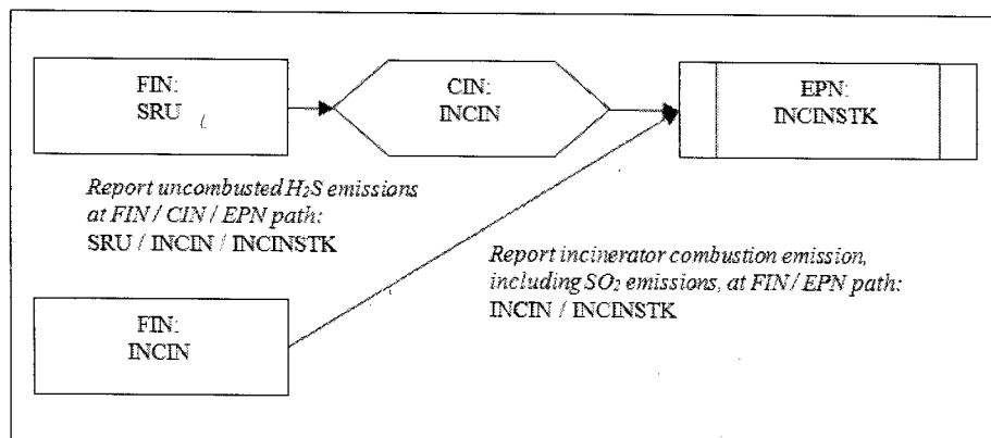
Figure 3-7. Sulfur Recovery Unit with Incinerator
