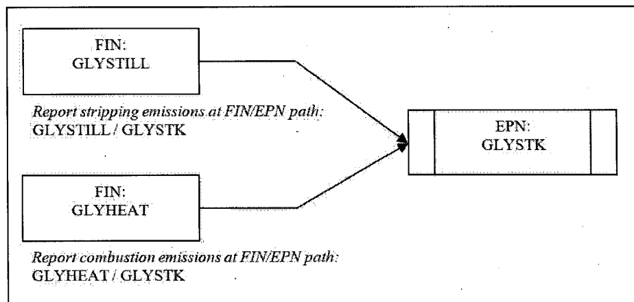
Figure 3-2. Glycol Unit-Common Still and Vents
