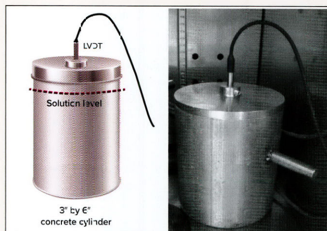
Left: The test setup for the ACCT method. Right: A fully assembled ACCT device placed inside an oven.
