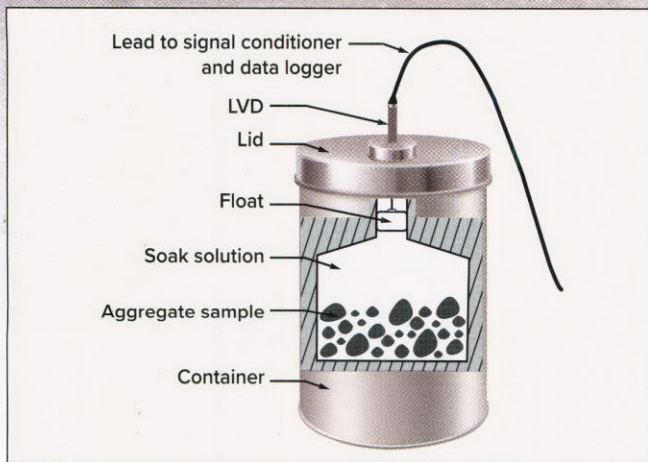
The test setup for the VCMD method.
