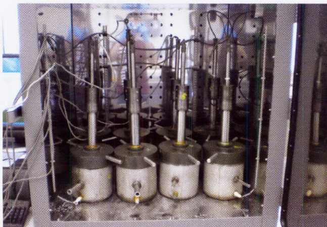
Several fully assembled VCMDs inside an oven used for conducting this test at a particular temperature in the Center for Infrastructure Renewal’s Concrete Innovation Laboratory.
