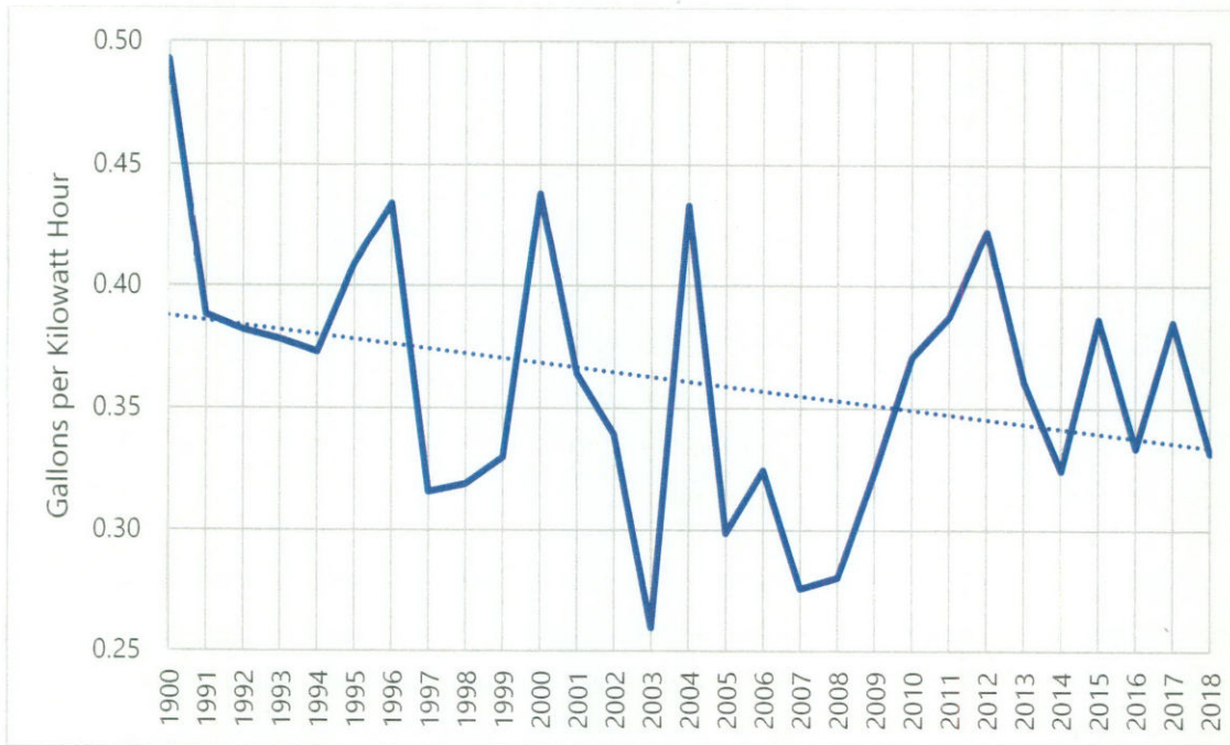
Figure 1. Electric Power Generation Water Use per Kilowatt Hour (Gallons per kWh). Prepared by Bill Hoffman using TWDB and U.S. Dept. of Energy data 7 .
