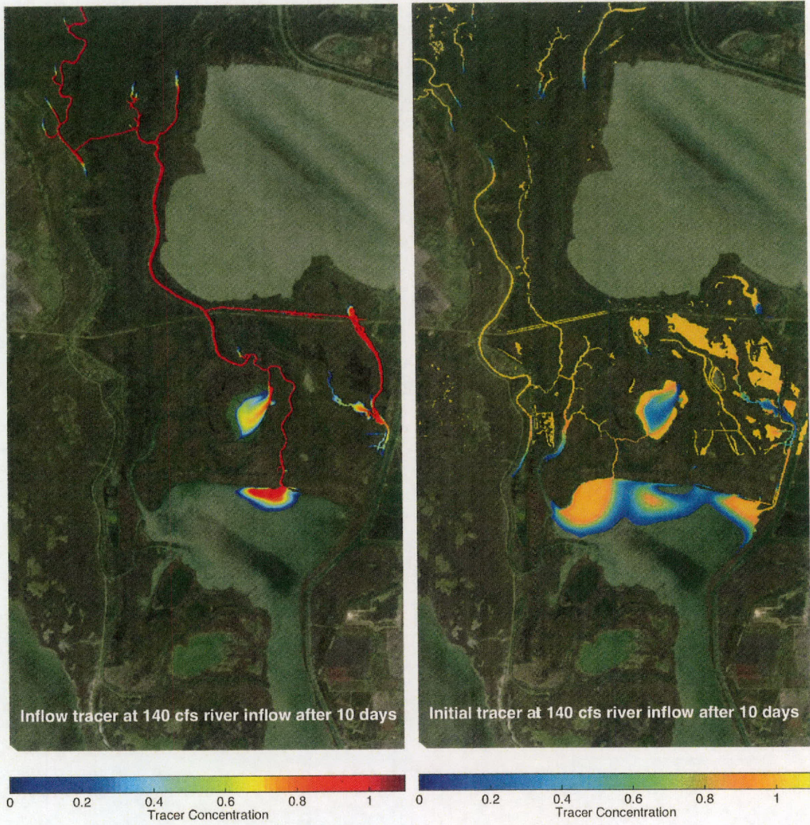
Figure D.2. Modeled tracer distributions for 140 cfs inflow case. Note that the colormaps extend beyond the [0,1] range of tracer concentrations for better contrast with the satellite image.
