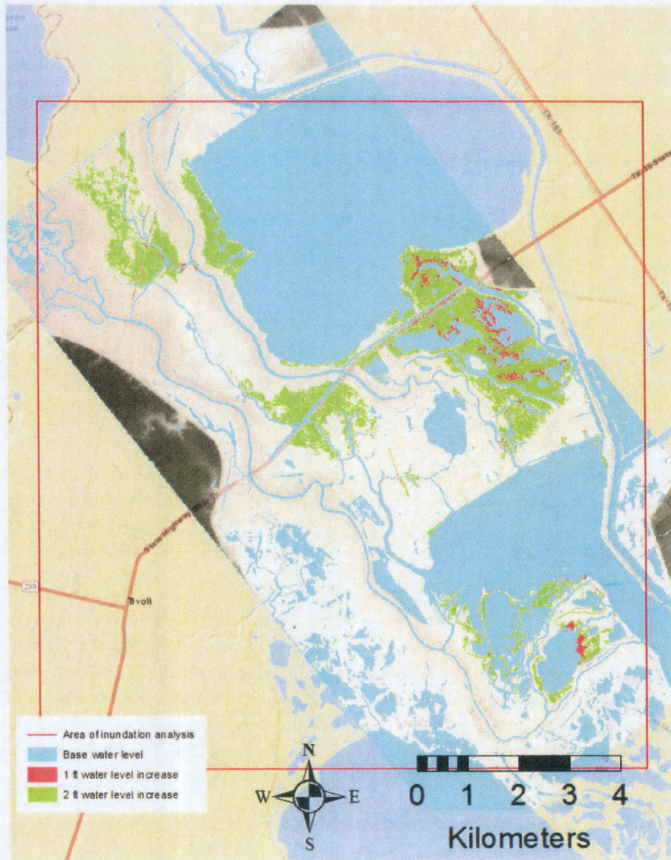
Figure 9. Inundation levels of 1-2 ft above base estimated water level
