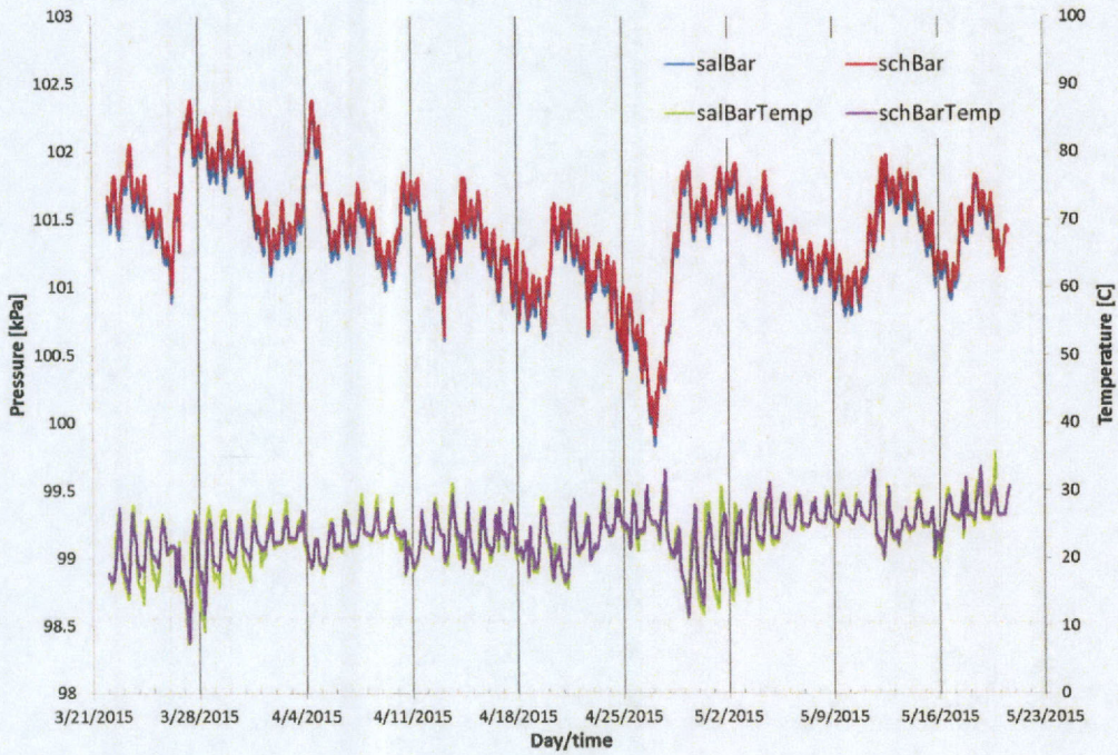
Figure C.7. Pressure for all sensors retrieved on May 23, 2015.
