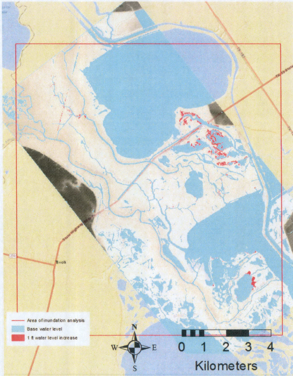
Figure B.3. Inundation resulting from a 1 ft Base water level increase
