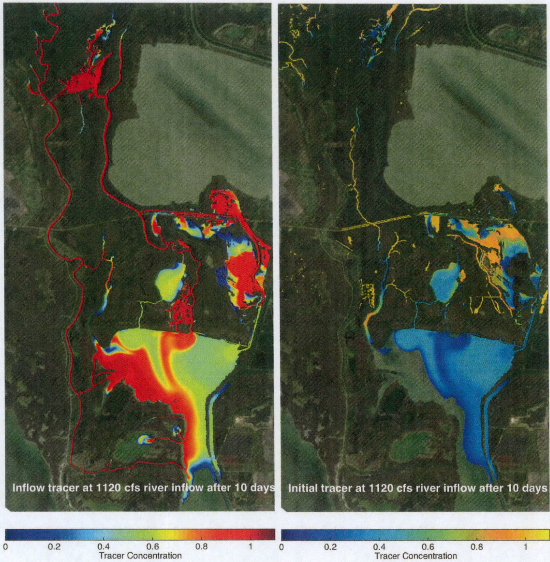
Figure D.5. Modeled tracer distributions for 1120 cfs inflow case. Note that the colormaps extend beyond the [0,1] range of tracer concentrations for better contrast with the satellite image.
