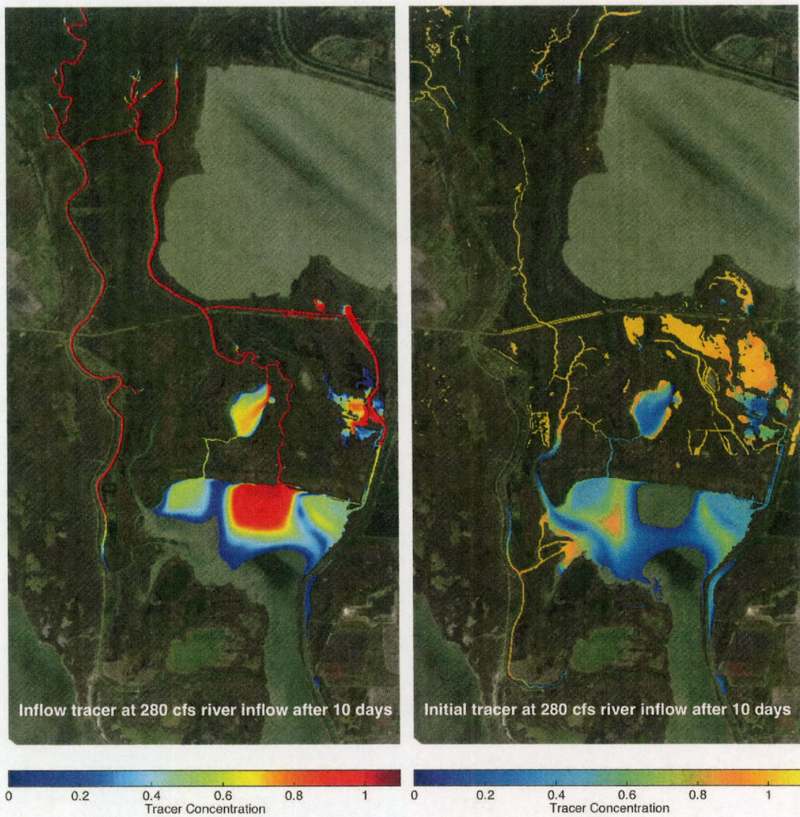
Figure 13. Inflow (left) and Initial (right) tracers after 10 days of simulation at 280 cfs. Note that the colormap for these figures extends beyond the [0,1] range of tracer concentrations for better contrast with the satellite image.
