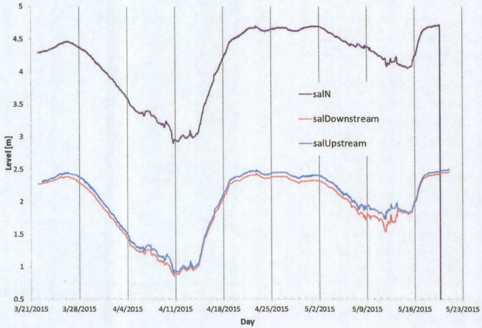
Figure 12. Comparison of water level data collected upstream of salt water barrier (salN) and USGS gages upstream (salUpstream) and downstream (salDownstream) of the barrier.
