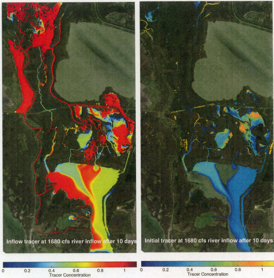
Figure D.6. Modeled tracer distributions for 1680 cfs inflow case. Note that the colormaps extend beyond the [0,1] range of tracer concentrations for better contrast with the satellite image.
