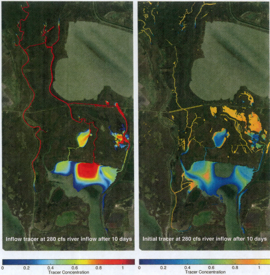
Figure D.3. Modeled tracer distributions for 280 cfs inflow case. Note that the colormaps extend beyond the [0,1] range of tracer concentrations for better contrast with the satellite image.
