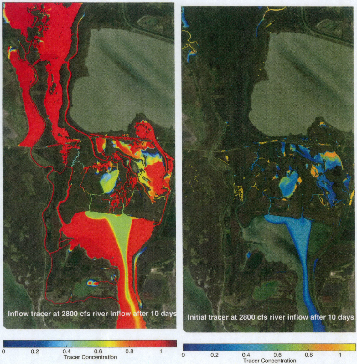
Figure D.7. Modeled tracer distributions for 2800 cfs inflow case. Note that the colormaps extend beyond the [0,1] range of tracer concentrations for better contrast with the satellite image.
