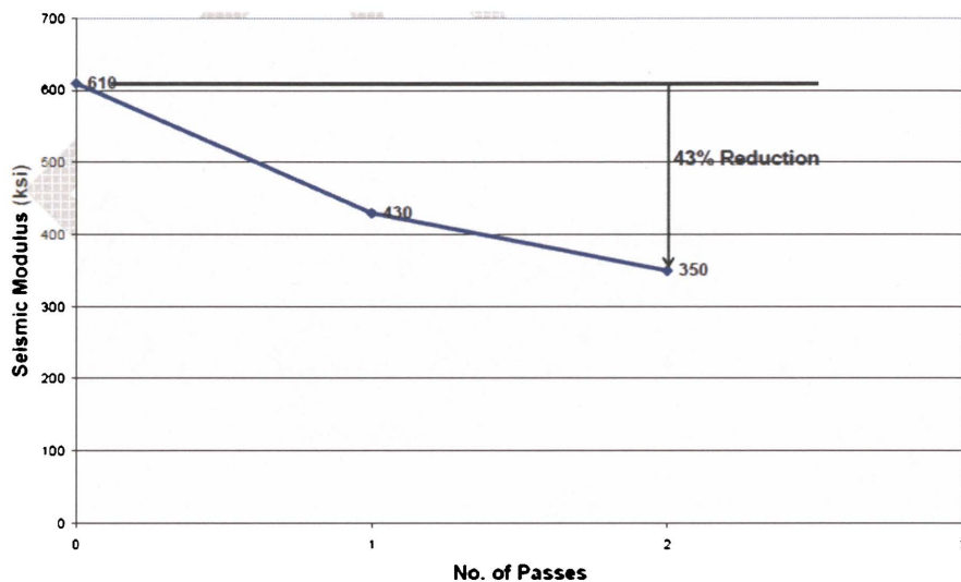
Figure 2.11: Reduction of base modulus with micro-cracking
