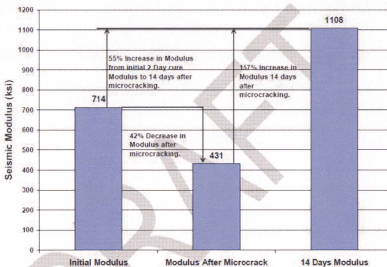
Figure 2.12: Overview of micro-cracking effectiveness
