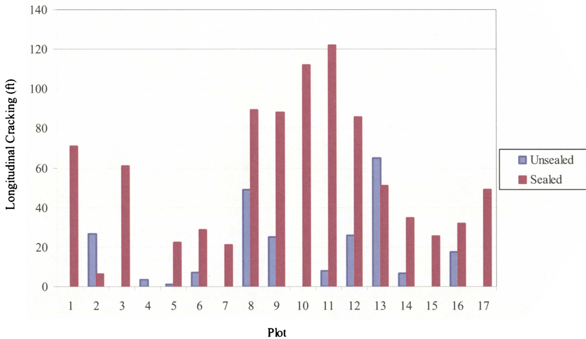
Figure 5.2: Longitudinal cracking measured along shoulder for each of the test plots (01/10)
