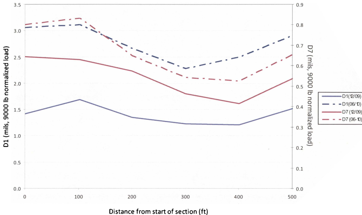
Figure 7.8: Rutting along perpetual pavement structure, R1, IH 35 (SAPERPIN)
