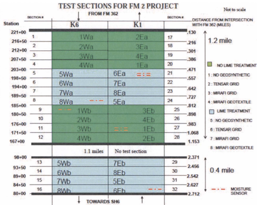
Figure 2.1: Section layout of geotextile/geogrid experiment
