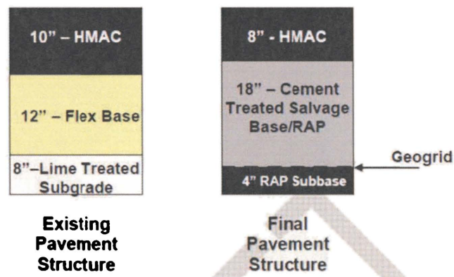
Figure 2.10: FM 734 pavement redesign
