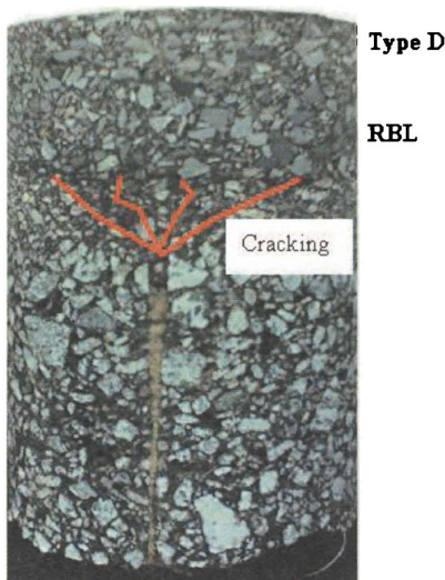
Figure 8.5: Cracking in underlying structure that did not propagate through RBL
