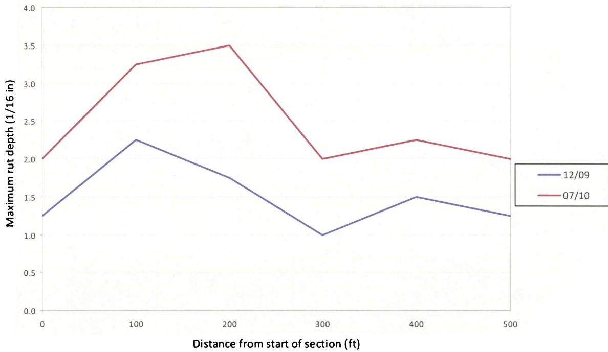
Figure 6.5: Rutting along WMA (Advera) in FM 324, Lufkin (LFWMA1AS)
