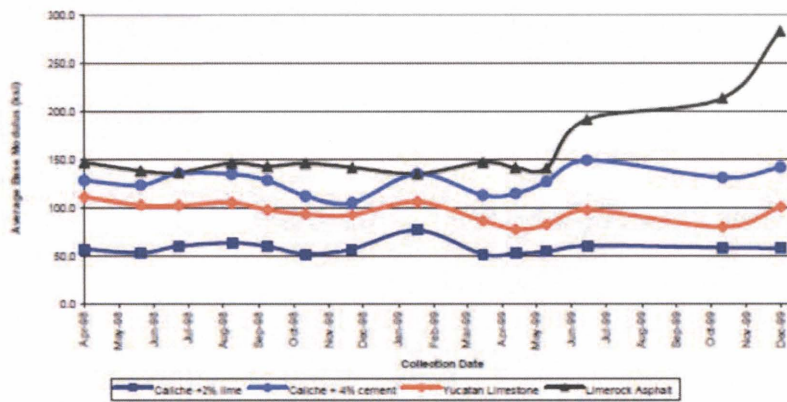
Figure 2.3: Base layer moduli on US 77 from 1998 to 1999
