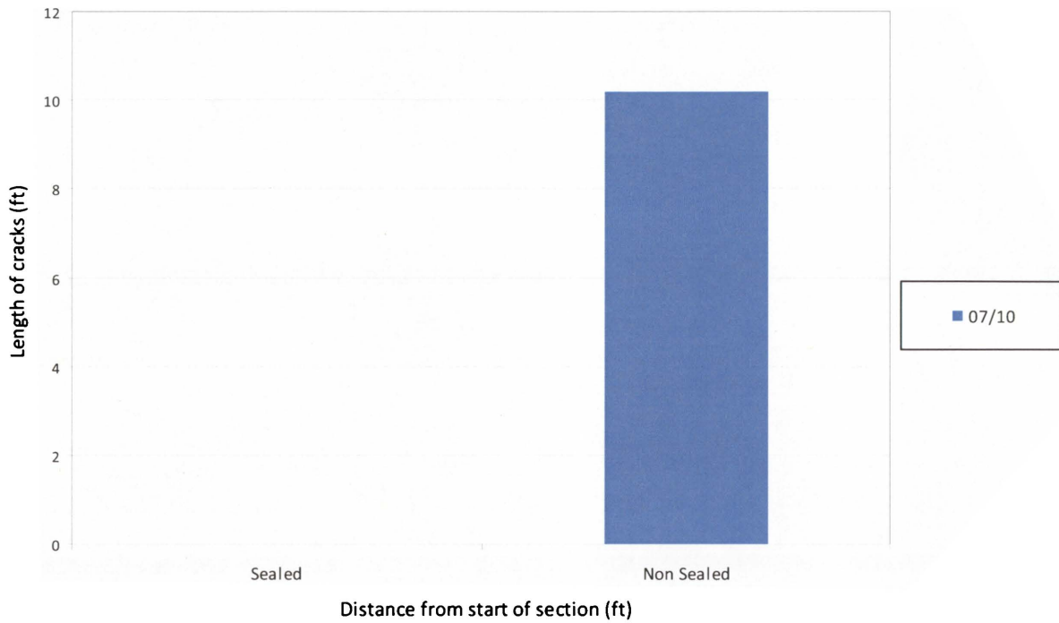
Figure 6.6: Longitudinal cracking along WMA (Advera) in FM 324, Lufkin (LFWMA1AS)
