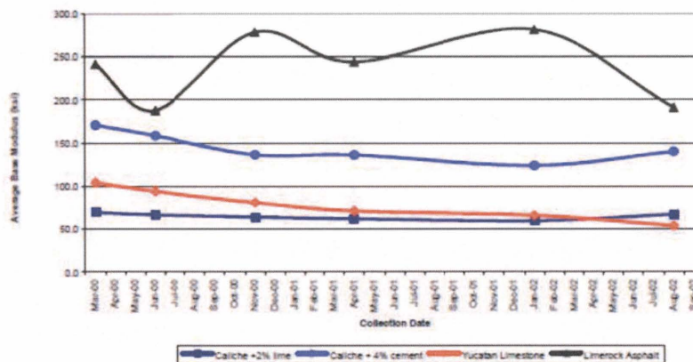
Figure 2.4: Base layer moduli on US 77 from 2000 to 2002
