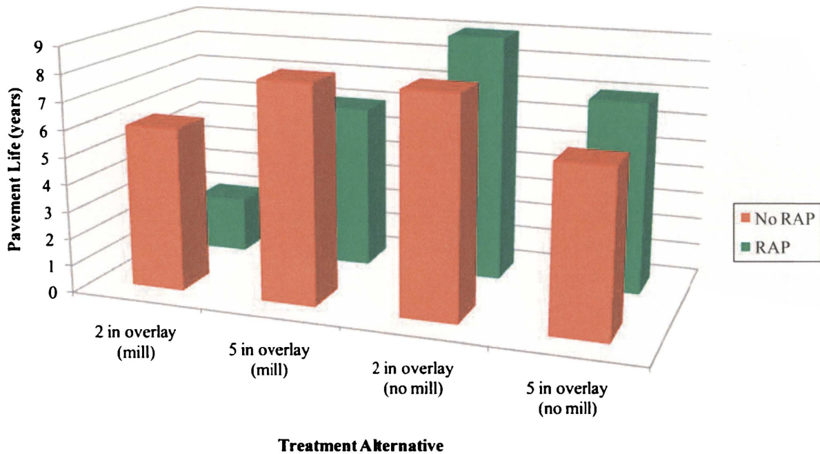
Figure 4.9: Estimated pavement life of analysis pavement sections
