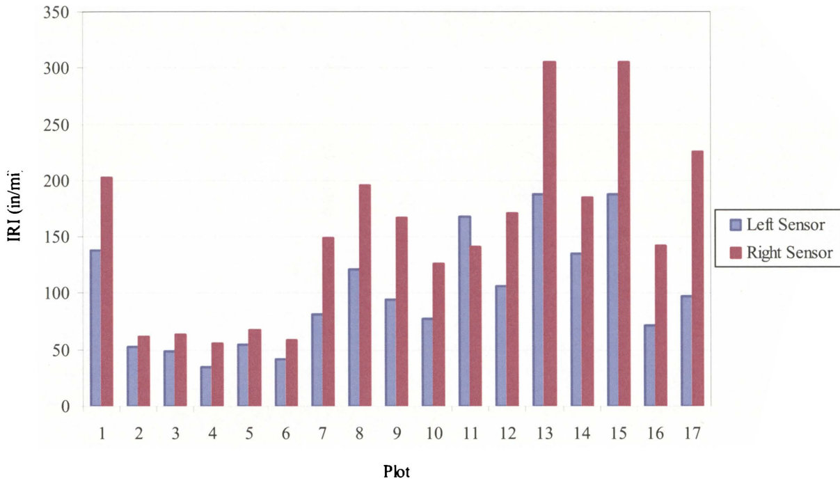
Figure 5.1: Roughness measured along shoulder for each of the test plots (01/10)
