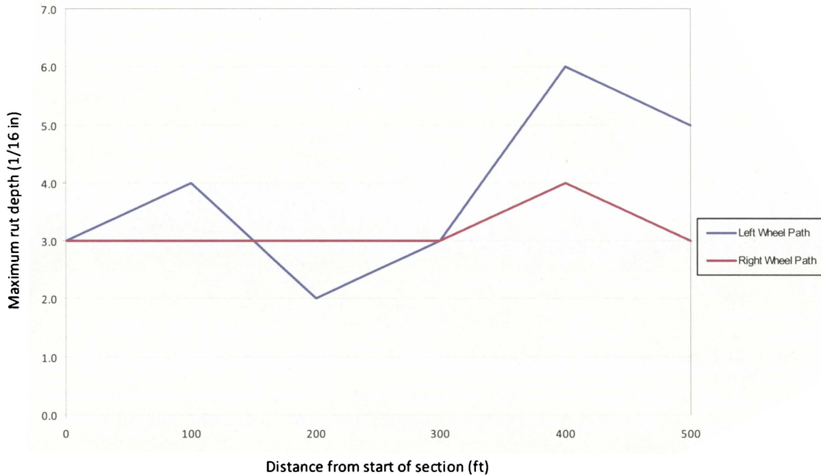
Figure 8.2: Rutting along CAM section on LP 20, Laredo (LACAM1W)
