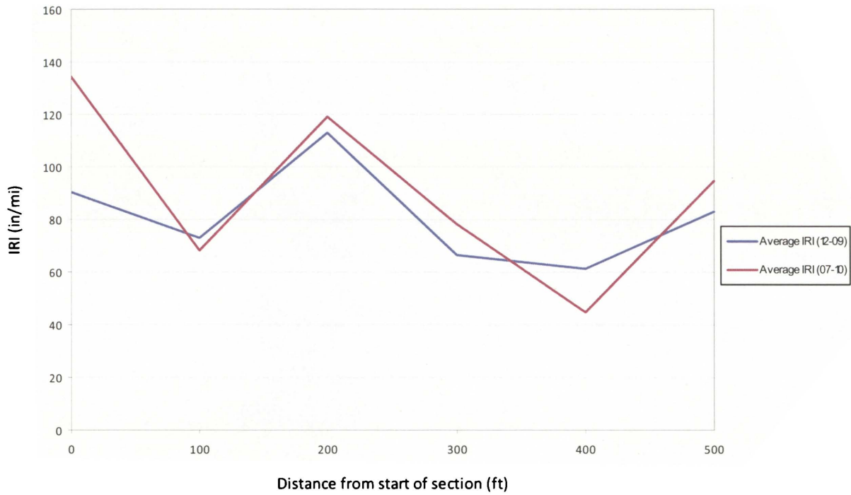
Figure 6.4: Roughness along WMA (Advera) in FM 324, Lufkin (LFWMA1AS)
