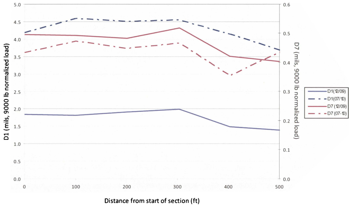
Figure 7.2: Deflections along perpetual pavement structure, R1, Fort Worth (FWPERP1E)
