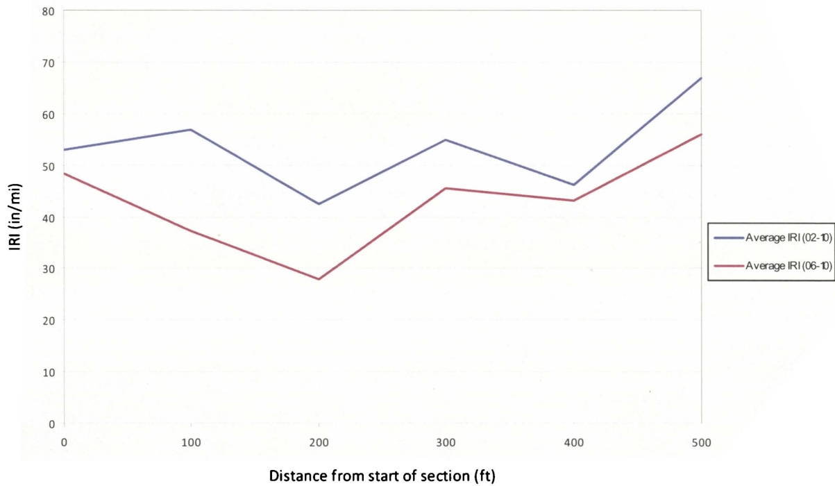
Figure 7.7: Roughness along perpetual pavement structure, R1, IH 35 (SAPERPIN)
