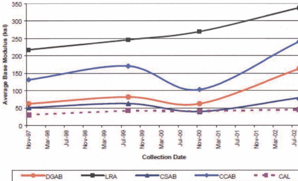
Figure 2.2: Base layer moduli for US 281 sections over time
