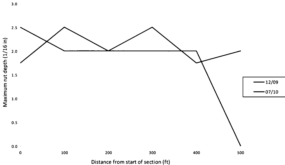
Figure 7.4: Rutting along perpetual pavement structure, R1, Fort Worth (FWPERP1E)
