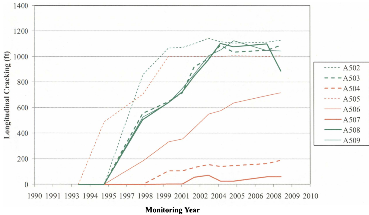
Figure 4.4: Longitudinal cracking of Texas SPS-5 pavement structures
