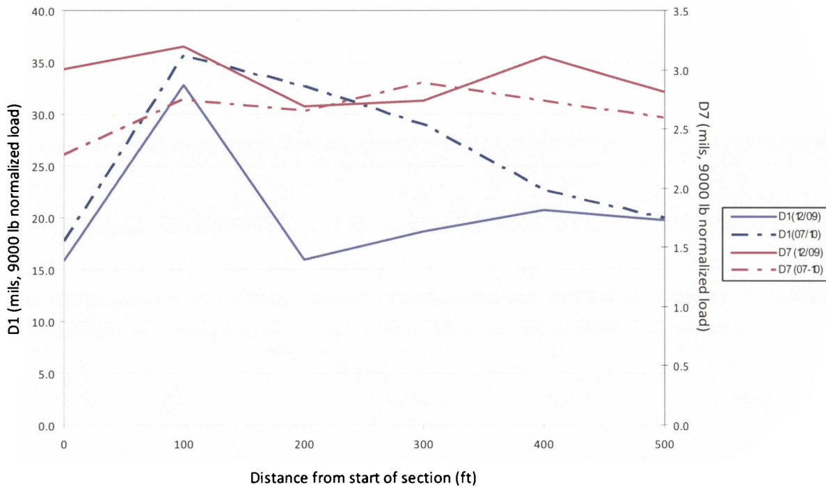
Figure 6.3: Deflections along WMA (Advera) in FM 324, Lufkin (LFWMA1AS)
