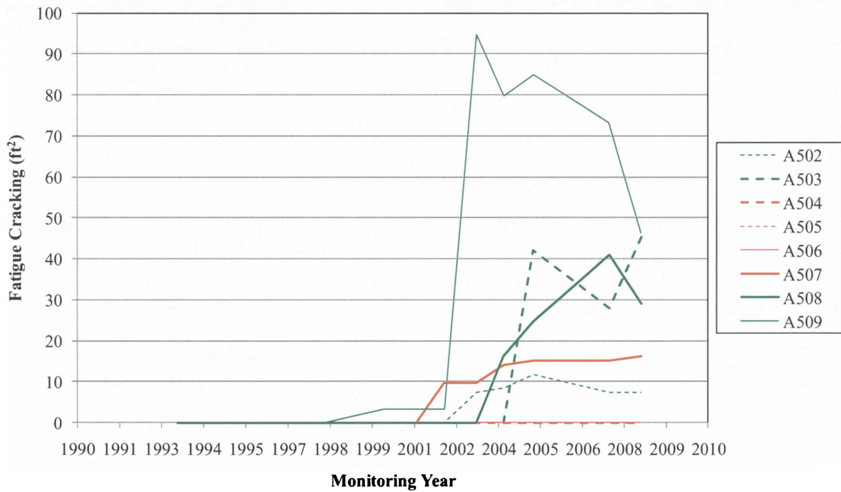
Figure 4.3: Fatigue cracking of Texas SPS-5 pavement structures
