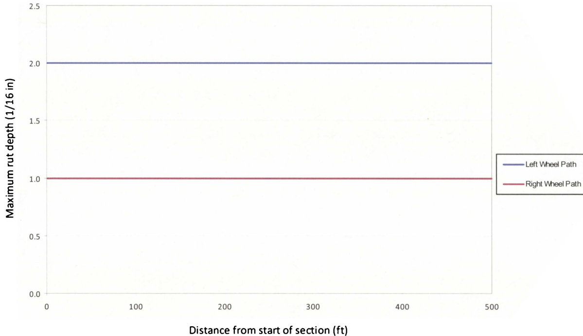
Figure 7.12: Rutting along perpetual pavement structure, R1, IH 35 (LAPERPIN)
