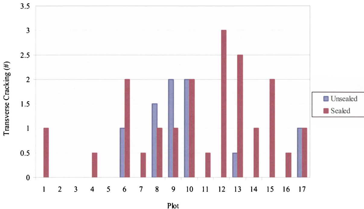
Figure 5.3: Transverse cracking measured along shoulder for each of the test plots (01/10)
