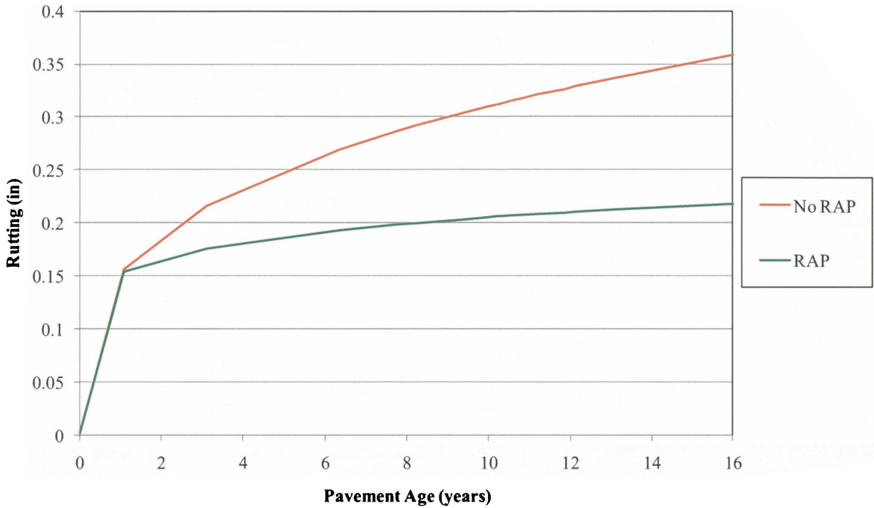
Figure 4.7: Rutting progression on a pavement with a thick overlay (with milling prior to overlaying)
