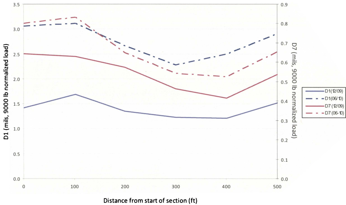
Figure 7.6: Deflections along perpetual pavement structure, R1, IH 35 (SAPERPIN)
