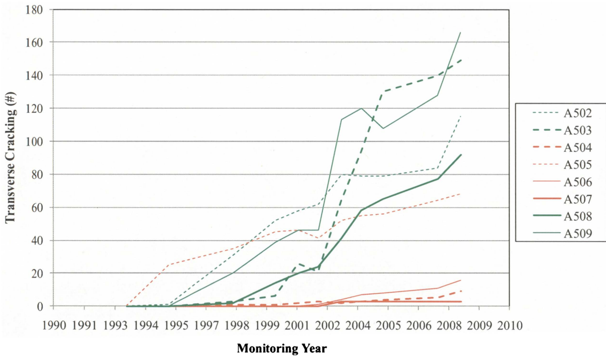
Figure 4.5: Transverse cracking of Texas SPS-5 pavement structures
