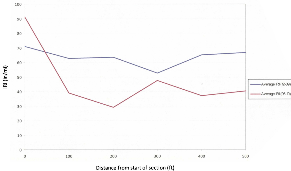
Figure 7.11: Roughness along perpetual pavement structure, R1, IH 35 (LAPERPIN)
