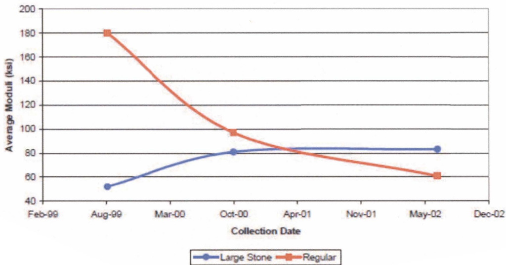
Figure 2.5: Base layer moduli on FM 1810 from 1999 to 2002.
