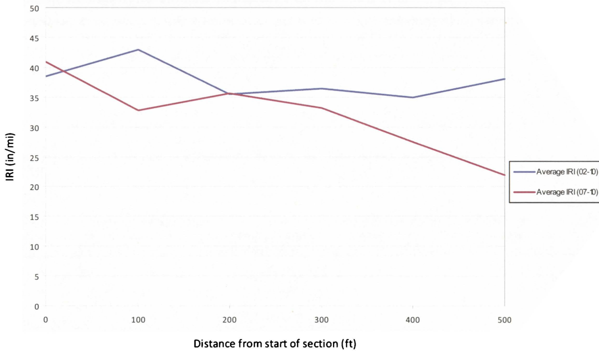
Figure 7.3: Roughness along perpetual pavement structure, R1, Fort Worth (FWPERP1E)
