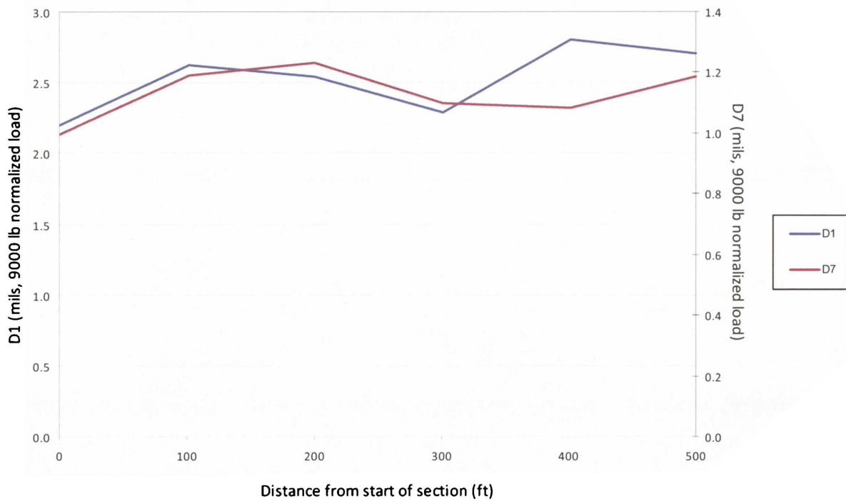
Figure 7.10: Deflections along perpetual pavement structure, R1, IH 35 (LAPERPIN)
