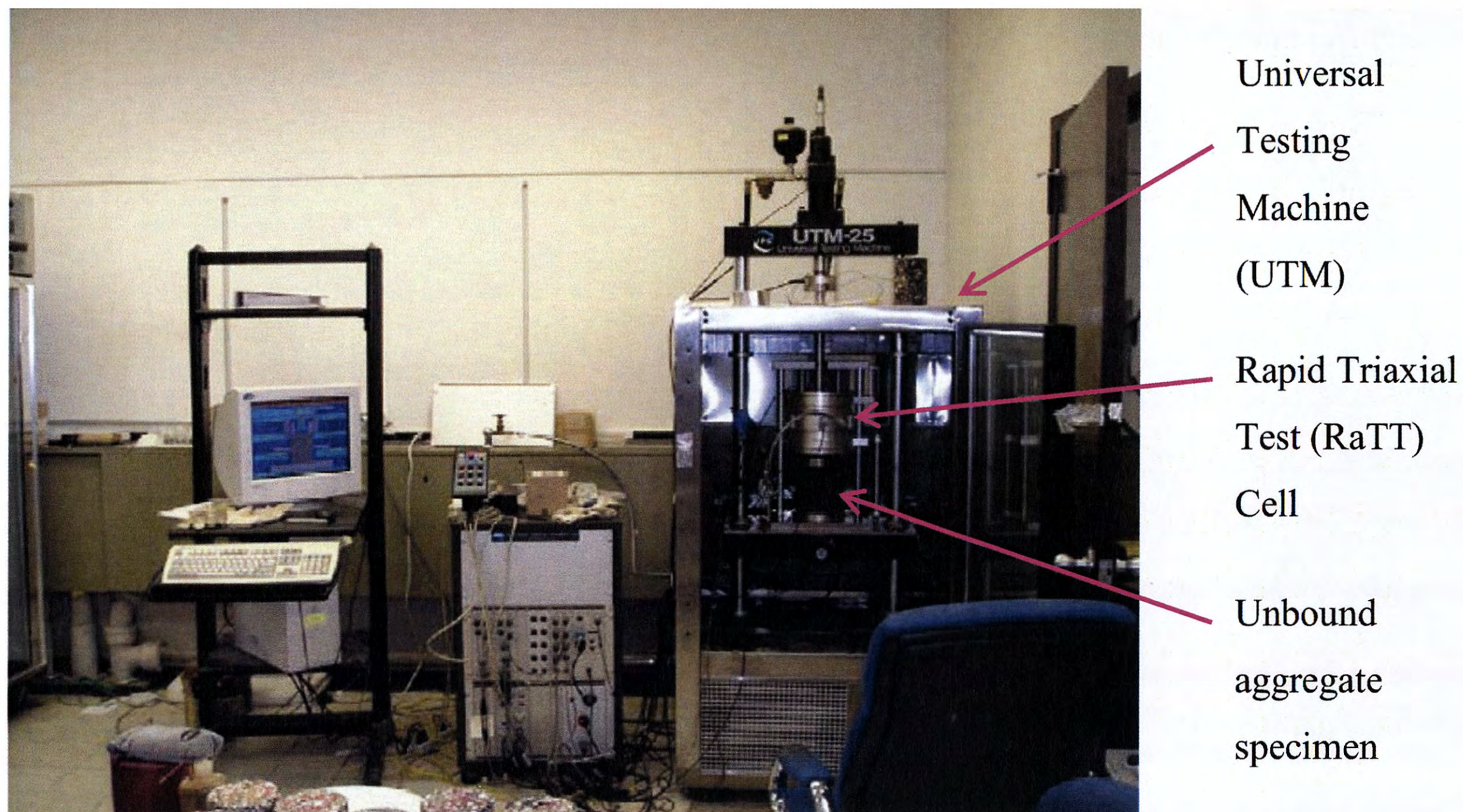
Figure B.1. Configuration of Rapid Triaxial Test.
