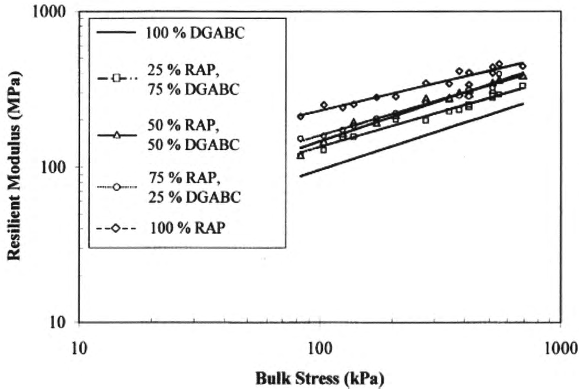
Figure 4.2. Resilient Modulus of Compacted RAP-Blended Specimens (24).
