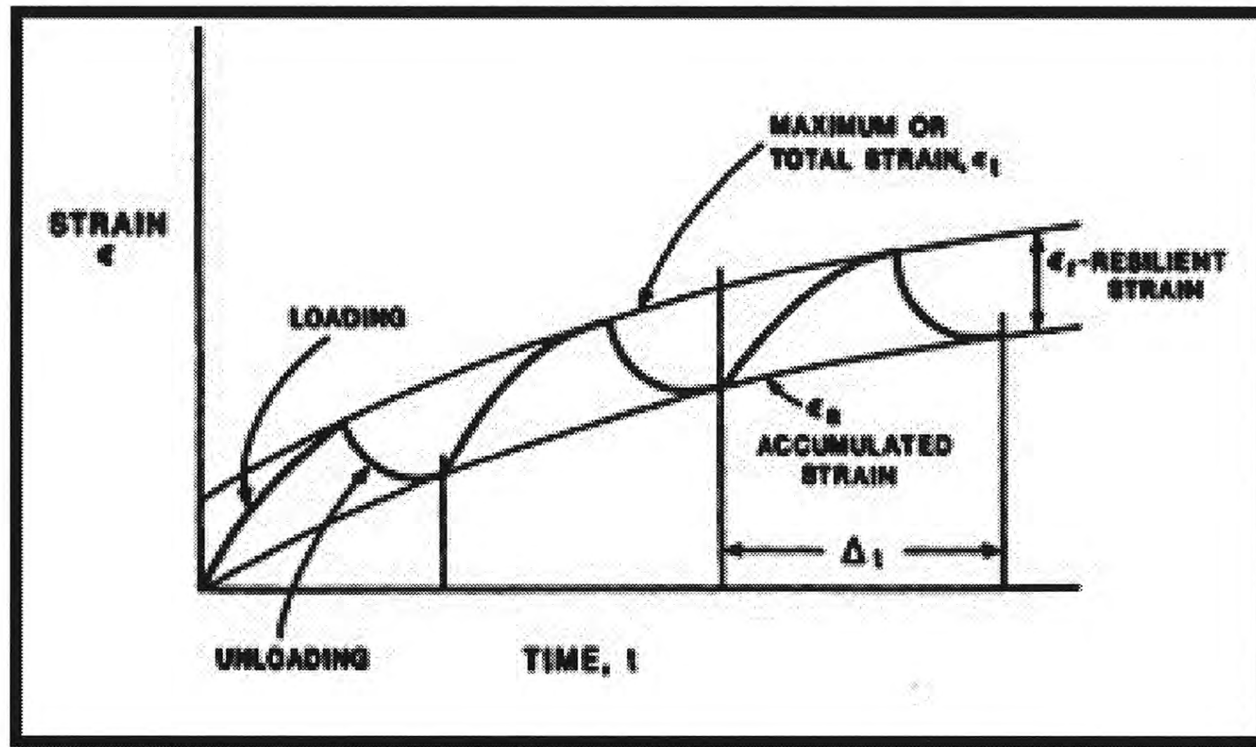
Figure 6.2. Repeated Load-Permanent Deformation Test (after Hoyt et al. 1987).
