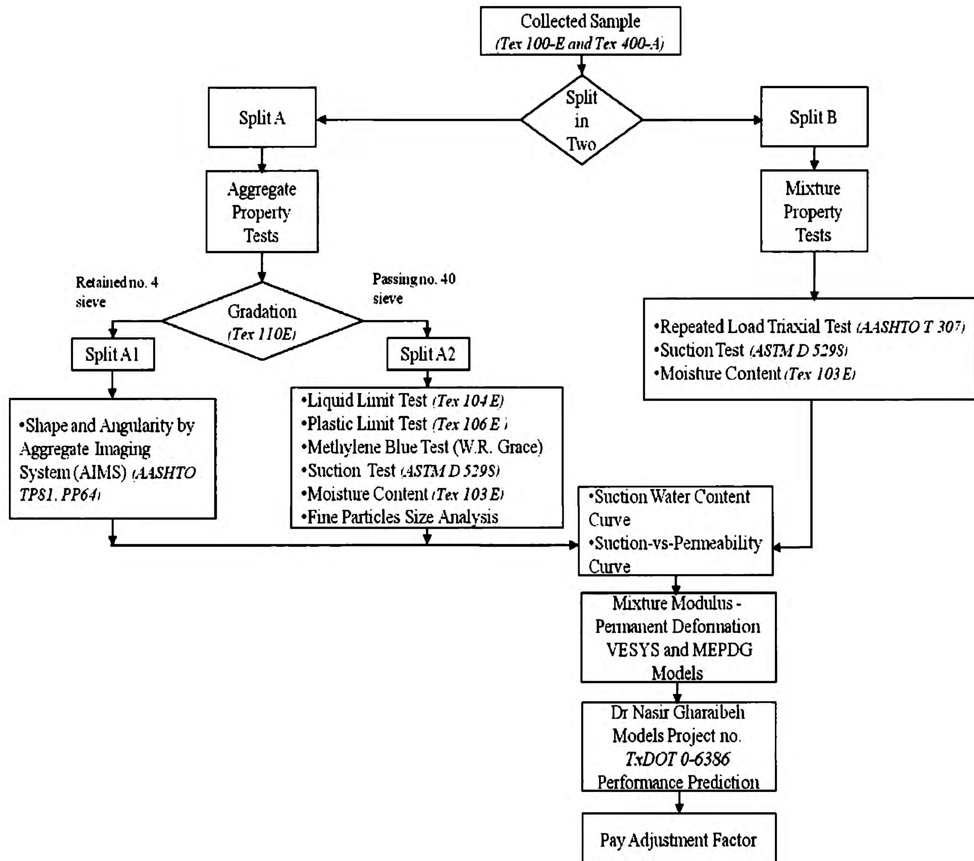
Figure 6.1. Potential Test Plan to Link Lab Tests to Performance for Flexible Base.
