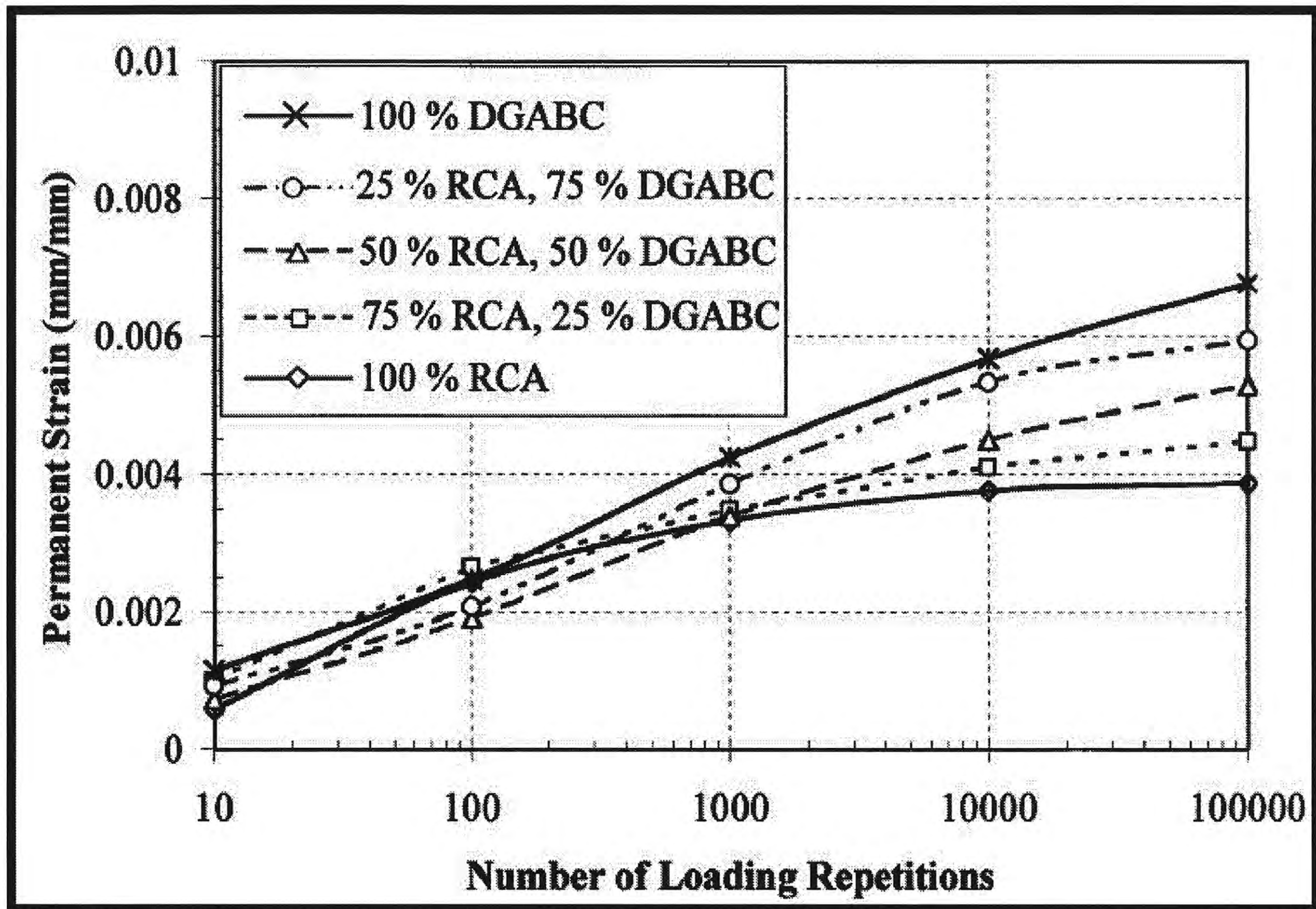
Figure 4.7. Permanent Deformation of Compacted Specimens with RCA (24).
