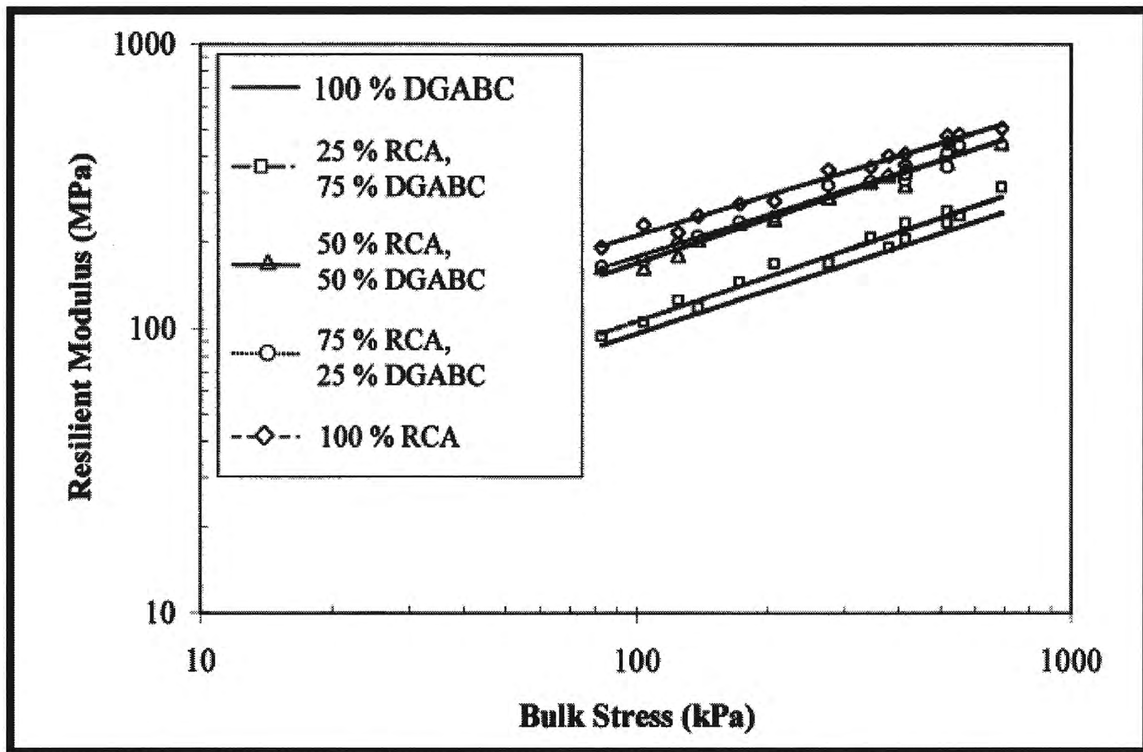
Figure 4.6. Resilient Moduli of Compacted Specimens with RCA (24).
