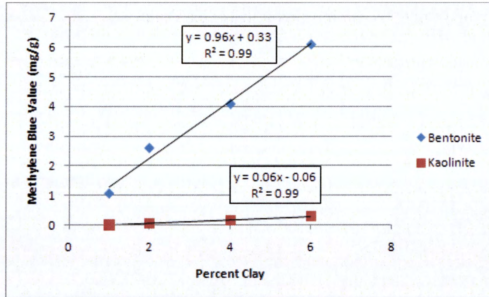
Figure 1.2. Methylene Blue Values with Bentonite and Kaolinite.
