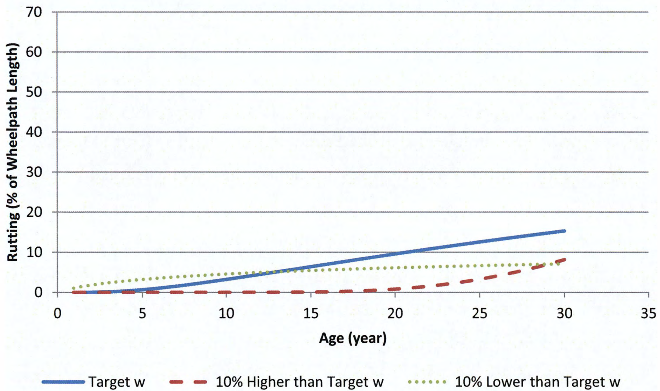
Figure B.9. Predicted Rutting Life in Climatic Zone IV.
