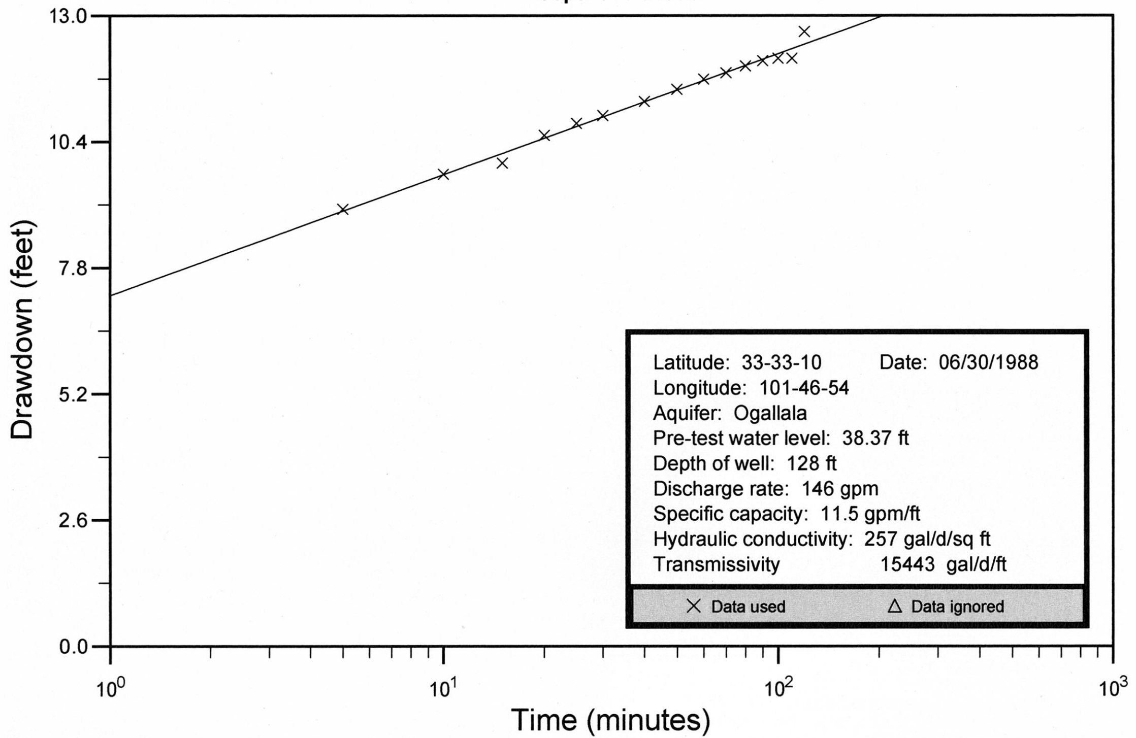
Lubbock County Well No. 23-26-614 Cooper and Jacob
