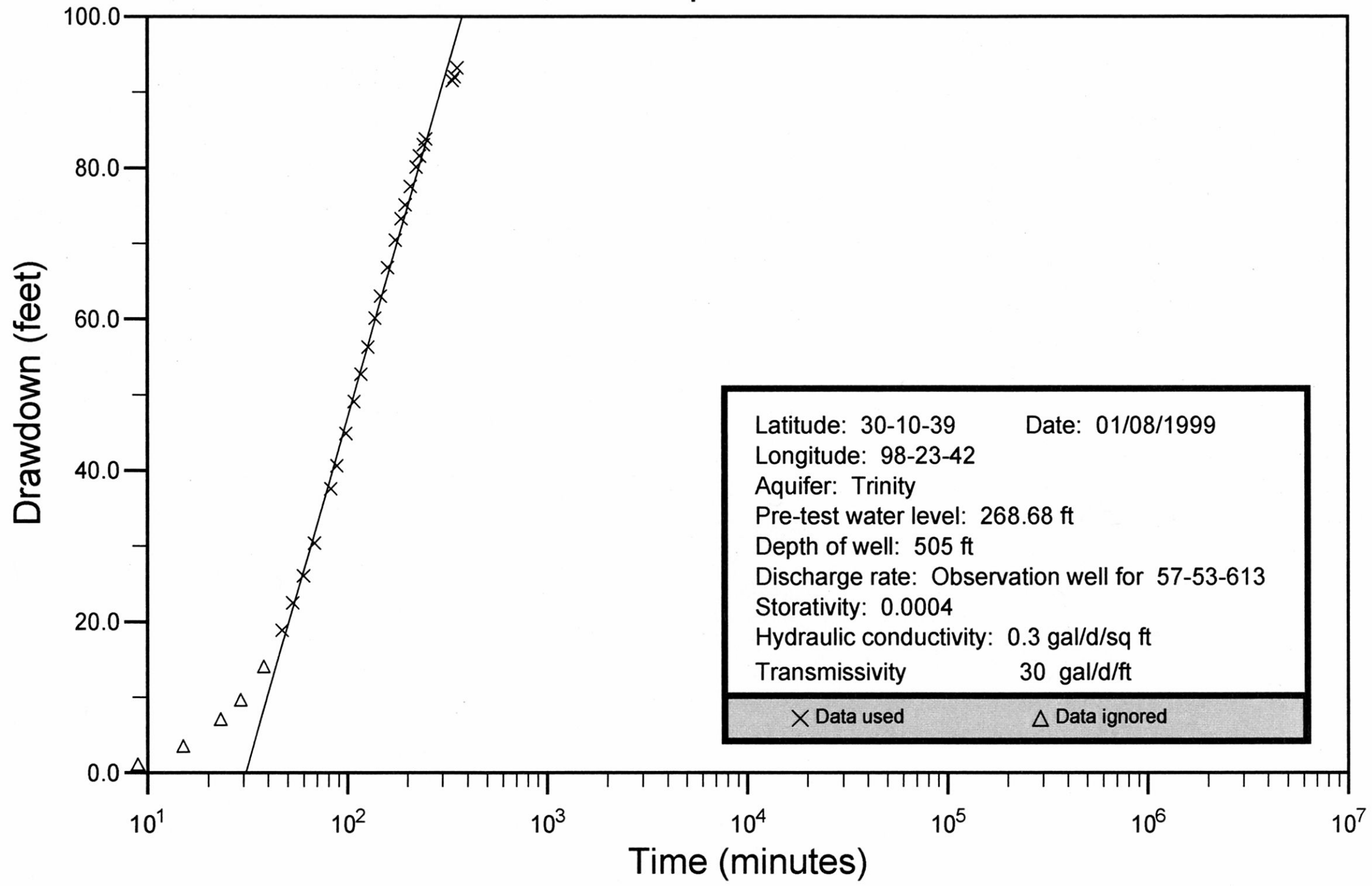
Blanco County Well No. 57-53-614 Cooper and Jacob
