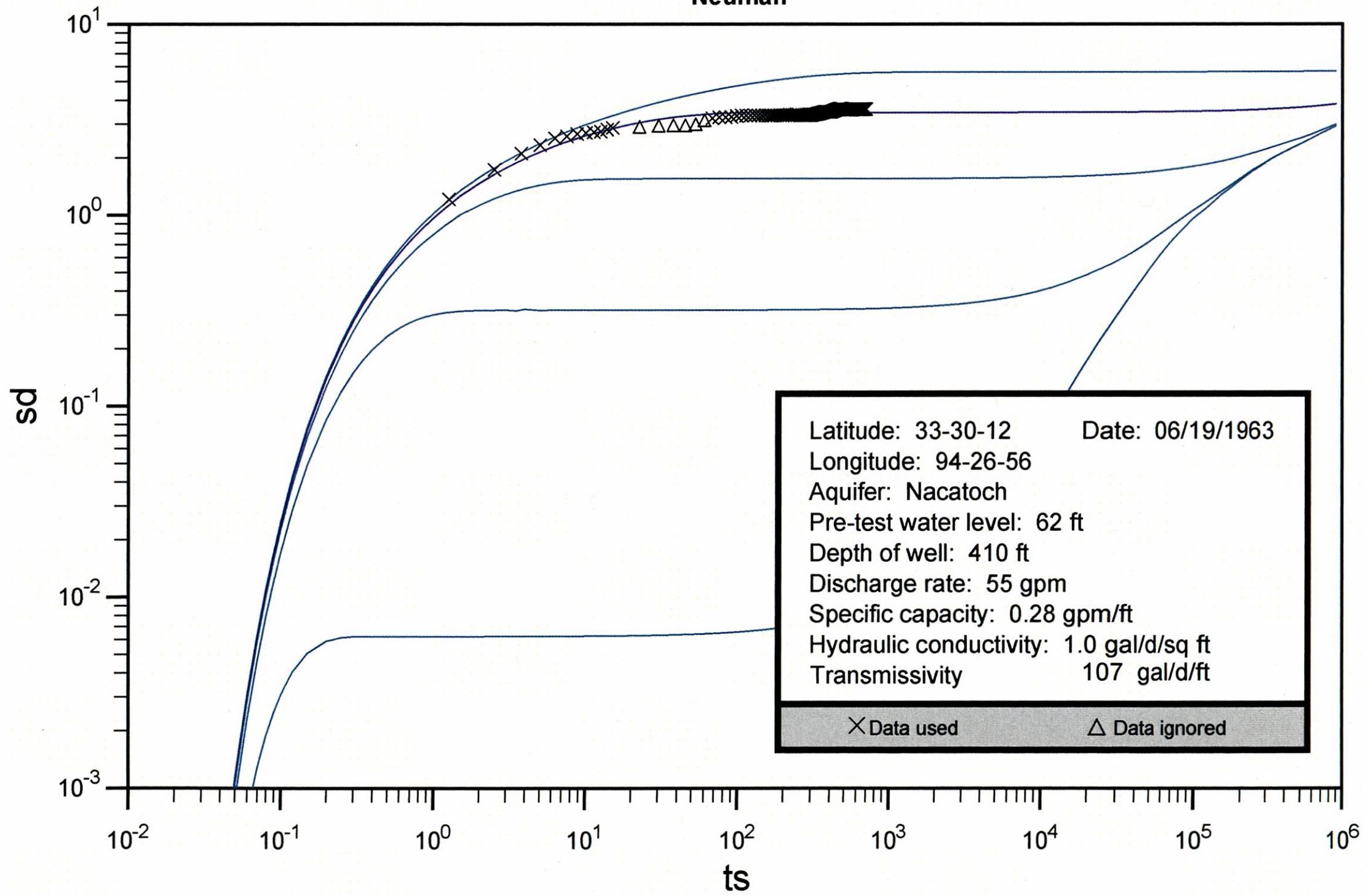
Bowie County Well No. 16-29-803 Neuman
