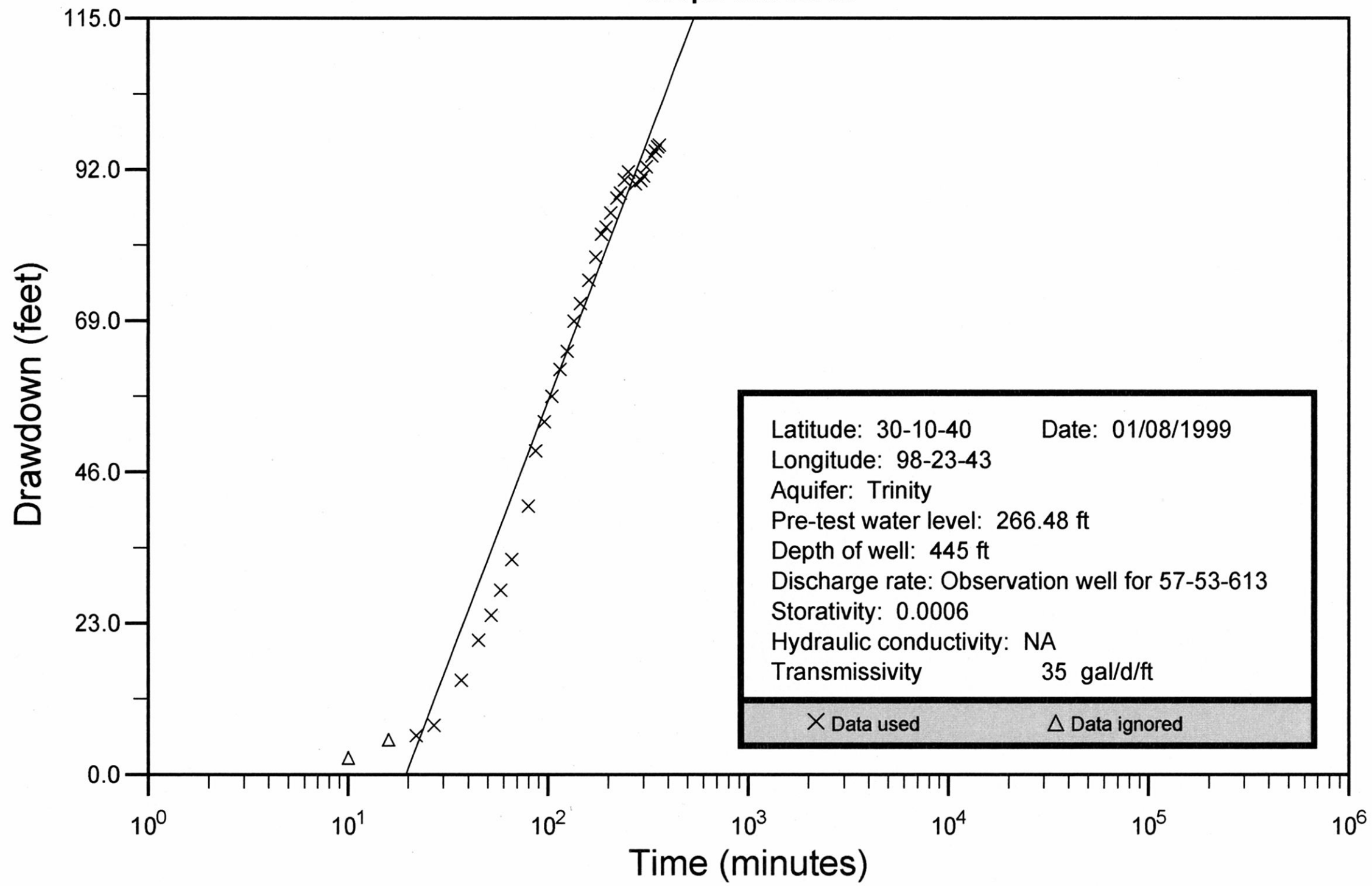
Blanco County Well No. 57-53-616 Cooper and Jacob
