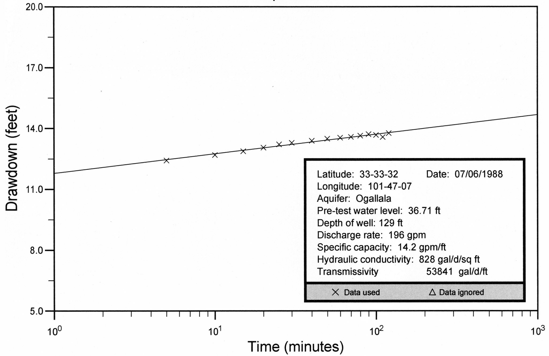
Lubbock County Well No. 23-26-613 Cooper and Jacob
