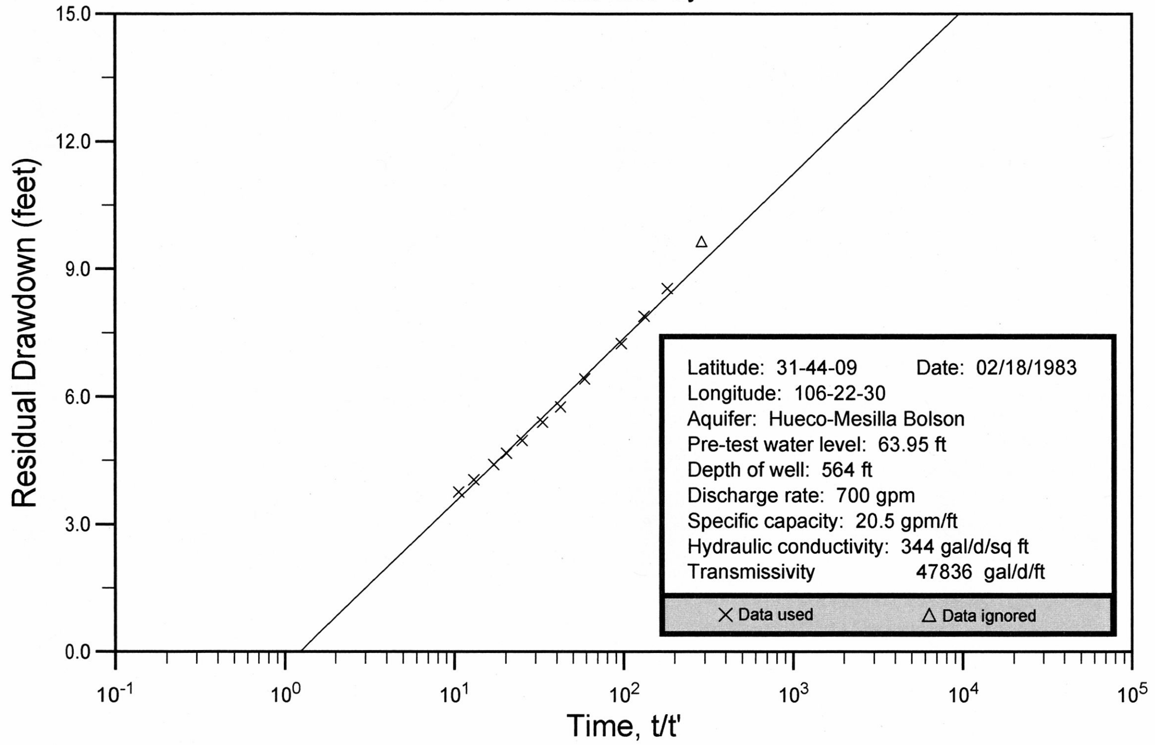
El Paso County Well No. 49-22-133 Theis Recovery
