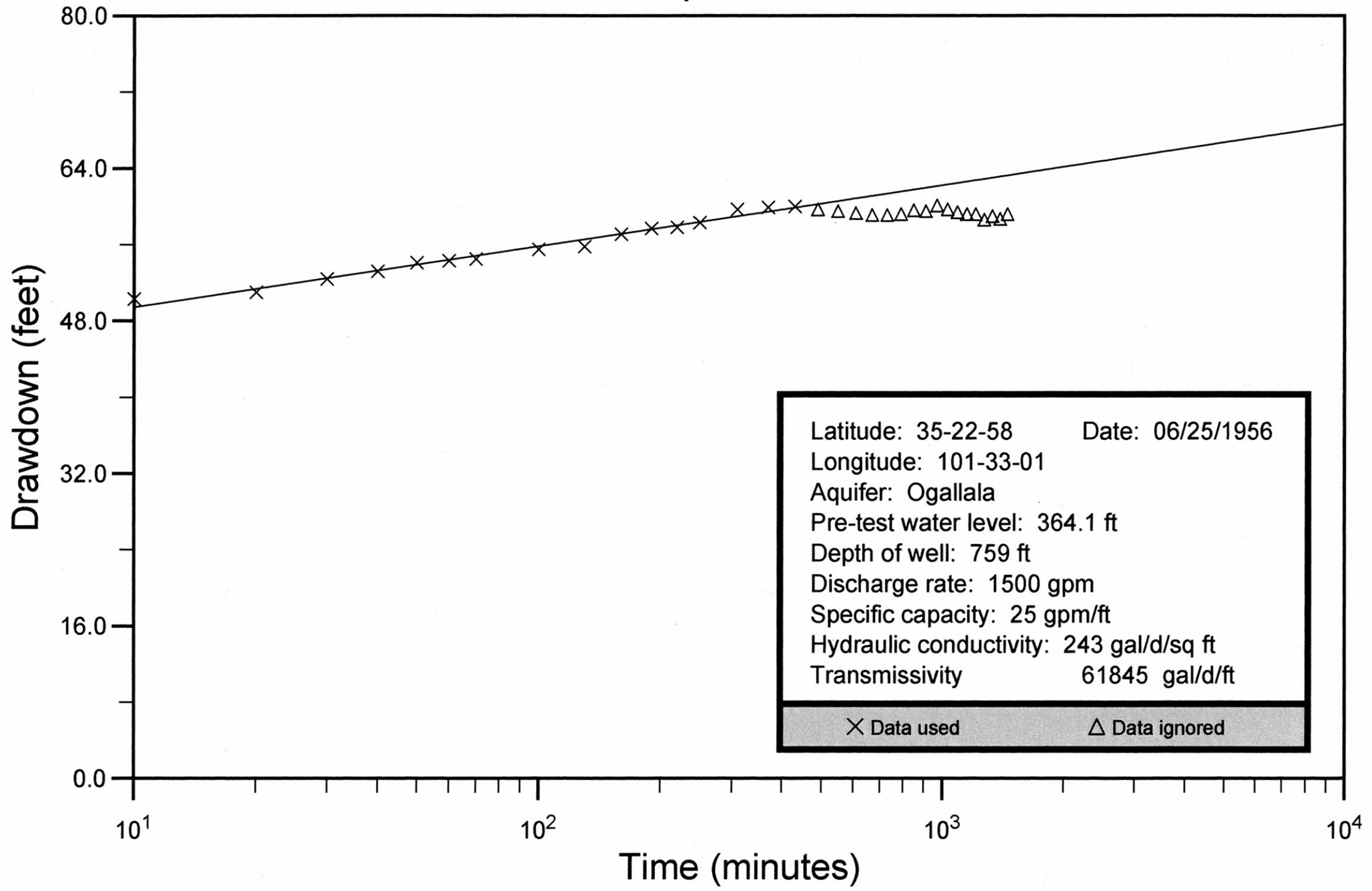
Carson County Well No. 06-36-808 Cooper and Jacob
