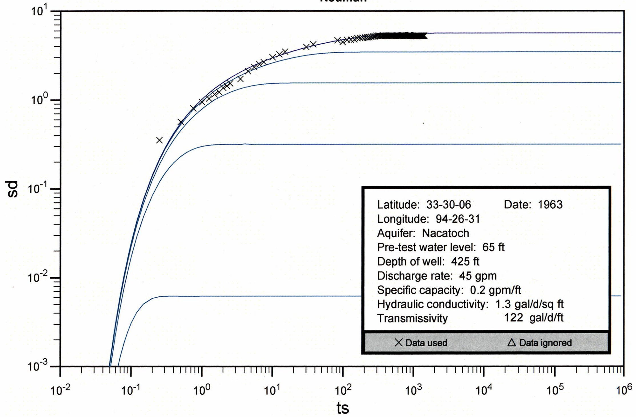
Bowie County Well No. 16-29-801 Neuman
