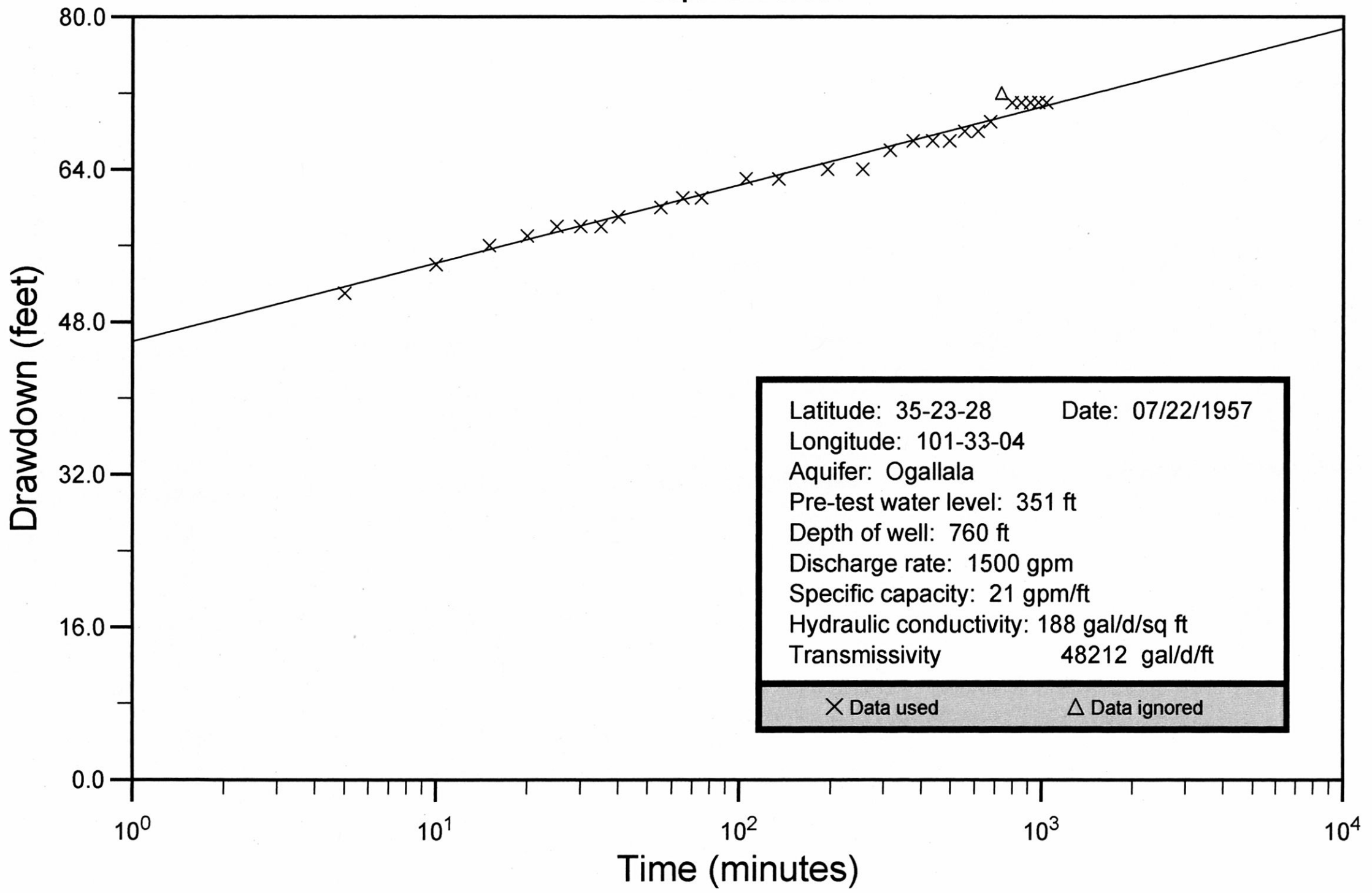
Carson County Well No. 06-36-809 Cooper and Jacob
