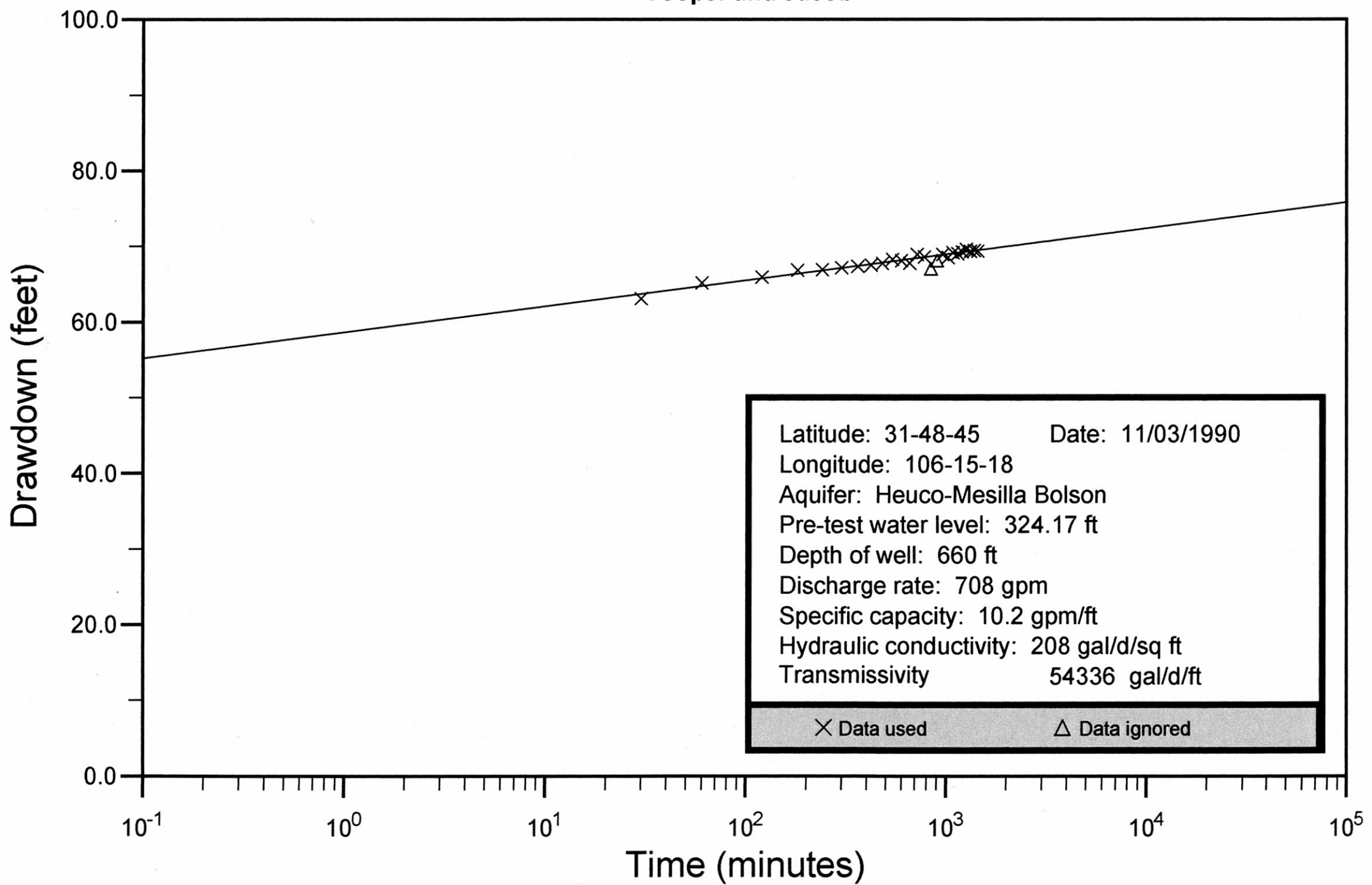
El Paso County Well No. 49-14-615 Cooper and Jacob
