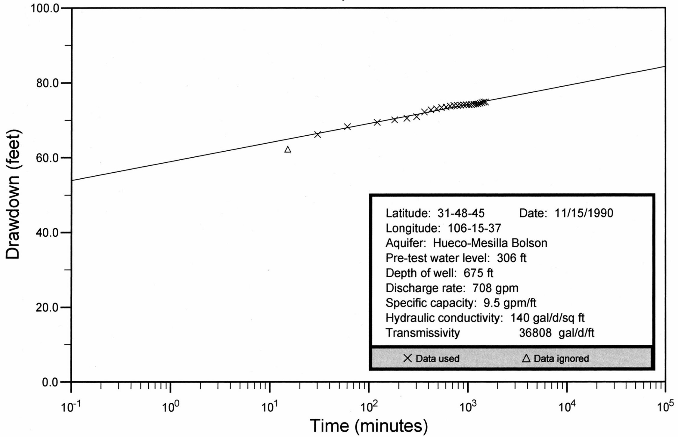
El Paso County Well No. 49-14-614 Cooper and Jacob
