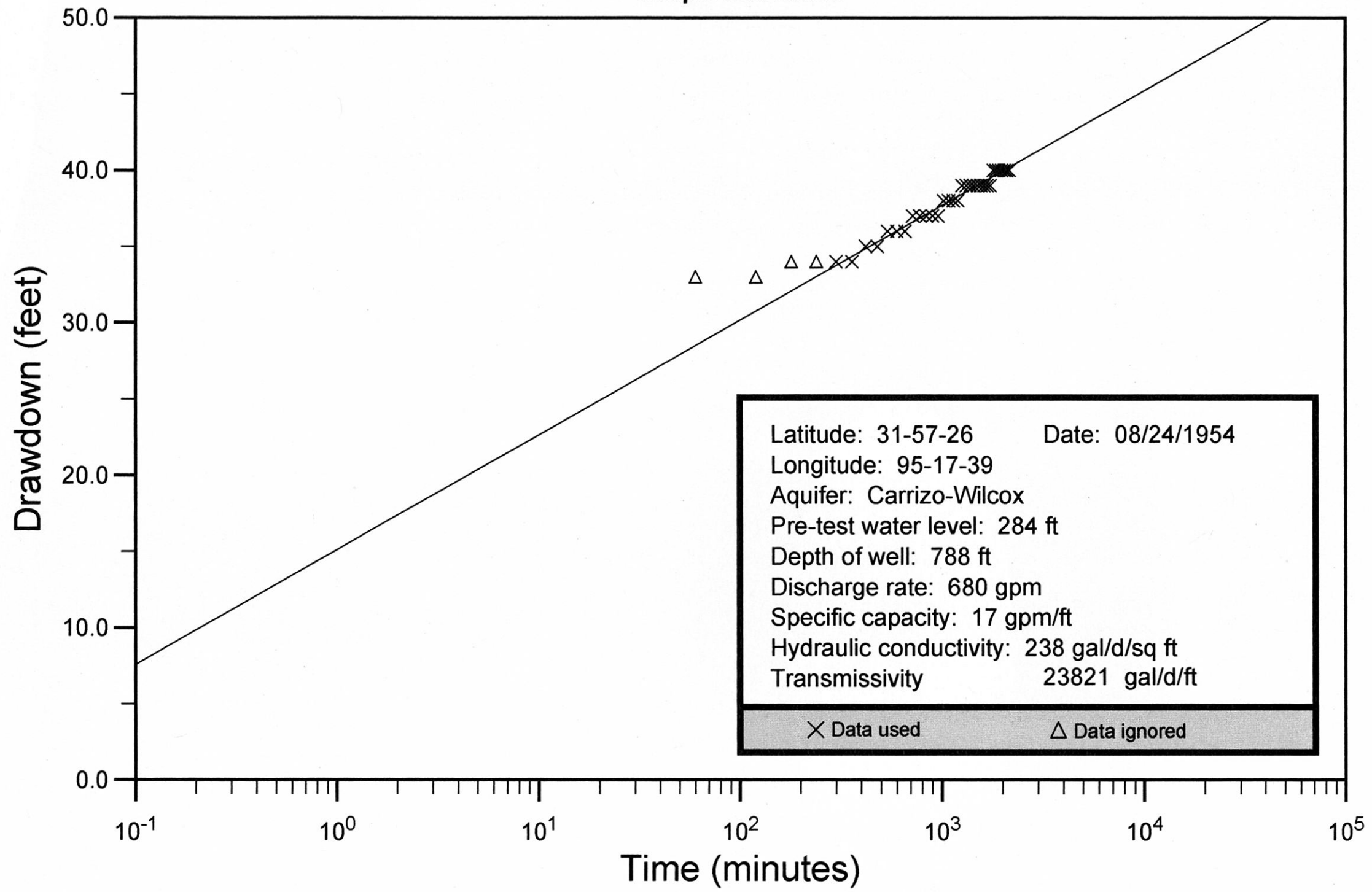
Cherokee County Well No. 38-06-501 Cooper and Jacob
