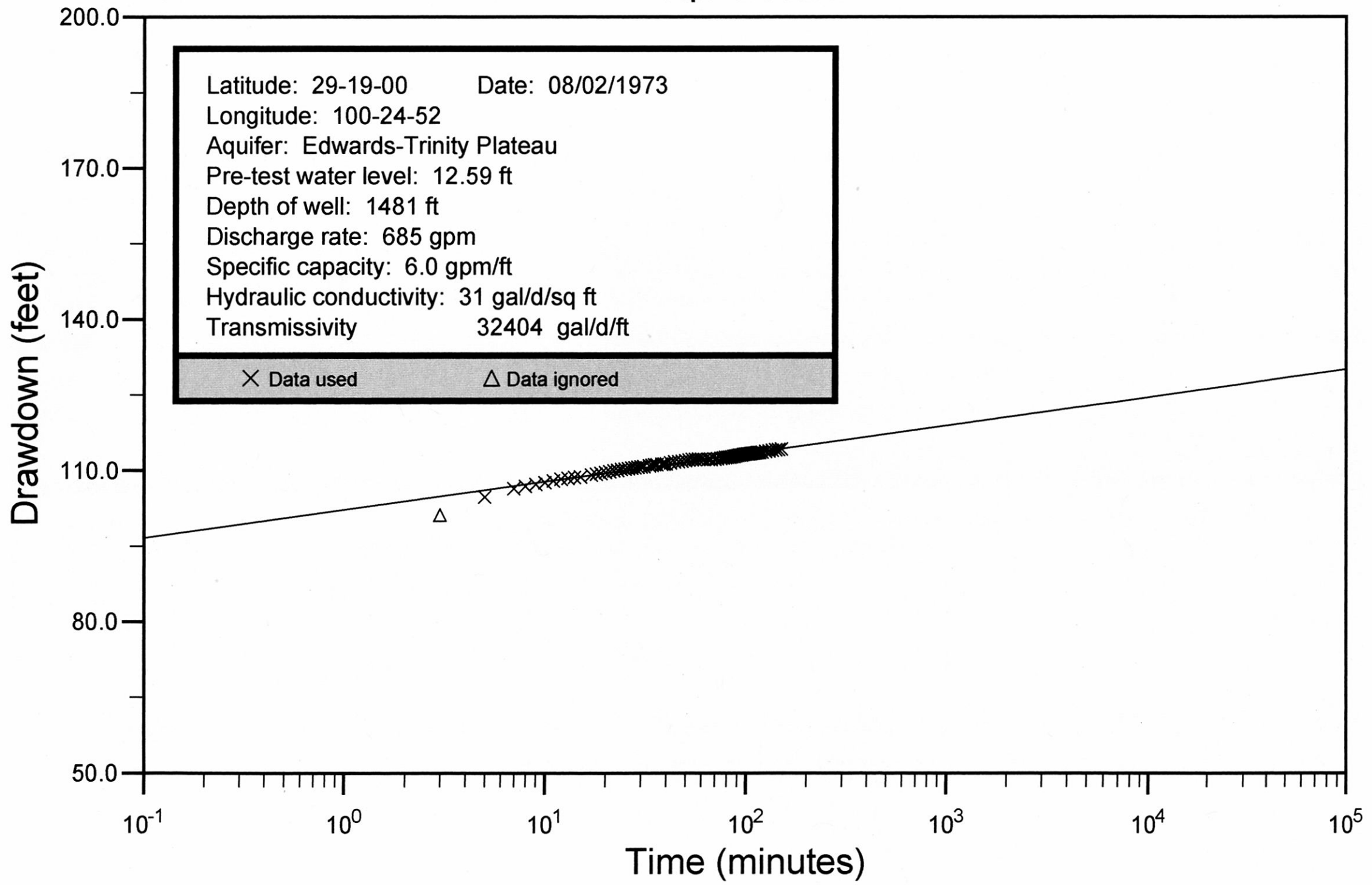
Kinney County Well No. 70-45-601 Cooper and Jacob
