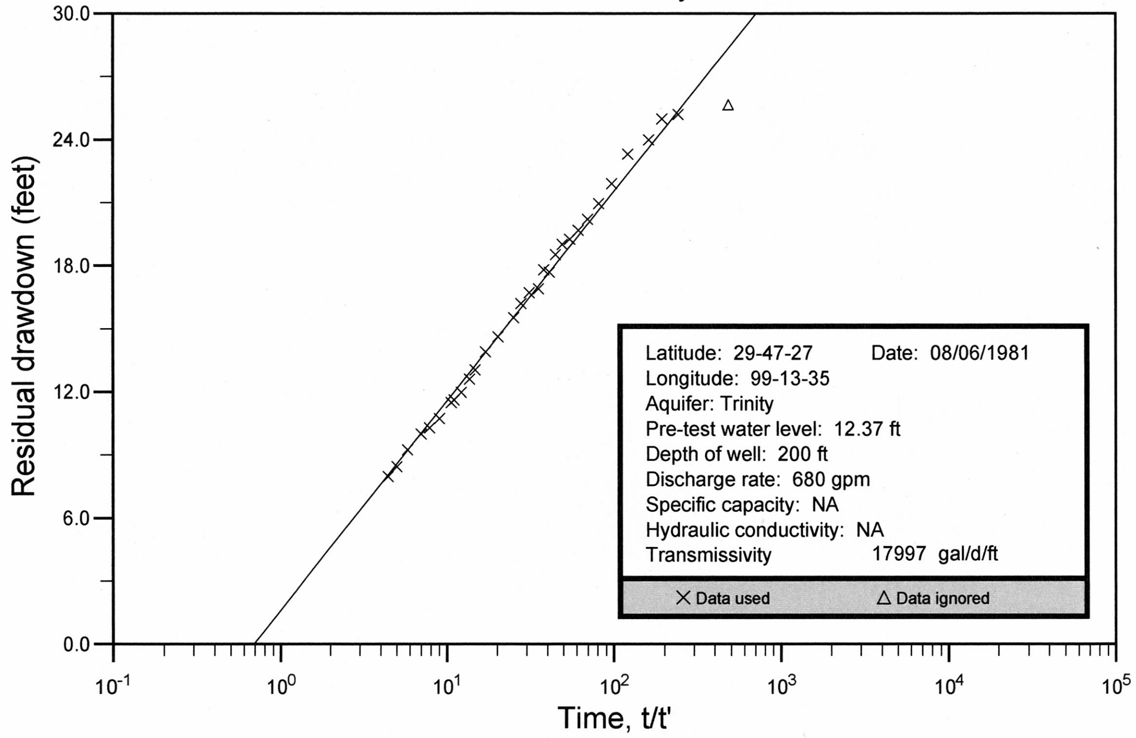
Bandera County Well No. 69-15-701 Theis Recovery
