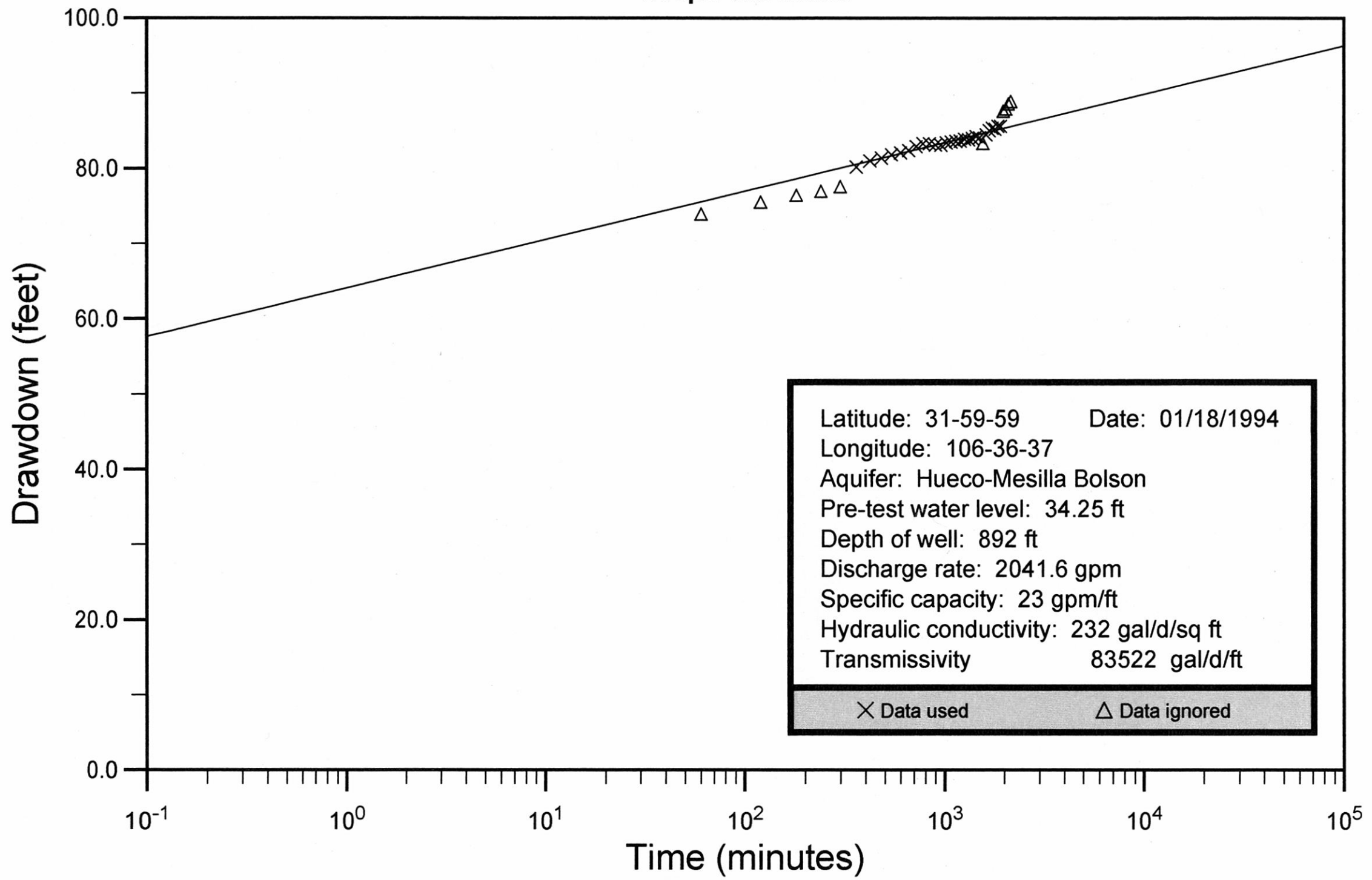
El Paso County Well No. 49-04-184 Cooper and Jacob
