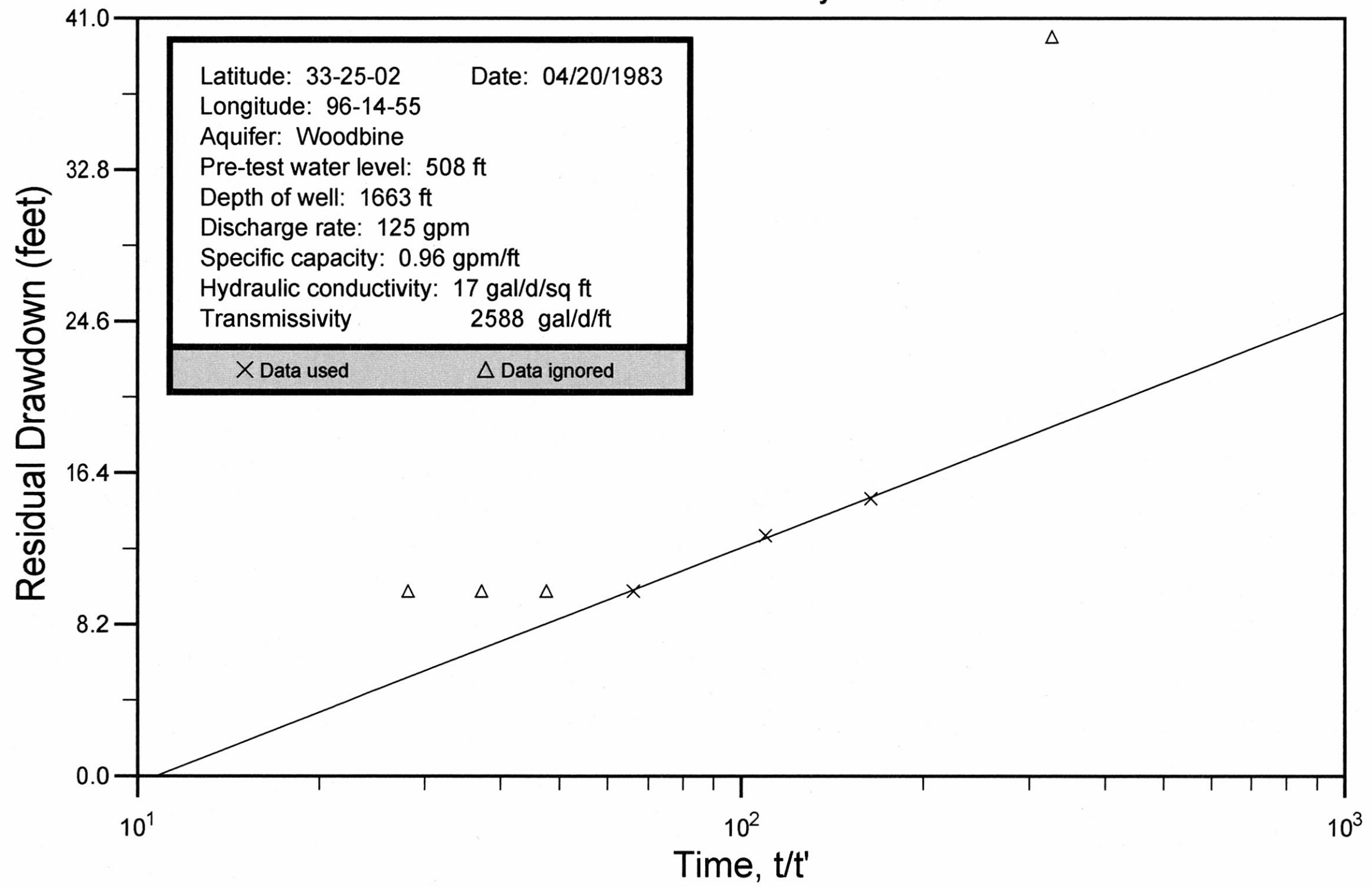
Fannin County Well No. 18-39-402 Theis Recovery
