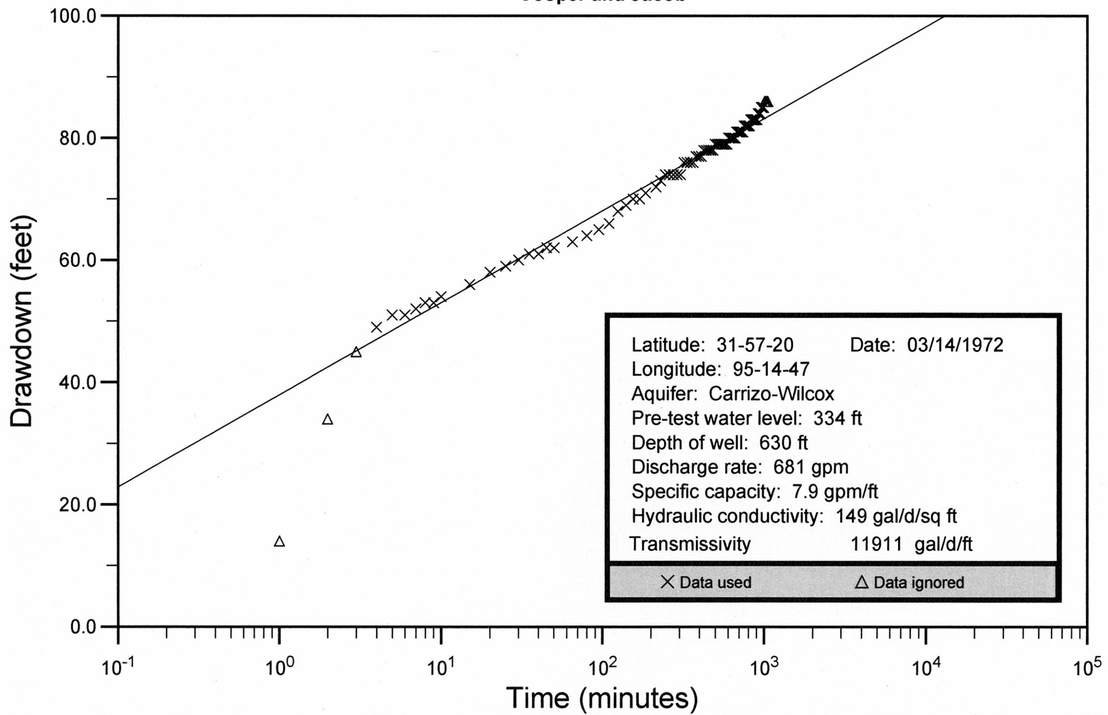
Cherokee County Well No. 38-07-408 Cooper and Jacob
