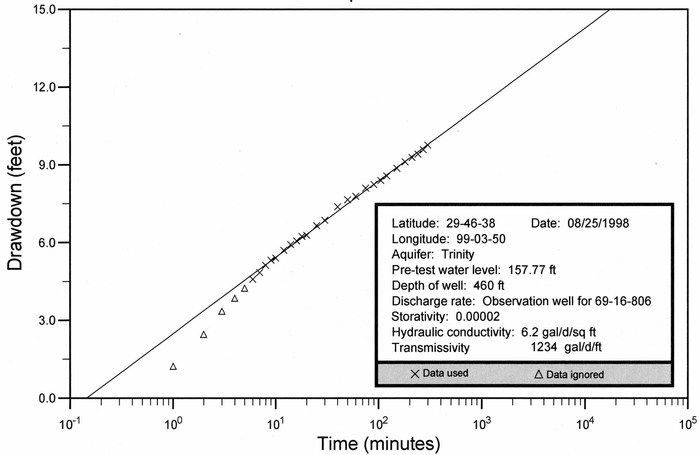
Bandera County Well No. 69-16-805 Cooper and Jacob
