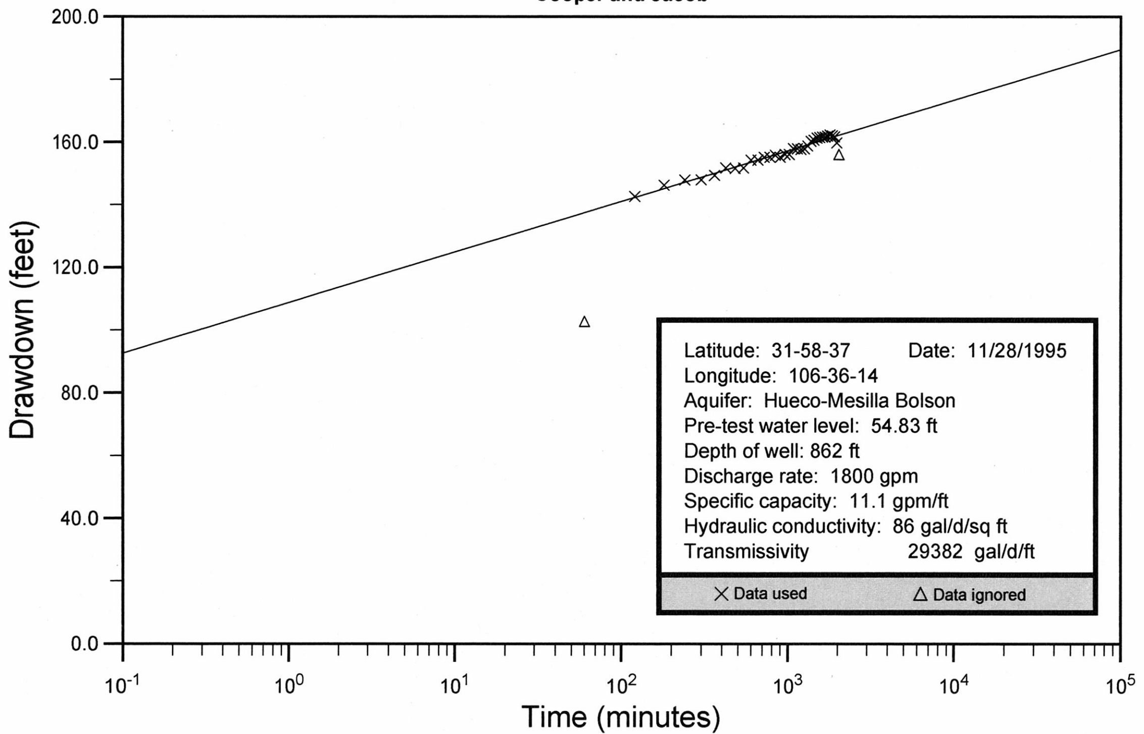
El Paso County Well No. 49-04-185 Cooper and Jacob
