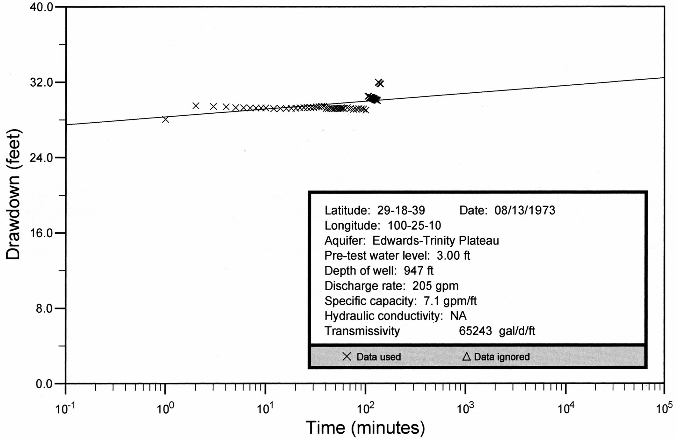
Kinney County Well No. 70-45-503 Cooper and Jacob
