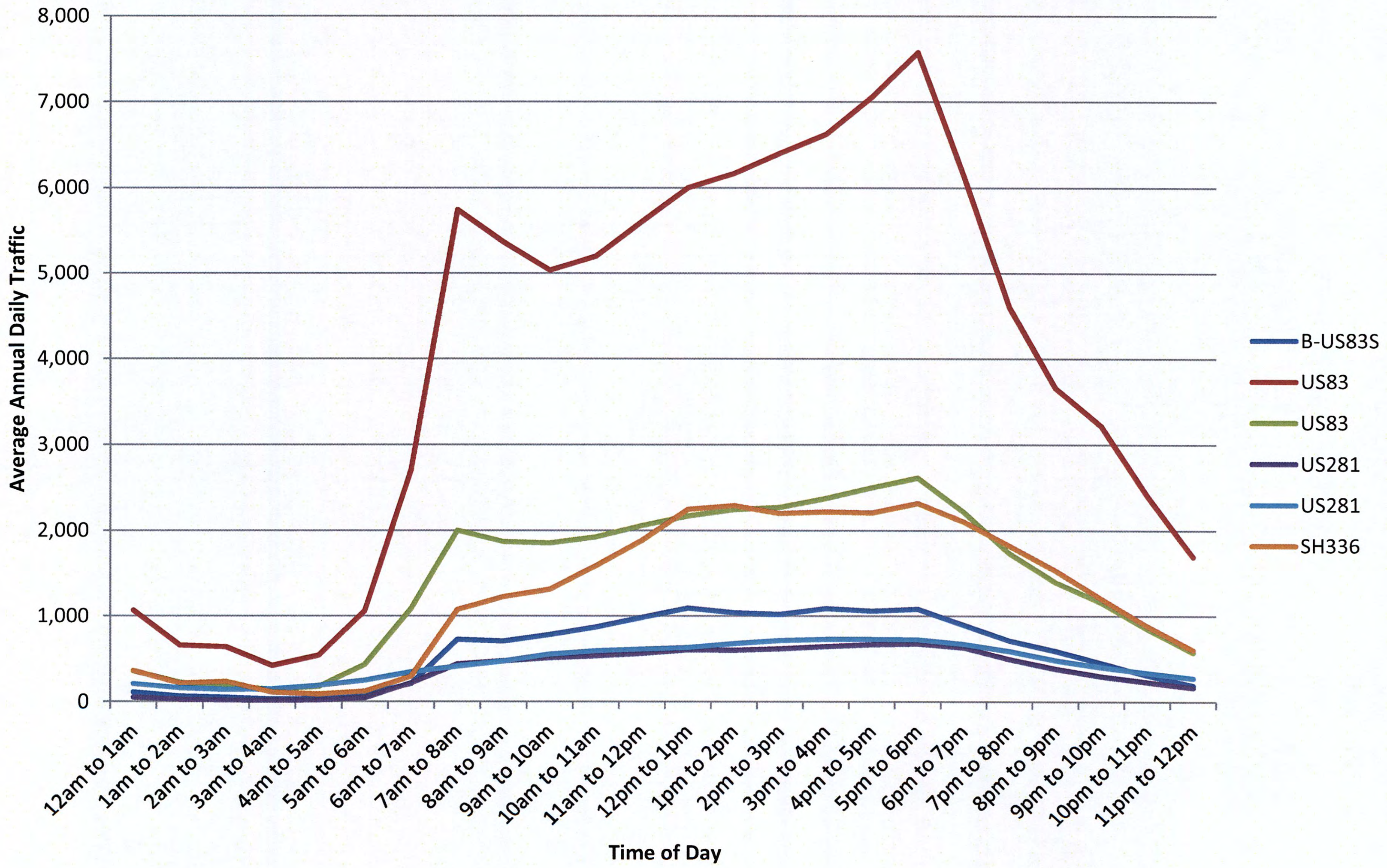
Figure 8. 2009 Hourly Counts (Hidalgo County).
