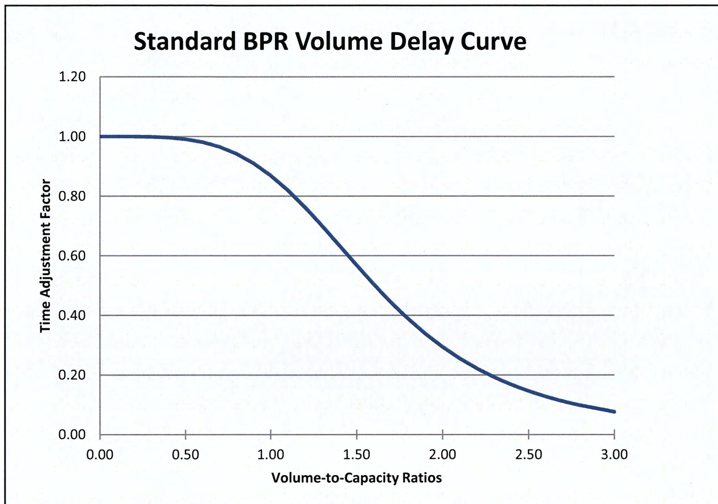
Figure 16. Standard BPR Volume Delay Formulation.
