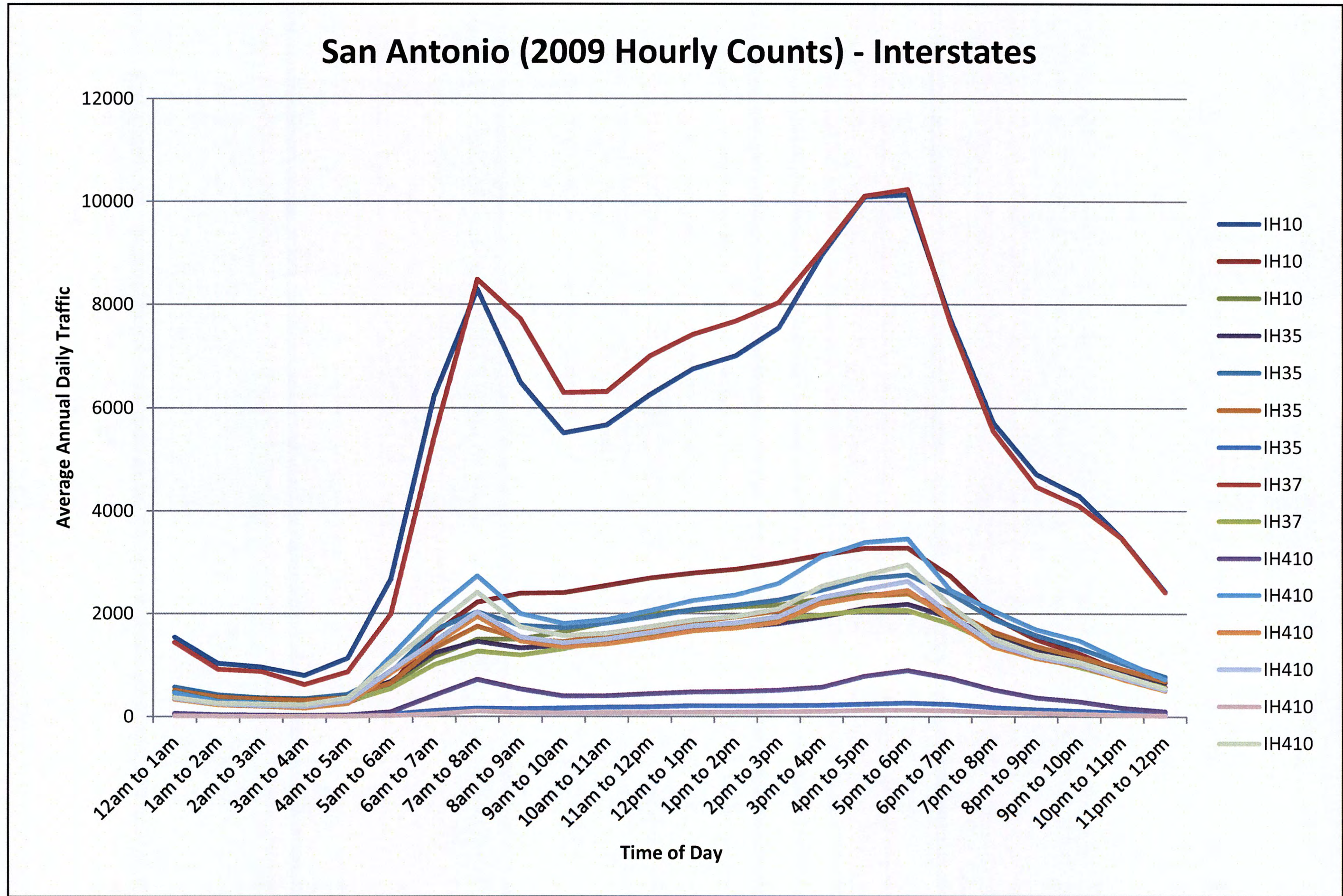
Figure 12. 2009 Hourly Counts (San Antonio)–Interstates Only.
