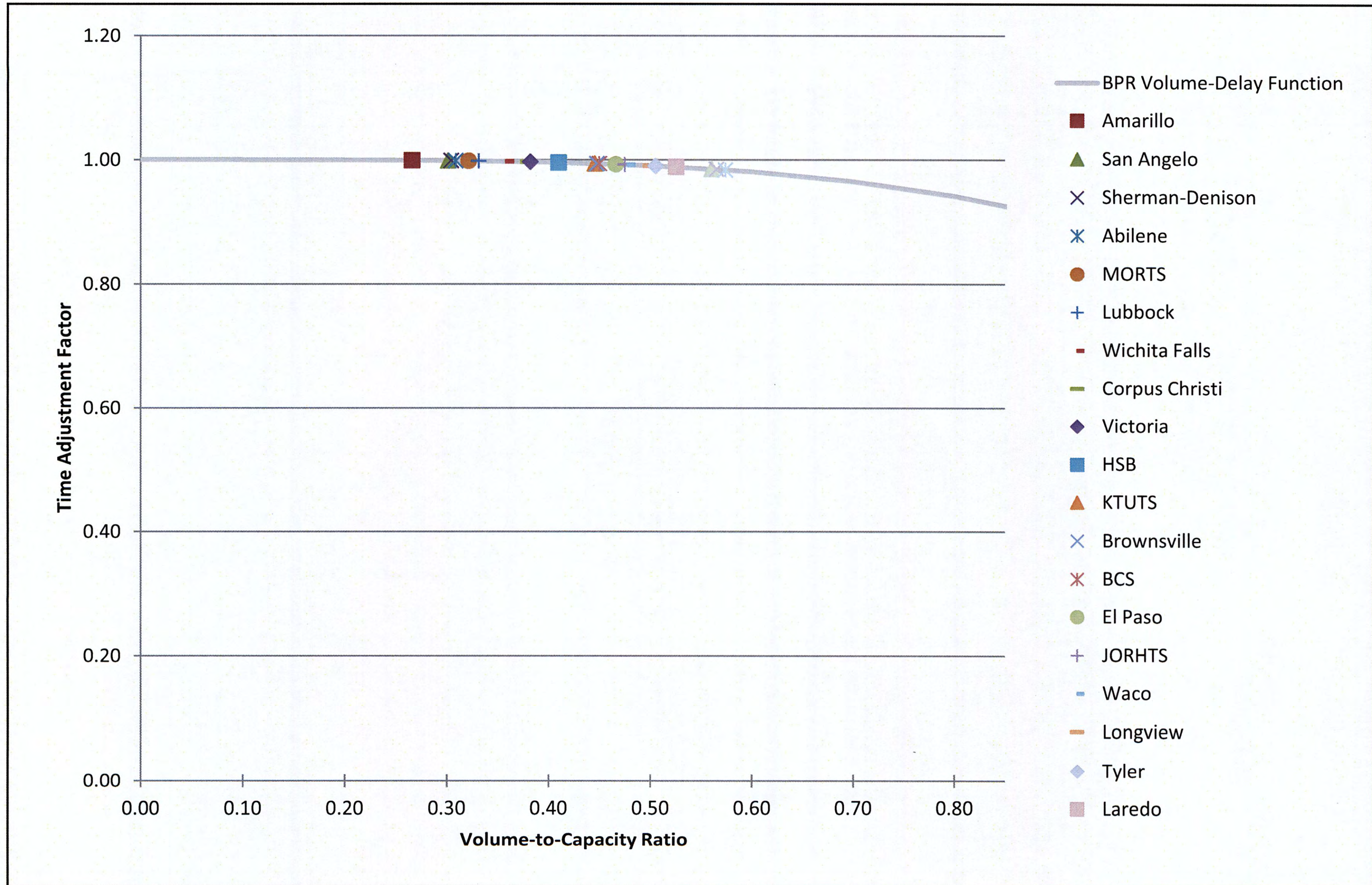
Figure 20. V/C Ratios Relative to BPR Formulation (Magnified).
