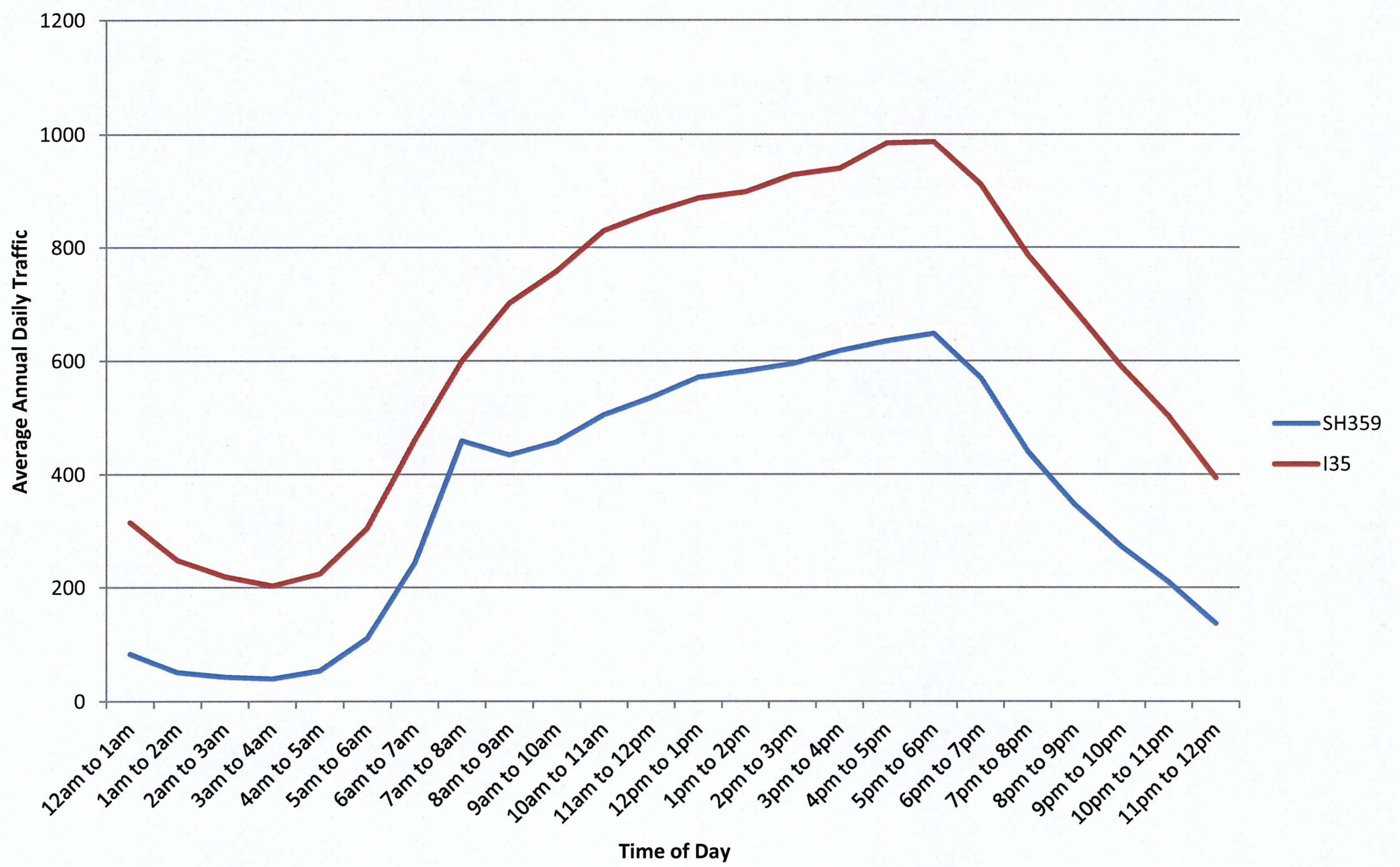
Figure 9. 2009 Hourly Counts (Laredo).
