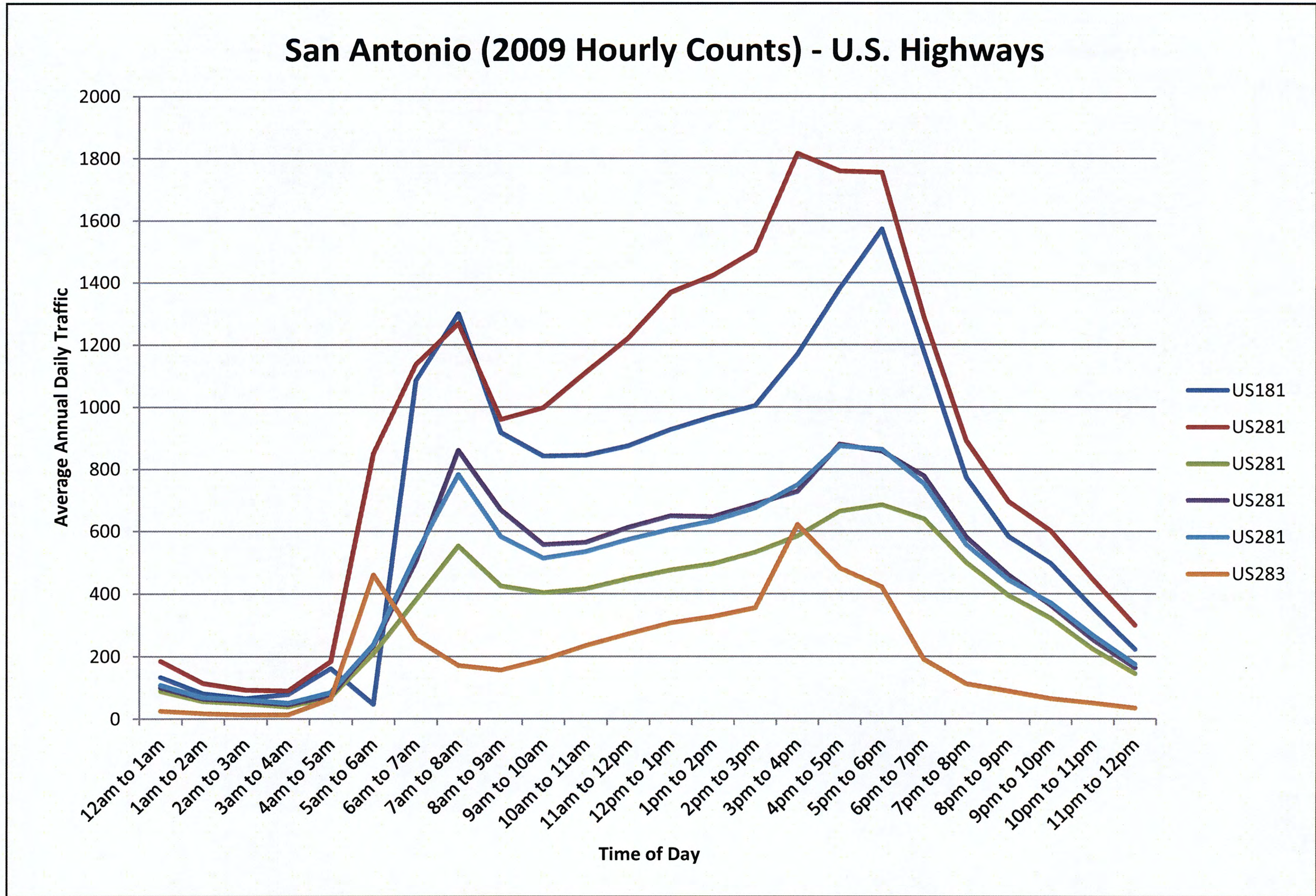
Figure 13. 2009 Hourly Counts (San Antonio)–U.S. Highways Only.
