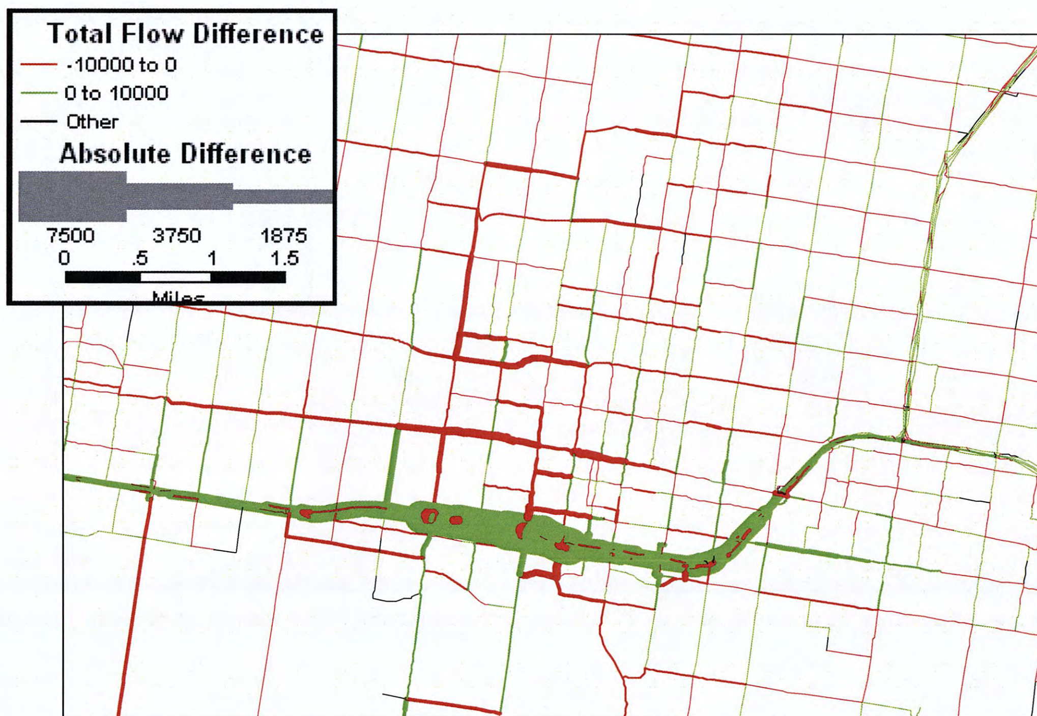
Figure 31. Feedback Model Results with OUE Assignment: Flow Difference after Capacity Added to US 83 in McAllen.
