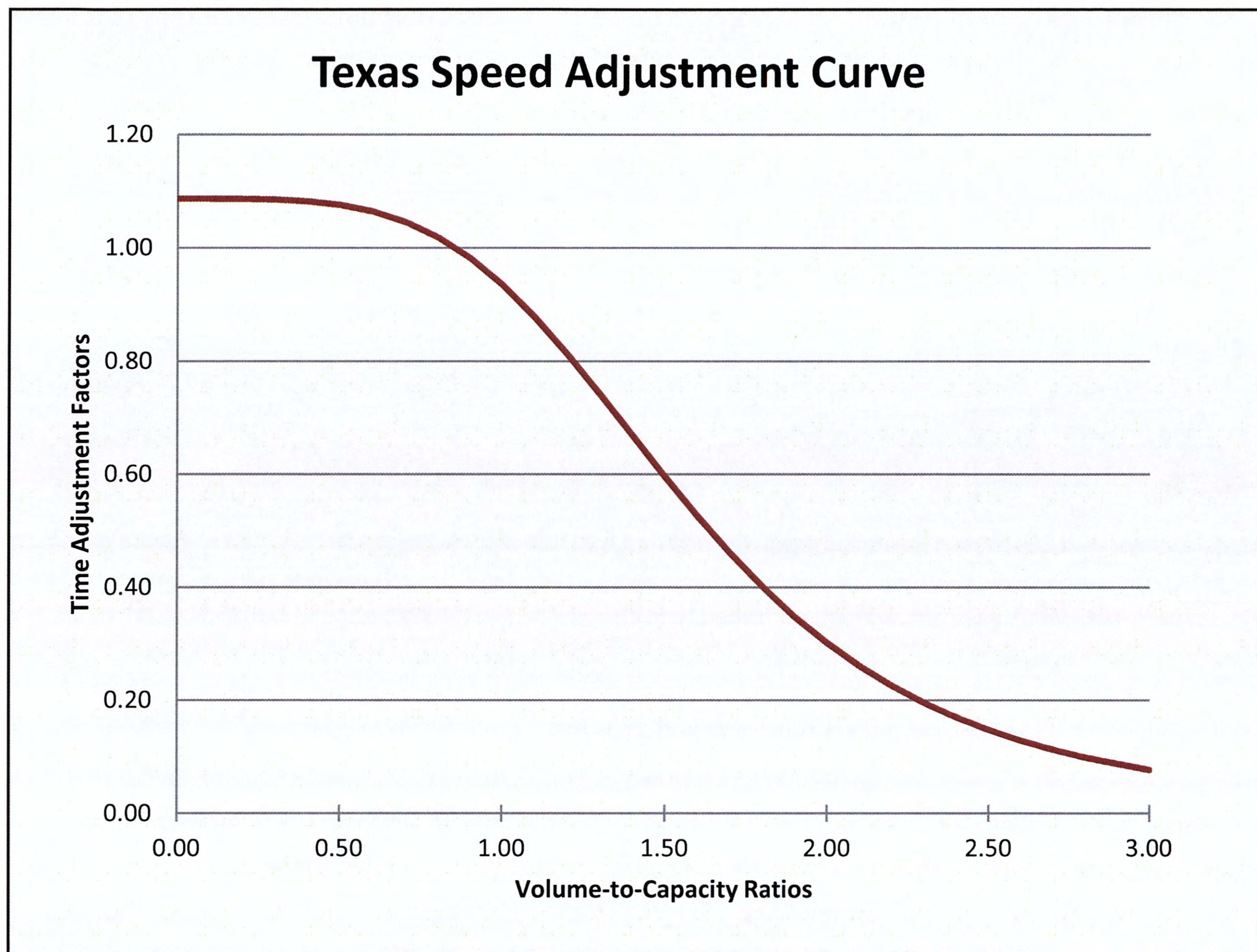
Figure 15. Texas Speed Adjustment Curve.
