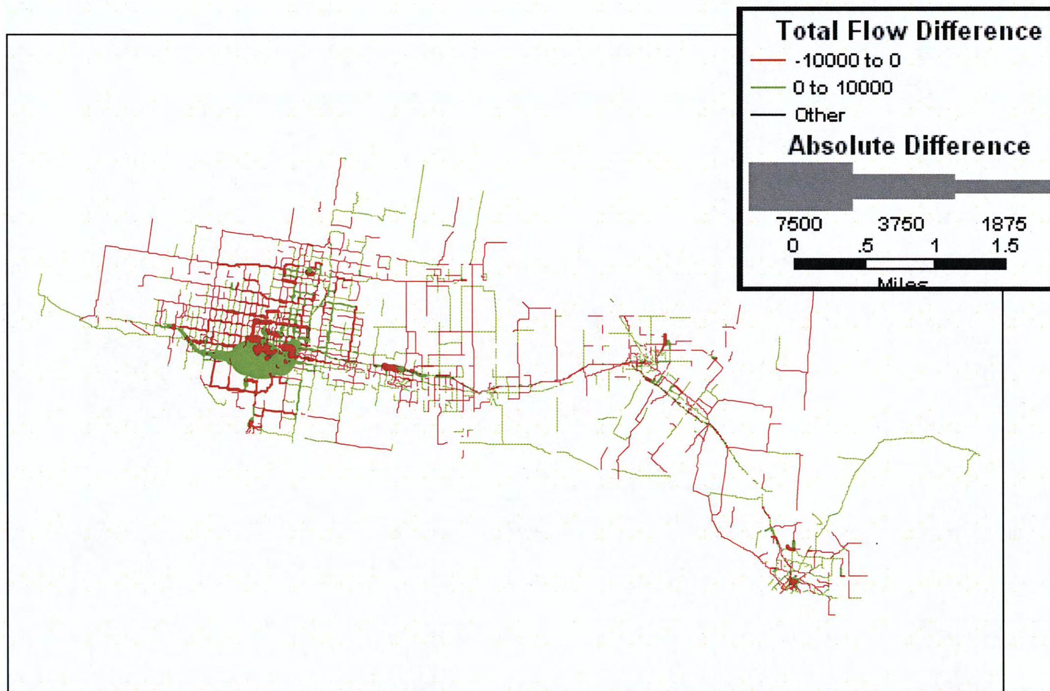
Figure 30. Feedback Model Results: Flow Difference over 10 Trips after Capacity Added to US 83 in McAllen.
