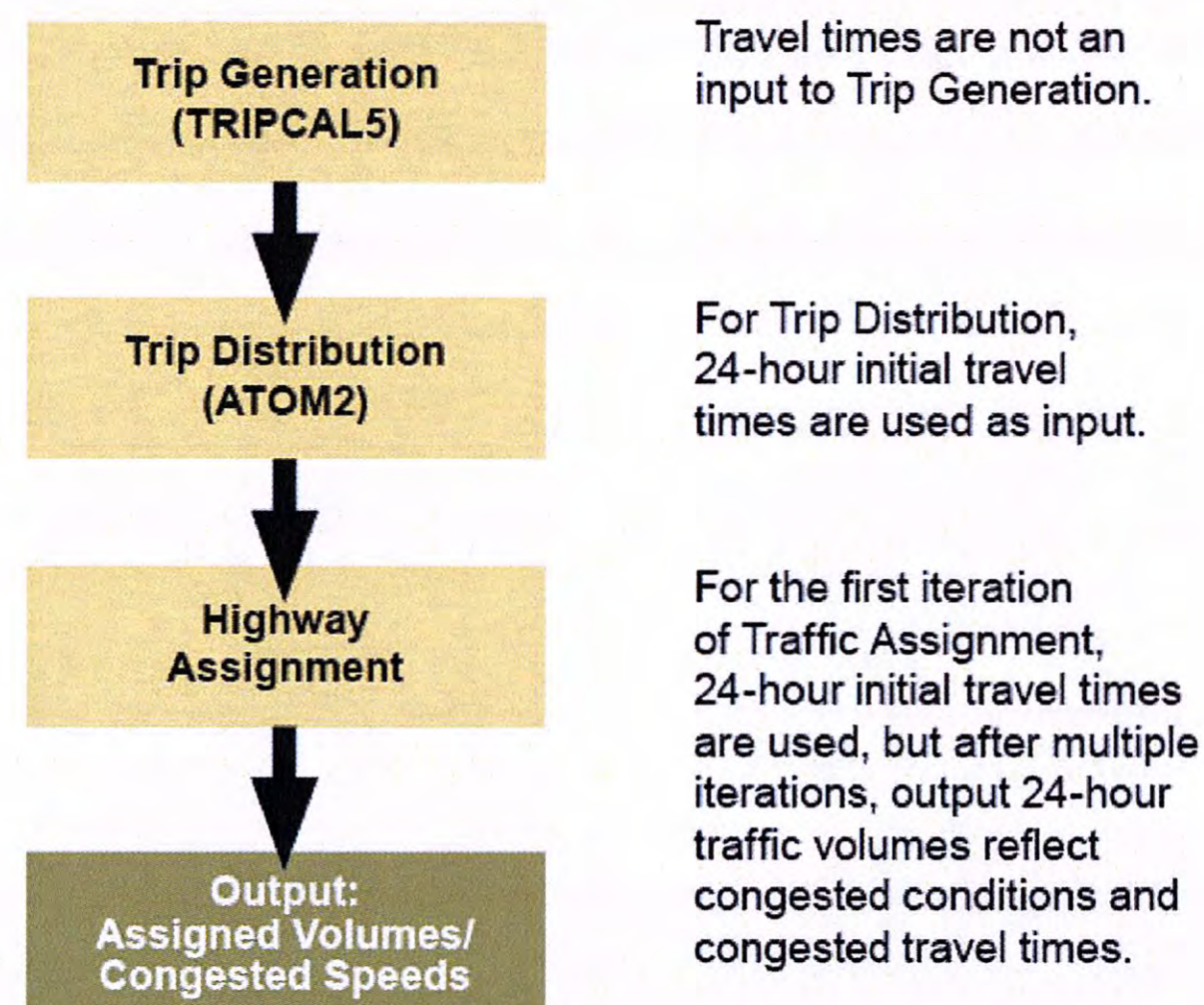
Figure 1. Current TxDOT Three-Step Sequential Travel Demand Model.
