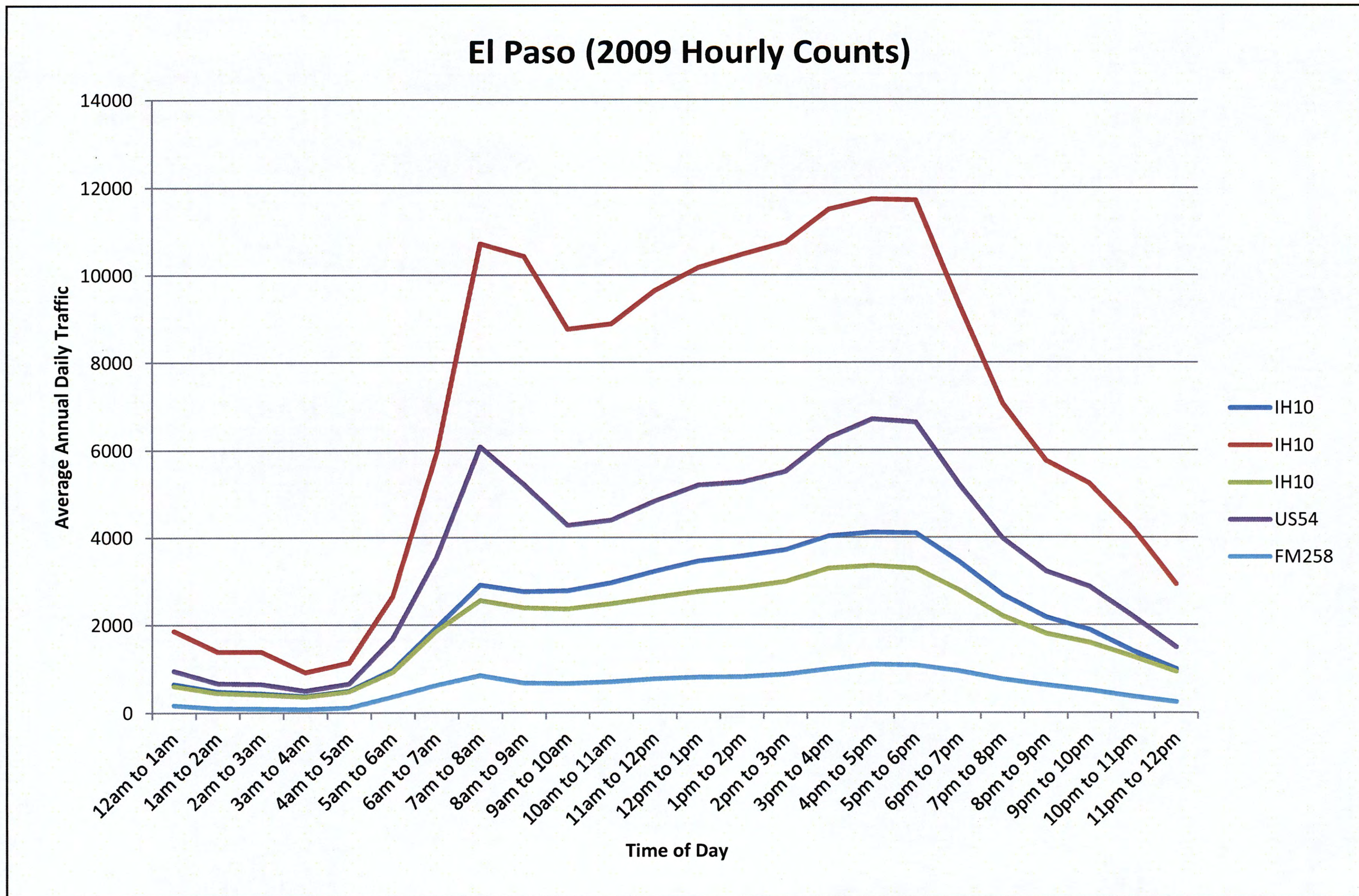
Figure 7. 2009 Hourly Counts (El Paso).
