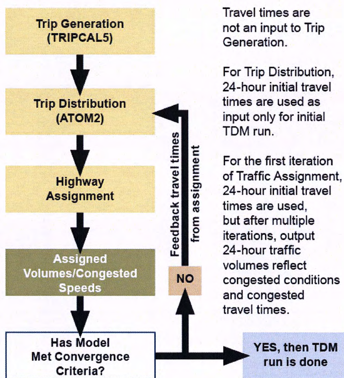
Figure 2. Current TxDOT TDM with Potential Feedback Loop.
