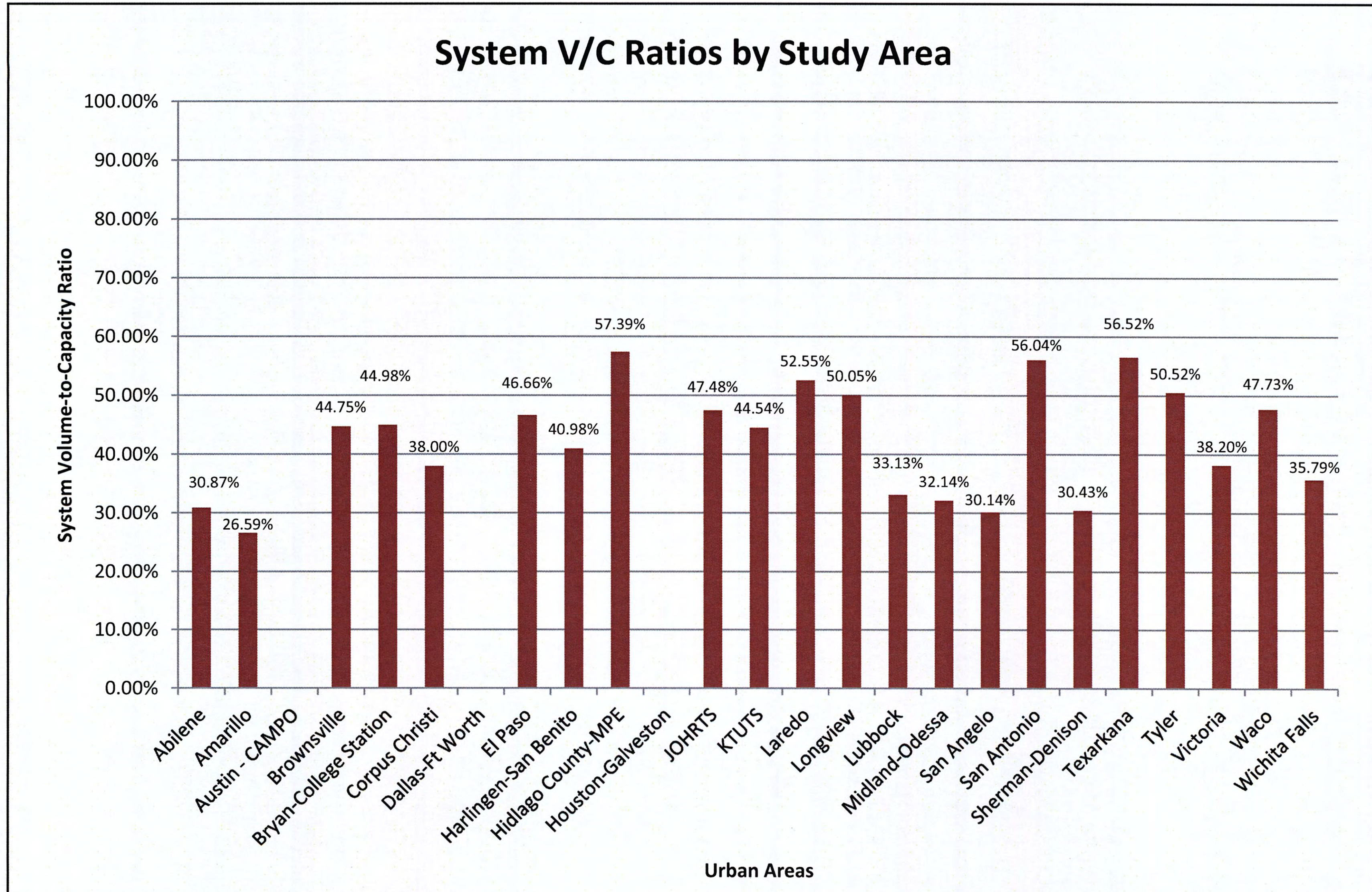
Figure 18. Volume-to-Capacity Ratios by Study Area.
