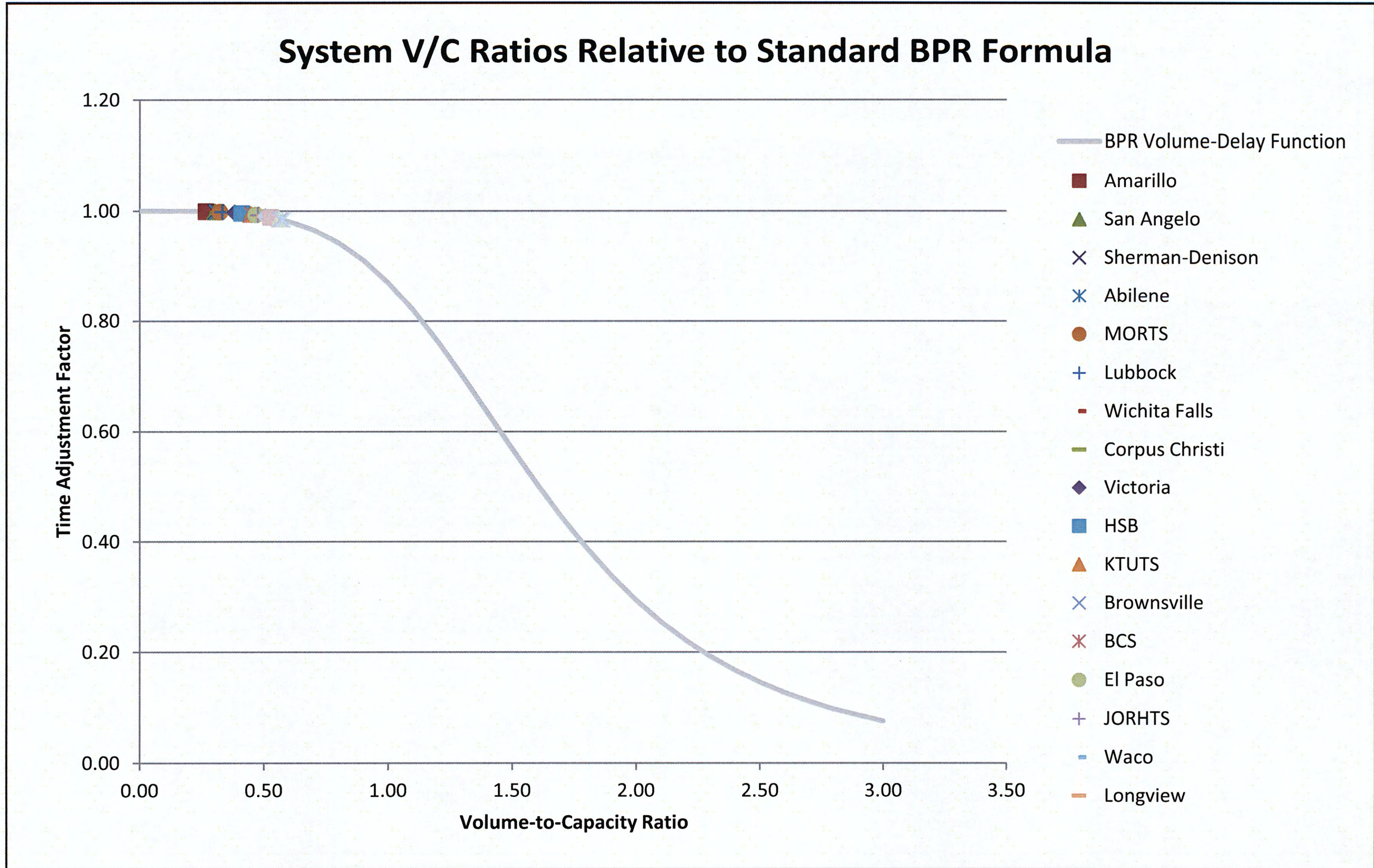
Figure 19. System Volume-to-Capacity Ratios Relative to BPR Formulation.
