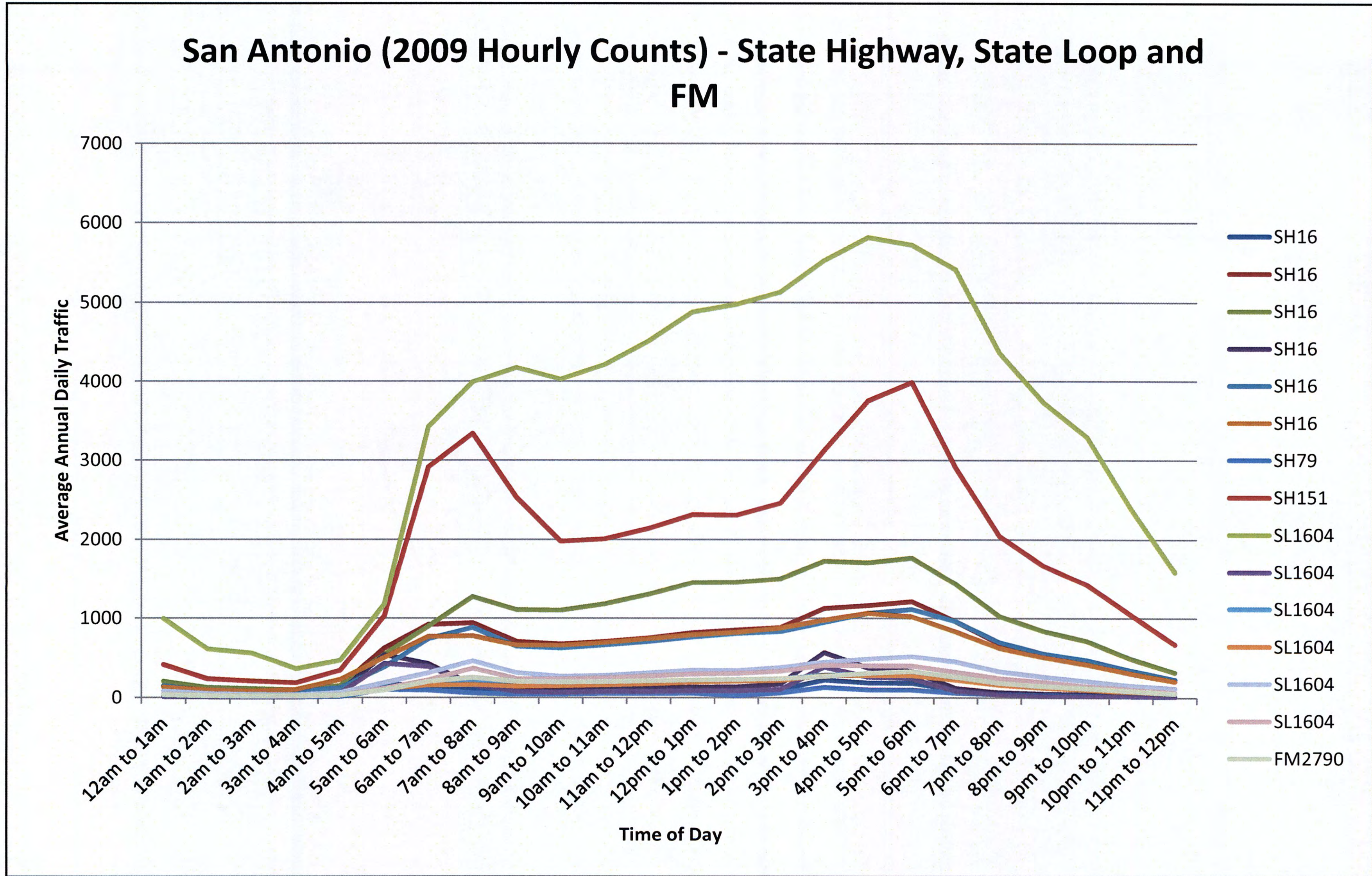
Figure 14. 2009 Hourly Counts (San Antonio)–State Highways, State Loop Roads, and Farm-to-Market.
