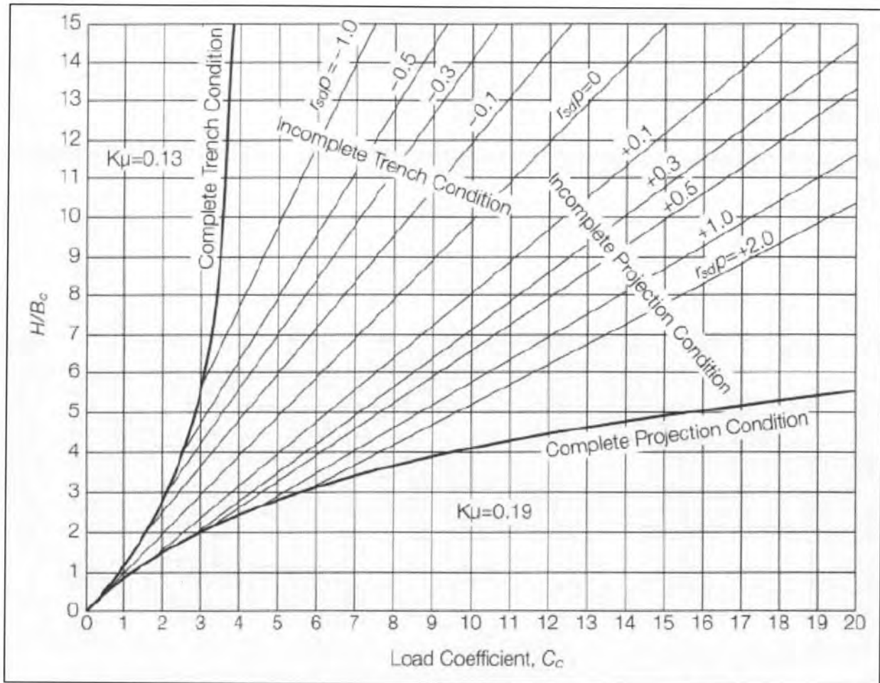
Figure 5. Load Coefficient for Positive Projection Embankment Condition (8).
