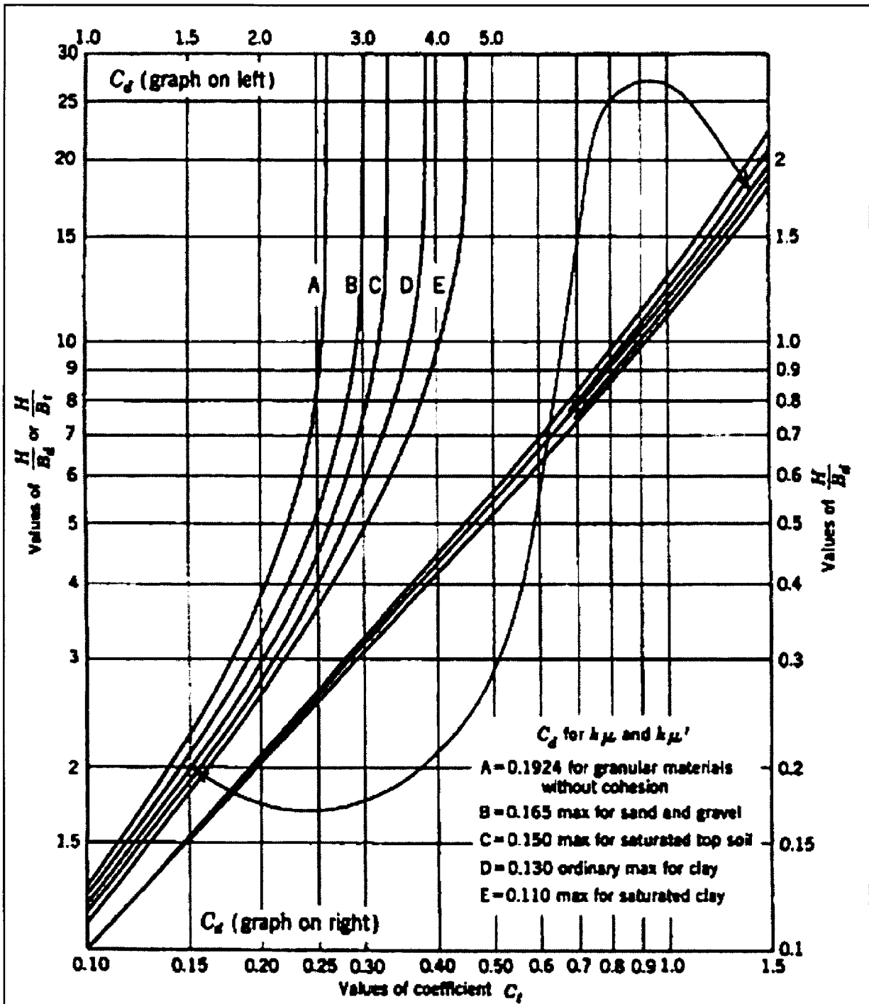
Figure 3. Computational Diagram for Load Coefficient (1).
