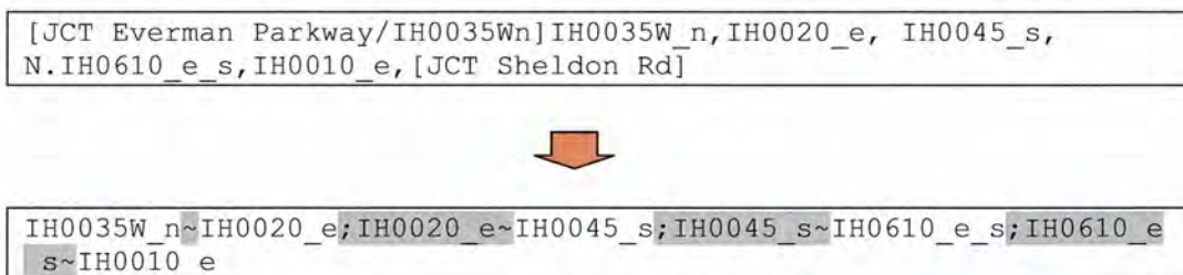
Figure 21. Route Description Before and After Intersection Parsing.
