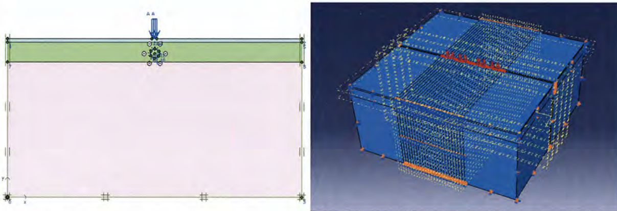
Figure 62. Finite-Element Meshes Used in Analysis (Cross Sectional View and 3D View.)
