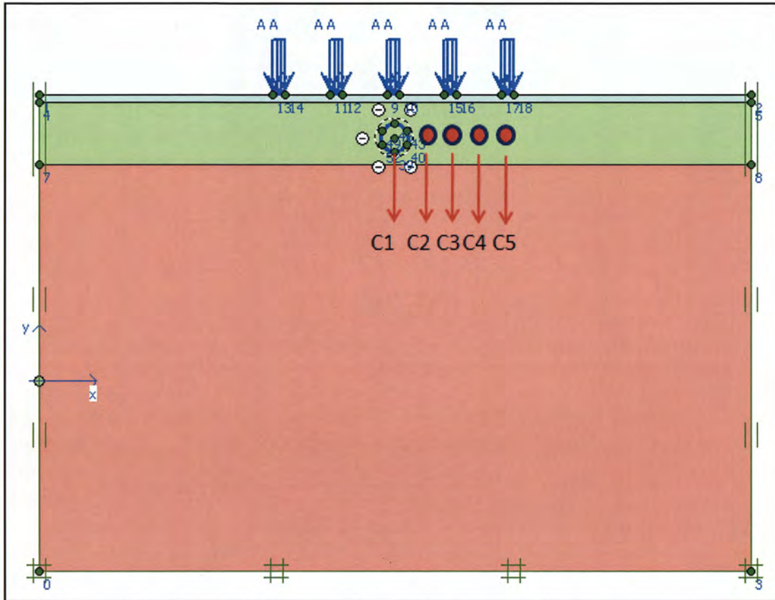
Figure 26. Varied Axle Positions with Respect to Pipe.
