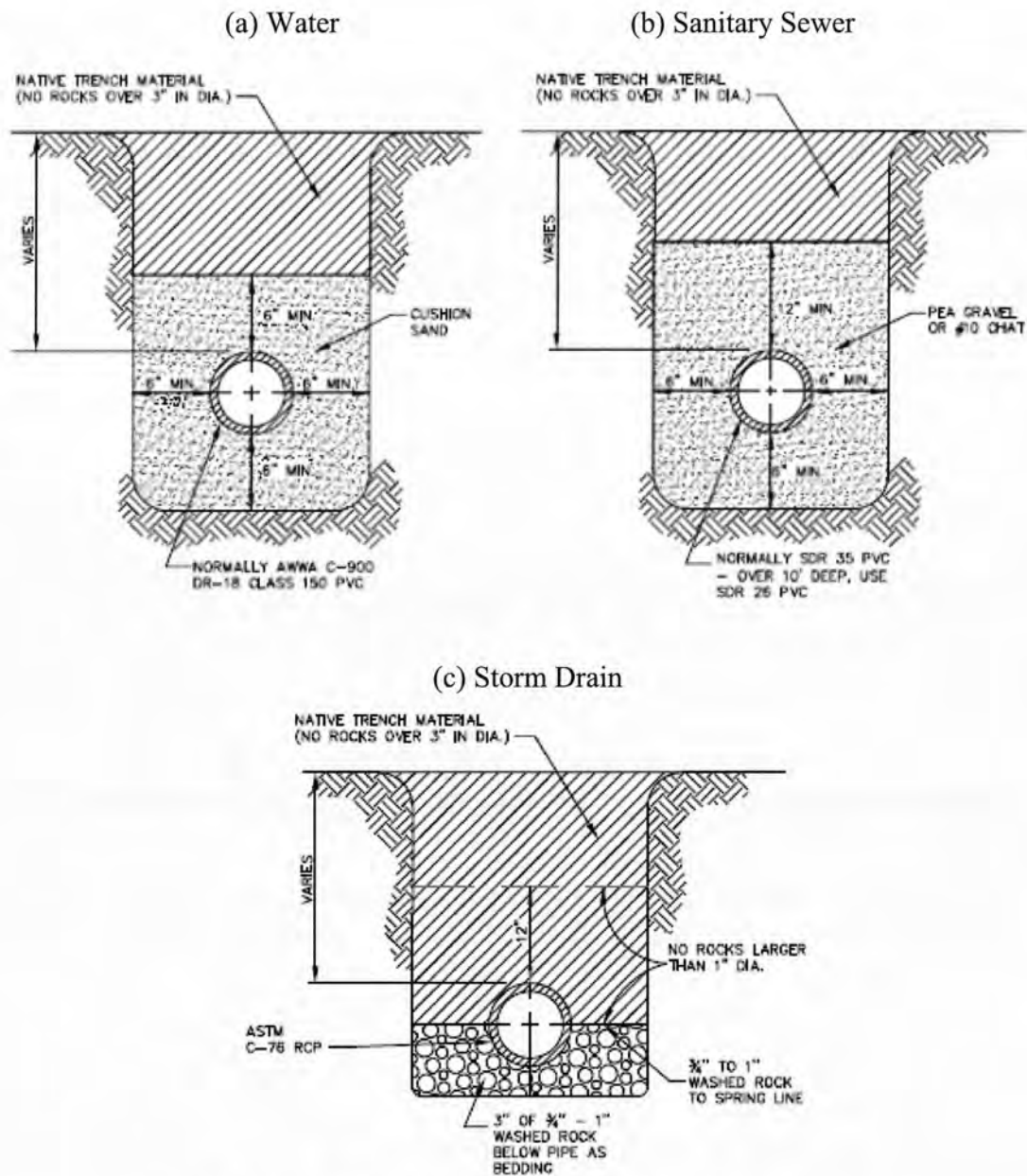
Figure 12. Trench Embedment and Backfill Details.
