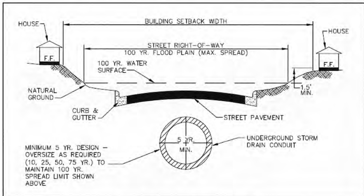
Figure 11. Storm Drain in Street (27).
