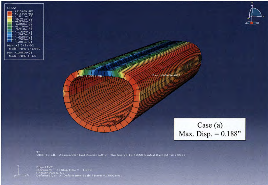
Figure 71. Calculated Vertical Displacement, Condition (a) (Blue Indicates Largest Displacement).
