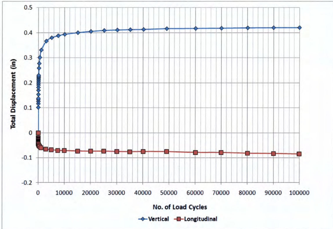
Figure 50. Total Displacement versus Number of Load Cycles of Jointed PVC Pipe.
