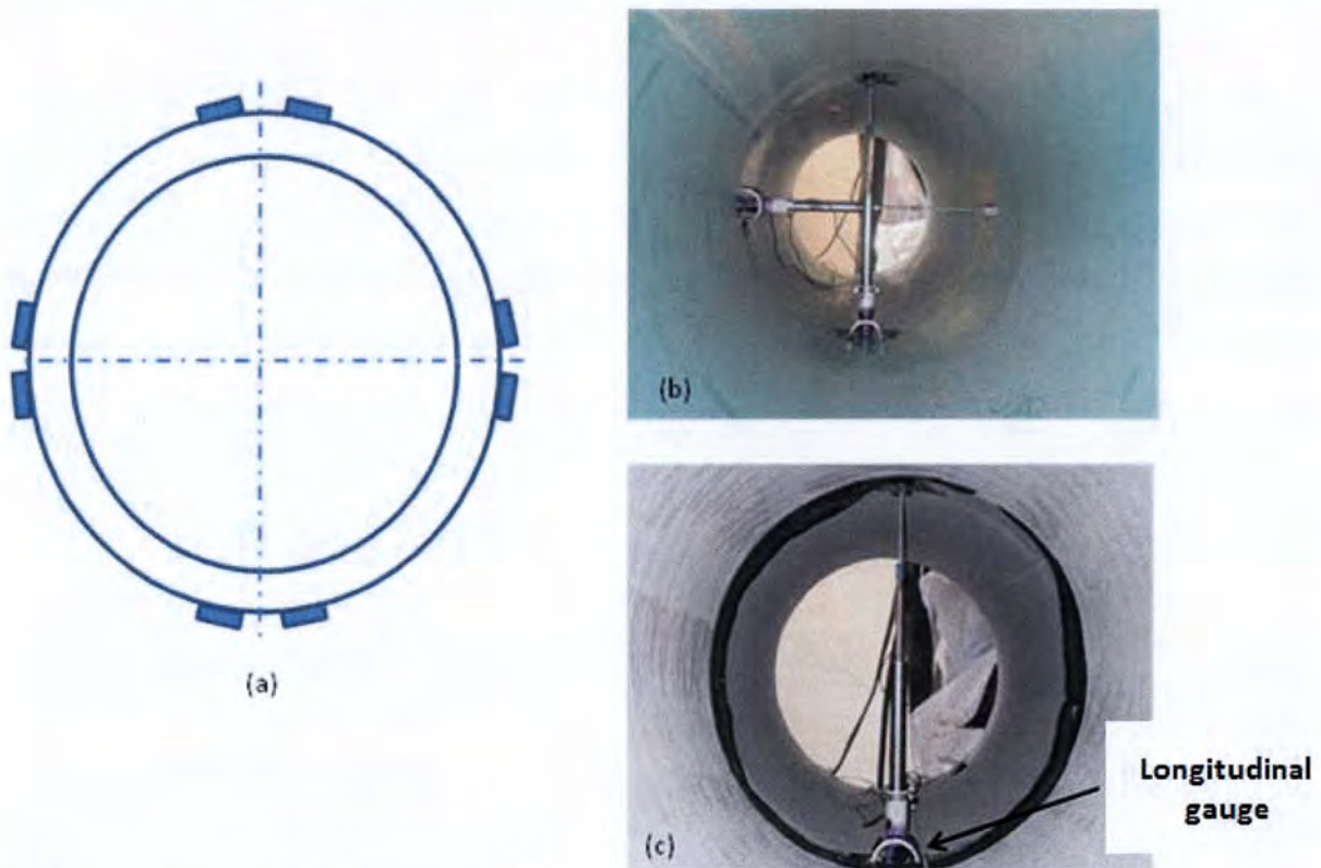
Figure 39. Layout of Instrumented Sensors: (a) 8 Strain Gauges for Unjointed PVC Pipe; (b) 2 LVDTs for Unjointed PVC Pipe; (c) Vertical and Longitudinal LVDTs for Jointed Concrete Pipe.
