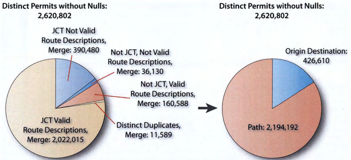
Figure 91. Development of Origin Destination and Path Datasets.
