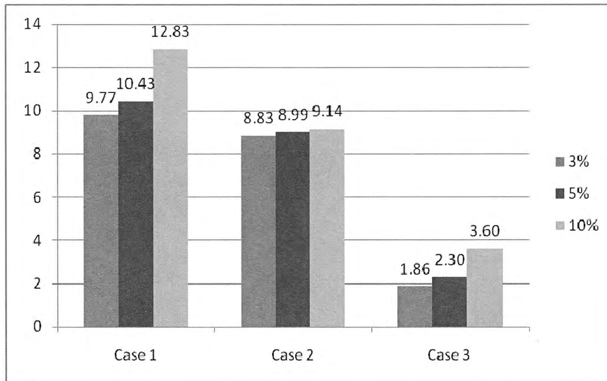
Figure 7 Queue Time (mins) for all Cases by Comparison for all Secondary Inspection Levels
