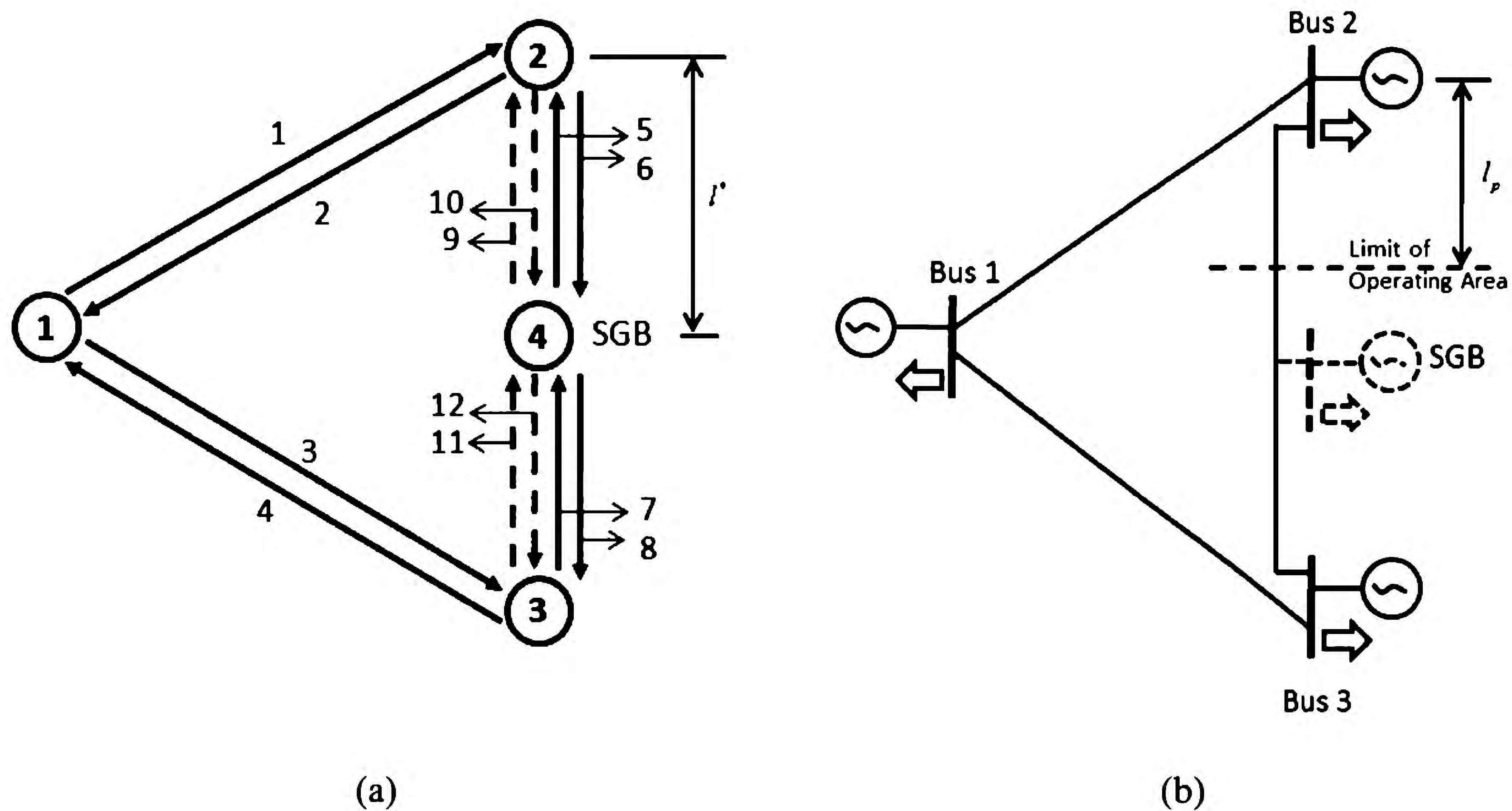
Figure 4.2. Example Networks
