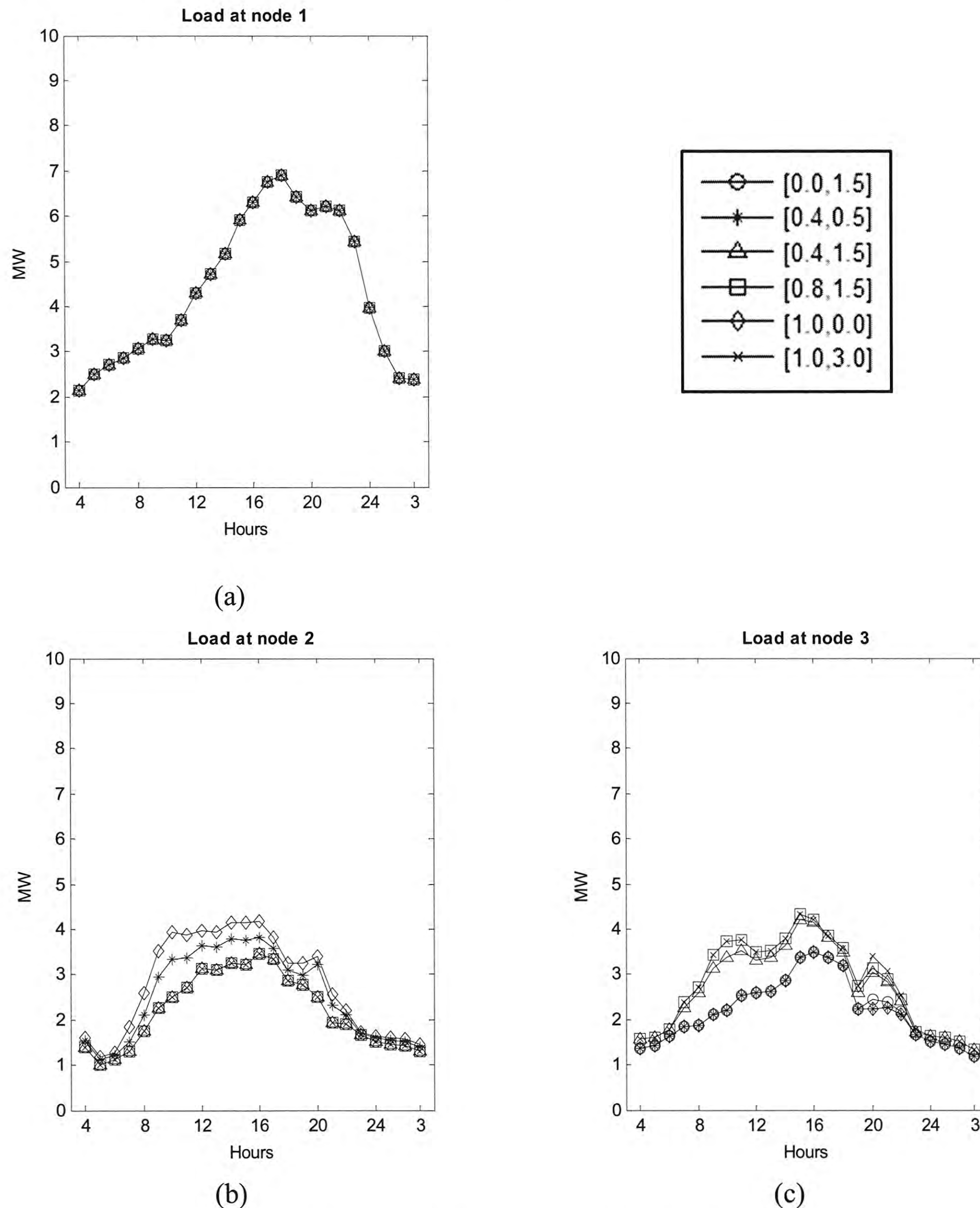
Figure 4.6. Power Load in G2V
