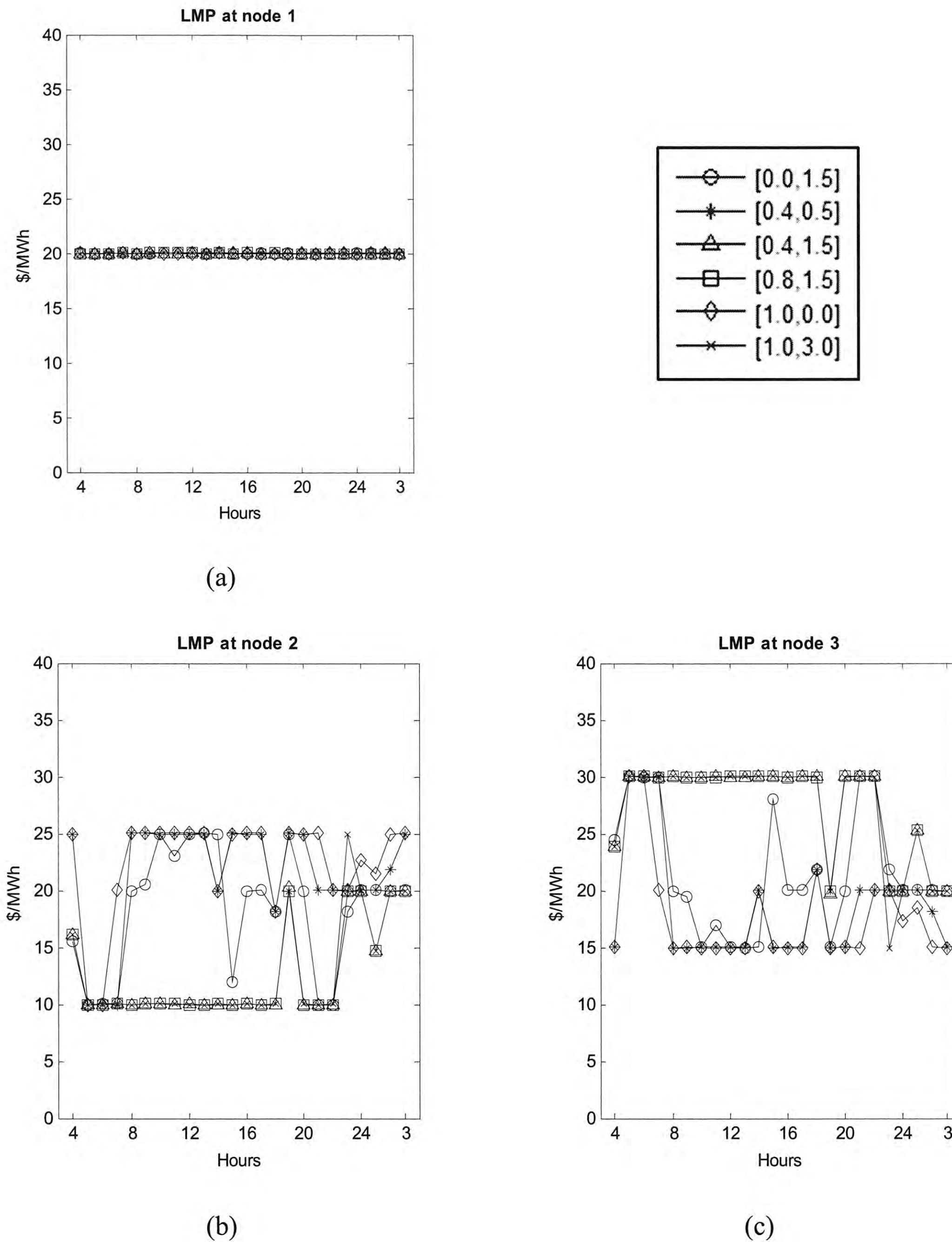
Figure 4.8. LMP in G2V
