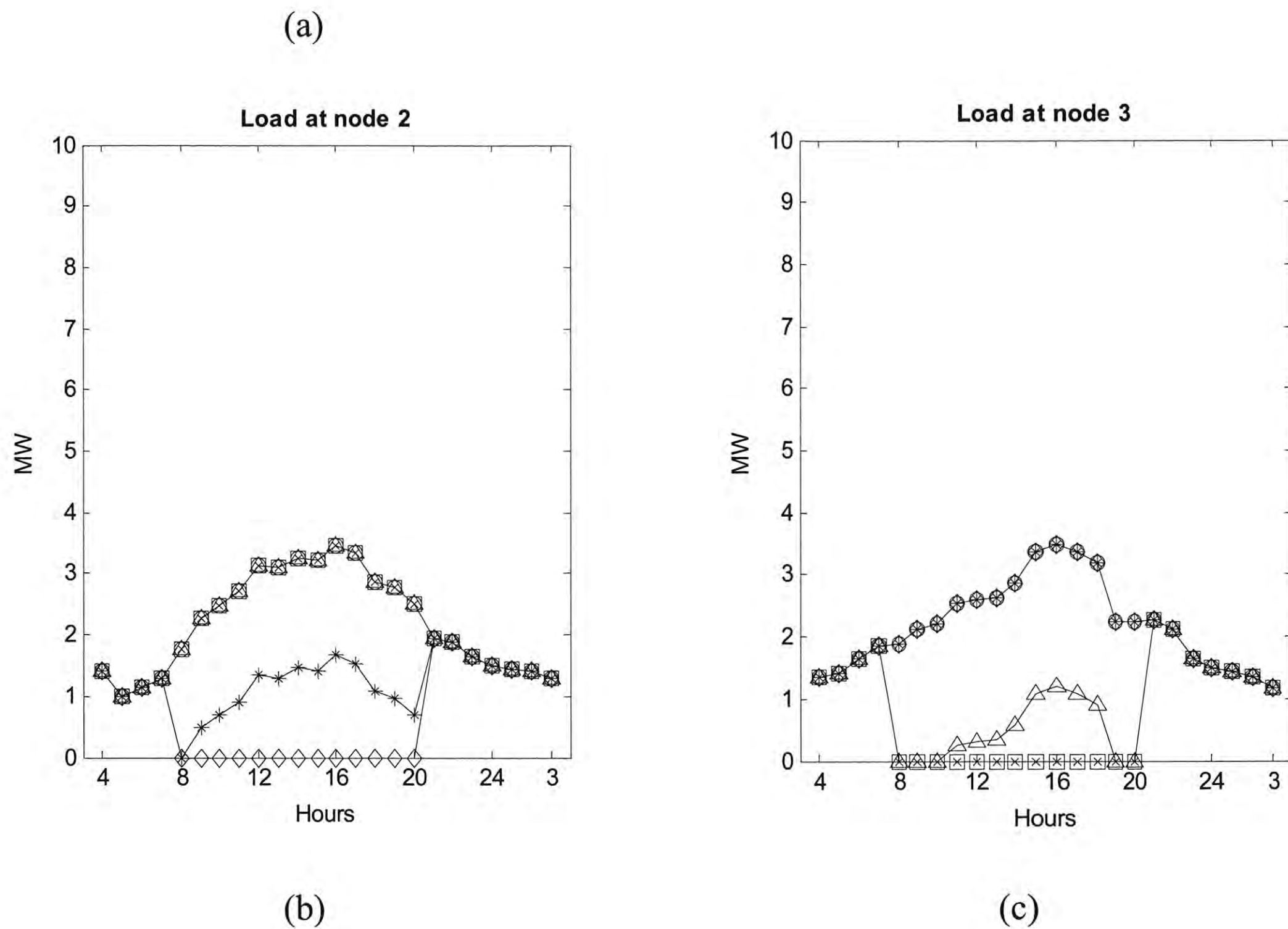
Figure 4.3. Power Load in V2G.
