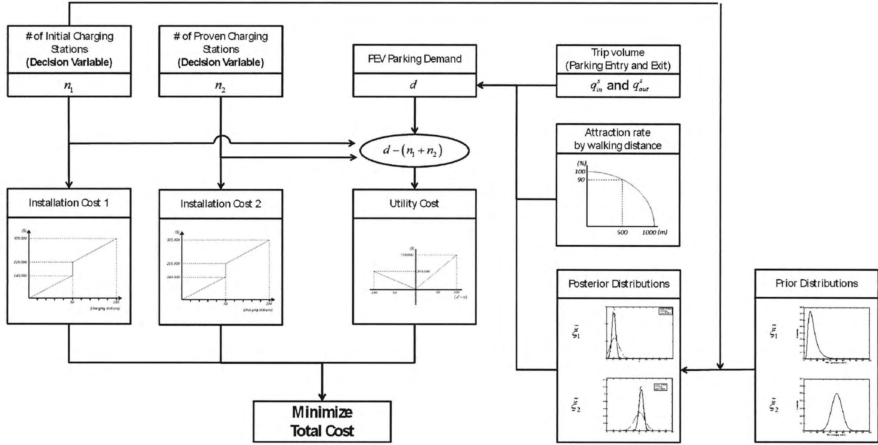
Figure 6.1 Model Framework
