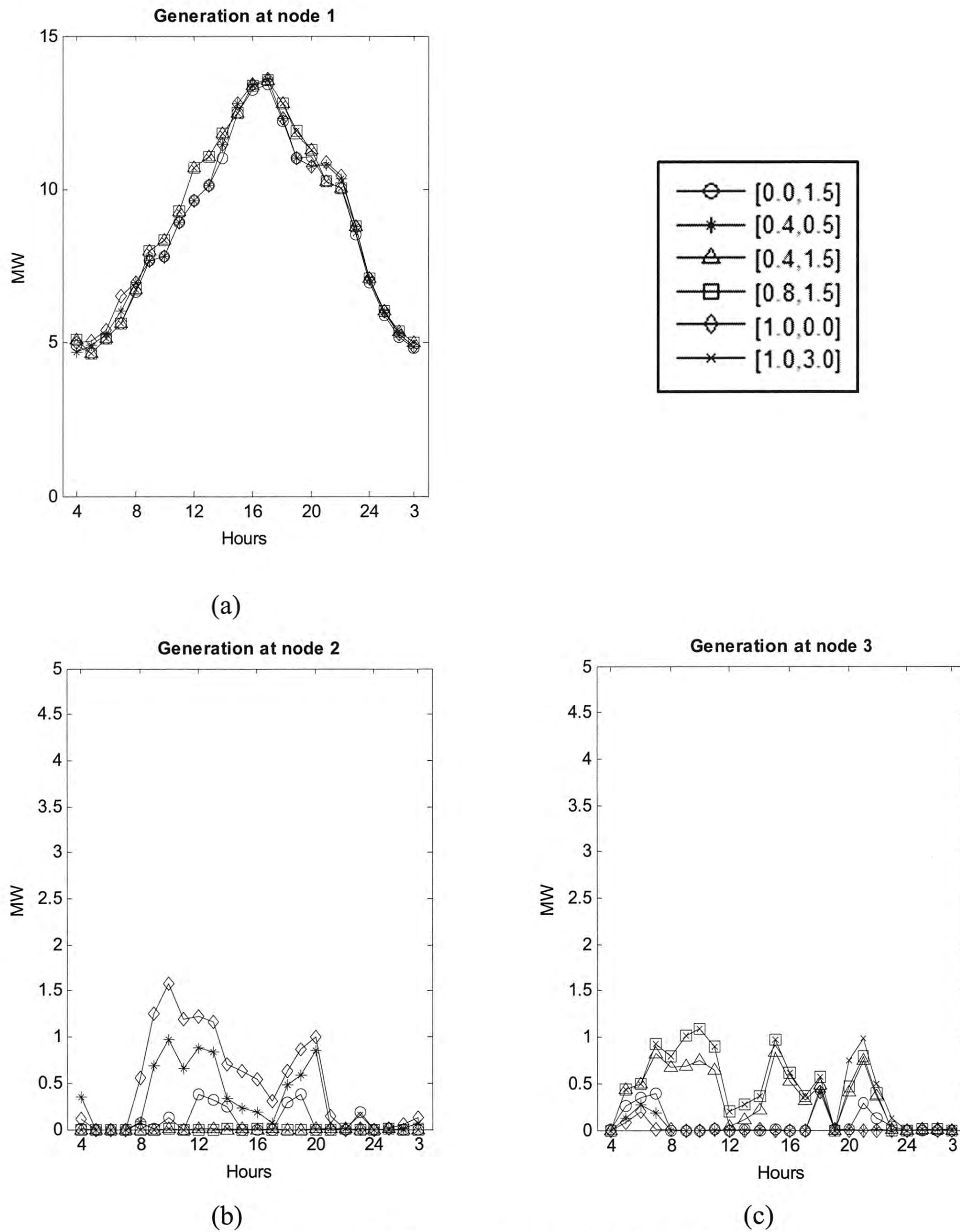
Figure 4.7. Power Generation in G2V
