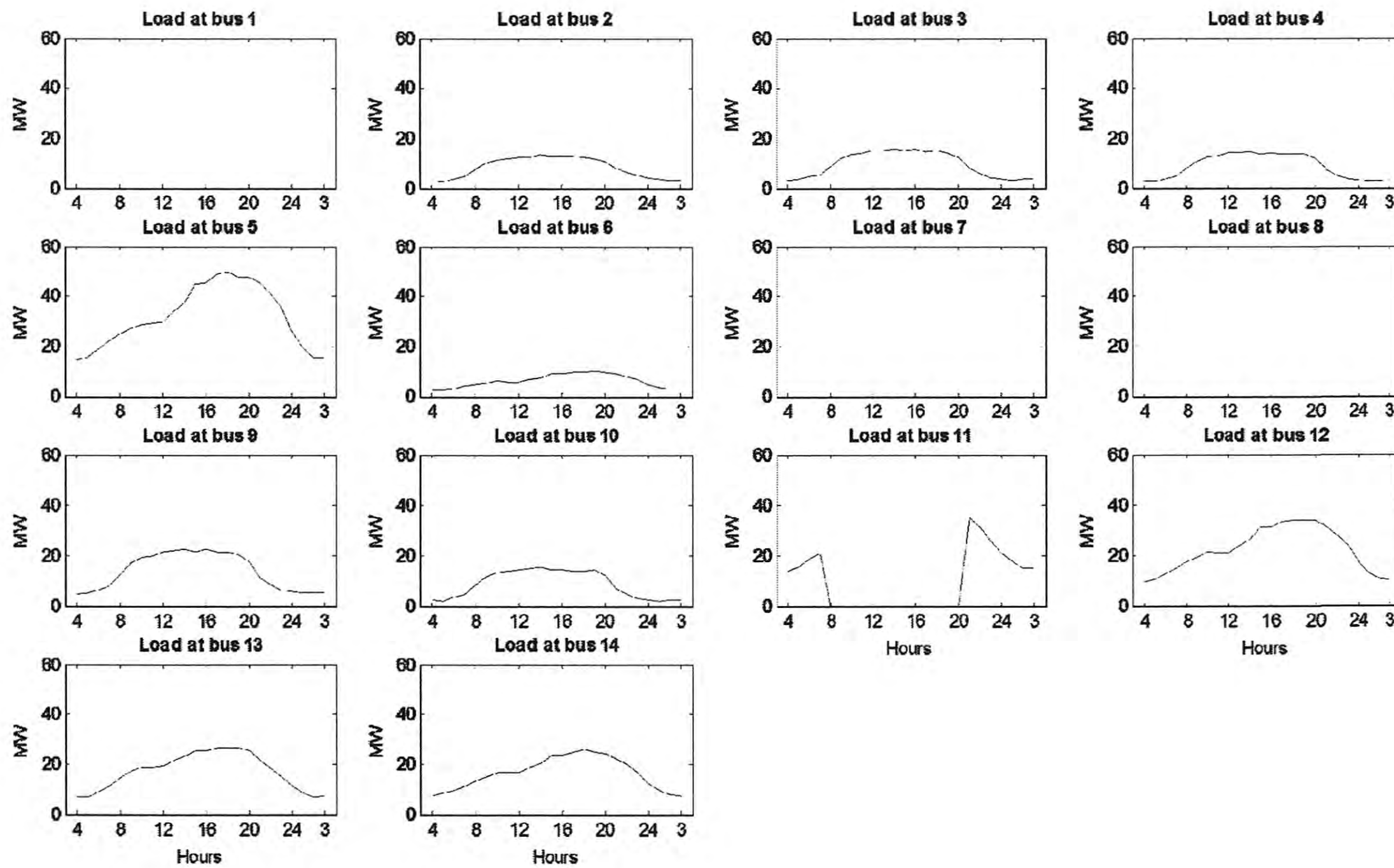
Figure 4.14 Power Load in V2G of Large Network
