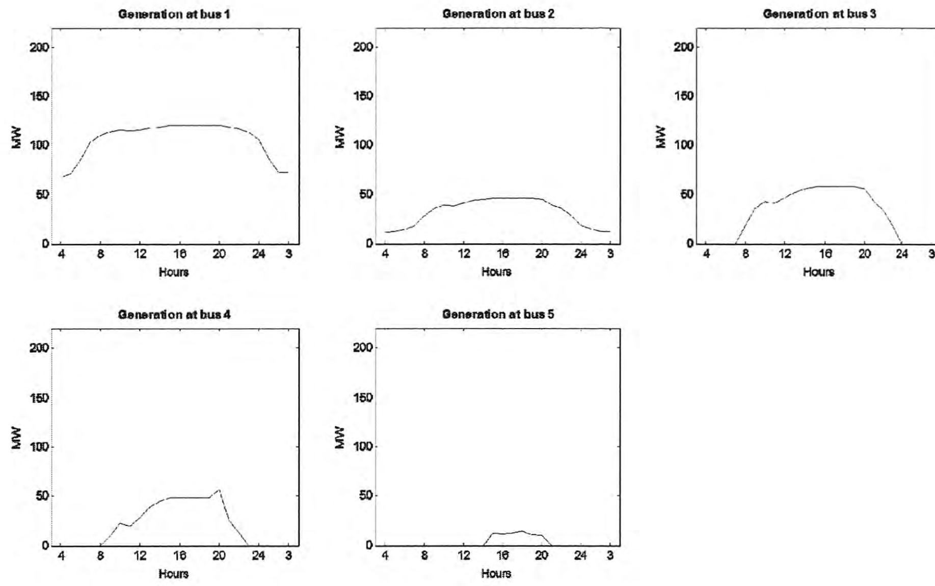
Figure 4.18 Power Generation in G2V of Large Network
