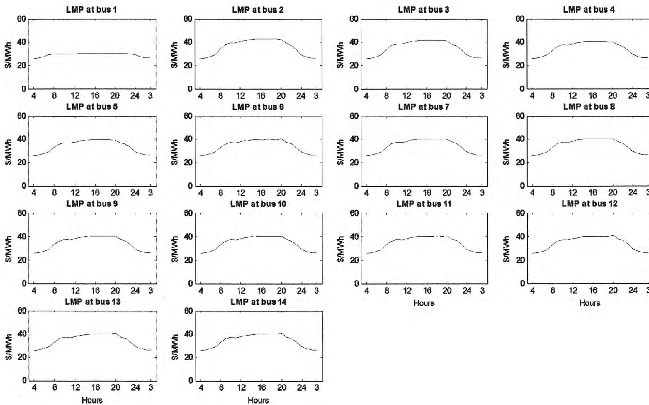
Figure 4.19 LMP in G2V of Large Network
