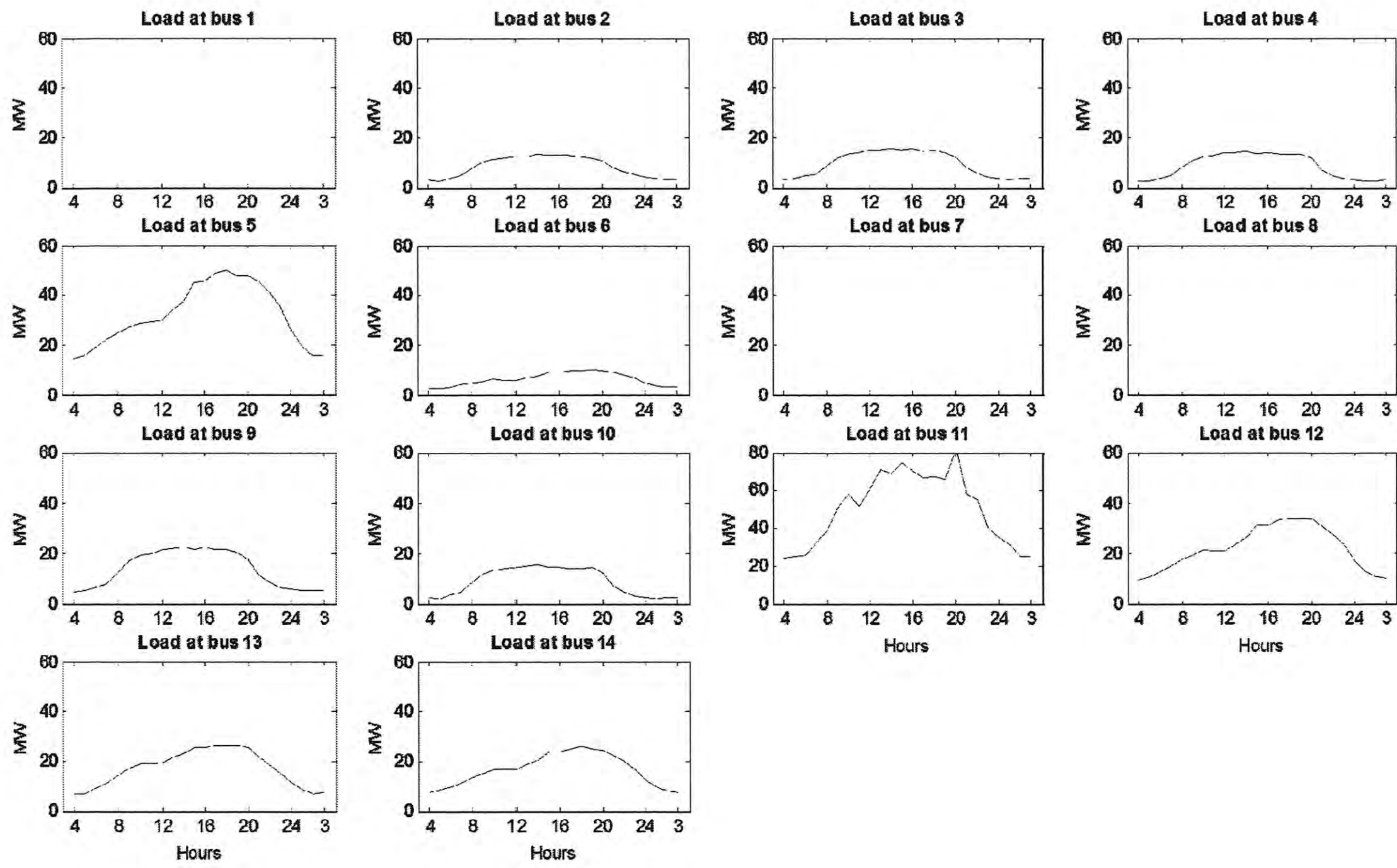
Figure 4.17 Power Load in G2V of Large Network
