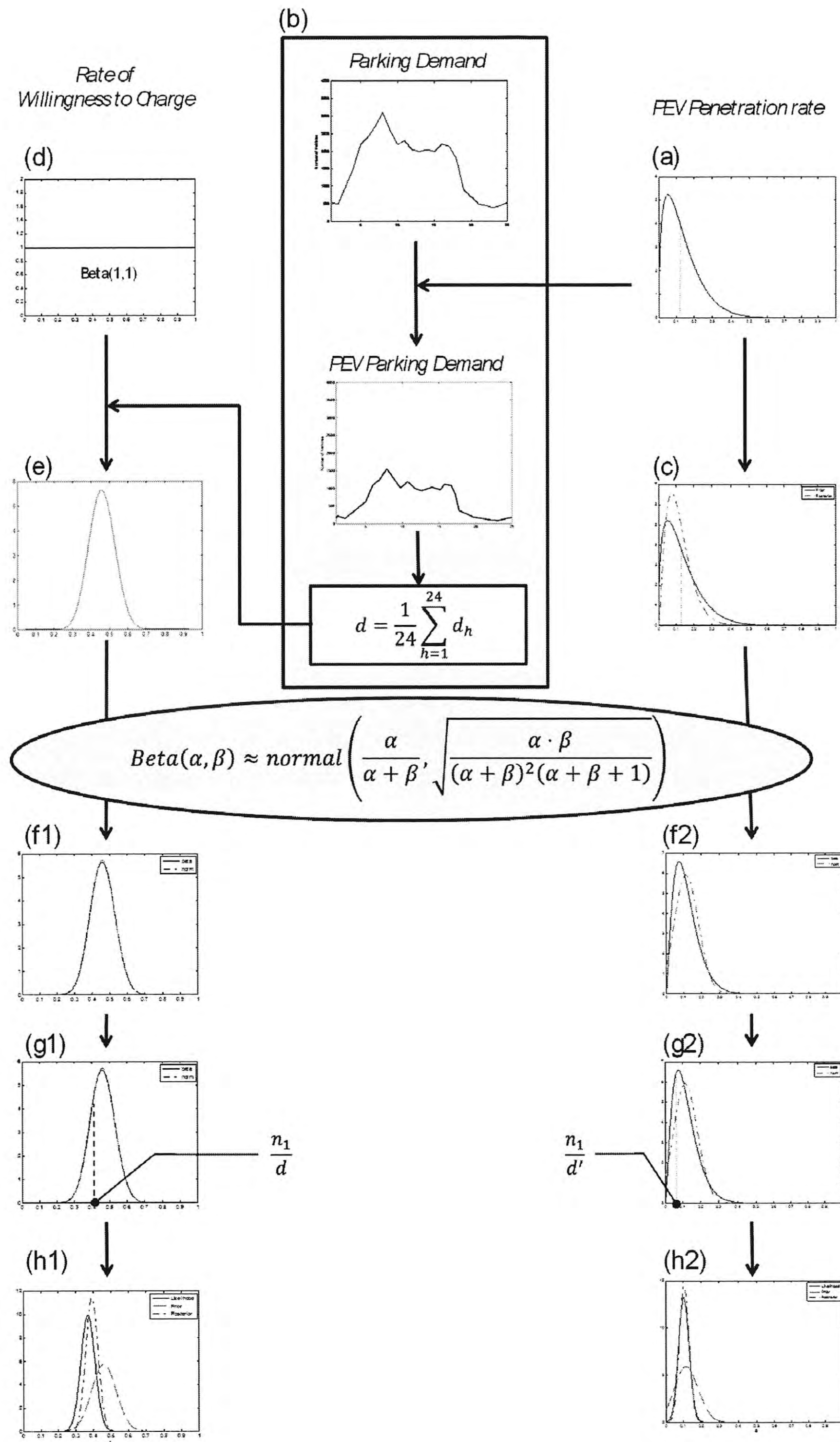
Figure 6.2. Procedure of Bayesian Updating
