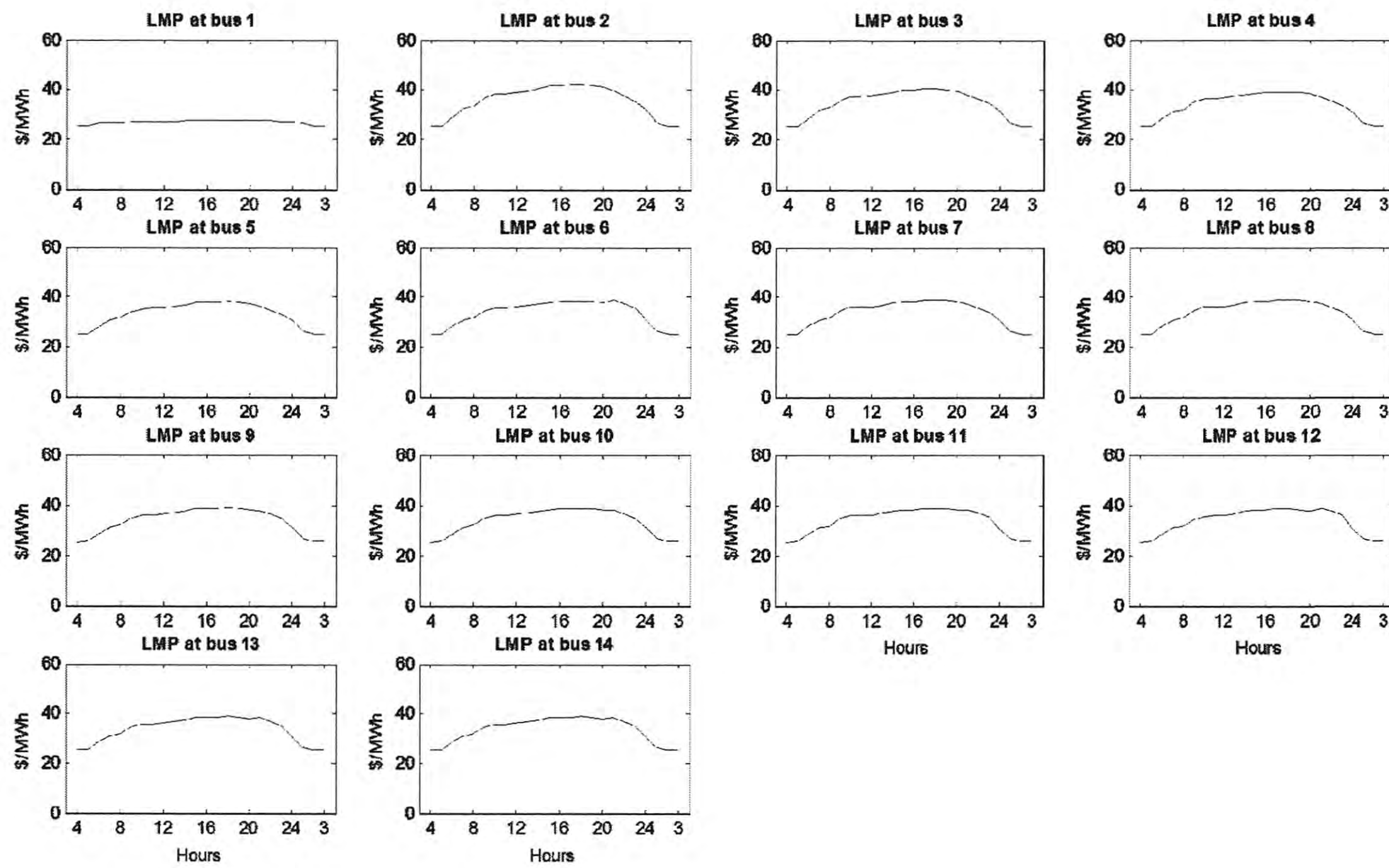
Figure 4.16 LMP in V2G of Large Network
