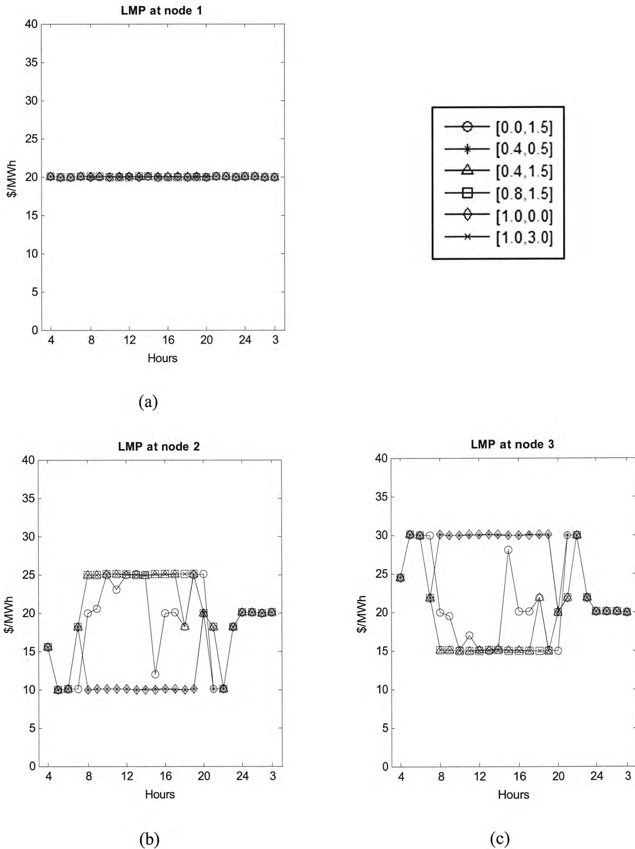
Figure 4.5. LMP in V2G.
