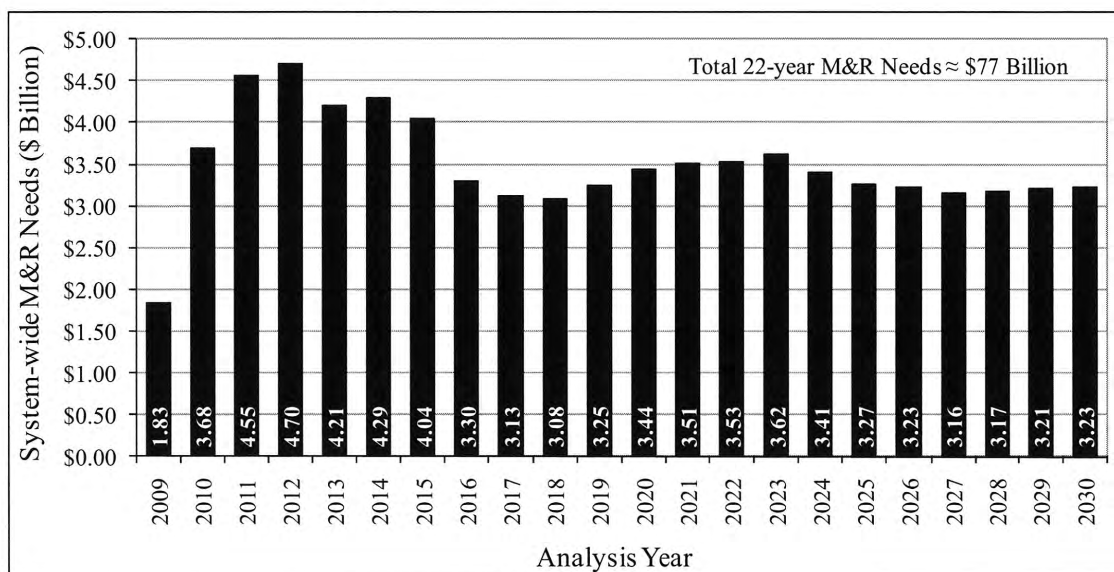
Figure 5: Annual M&R needs to attain and maintain 90% 'Good' or better condition.
