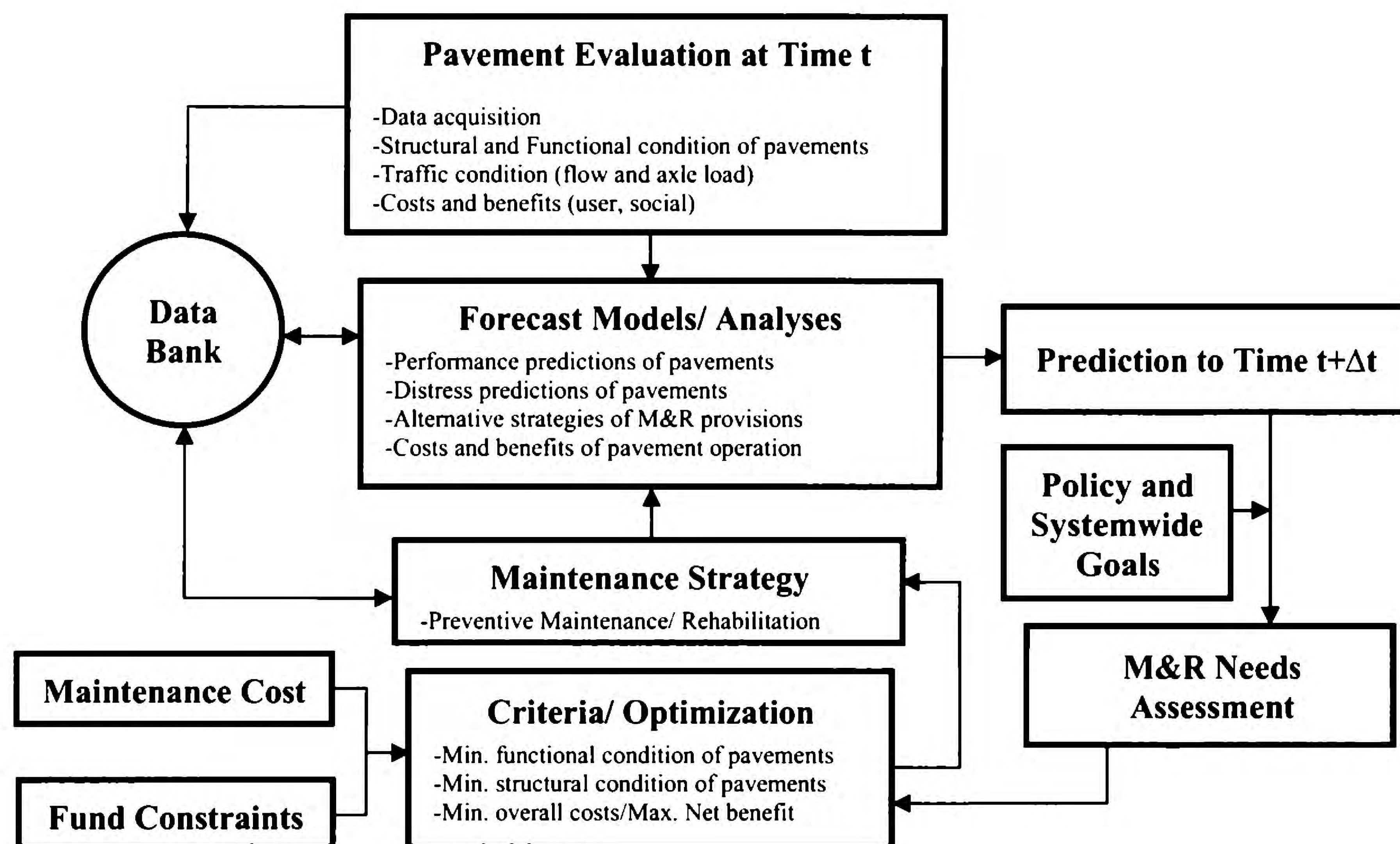
Figure 1: Model Flowchart of Pavement Management Process.
