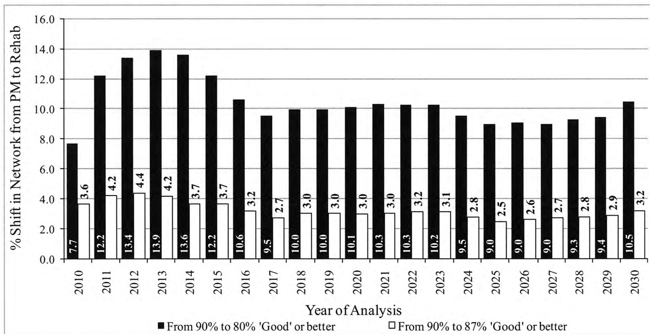
Figure 10: Shift in percent of network from Preventive Maintenance to Rehabilitation category due to reduction in performance goal from 90% 'Good' or better to 87% or 80% 'Good' or better.
