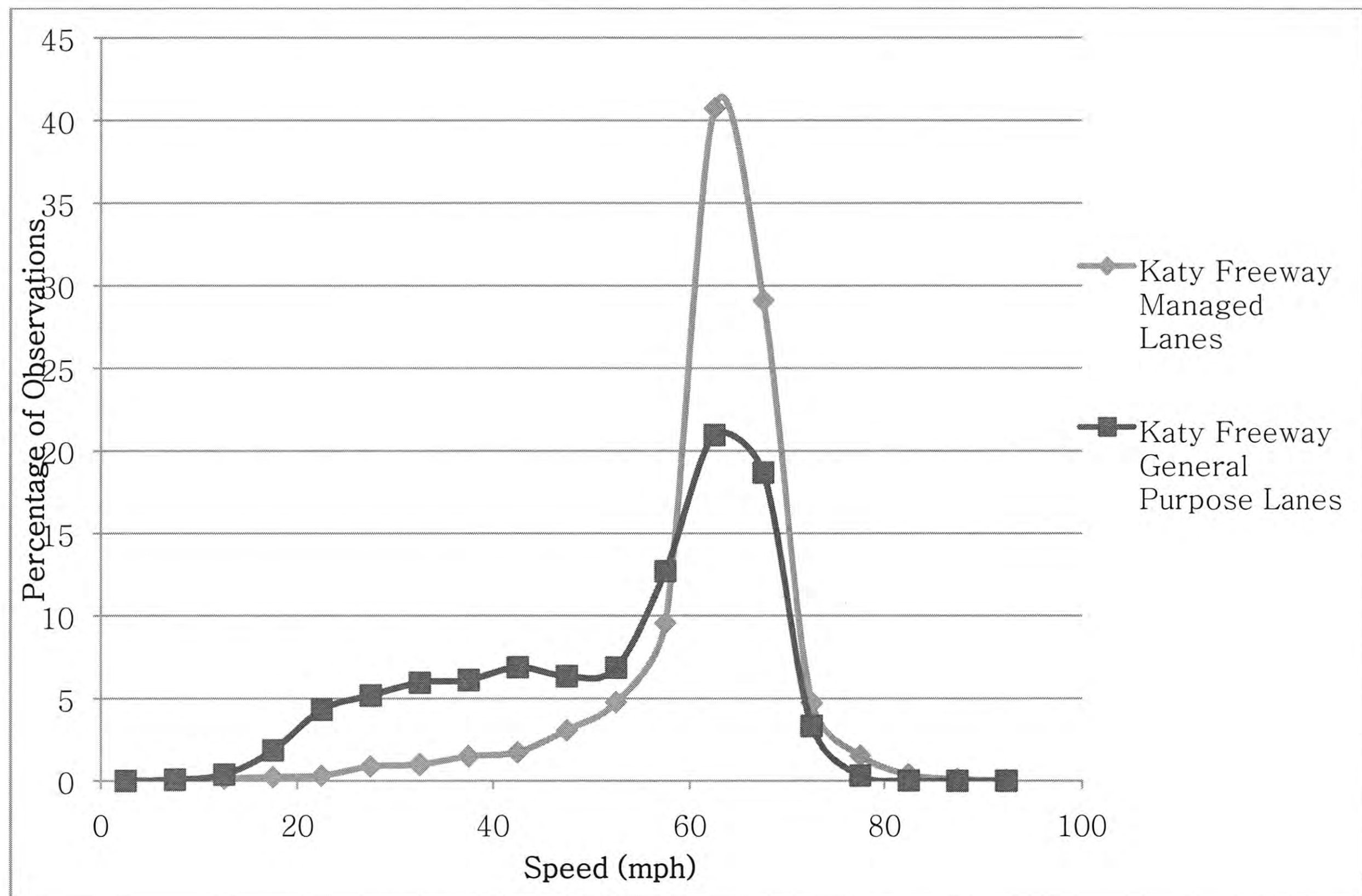
Figure 2: Speed Variation on Katy Freeway (Eastbound) during Peak Hours (7:00 AM to 9:00 AM)
