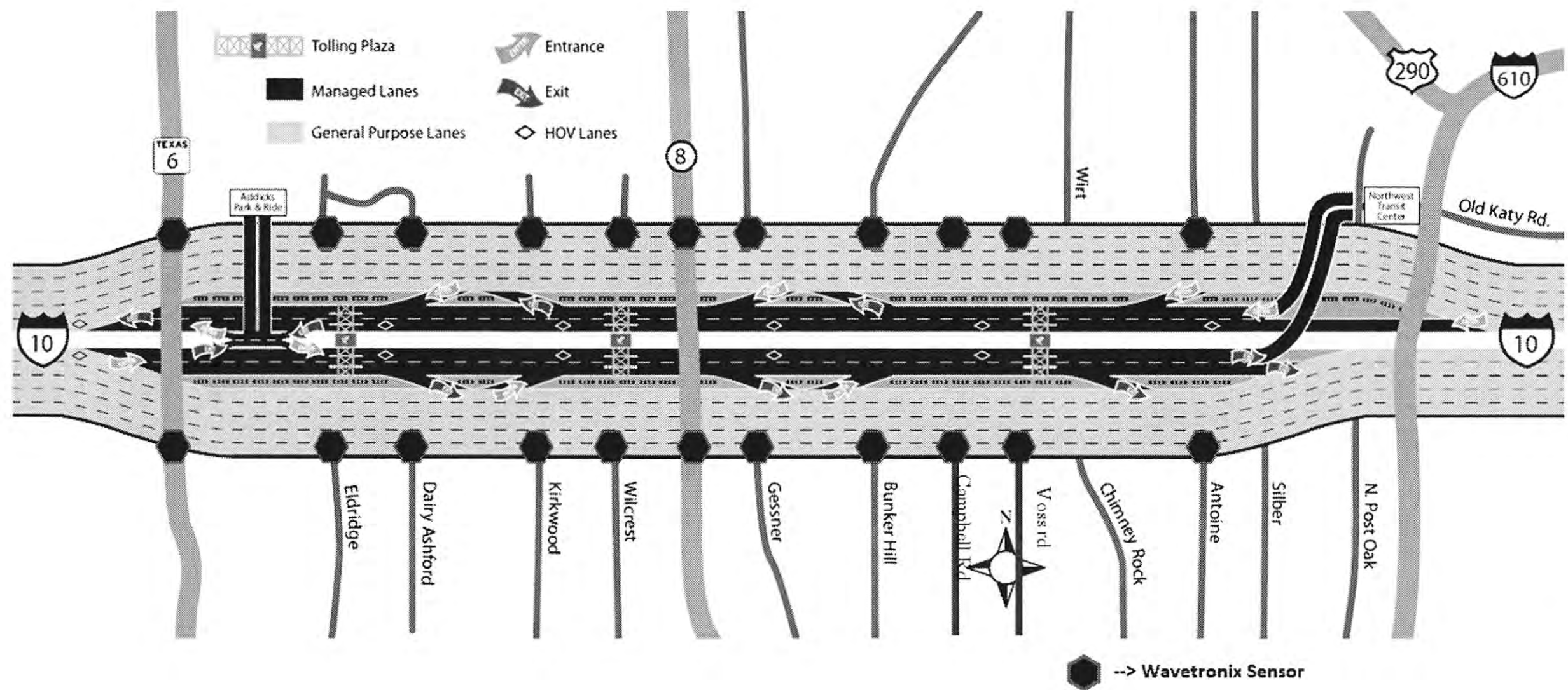
Figure 9: Wavetrax Sensor Locations on Katy Freeway
