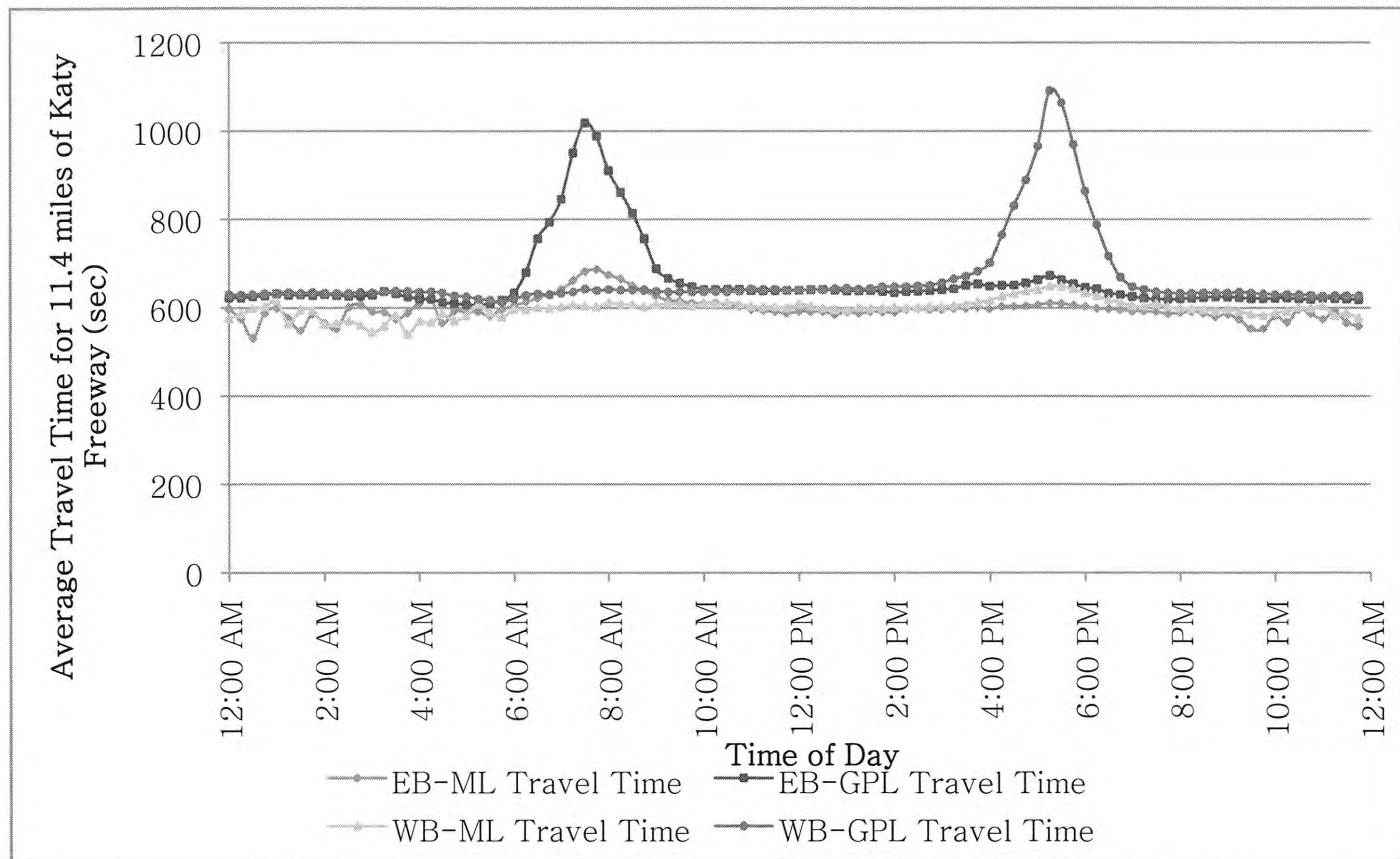
Figure 11: Average Travel Time for 11.4 Miles of Katy Freeway on the MLs and the GPLs by Time of Day
