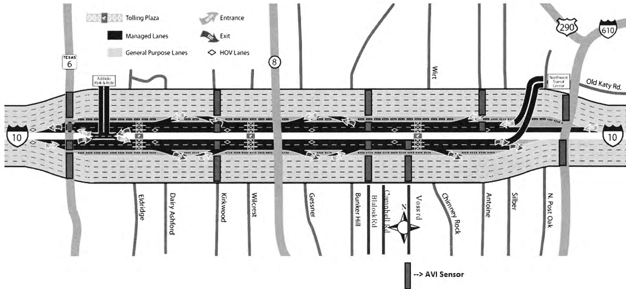
Figure 10: AVI Sensor Locations on Katy Freeway
