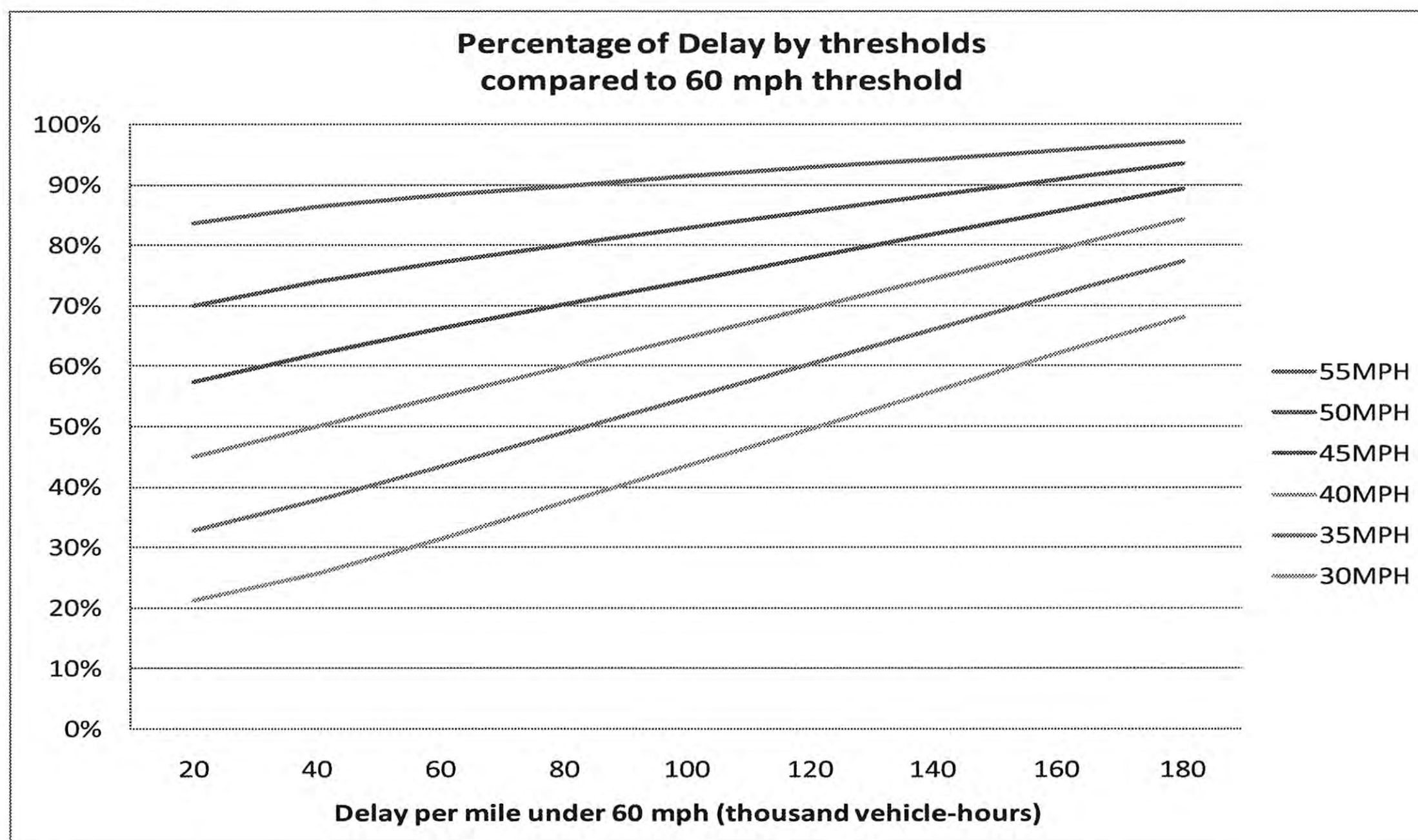
FIGURE 5.17 Percentage of delay per mile under an alternative threshold compared to the 60 mph.
