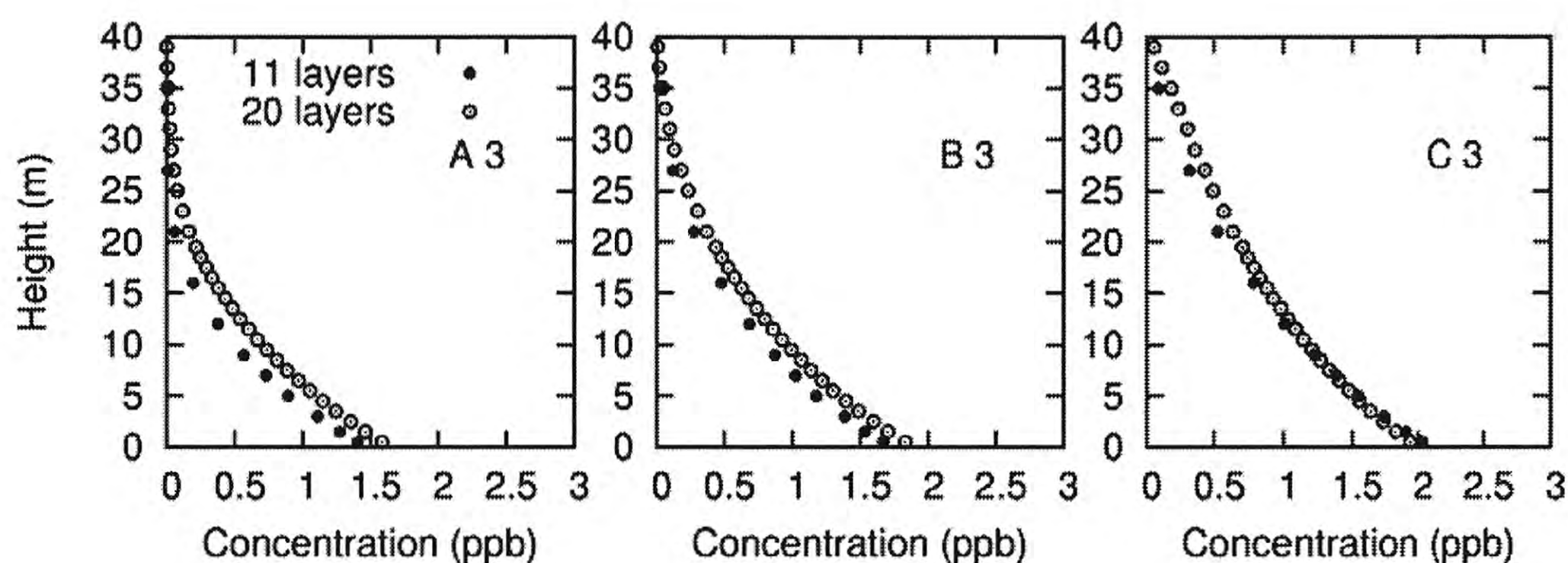
Figure 11. Comparison of the vertical SF 6 concentration profiles at tower 4 predicted by the base case model and the model with finer vertical resolution
