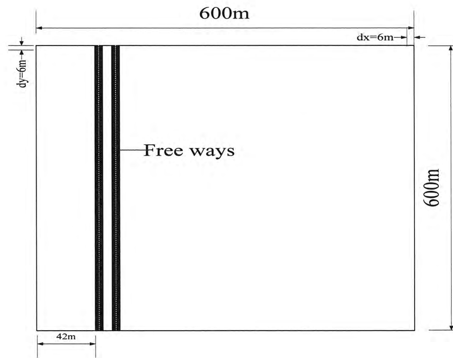
Figure 5. Model domain
