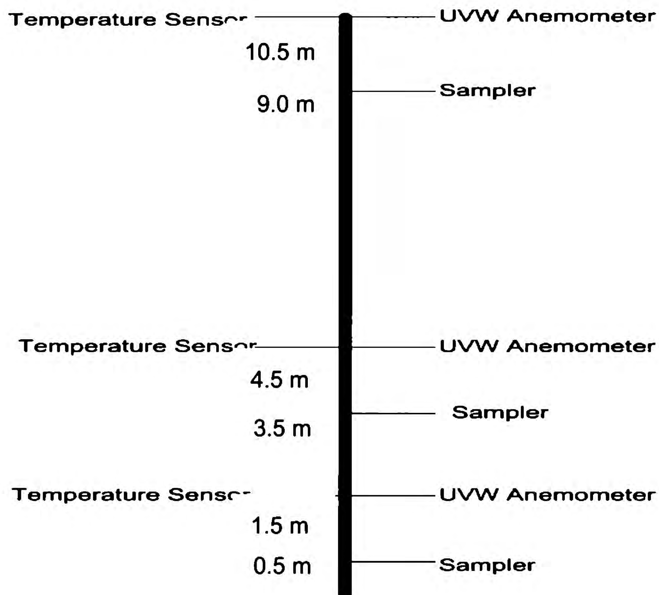
Figure 4. Schematic view of a tower
