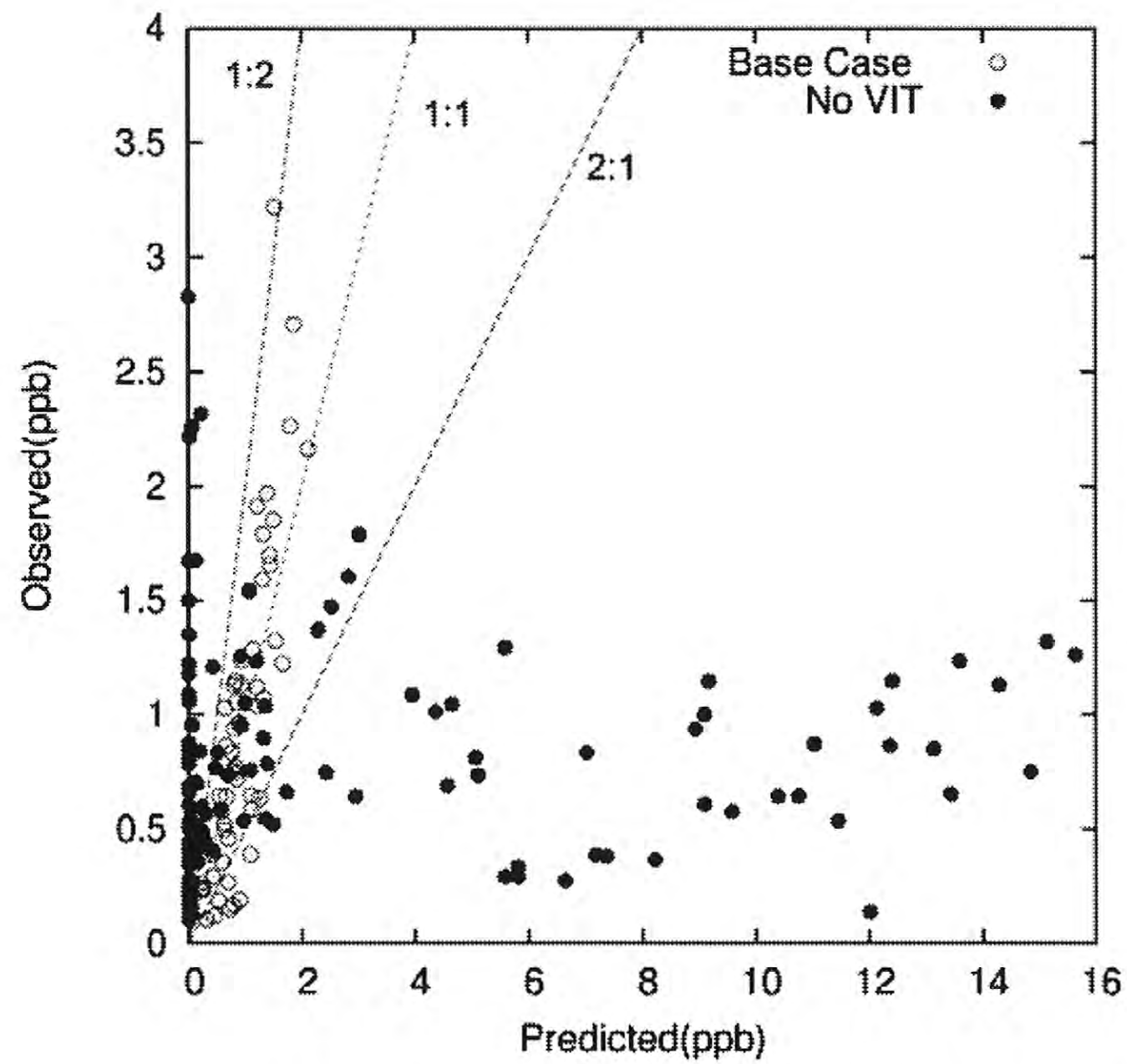
Figure 8. Predicted SF 6 concentrations compared with observations
