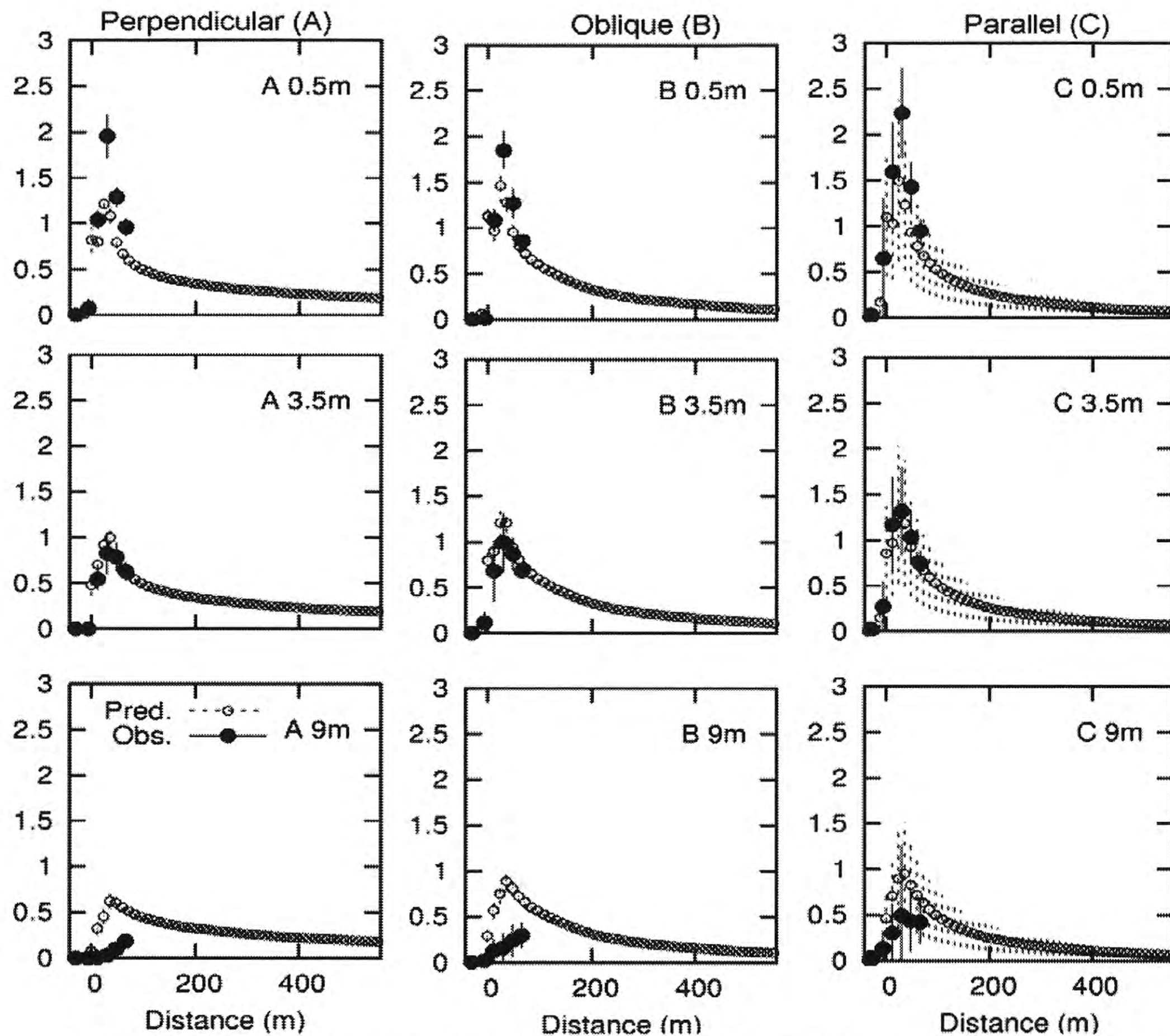
Figure 7. Observed and predicted spatial distribution of SF 6 concentrations (ppb)
