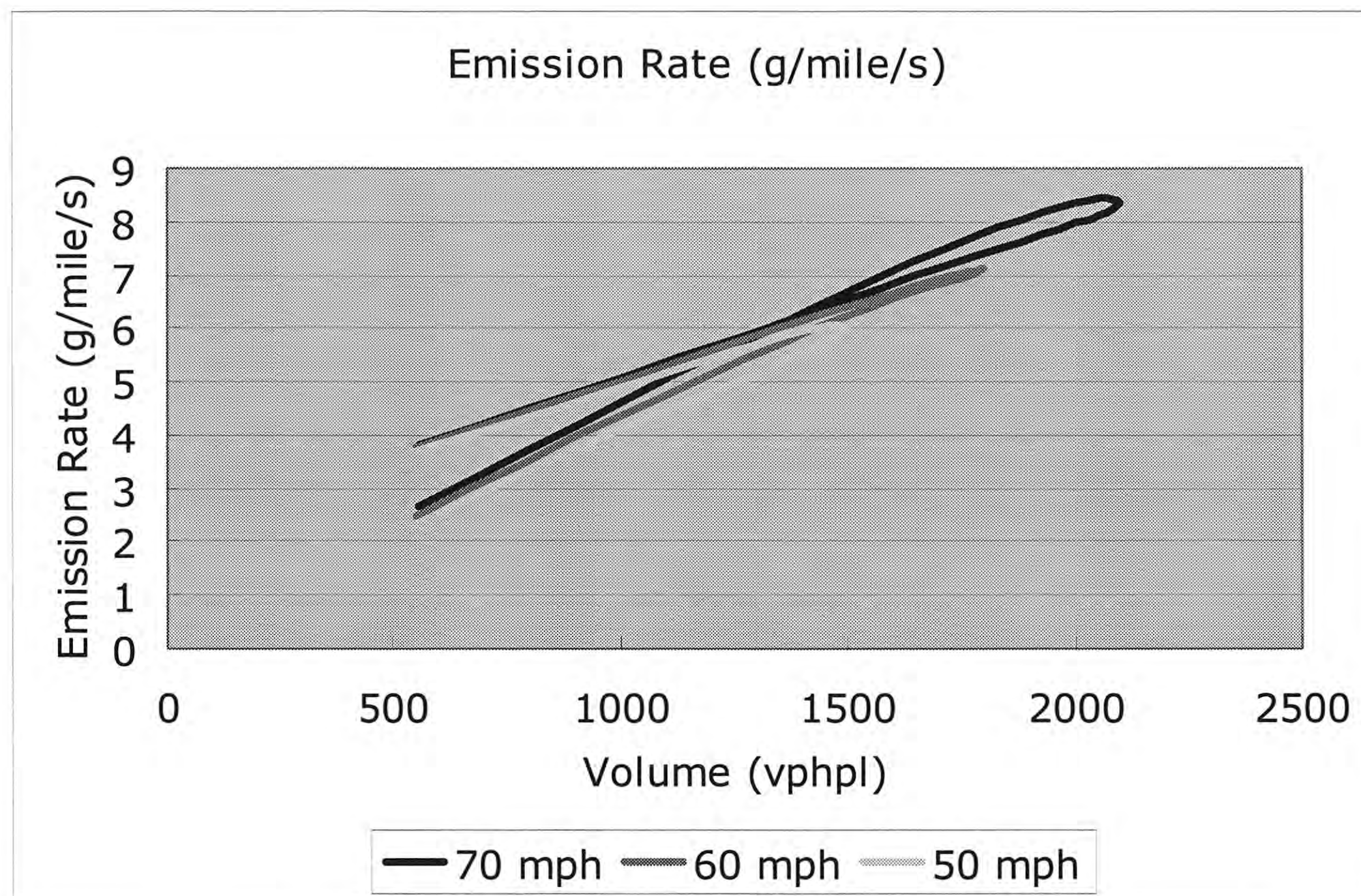
Figure 21. Relationship between volume and emission rate
