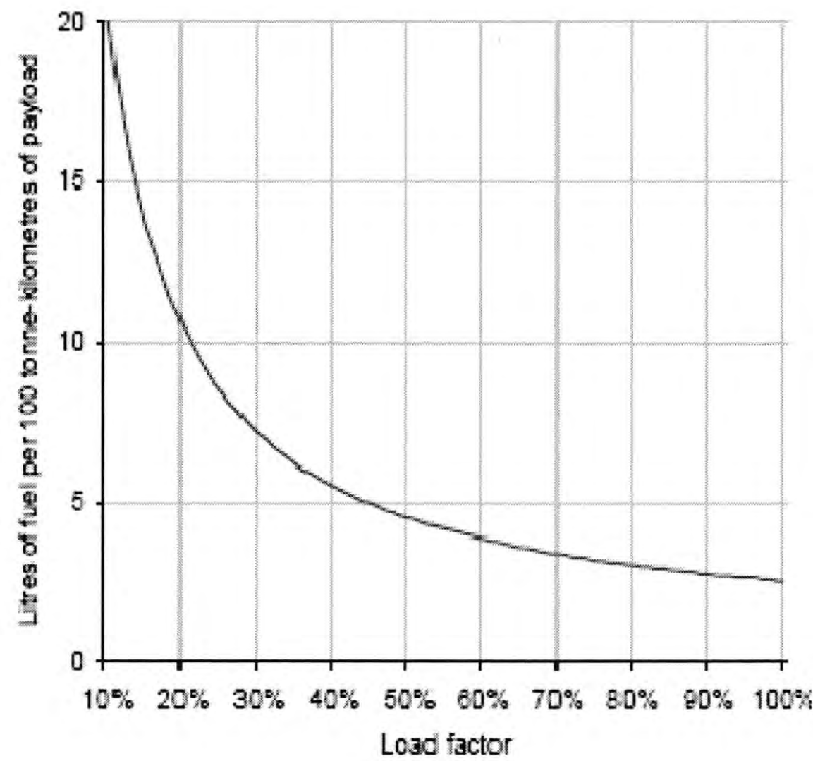
Figure 6: Relationship Between Payload and Fuel Consumption (Source: Gilbert, 2004)
