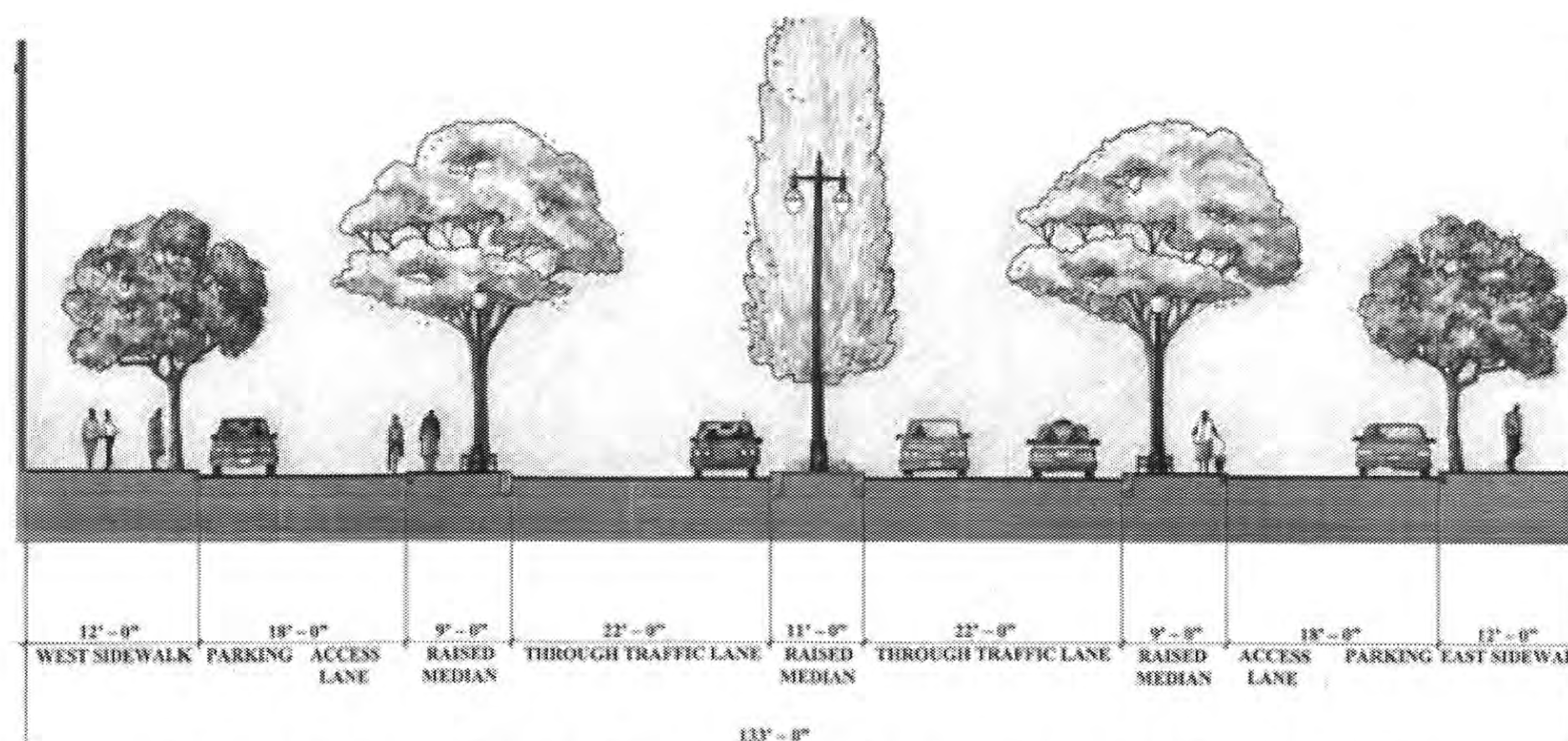
Figure 59. A Typical Cross-Section of Octavia Boulevard.
