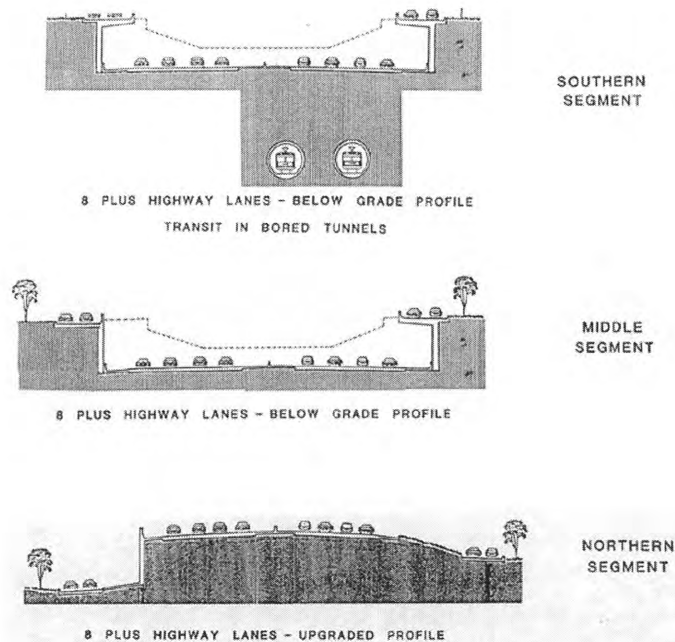
Figure 5. Typical Cross-Sections of the NC Expressway Segments.
