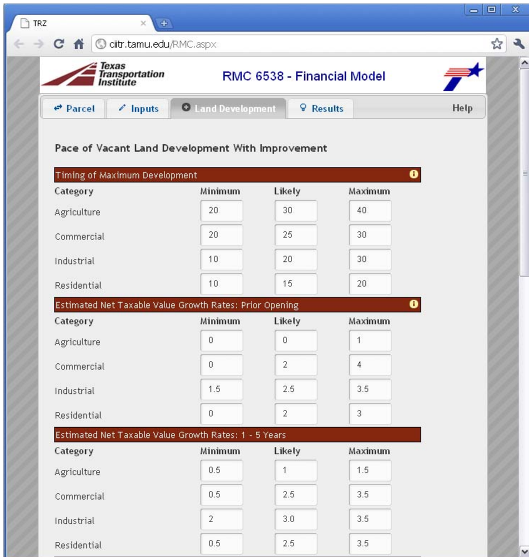
Figure 6.7. Illustration of the Input Variables that Use Triangular Distribution.
