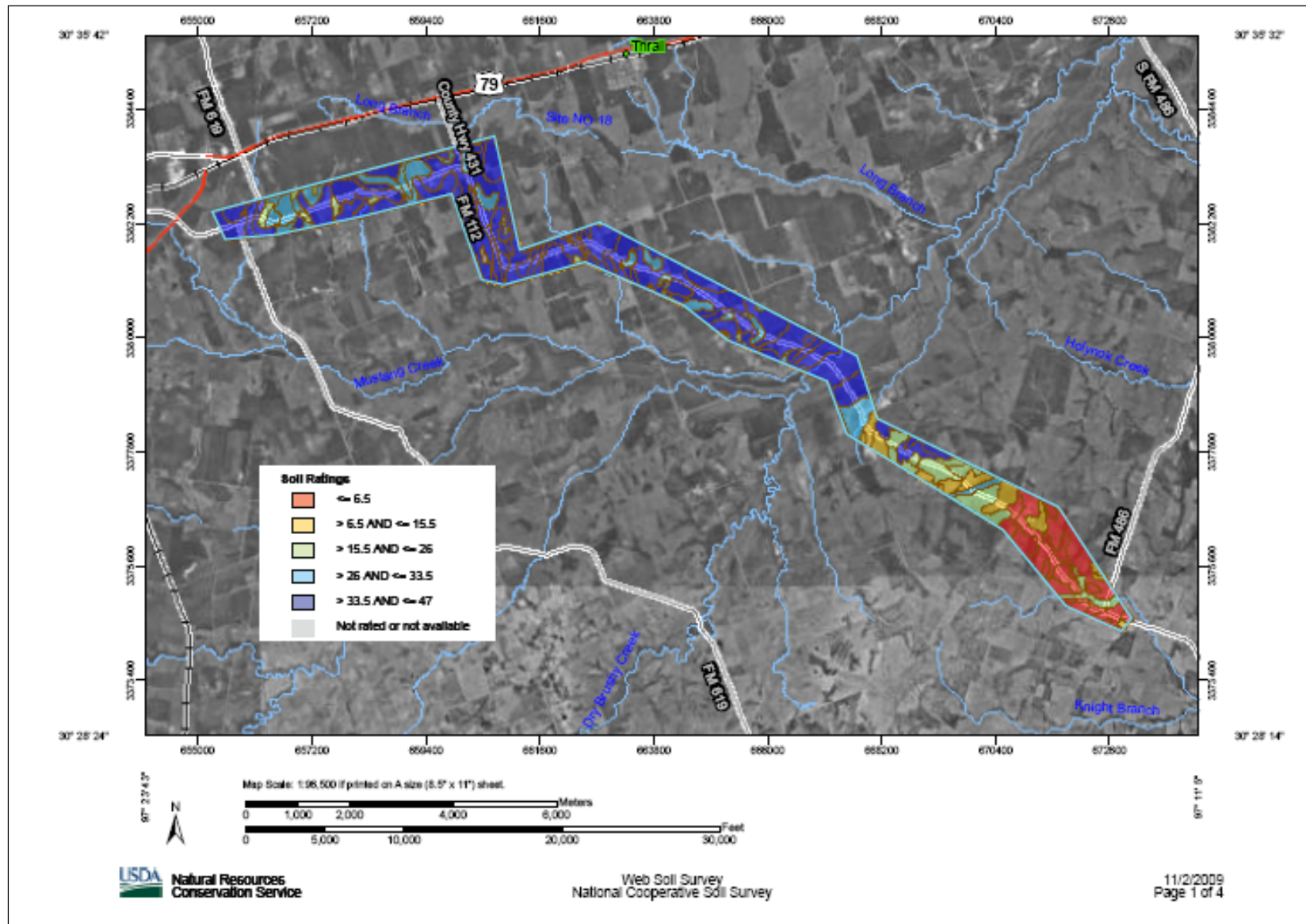
Figure 4.2. Surface Soil Plasticity Index on FM 112.
