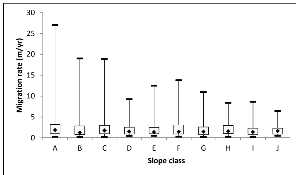
Figure 26. Boxplot for total migration values for each slope class. The dot in the center of each rectangle represents the mean value for each time period. The upper and lower edges of the rectangle represent the 25 th and 75 th percentiles, respectively. The upper and lower bars are the highest and lowest values for a given time period.
