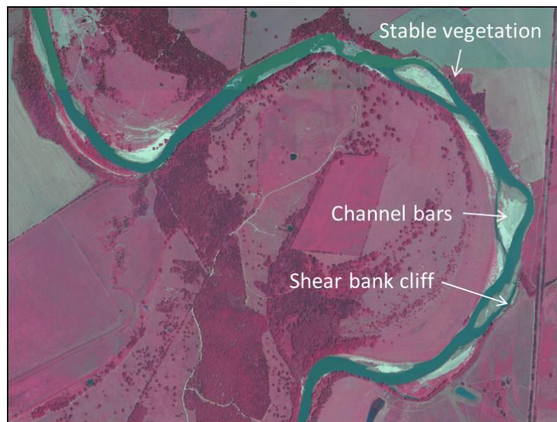
Figure 18. Typical large meander bend displaying stable outer banks, with vegetation, in upstream and relatively unstable outer downstream outer banks. Scale is 1:14,500. (Photograph is 2004 NAIP image).
