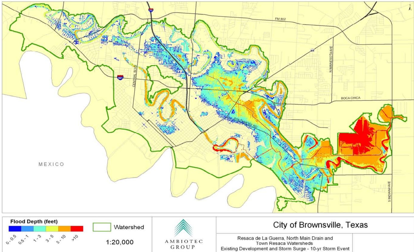
Figure 5-7. Floodplain for the merged model (RDLG, NMD, and TR watersheds) under extreme storm surge conditions (28-ft) assuming a 10-yr design rainfall total of 7.48 inches over a 24-hr period over the entire watershed area
