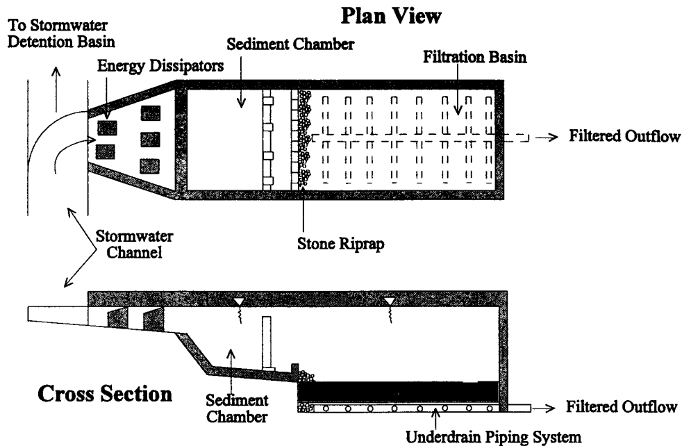
Figure 3-4 Schematic of a Sand Filter System (Young et al., 1996)
