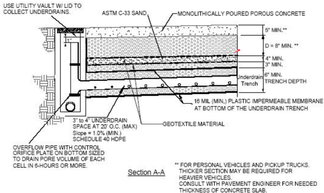
Figure 3-32 Schematic of Permeable Concrete Installation (after UCFCD, 2004)
