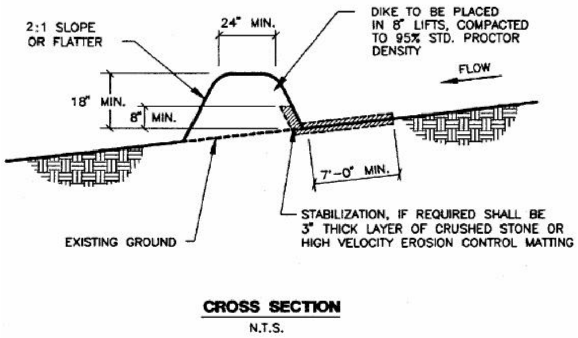
Figure 1-8 Schematic of a Diversion Dike (NCTCOG, 1993b)
