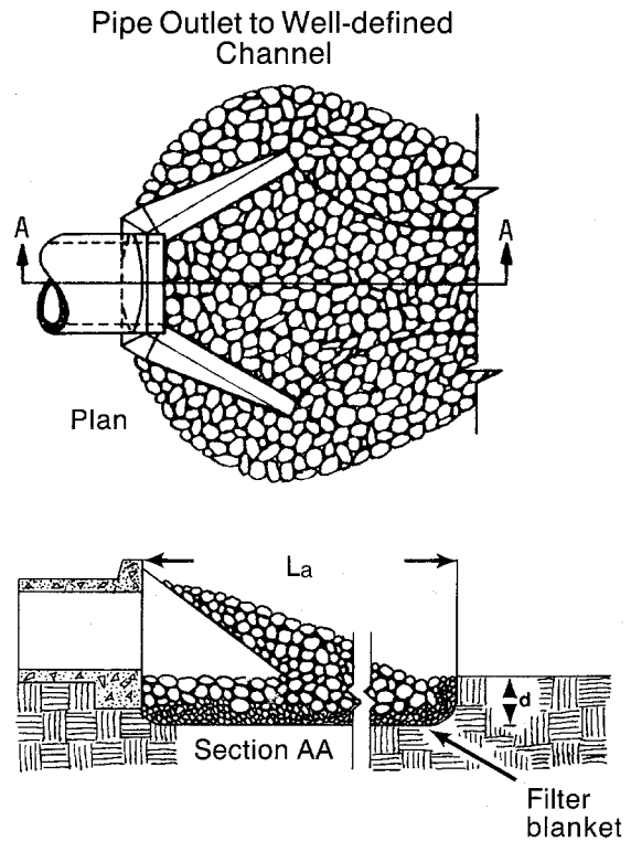
Figure 1-11 Riprap Outlet Design (North Carolina, 1993)
