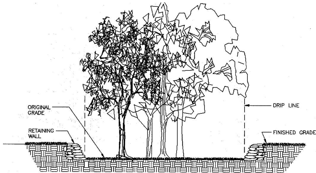
Figure 2-2 Example of a Tree Well (VA Dept of Conservation, 1992)
