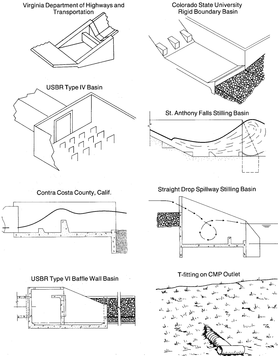
Figure 1-10 Examples of Stilling Basin Designs (North Carolina, 1993)
