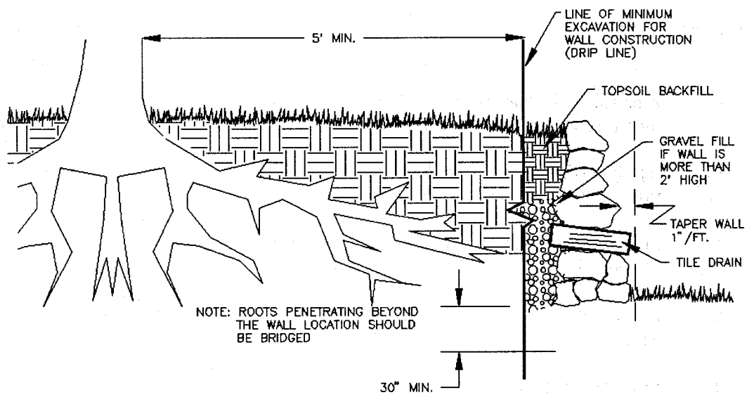
Figure 2-4 Example of a Tree Wall (VA Dept of Conservation, 1992)
