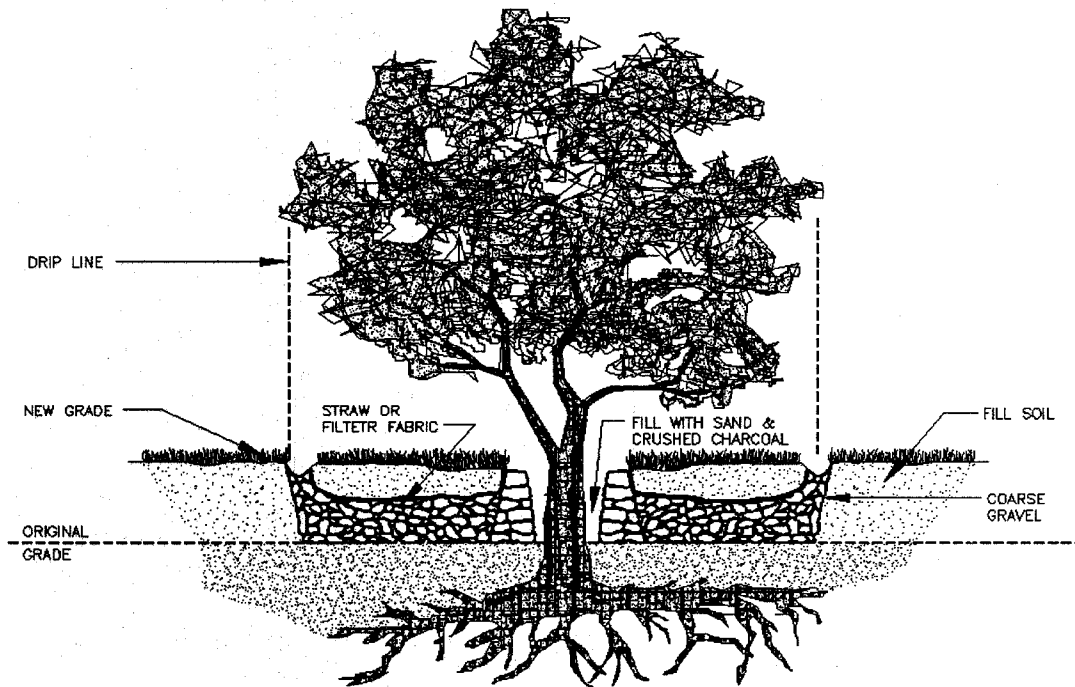
Figure 2-3 Tree Well with Higher Finished Grade (VA Dept of Conservation, 1992)
