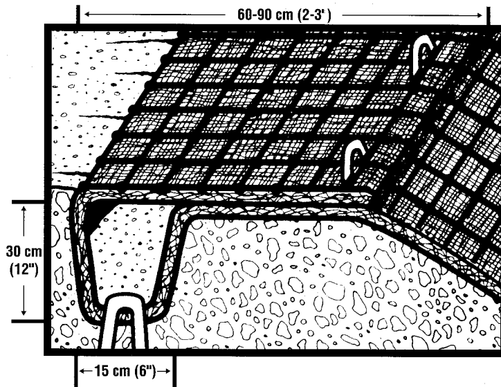
Figure 1-21 Terminal Anchor Trench for Blankets and Mats
