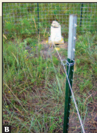
A board is used as a prop on a swing gate (A). T-posts guide the wire from the prop to the back of the trap (B). The wire is then attached to another wire forming a T-intersection at the trigger point (C). As the hogs feed on the bait, the wire is stretched, and the prop pulls from the gate. (Source: Greg Pleasant).
