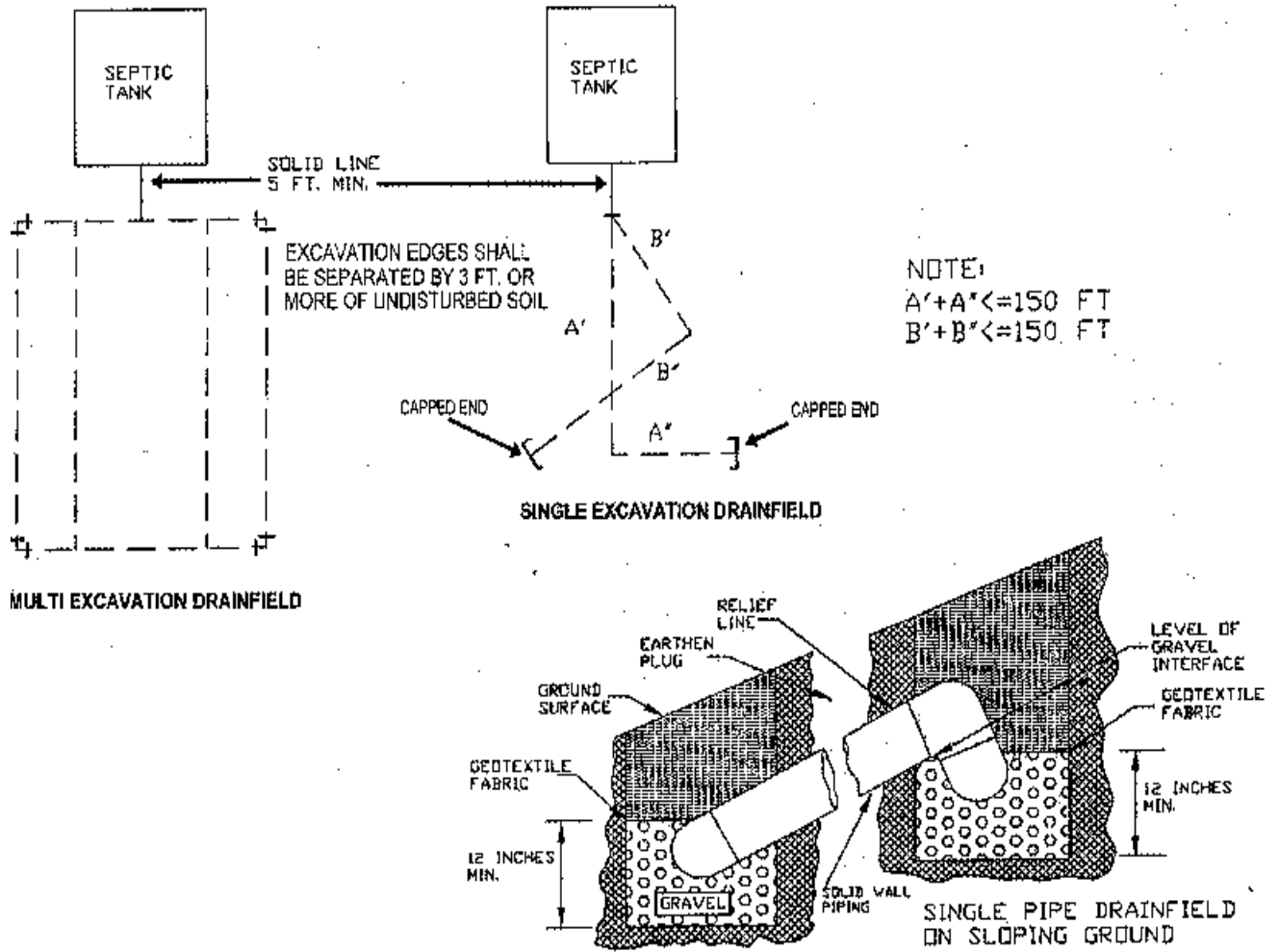
(5) Figure 5. Typical Drainfields.
