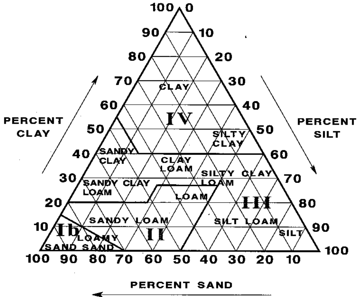
(6) Table VI. USDA Soil Textural Classifications.
