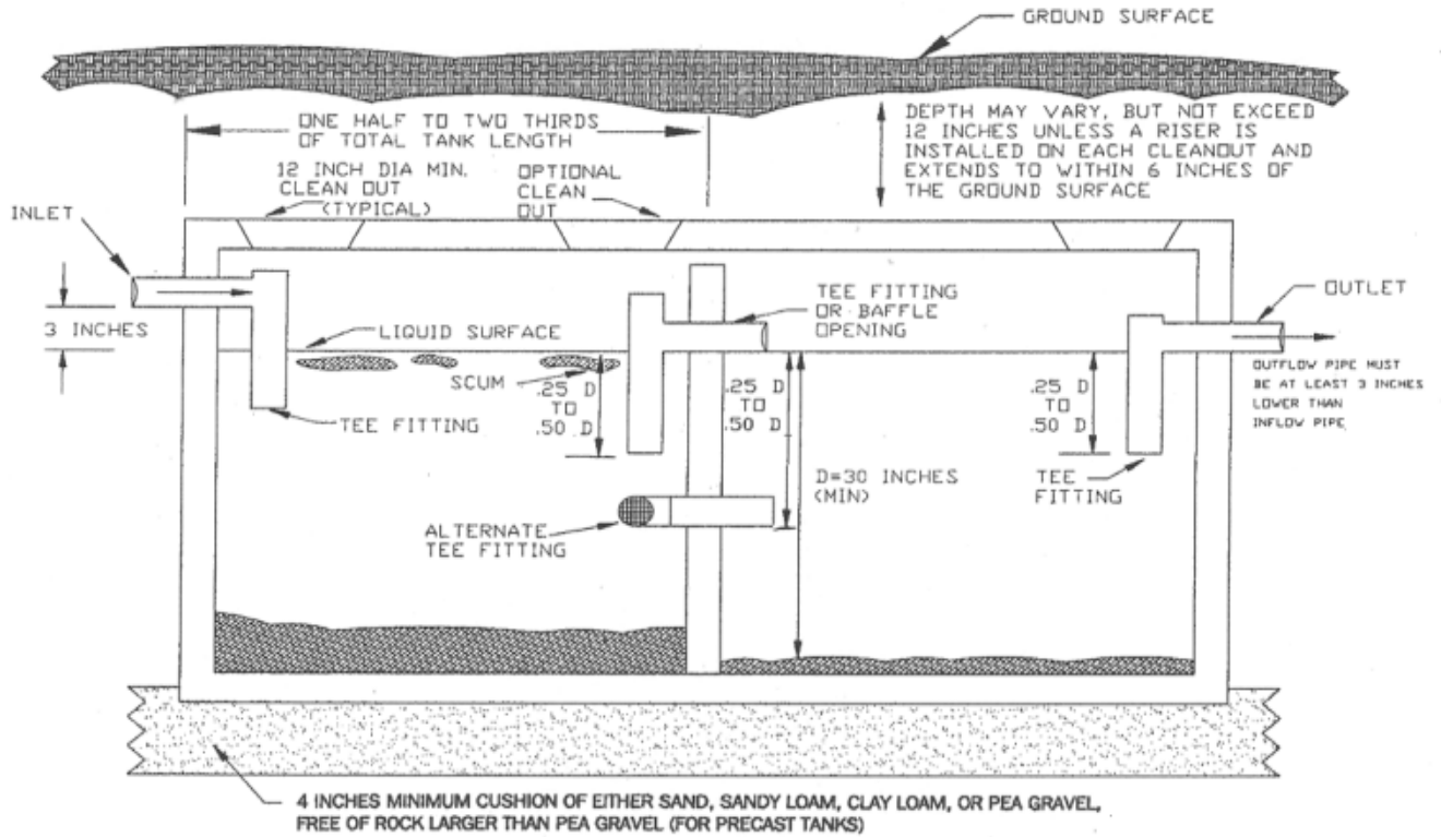
(6) Figure 6. Two Compartment Septic Tank.
