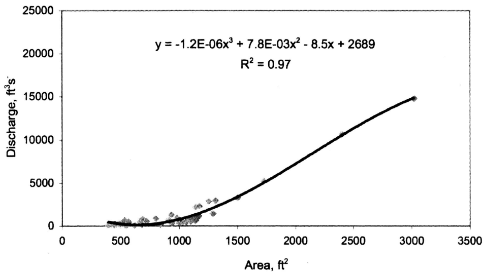
Figure 10. Relation between discharge and flow area
