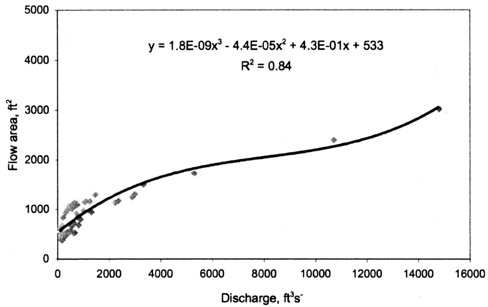
Figure 8. Relation between flow area and discharge
