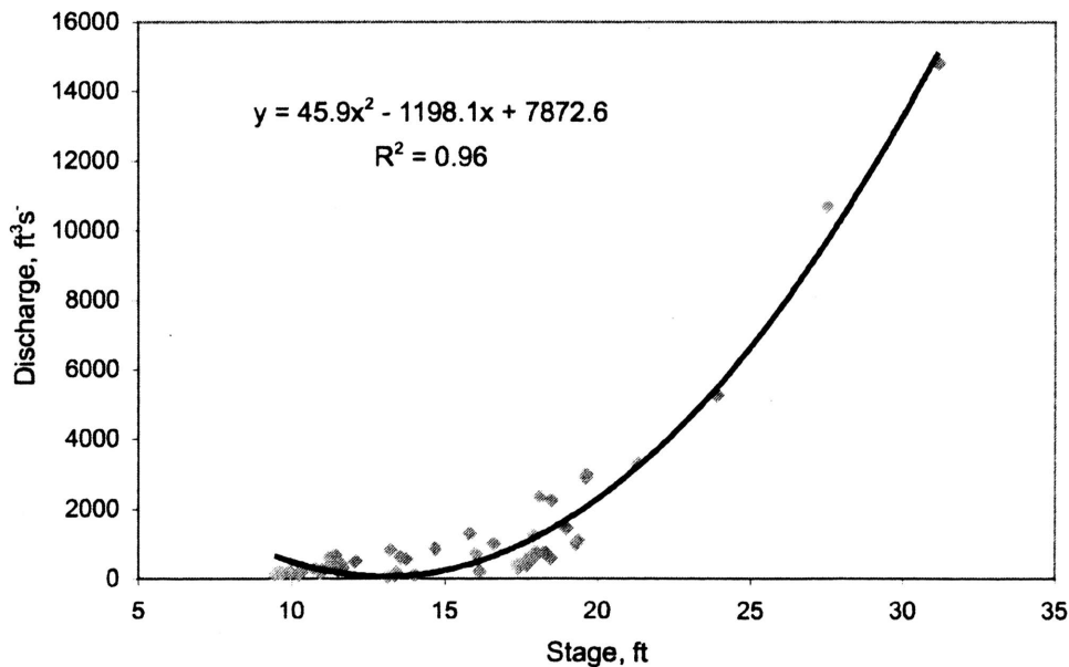
Figure 7. Discharge-stage rating relation.
