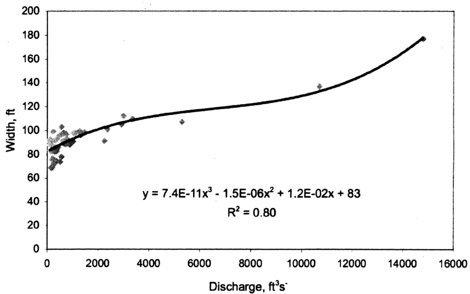
Figure 9. Relation between flow width and discharge
