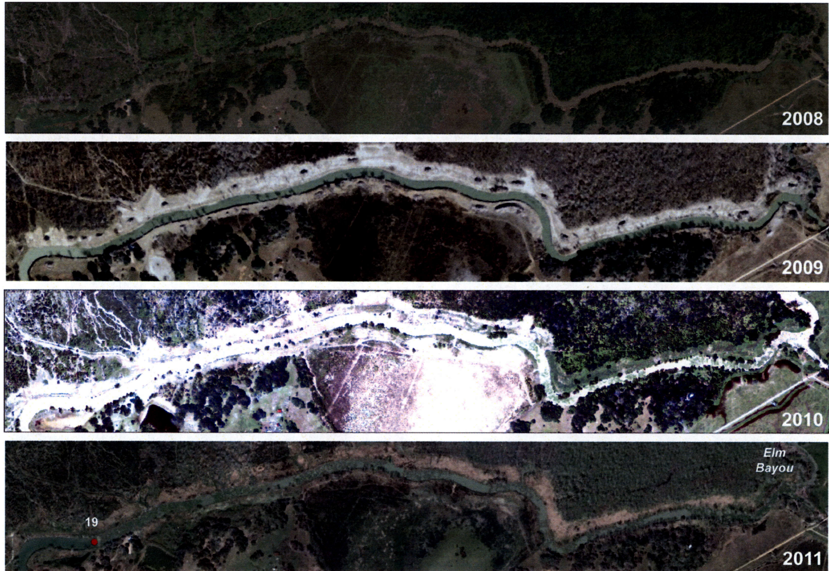
Figure 6. Accumulation of large woody debris in subreach 19. Flow direction is from left to right. The upstream limit of the subreach is indicated by numbered circle on the 2011 image.
