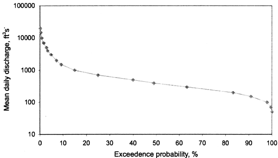
Figure 11. Flow duration curve for the McFaddin gauge.
