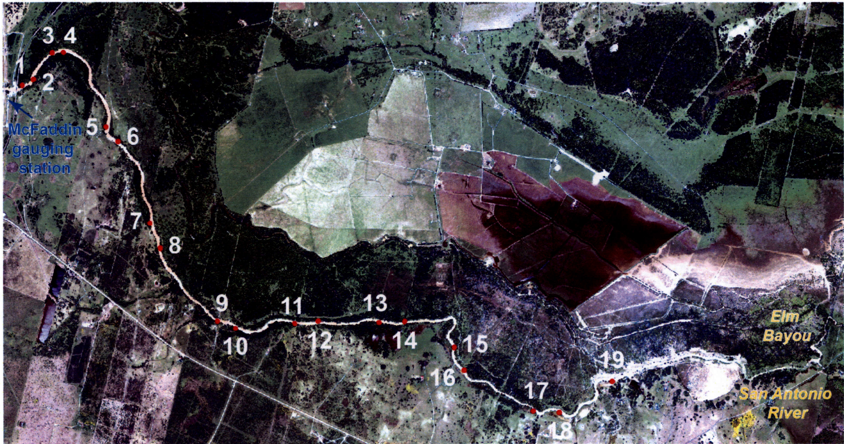
Figure 1. The lower reach of the San Antonio River. Flow direction is from left to right. Circles show the midpoint of subreaches used in the study except for the most downstream symbol that indicates the upstream limit of the last subreach. The far left boundary is defined by State Highway 77 where streamflow gauging station is located.
