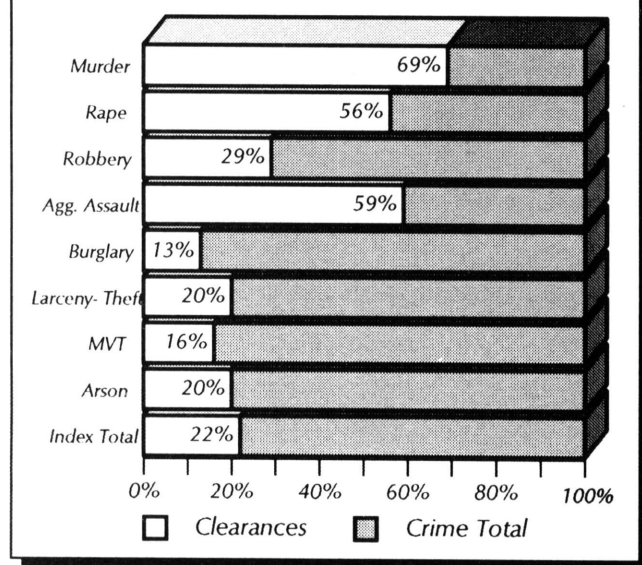
Index Crime Clearance Rates
