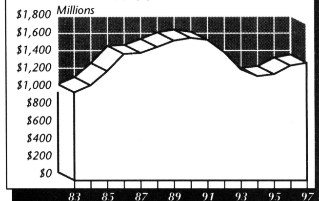
Property Value Lost to Crime 1983 - 1997
