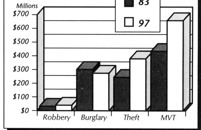
Property Value Lost to Crime 1983 and 1997
