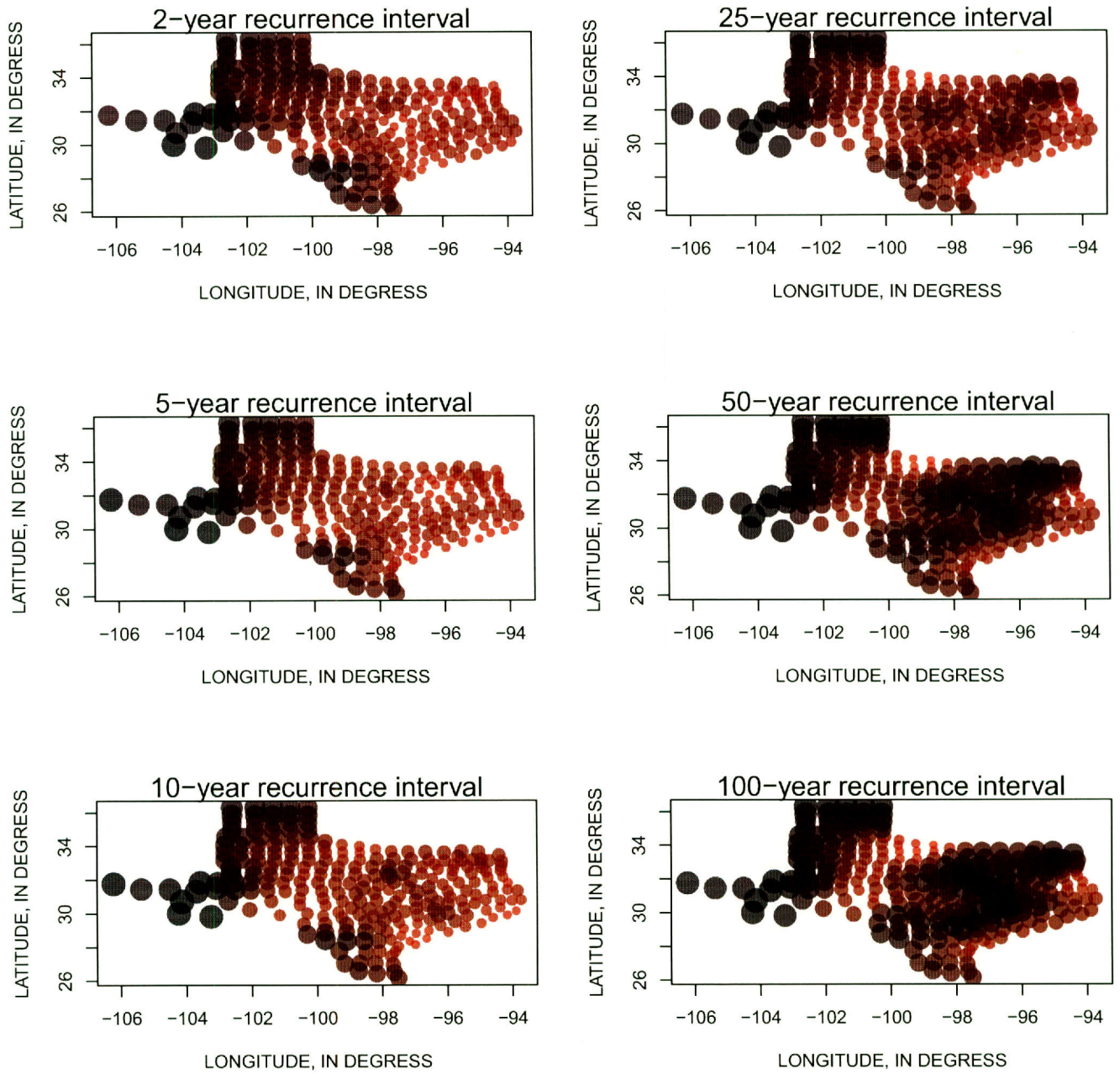
Figure 3.3: Exponent on dimensionless main-channel slope for unified rational method in Texas. Increasing size and hue towards black indicates relatively higher values.
