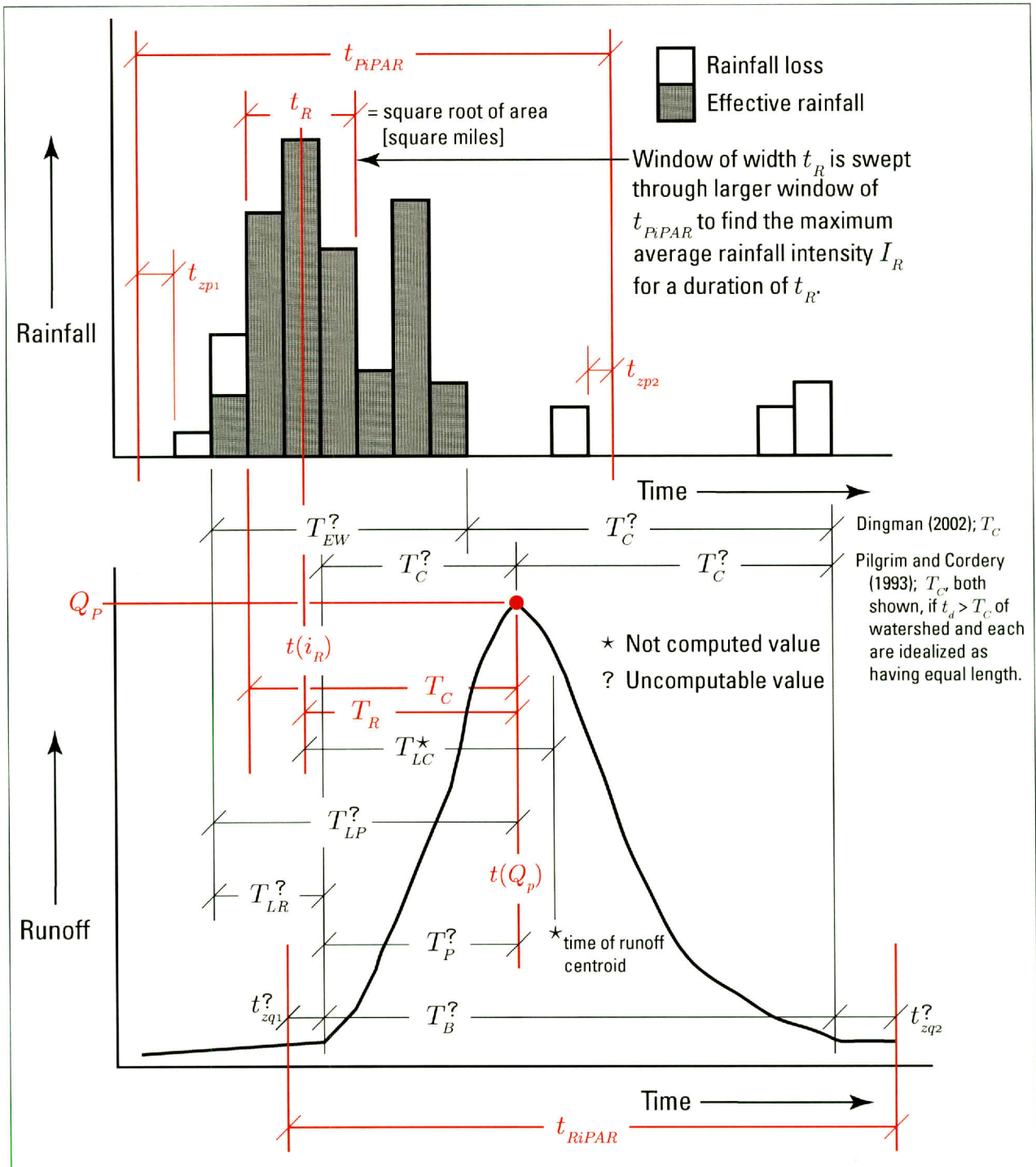
Figure C.1: Overview of the rainfall- and runoff-parsing process using the iPAR program inclusive of definitions of selected metrics and computational versus conceptual availability with a specific focus on the square-root-of-area rule for first order estimation of time of concentration.
