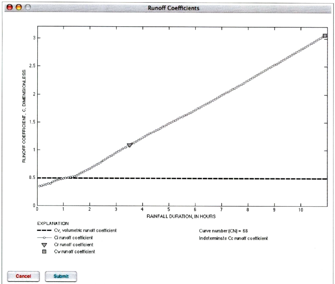
Figure C.3: Screenshot of output for parsed storm in Figure C.2 that shows the relation between runoff coefficient of rational method computed in hind-casting mode and rainfall duration (characteristic time) for each successively-incremented and aggregated, 5-minute window, which has been slid through the parsed rainfall (white window in top plot of figure C.2) to determine maximum rainfall intensity for indicated duration. Notice that runoff coefficient increases as duration increases. Of particular interest for this study are the volumetric runoff coefficient (dashed line) and the runoff coefficient C_R(t_R) based on t_R = \sqrt{A[\text{sqmi}]} (square-root-of-area rule; sqmi, square miles). For this parsed event, C_V = 0.49 , C_R = 1.09 , T_R = 2.21 hours (Time-R, lag time, a time not shown on the plot).
