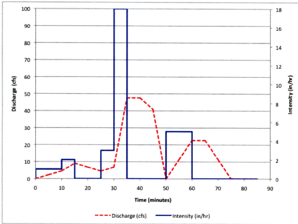
Figure 4.8: Modified rational method runoff hydrograph for example drainage area. Applied storm is non-uniform. Watershed characteristic time increased to T^* = 15 minutes. Q_p = 47.6 cfs at 35 minutes.
