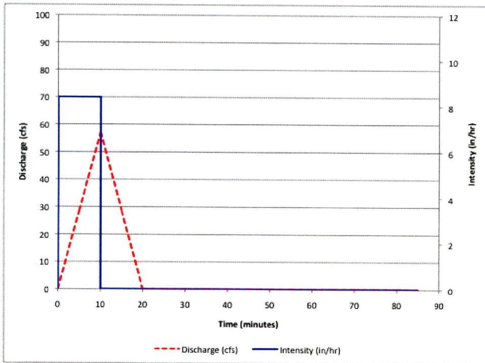
Figure 4.4: Modified rational method runoff hydrograph for example drainage area. Applied storm duration is equal to the watershed characteristic time T^* = 10 minutes. The peak discharge is Q_p = 57.1 cfs; the same as the URAT peak estimate.
