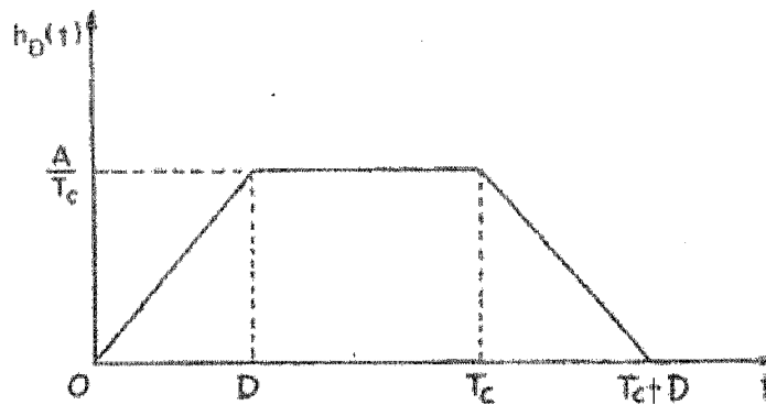
Figure 2.5: The D -hour unit hydrograph of the rational method for D < T_c (Singh and Cruise, 1992).
