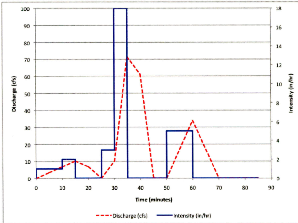
Figure 4.7: Modified rational method runoff hydrograph for example drainage area. Applied storm is non-uniform. Q_p = 71.4 cfs at 35 minutes.
