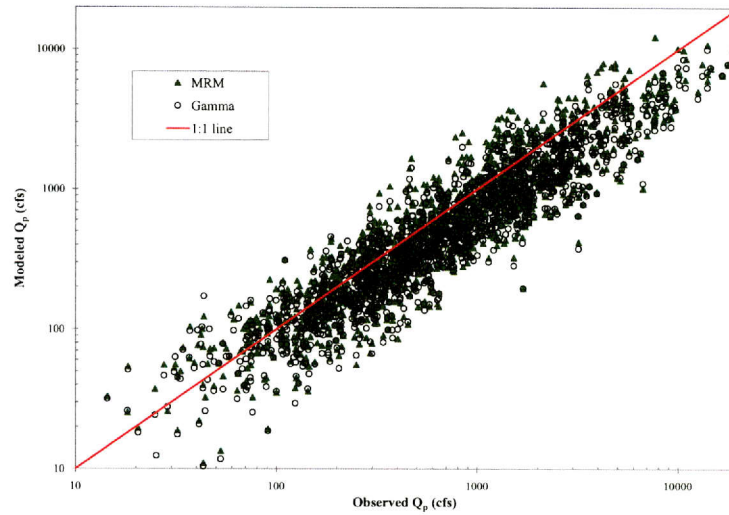
Figure D.12: Modeled and observed peak discharge from modified rational method (green) and gamma unit hydrograph method (black).
