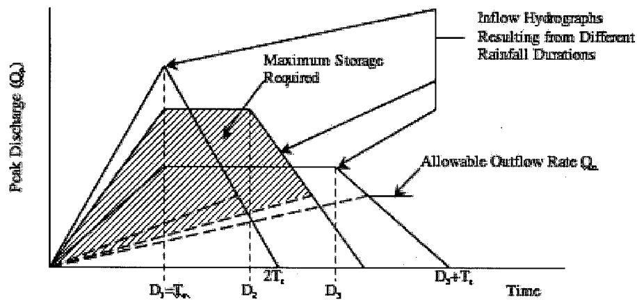
Figure A.3: Modified Rational Formula Hydrographs by Aron and Kibler (1990). Adapted from Thompson (2006).
