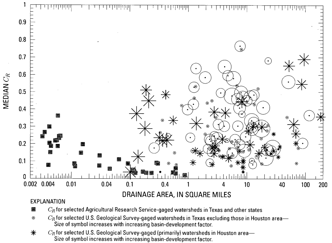
Figure C.6: Relation between C_R and drainage area and basin-development factor ( BDF ) by watershed type for median observed values.
