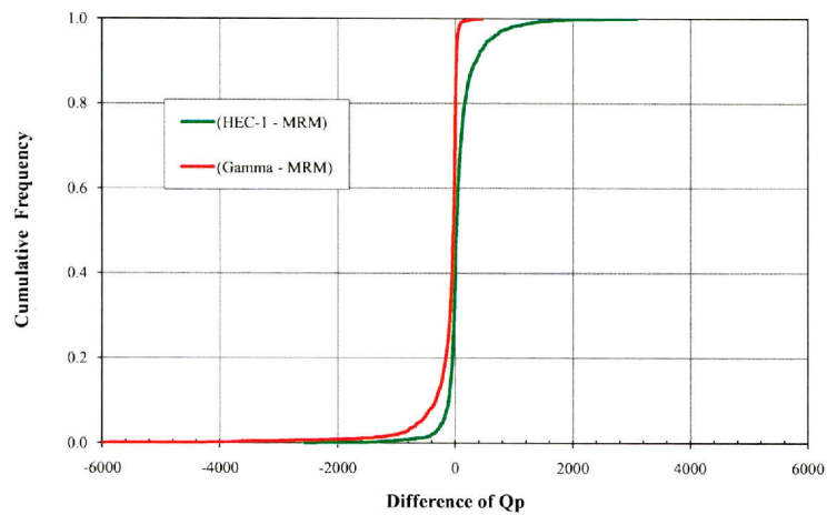
Figure D.13: Cumulative distributions of differences of simulated Q_p between different methods. The green curve is for differences of simulated Q_p between Clark and MRM unit hydrographs, and the red curve is for differences of simulated Q_p between gamma and MRM unit hydrographs.
