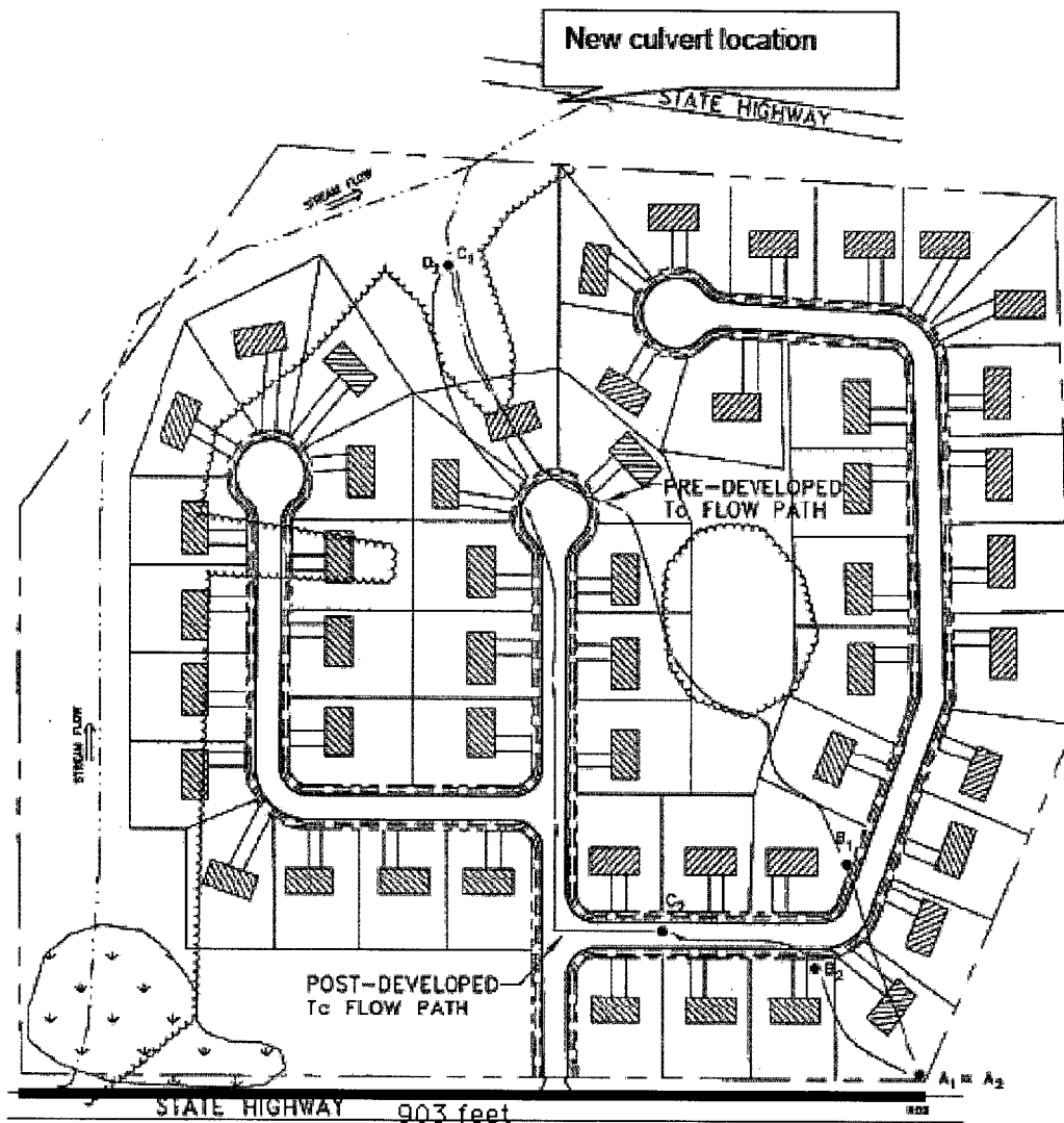
Figure 4.1: Subdivision X Drainage to a Highway Culvert
