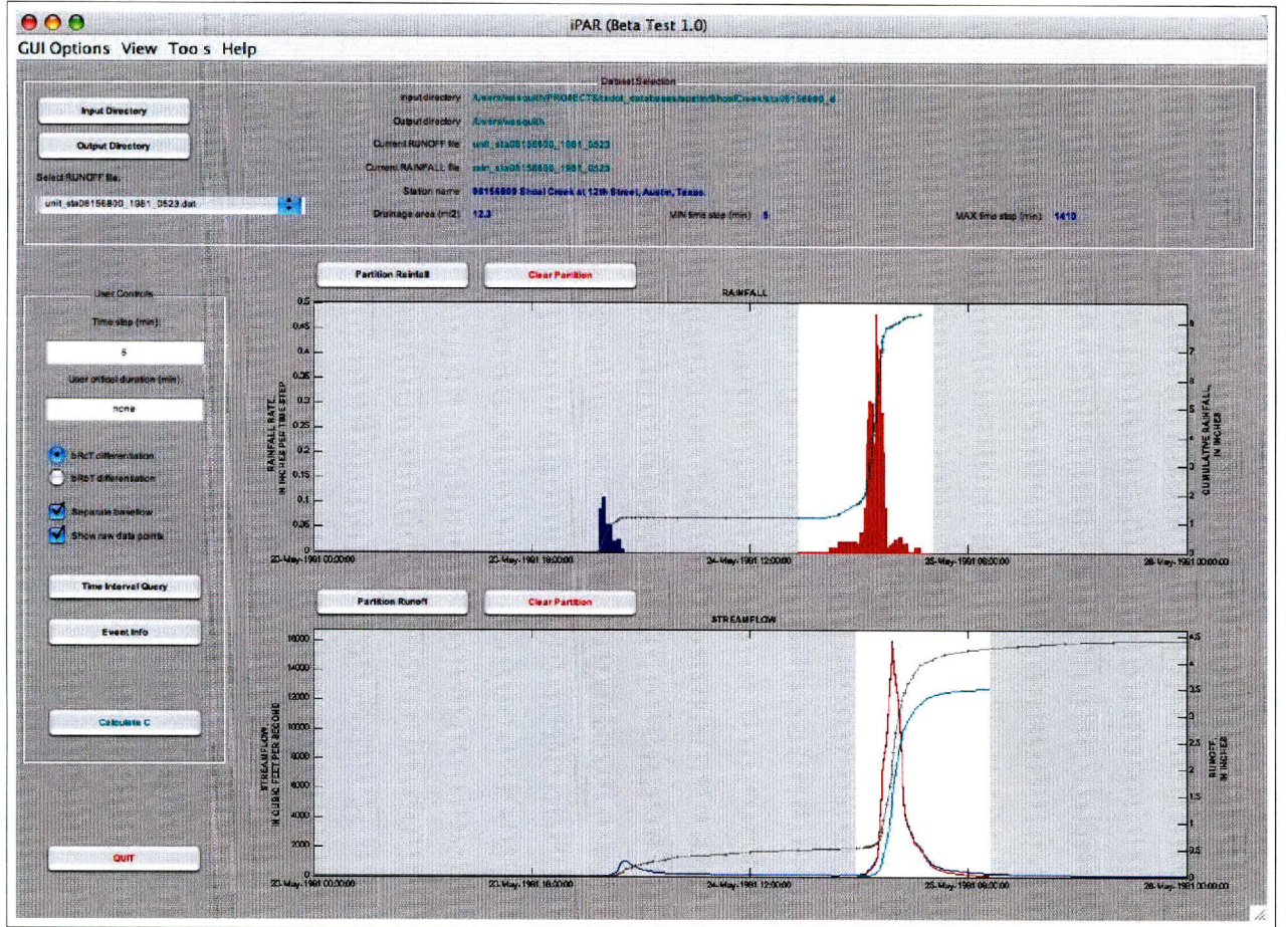
Figure C.2: Screenshot of custom-built iPAR program used to parse a historically significant flood event at U.S. Geological Survey streamflow-gaging station 08156800 Shoal Creek at 12th Street, Austin, Texas, May 24, 1981, which has a drainage area of about 12.3 square miles. The top plot shows the incremental rainfall and the bottom plot shows the resultant runoff hydrograph.
