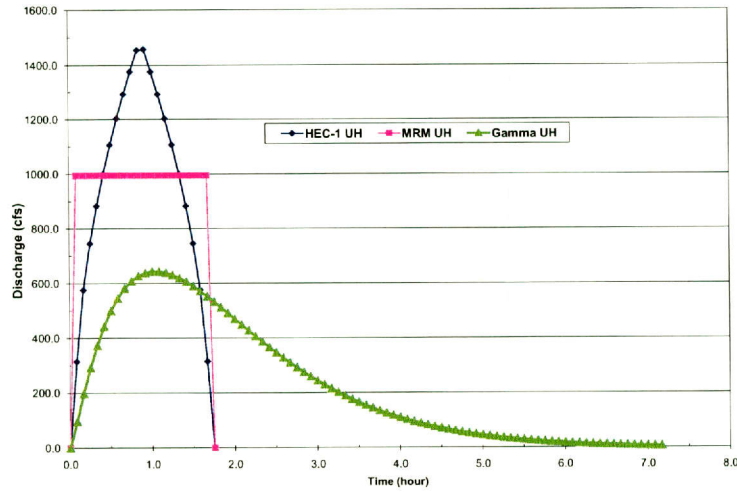
Figure D.8: Unit hydrographs for USGS Streamflow-gaging Station 08048600. The unit hydrographs are: MRM (pink), gamma (green) and Clark (blue).
