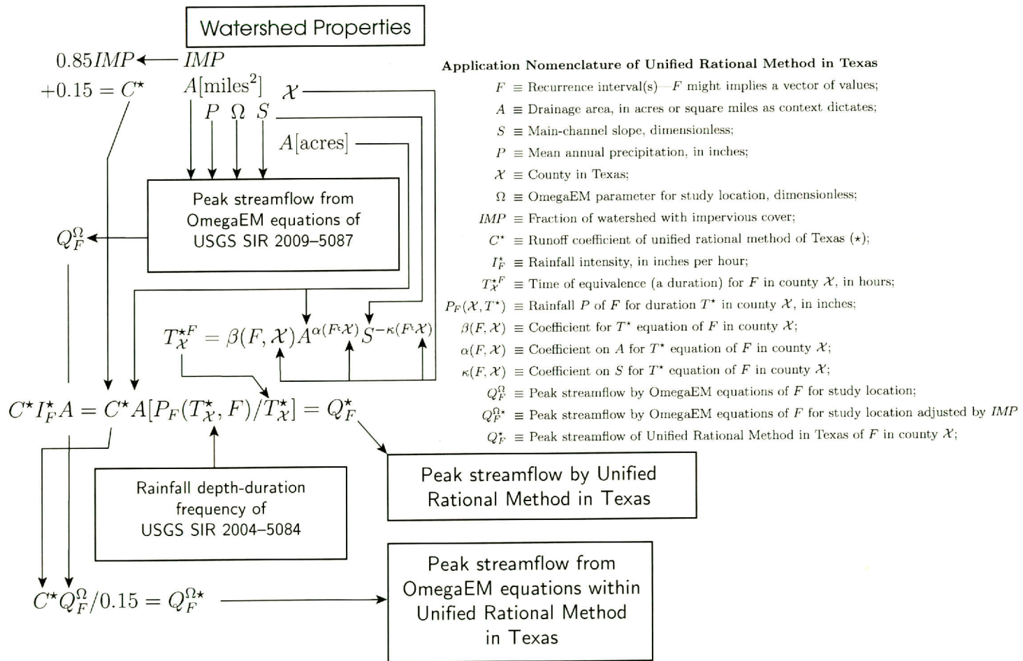
Figure 4.9: Flowchart of application of Unified Rational Method for Texas.
