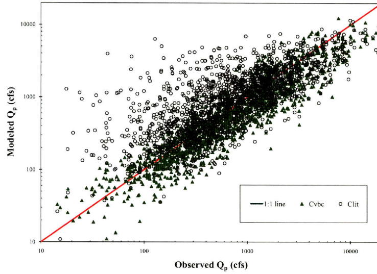
Figure D.5: Modeled and observed peak discharge from C_v^{bc} (green) and C_v^{lit} (black) with timing parameters derived from the Kerby-Kirpich method.
