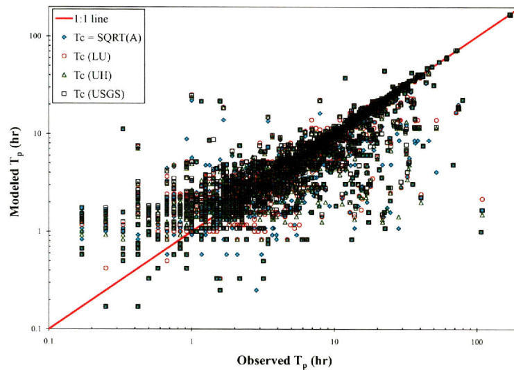
Figure D.3: Modeled and observed time to peak for C_v^{bc} and different timing parameters.
