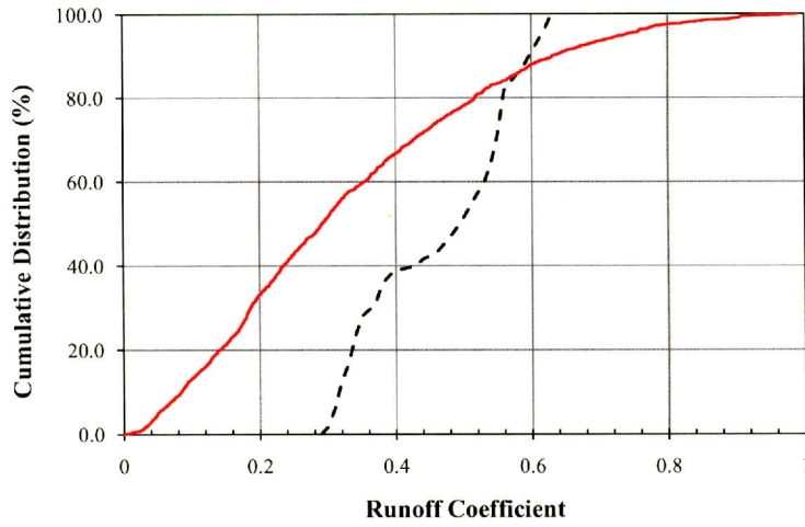
Figure 2.6: Cumulative distributions of the runoff coefficients C_v^{bc} (solid) and C_v^{lit} (dashed).
