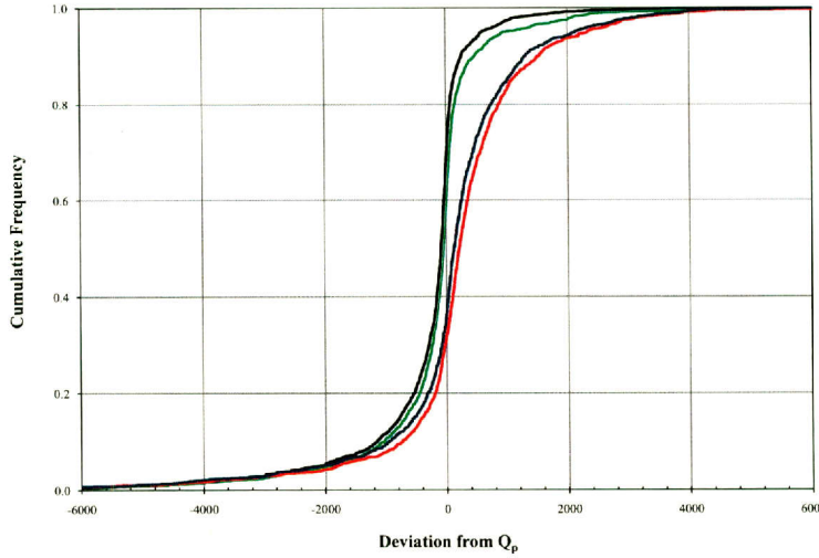
Figure D.7: Cumulative distribution of deviations (modeled Q_p - observed Q_p ) from Q_{p, \text{obs}} for Q_{p, \text{bc}} using Kerby-Kirpich and C_{vbc} (black curve), Q_{p, \text{lit}} using Kerby-Kirpich and C_{\text{lit}} (blue curve), Q_{p, \text{bc}} using square-root-area and C_{v, \text{bc}} (green curve) and Q_{p, \text{lit}} using square root of the drainage area and C_{\text{lit}} (red curve).
