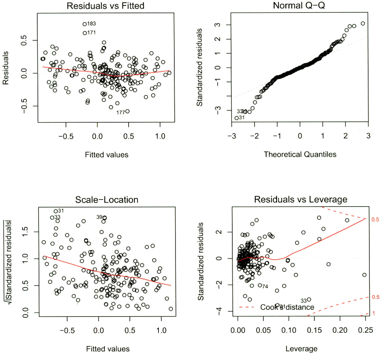
Figure C.4: Standard residual and diagnostic plots from the R environment using the plot.lm() function for the T_R regression equation.
