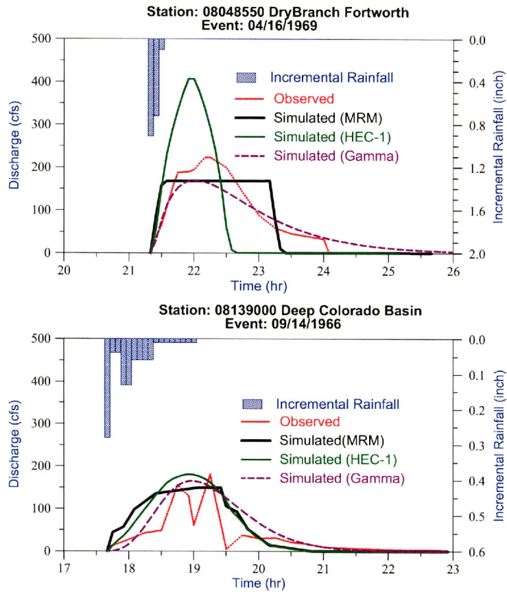
Figure D.9: Incremental rainfall hyetographs and observed (red) and simulated runoff hydrographs using the modified rational method (black), gamma unit hydrograph (purple) and Clark unit hydrograph (green). Upper panel is for the event on 4/16/1969 at the USGS streamflow-gaging station 08048550 Dry Branch, Fort Worth, Texas. Lower panel is for the event on 9/14/1966 at the USGS streamflow-gaging station 08139000 Deep Creek, Colorado Basin, Texas.
