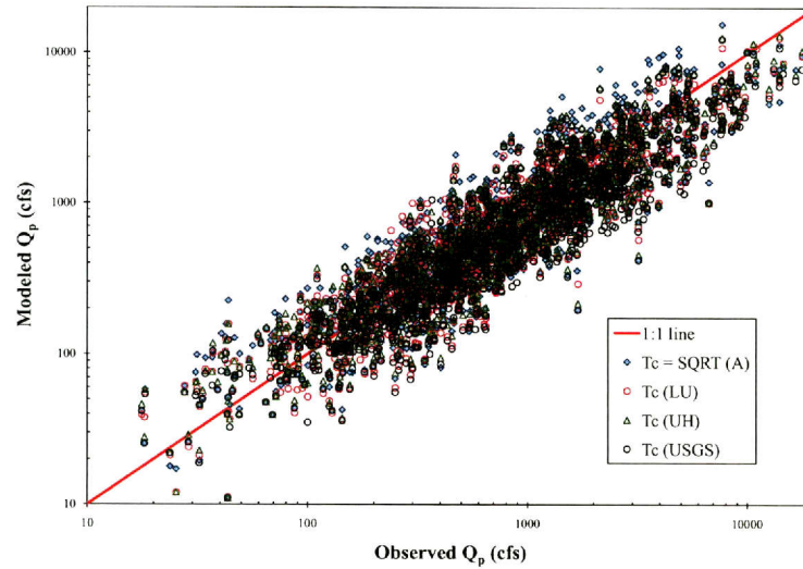
Figure D.2: Modeled and observed peak discharge from C_v^{bc} and different timing parameters.
