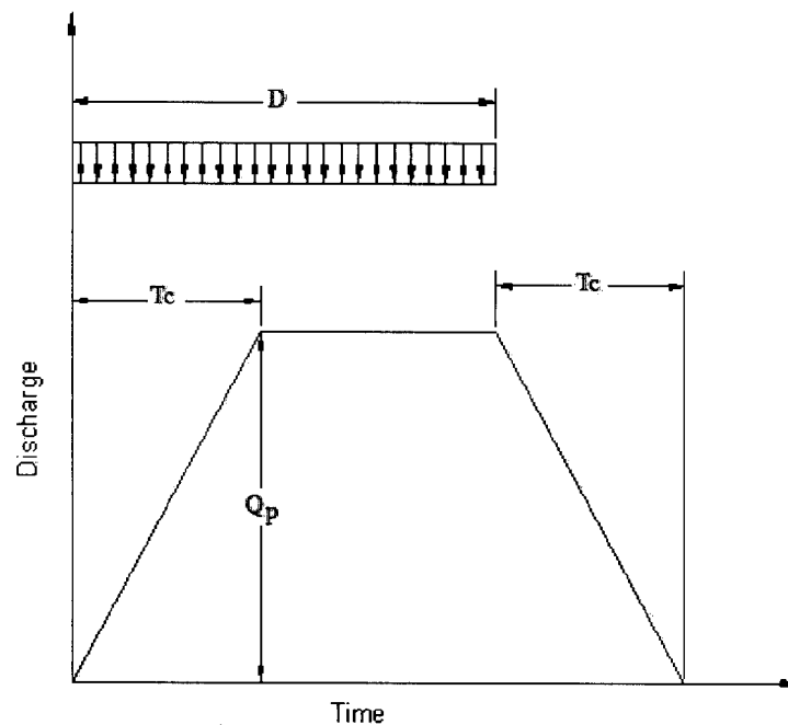
Figure 2.2: The MRM hydrograph when duration of rainfall is greater than T_c .
