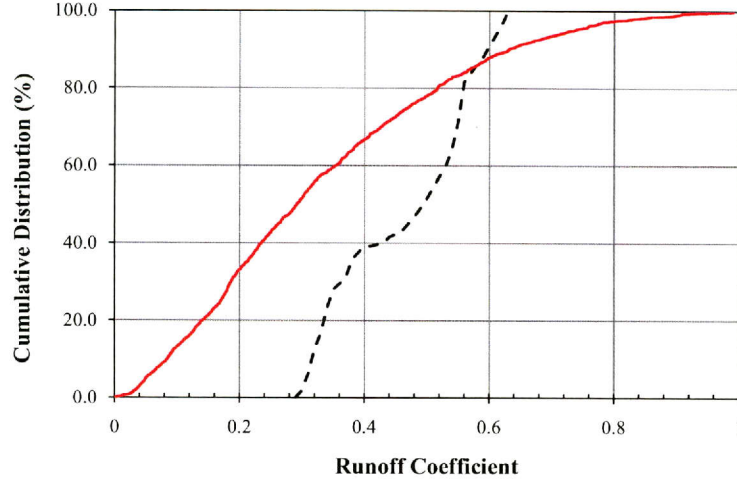
Figure D.1: Cumulative distributions of the runoff coefficients C_v^{bc} (red) and C_v^{lit} (black).
