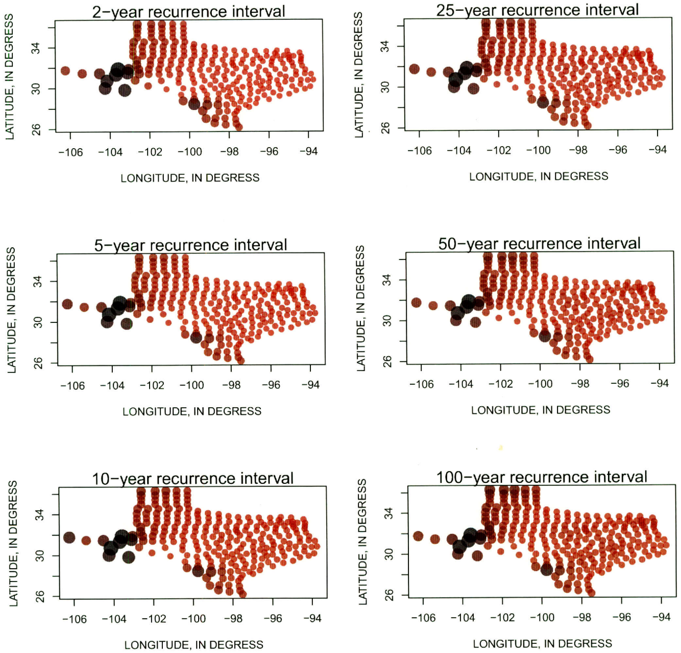
Figure 3.1: Intercept of regression by county for unified rational method in Texas. Increasing size and hue towards black indicates relatively higher values.
