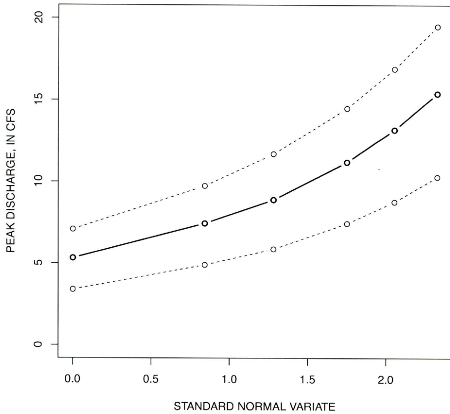
Figure 3.4: Estimated peak discharge frequency curves of Unified Rational Method for Texas for the Dickens county example. The thick line represents the \bar{Q}^* and is considered the best estimate of the peak-streamflow frequency curve. The dashed lines represent the upper and lower boundaries of the estimate by Q_U^* and Q_L^* , respectively.
