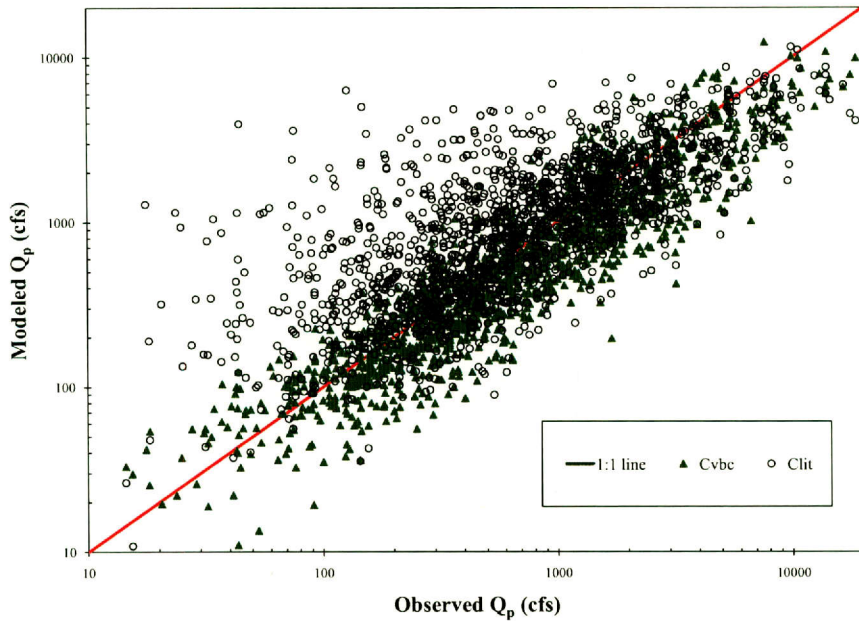
Figure 2.7: Modeled and observed peak discharge from C_v^{bc} (solid triangle) and C_v^{lit} (open circle) with timing parameters derived from the Kerby-Kirpich method.
