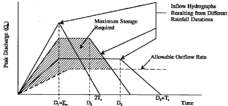
Figure A.2: Modified Rational Formula Hydrographs by Poertner (1974). Adapted from Thompson (2006).
