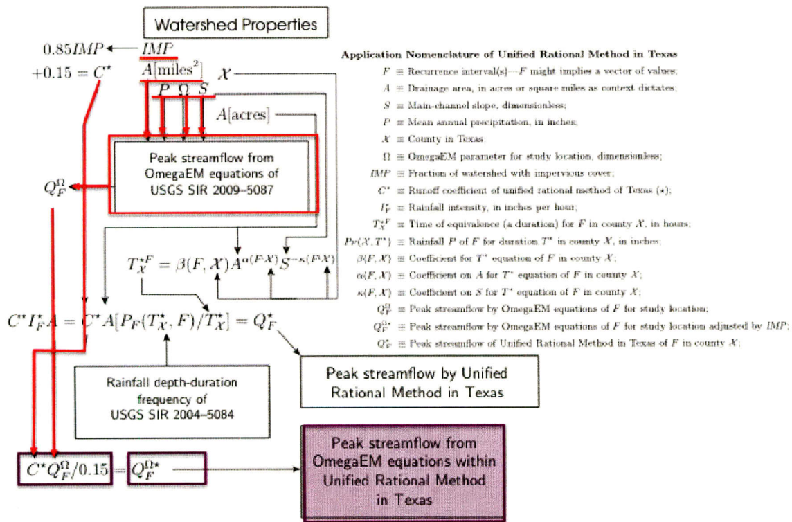
Figure 4.11: Unified Rational Method – Regression Equation Adjustment. Result is an adjusted peak discharge to reflect potential infrastructure additions in Texas for a specified frequency.
