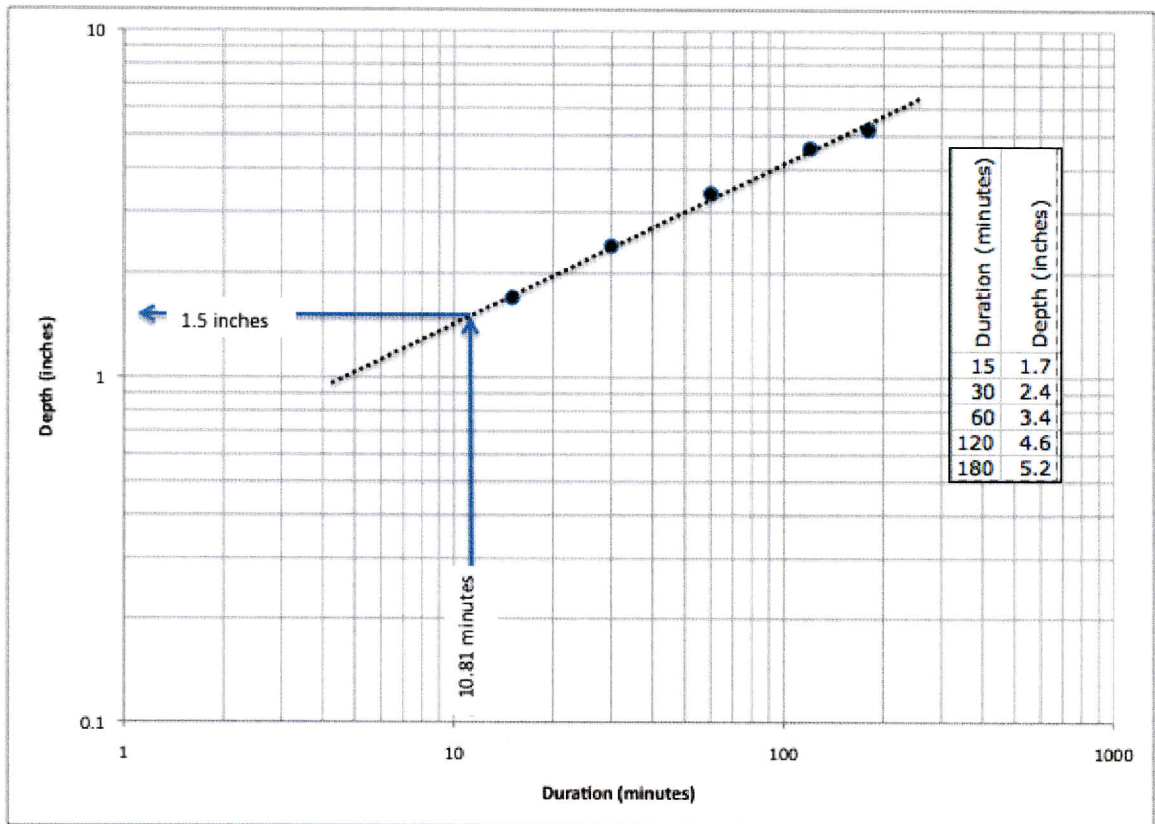
Figure 4.2: Depth-Duration diagram for Harris County for the application example. Values are from maps in Asquith and Roussel (2004). Dashed line is used to extrapolate mapped values to unmapped durations.
