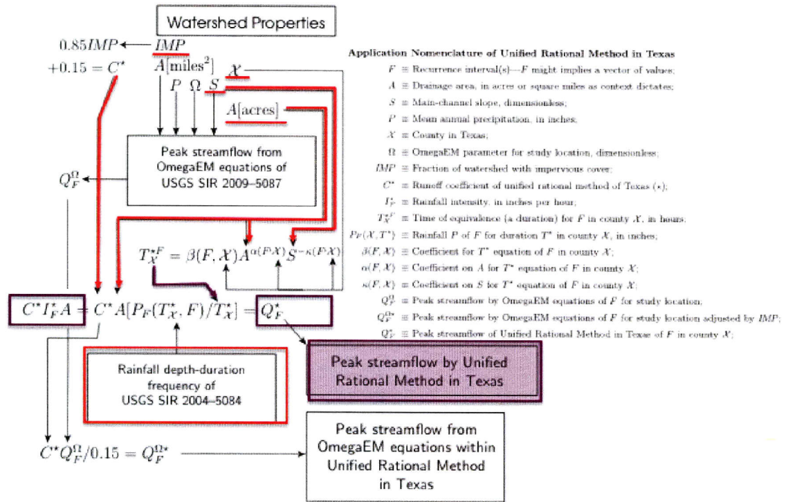
Figure 4.10: Unified Rational Method – Forward Modeling Pathway. Result is a peak discharge estimate for a location in Texas for a specified frequency.
