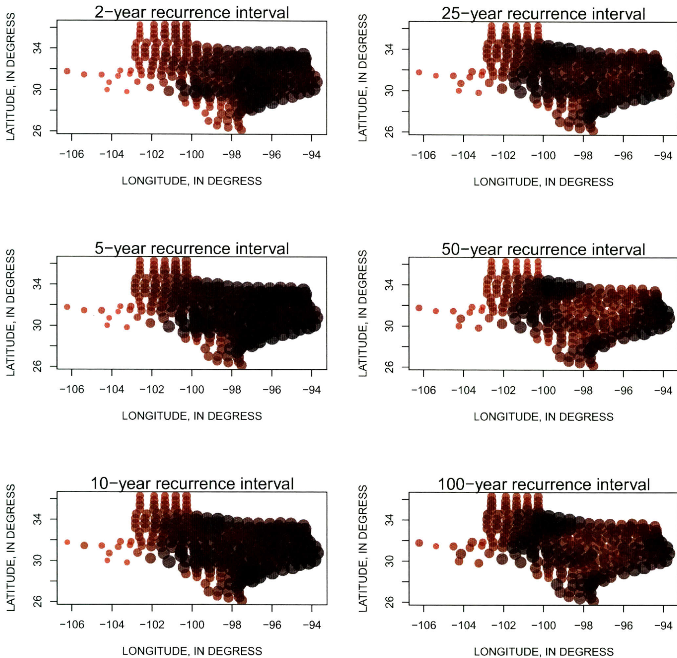
Figure 3.2: Exponent on drainage area for unified rational method in Texas. Increasing size and hue towards black indicates relatively higher values.
