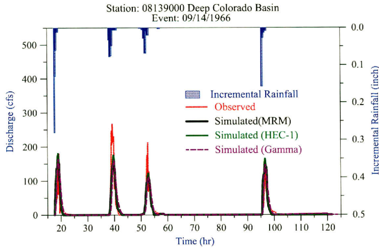
Figure D.10: Incremental rainfall hyetographs and observed (red) and simulated runoff hydrographs using the modified rational method (black), gamma unit hydrograph (purple) and HEC unit hydrograph (green) for USGS streamflow-gaging station 08139000 Deep Creek, Colorado Basin, Texas.
