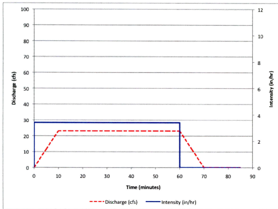
Figure 4.6: Modified rational method runoff hydrograph for example drainage area. Applied storm duration T_D = 60 minutes is six times the watershed characteristic time of T^* = 10 minutes. The peak discharge is Q_p = 23.1 cfs and is sustained for 50 minutes.
