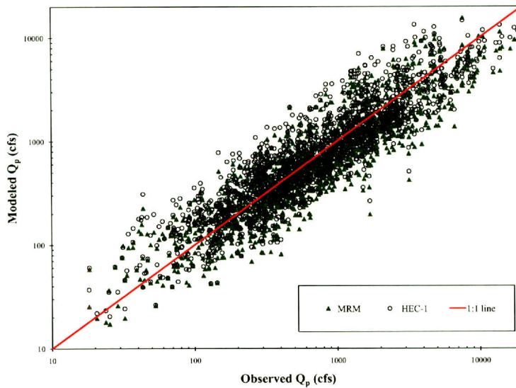
Figure D.11: Modeled and observed peak discharge from modified rational method (green) and HEC-1 unit hydrograph method (black).
