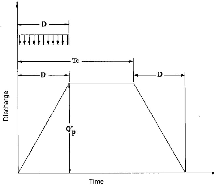
Figure 2.3: The MRM hydrograph when duration of rainfall is less than T_c .
