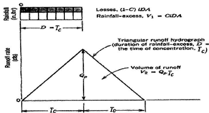
Figure 2.1: The MRM hydrograph when duration of rainfall is equal to T_c , from Wanielista and others (1997a).
