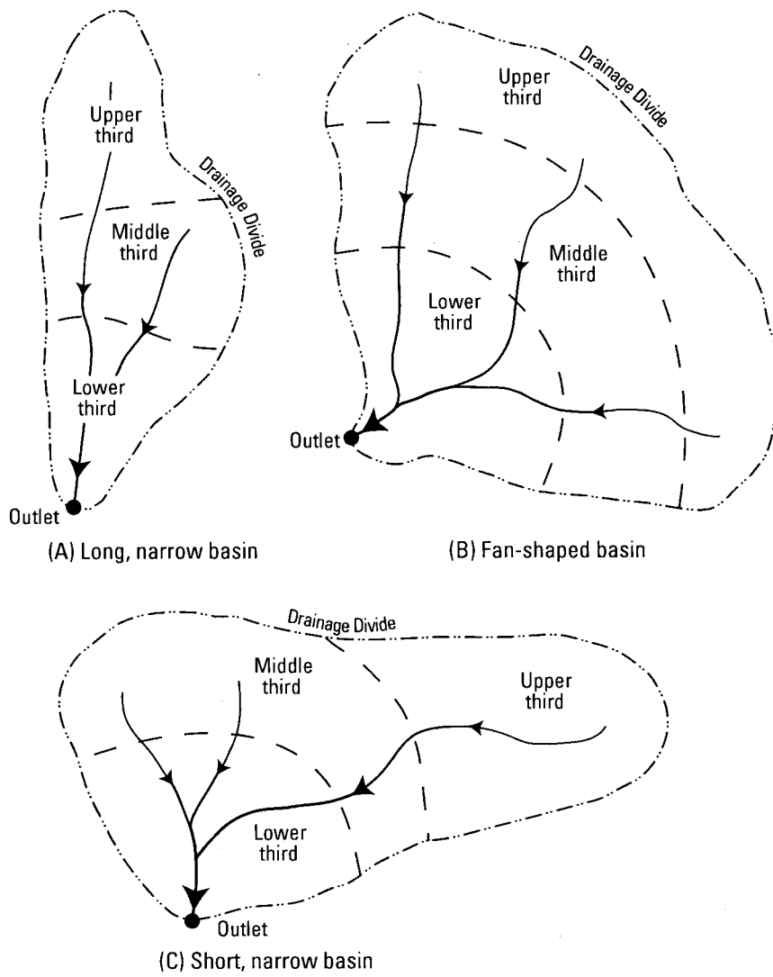
Figure B.1: Schematic of typical drainage basin shapes and subdivision into basin thirds.
