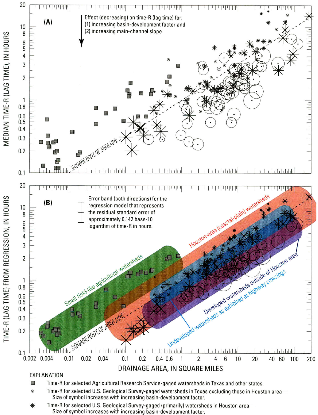
Figure C.5: Relation between Time-R and drainage area and basin-development factor by watershed type for observed (median, plot A) values and those estimated by regression (plot B).
