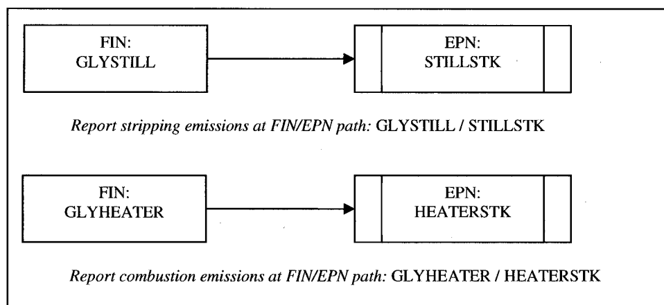
Figure 3-1. Glycol Unit—Separate Still and Heater Vents
