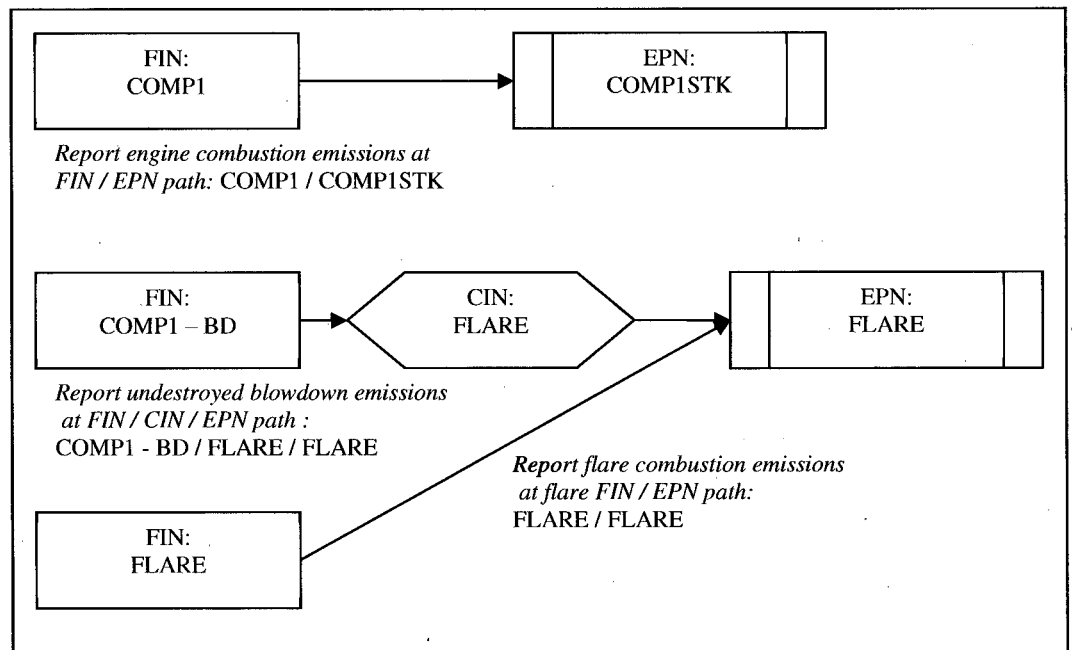
Figure 3-13. Blowdown Operations—Flared Blowdown Emissions
