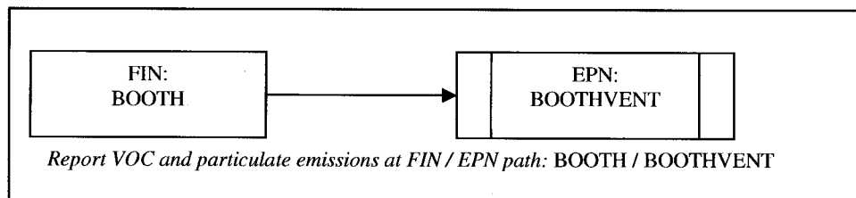
Figure 3-15. Paint Booth—Unabated
