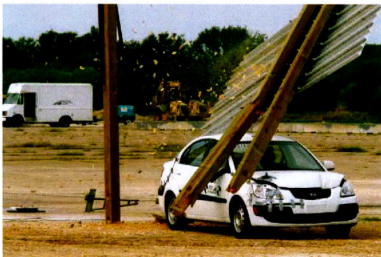
Figure B1. Sequential Photographs for Test No. 467823-1(Oblique and Perpendicular Views).
