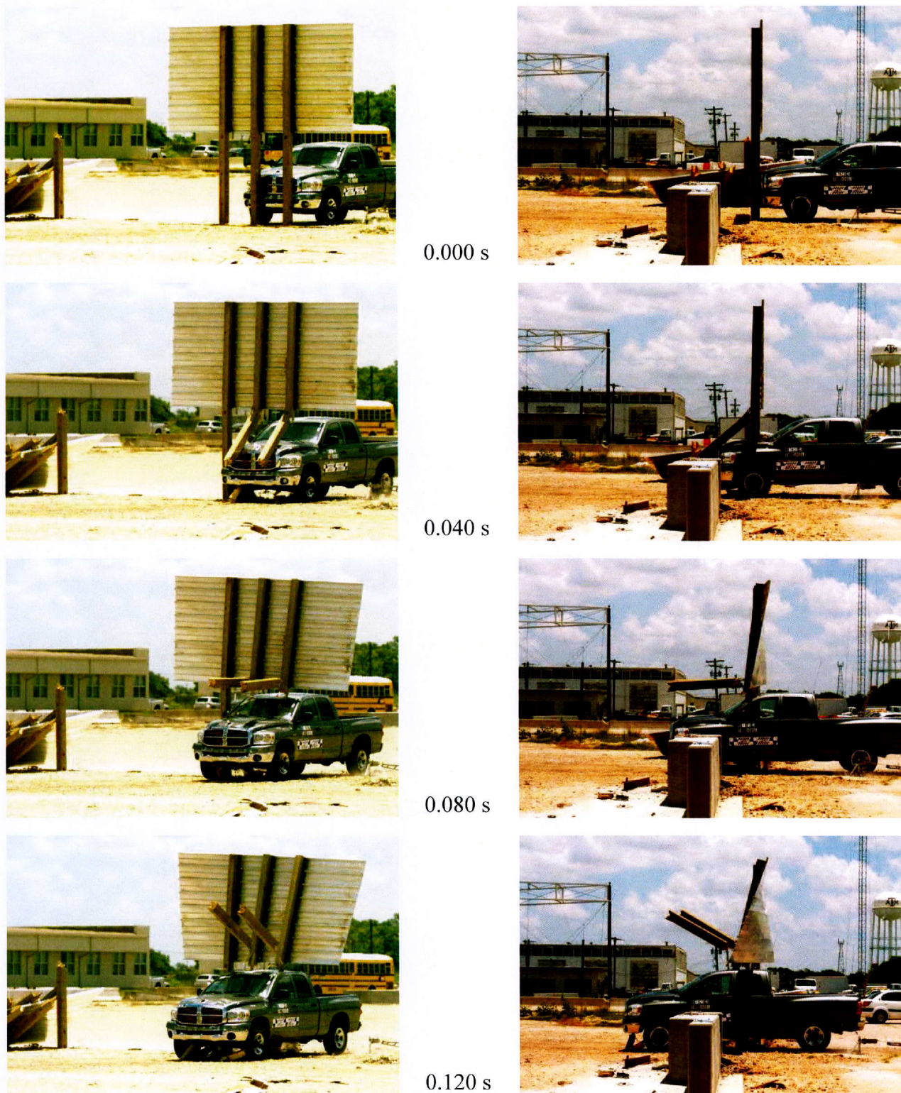
Figure F1. Sequential Photographs for Test No. 467823-3(Oblique and Perpendicular Views).
