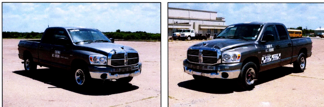
Figure 4.20. Vehicle after Test No. 467823-3.
