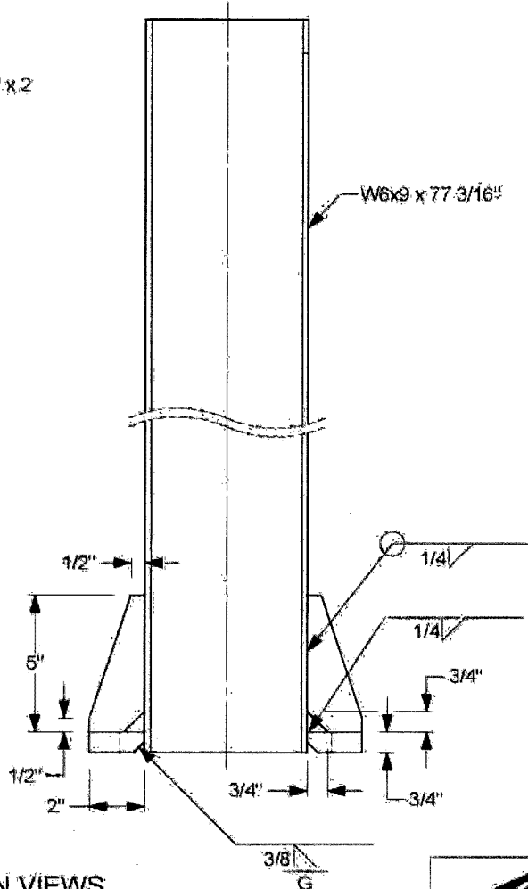
ELEVATION VIEWS
