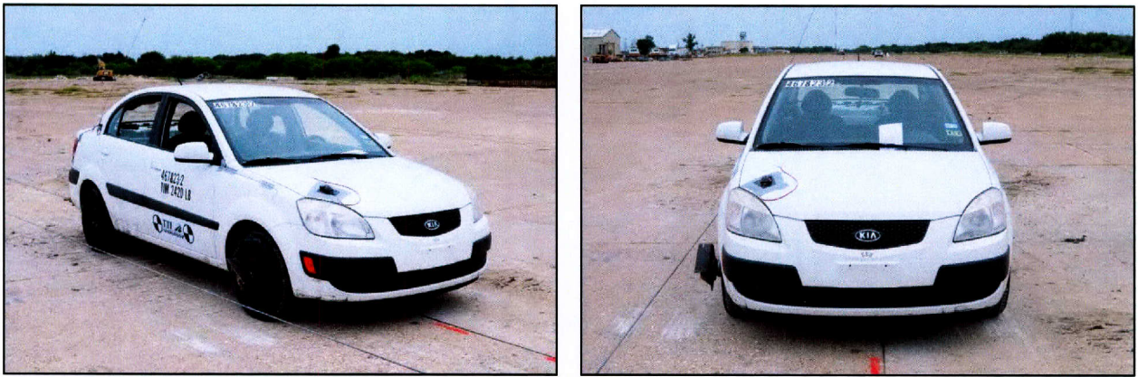
Figure 4.7. Vehicle before Test No. 467823-2.
