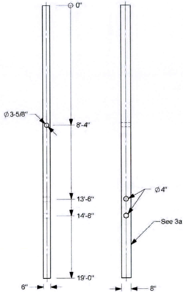
3a. Timber Post is rough-cut treated #1 yellow pine.
