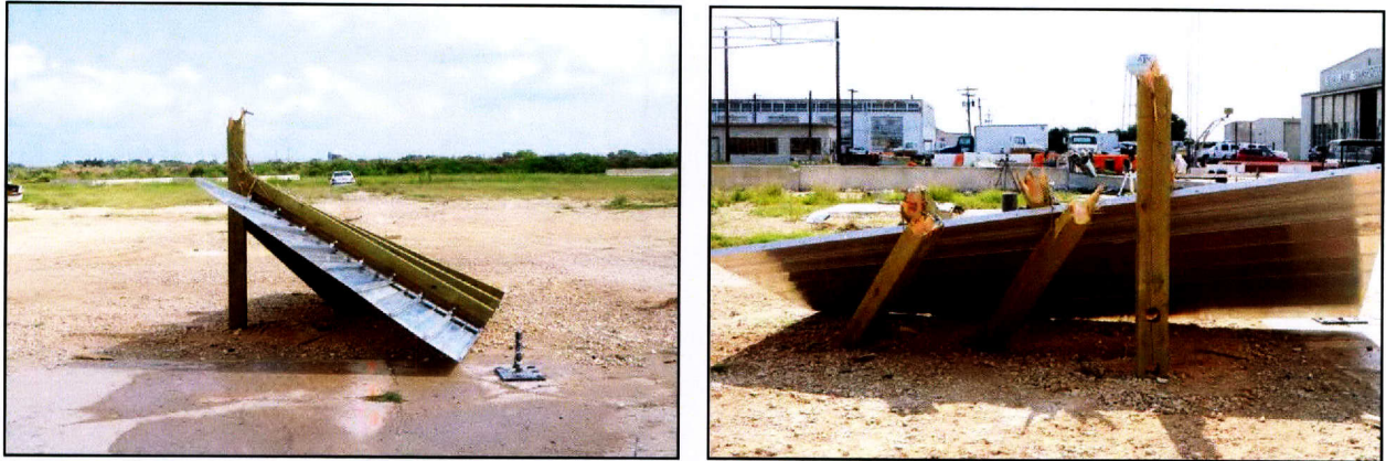
Figure 4.15. Modified Direct Embedded Wood Support Temporary Guide Sign System after Test No. 467823-2b.
