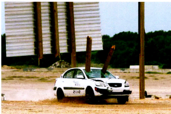
Figure C1. Sequential Photographs for Test No. 467823-2(Oblique and Perpendicular Views).
