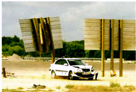
Figure E1. Sequential Photographs for Test No. 467823-2b (Oblique and Perpendicular Views) (Continued).
