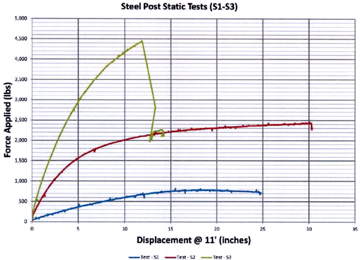
Figure 5.1. Static Test Results for S3×5.7 (Test S1), W6×9 (Test S2), and W8×18 (Test S3).
