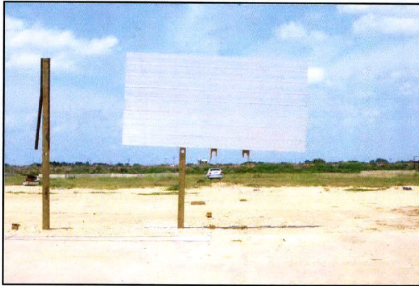
Figure 4.8. Direct Embedded Wood Support Temporary Guide Sign System after Test No. 467823-2.
