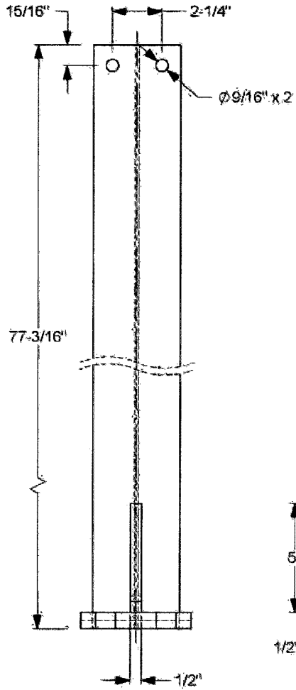
ELEVATION VIEWS
