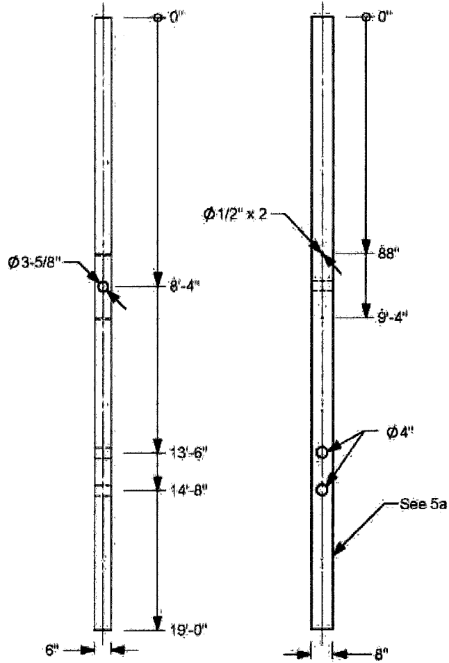
5a. Timber Post is rough-cut treated #1 yellow pine.
