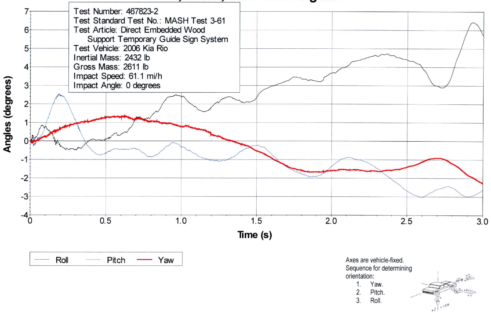
Figure C2. Vehicle Angular Displacements for Test No. 467823-2.
