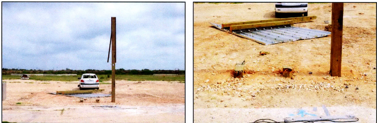
Figure 4.4. Direct Embedded Wood Support Temporary Guide Sign System after Test No. 467823-1.
