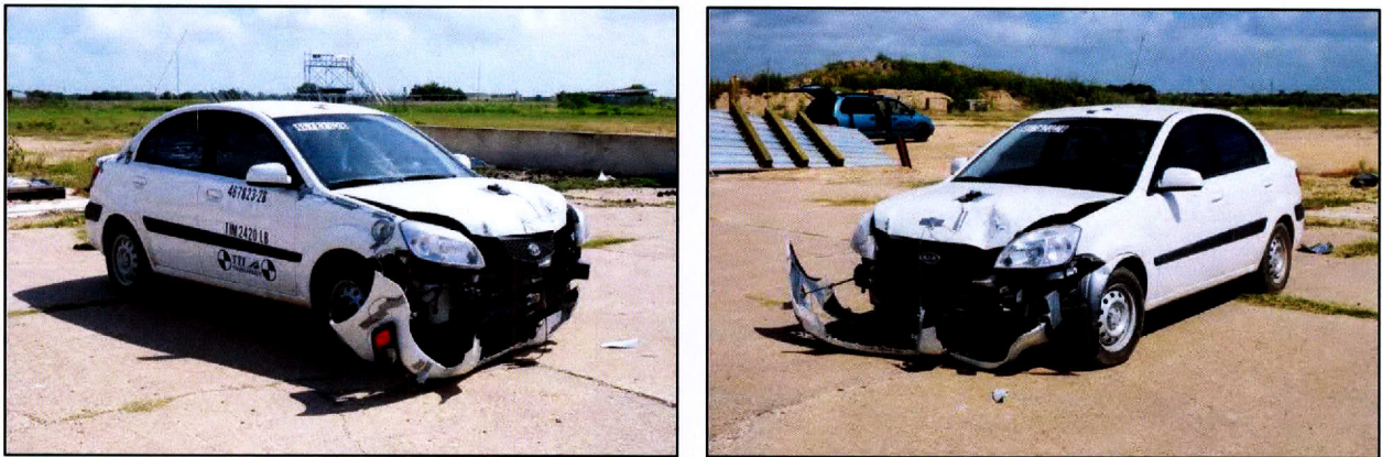
Figure 4.16. Vehicle after Test No. 467823-2.
