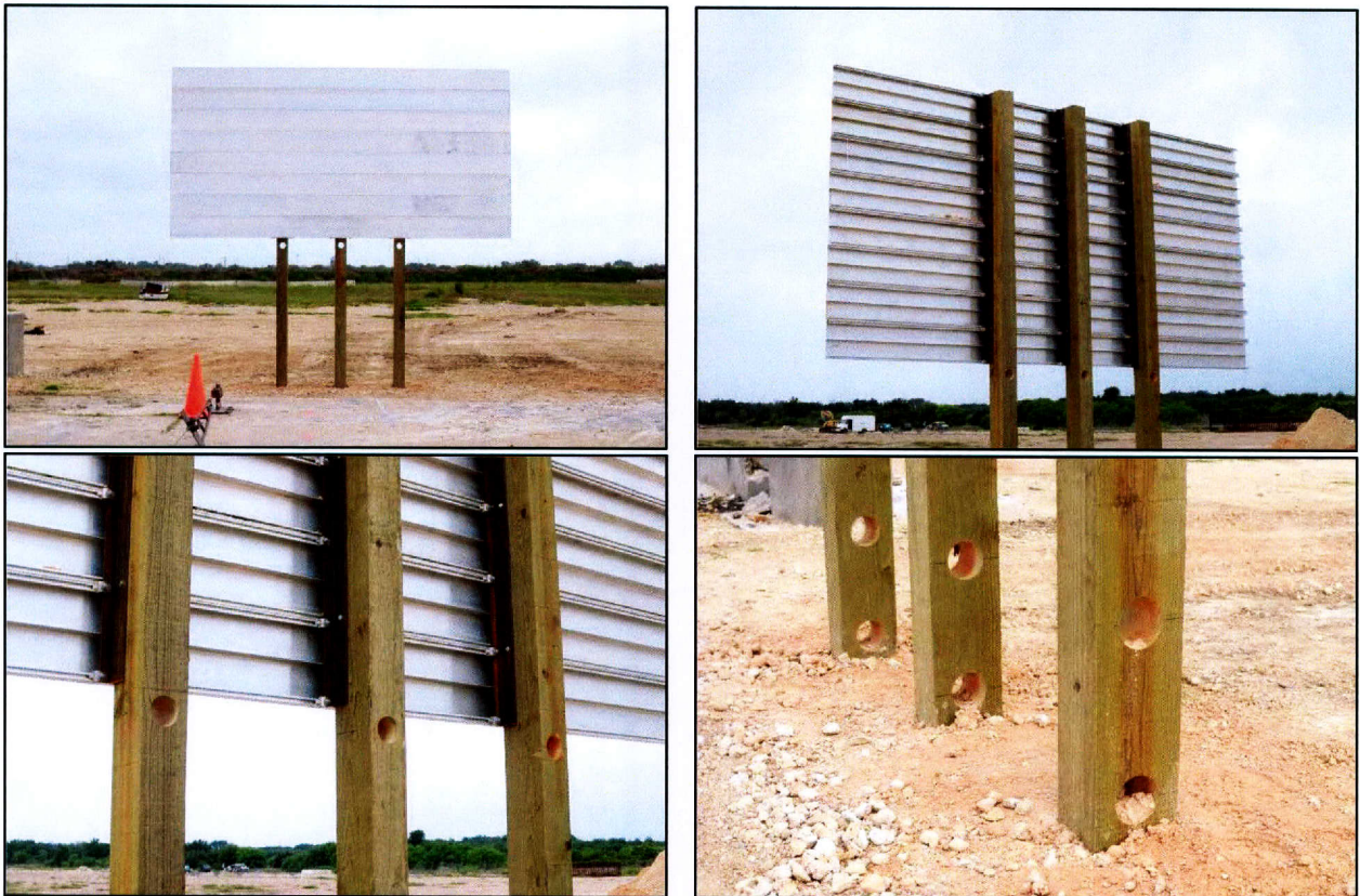
Figure 4.2. Direct Embedded Wood Support Temporary Guide Sign System before Test Nos. 467823-1 and 467823-2.
