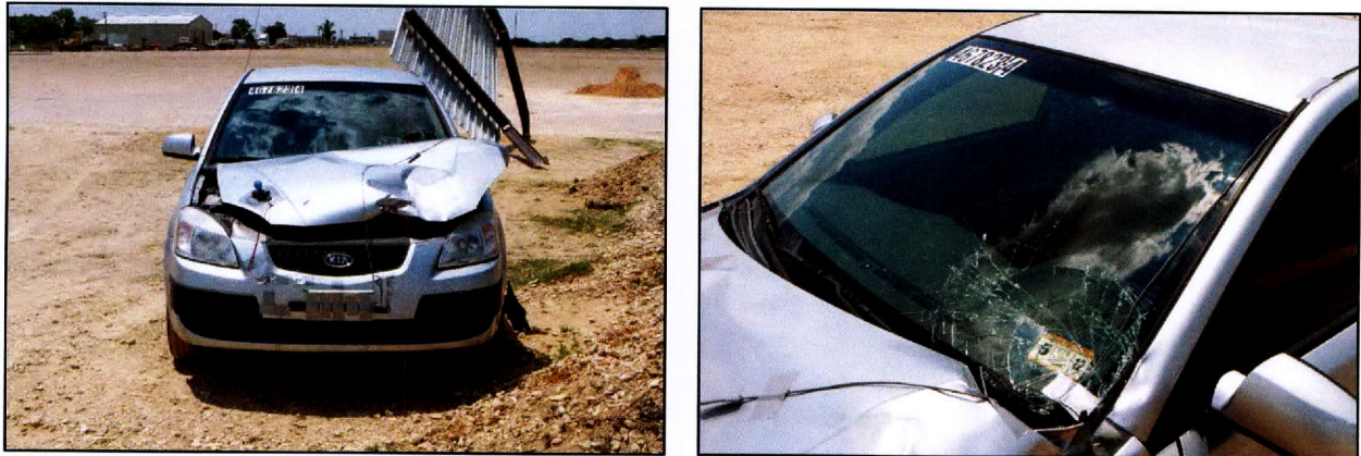
Figure 5.6. Vehicle after Test No. 467823-1.
