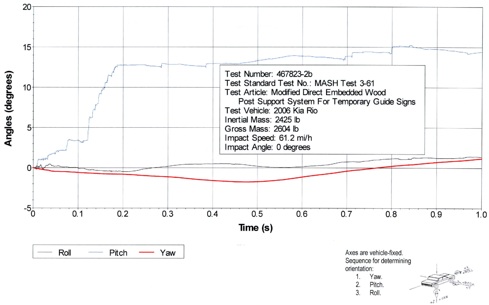
Figure E2. Vehicle Angular Displacements for Test No. 467823-2b.
