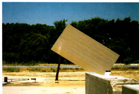
Figure H1. Sequential Photographs for Test No. 467823-4 (Oblique and Perpendicular Views) (Continued).
