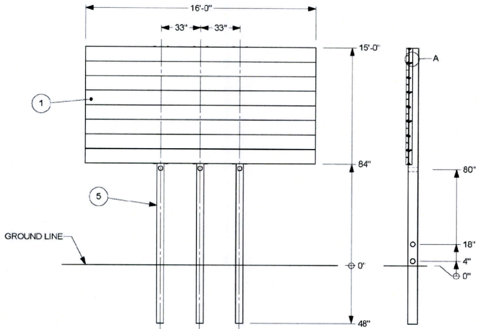
Figure 4.1. Overall Details of the Direct Embedded Wood Support Temporary Guide Sign System.
