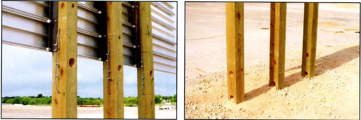
Figure 4.13. Modified Direct Embedded Wood Support Temporary Guide Sign System before Test Nos. 467823-2b and 467823-3.
