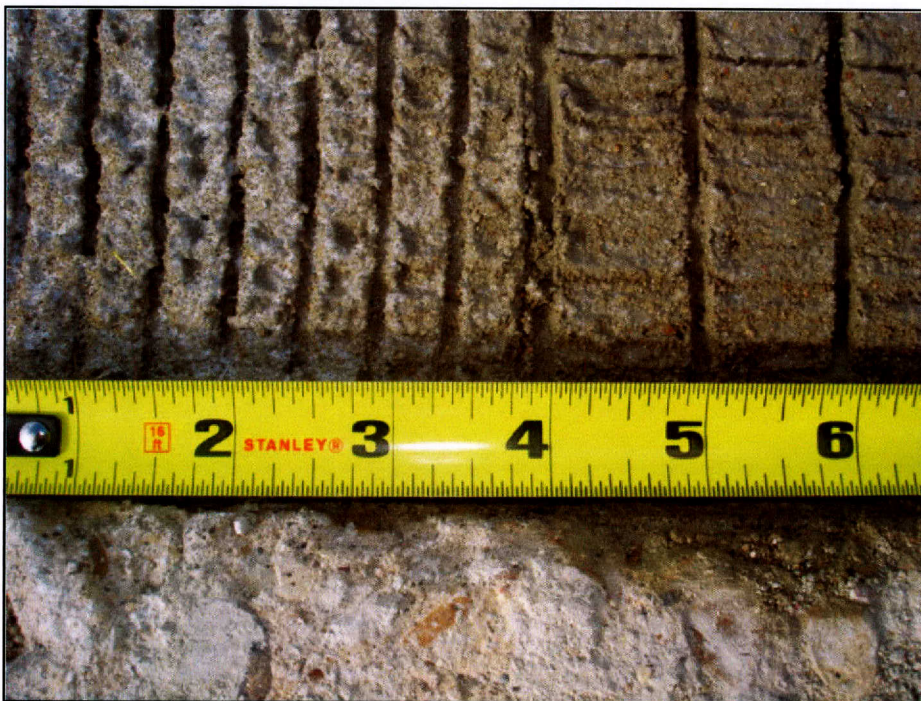
Figure 41. Change from ½-inch to 1-inch Transverse Tines.
