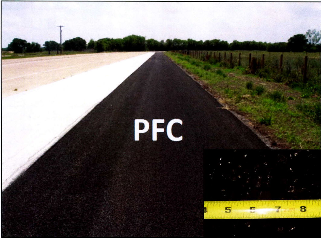
Figure 54. Permeable Friction Course Section.
