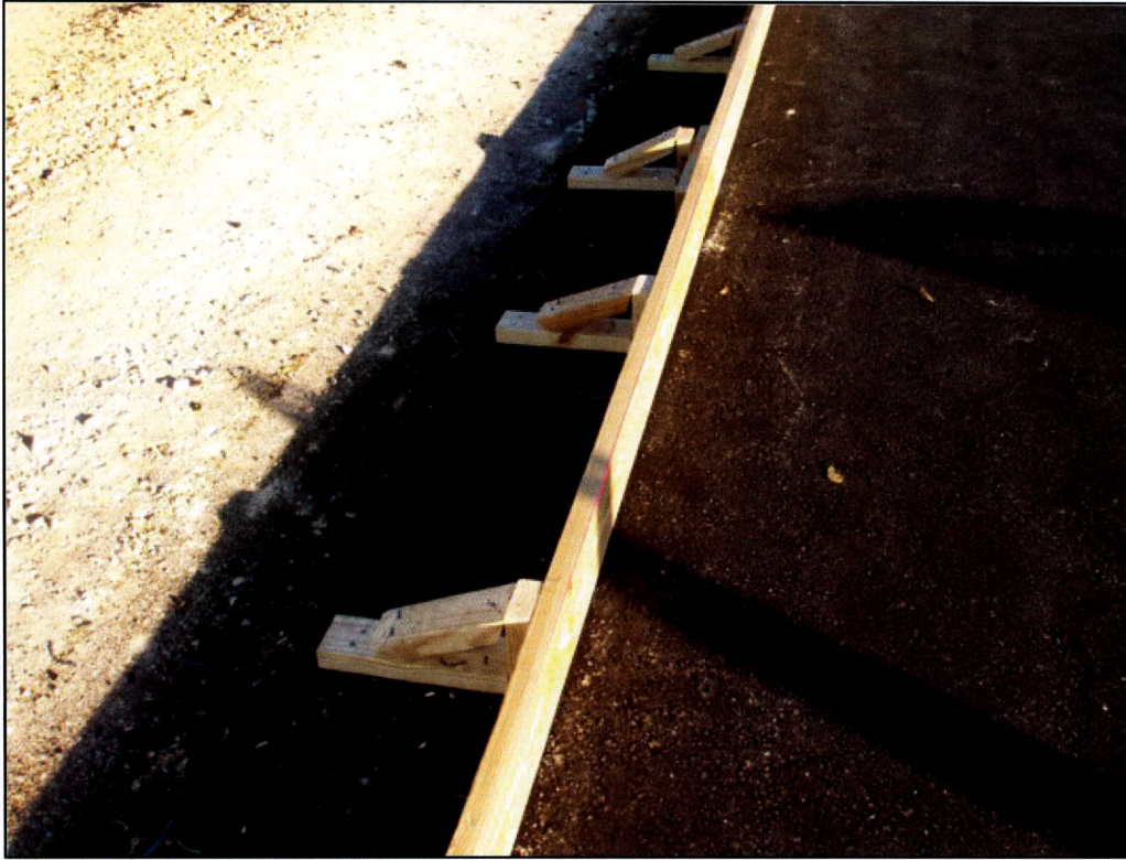
Figure 33. Form along West Side of Type C Base to Place CRCP.
