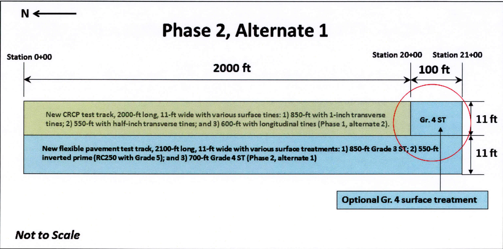
Figure 10. Plan View of Phase 2 Construction of Flexible Pavement Test Track Using Alternate 1, and Construction of Optional Grade 4 Surface Treatment at South End of 2000-ft CRCP Test Track Built under Phase 1, Alternate 2.
