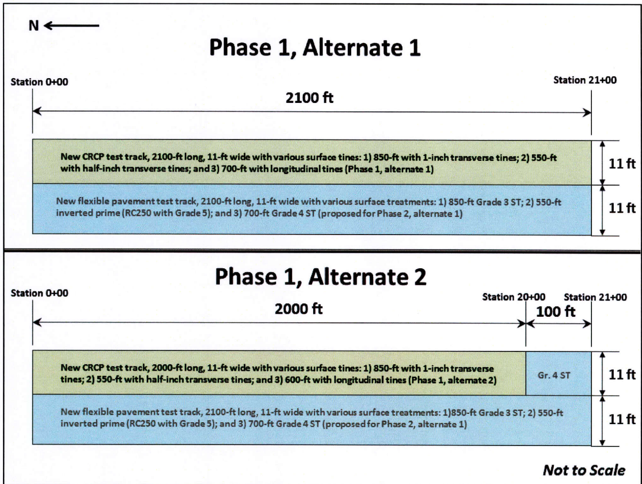
Figure 6. Plan View of Alternates for Construction of CRCP Test Track in Phase 1.
