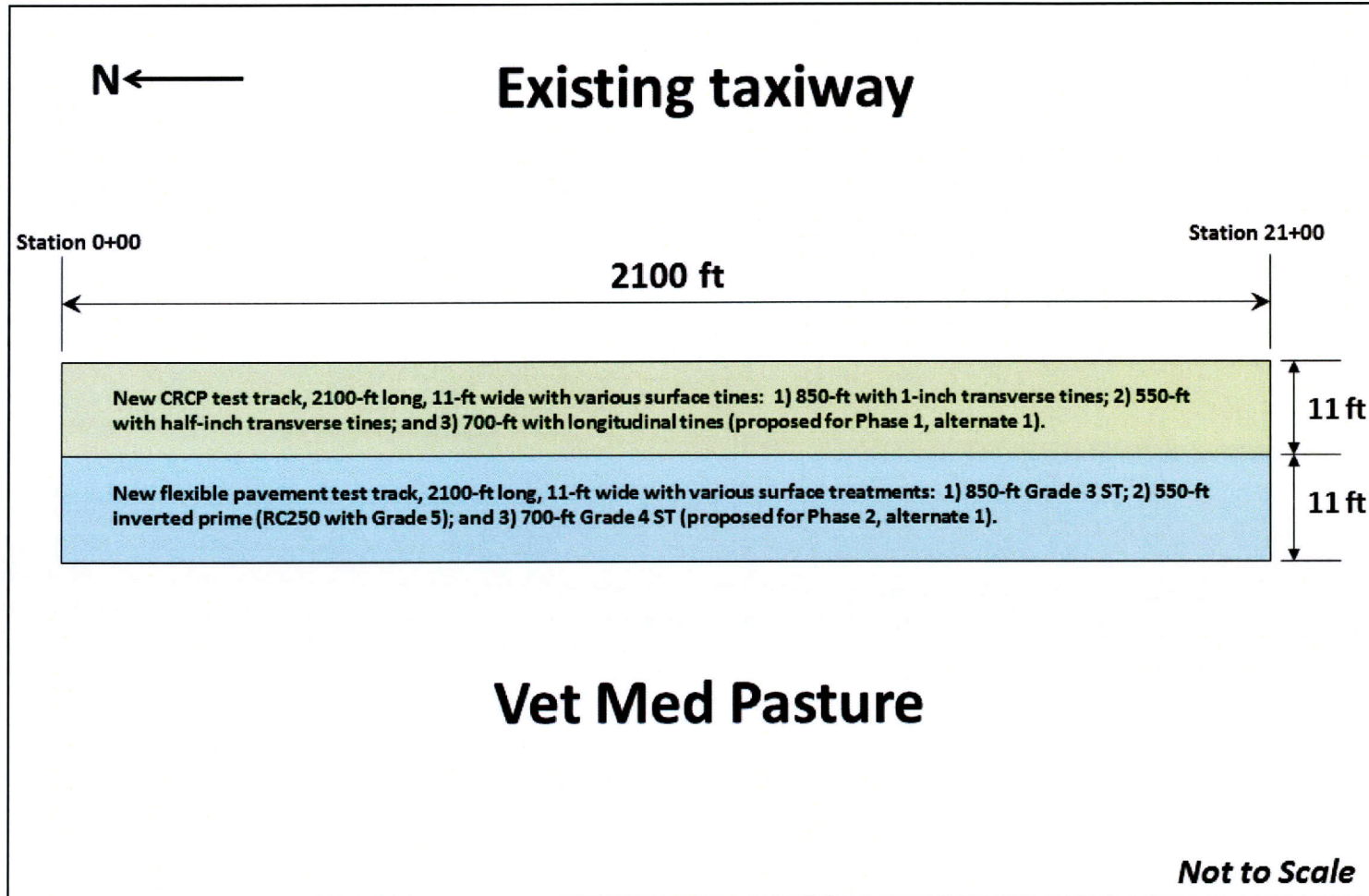
Figure 5. Plan View of Proposed New Test Tracks.
