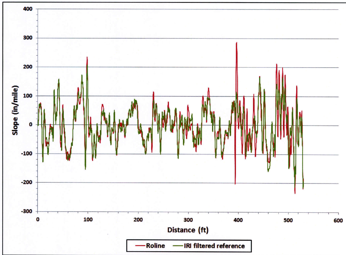
Figure 58. Comparison of IRI Filtered Profiles on a Section of CRCP Test Track.
