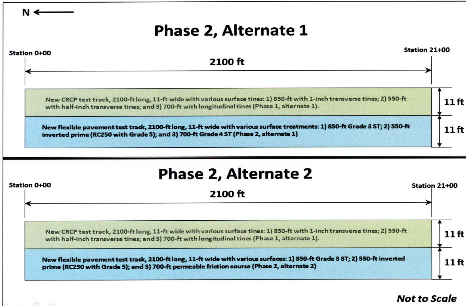
Figure 9. Plan View of Two Alternates for Construction of Flexible Pavement Test Track in Phase 2.
