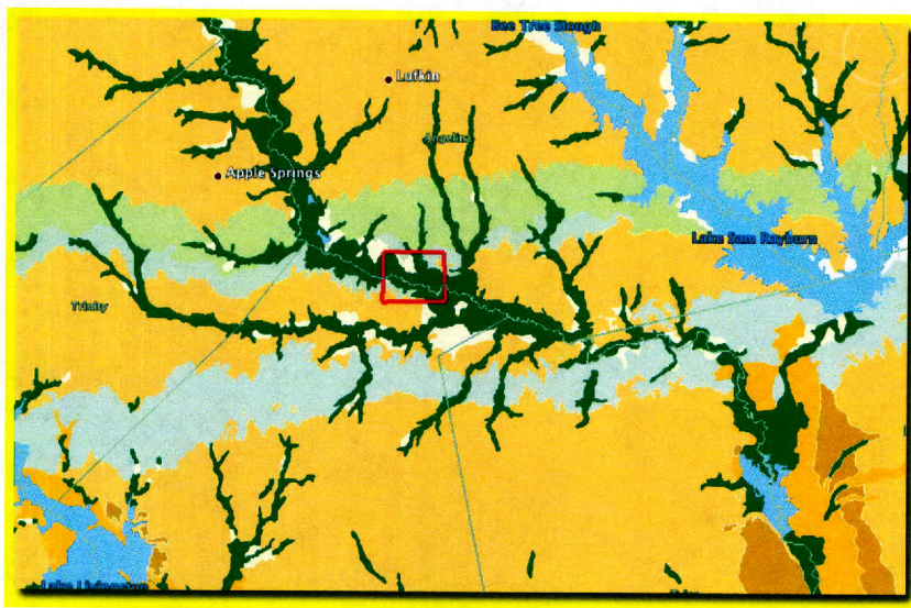
Figure 5.11. Intermediate location map on Texas Bureau of Economic Geology Google Earth geology map. Dark green areas are Holocene alluvium.
