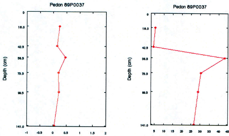
Figure 5.23. Data for the Telferner soil series ( % organic C to the left, and % clay to the right).
