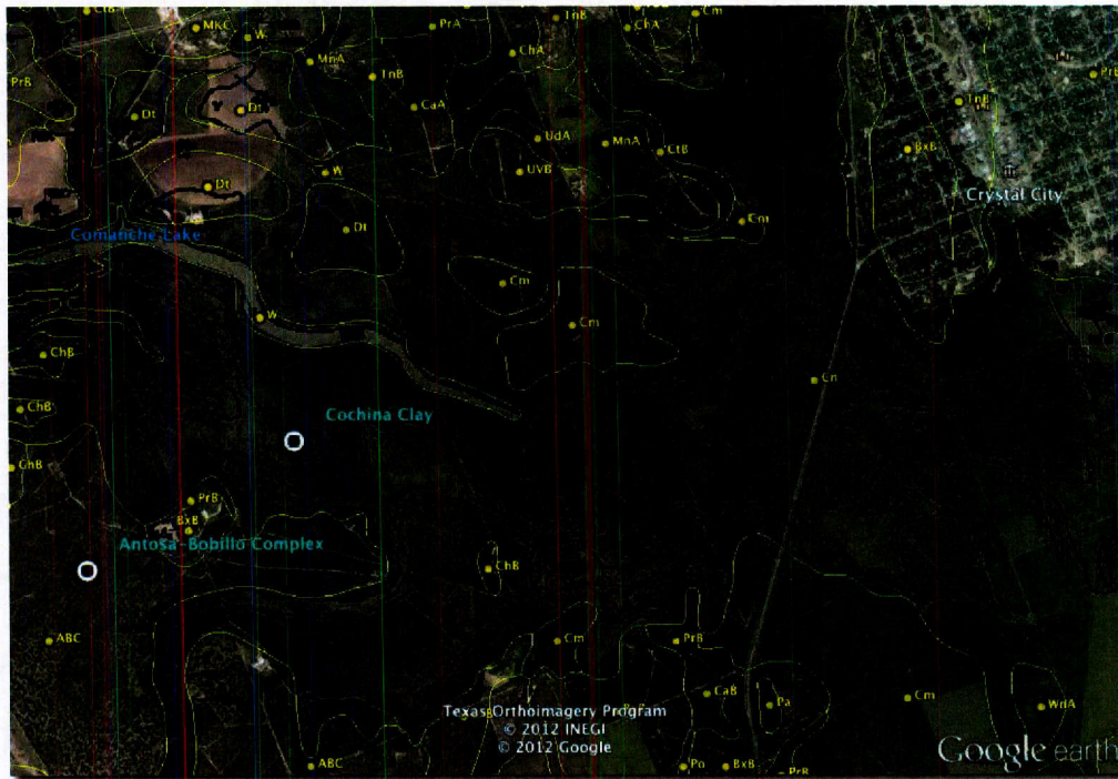
Figure 5.25. Geologic Context of the West Nueces River transect.
