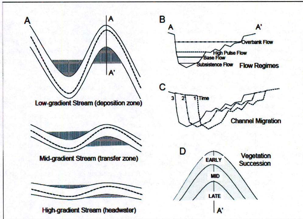
Figure 2.2. Schematic of river systems depicting A) river sinuosity and development of point bars on which riparian vegetation will establish, thalweg is shown as dotted line; B) flow regime levels; C) channel migration scenarios at meander bend; and D) riparian vegetation establishment on the point bar over time relating to channel migration (modified from BBEST 2011).
