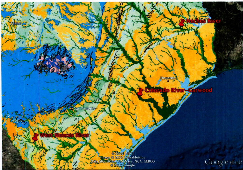
Figure 5.9. Location of the three soil-wetland transects on the Texas Coastal Plain. Texas geologic map, USGS. The Balcones Escarpment parallels the western contact between the blue and tan colors.
