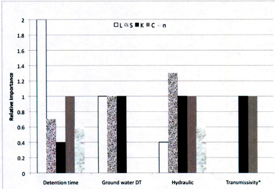
Figure 3.1. Relative importance of length or buffer width (L), slope (S), hydraulic conductivity (K), soil moisture storage capacity (C), and roughness (n) for the detention time, ground water detention time, hydraulic, and transmissivity indices of buffer effectiveness (*transmissivity is a function of conductivity and soil depth or thickness).
