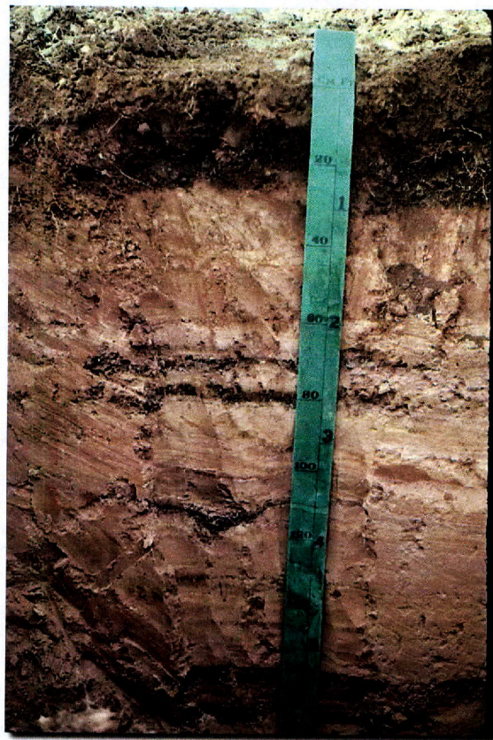
Figure 5.1. A “typical” riparian soil with relatively unaltered bedding planes. Coarsewood Series. J Jacob photo.
