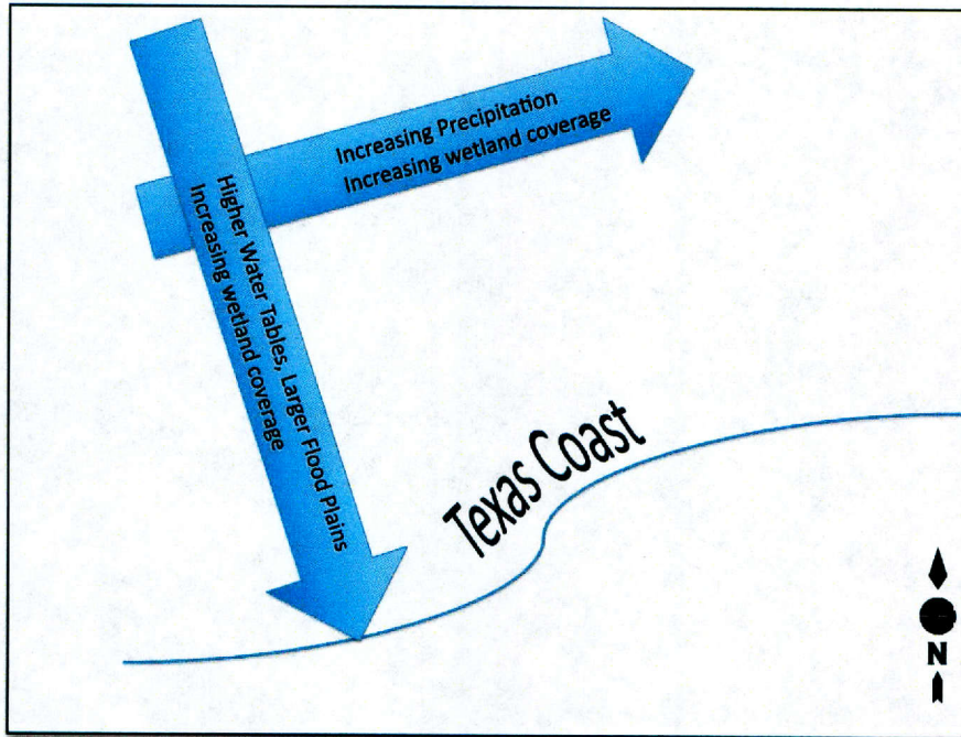
Figure 5.8. Longitudinal axes across and along the Texas coastal plain indicating relative distribution of wetland coverage on floodplains.
