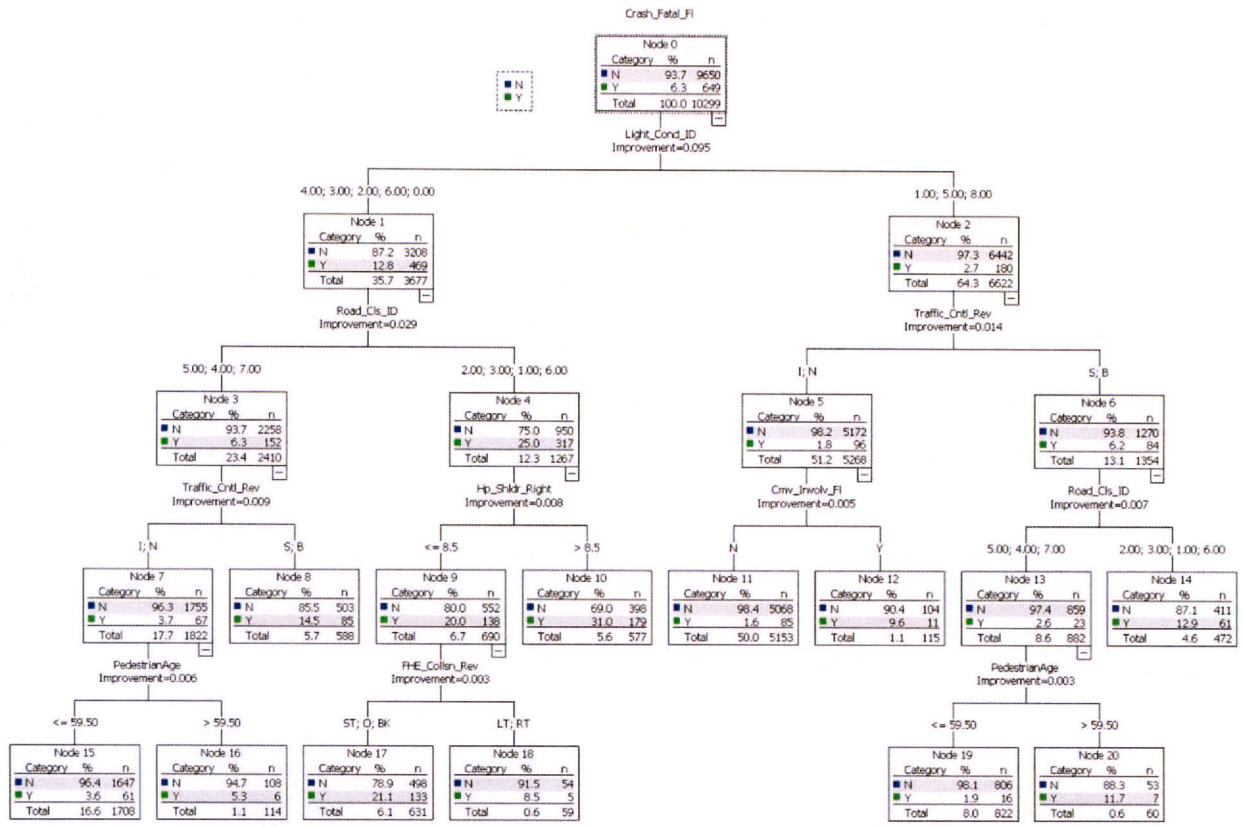
Figure 62. Classification Tree.
