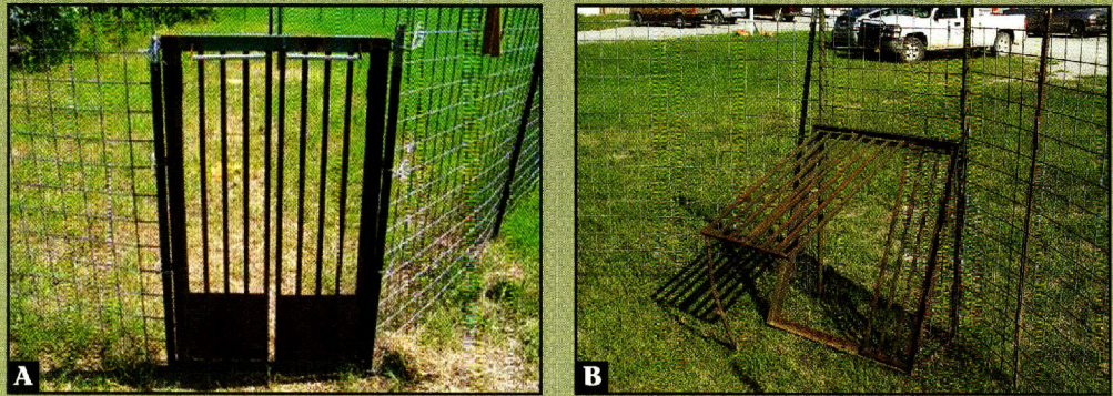
Swing gates require springs for closing (A). Lifting doors can be set in an open position like a drop gate, and once triggered, more hogs can push their way inside the trap (B). After triggering, the gate will close but permit more hogs to enter.
